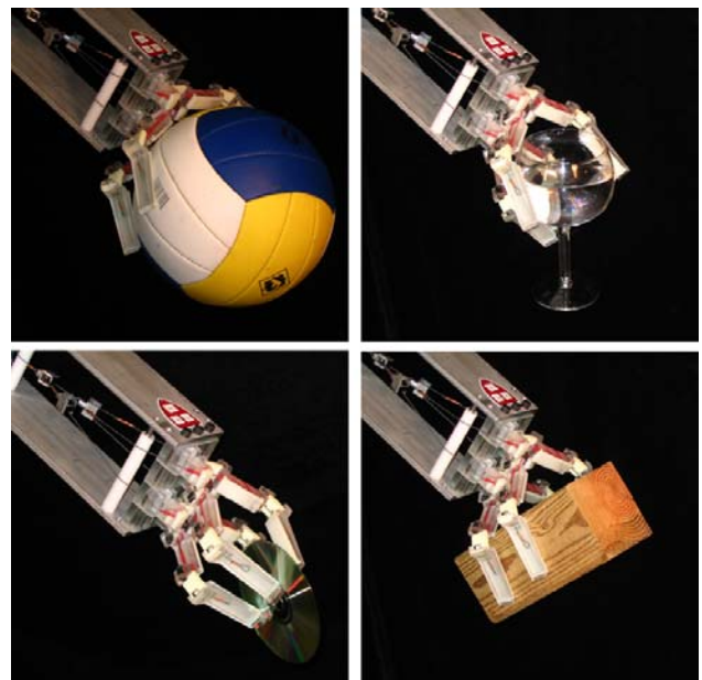
Fig. 2. Four-fingered SDM grasping a volleyball, a wine glass filled with water, a compact disc, and a large wood block.
