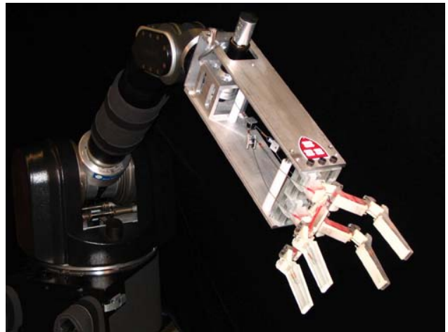
Fig. 1. Four-fingered, underactuated SDM hand mounted on a Whole-Arm Manipulator (Barrett Technology Inc., Cambridge, MA, USA). A single motor drives all eight joints of the hand
