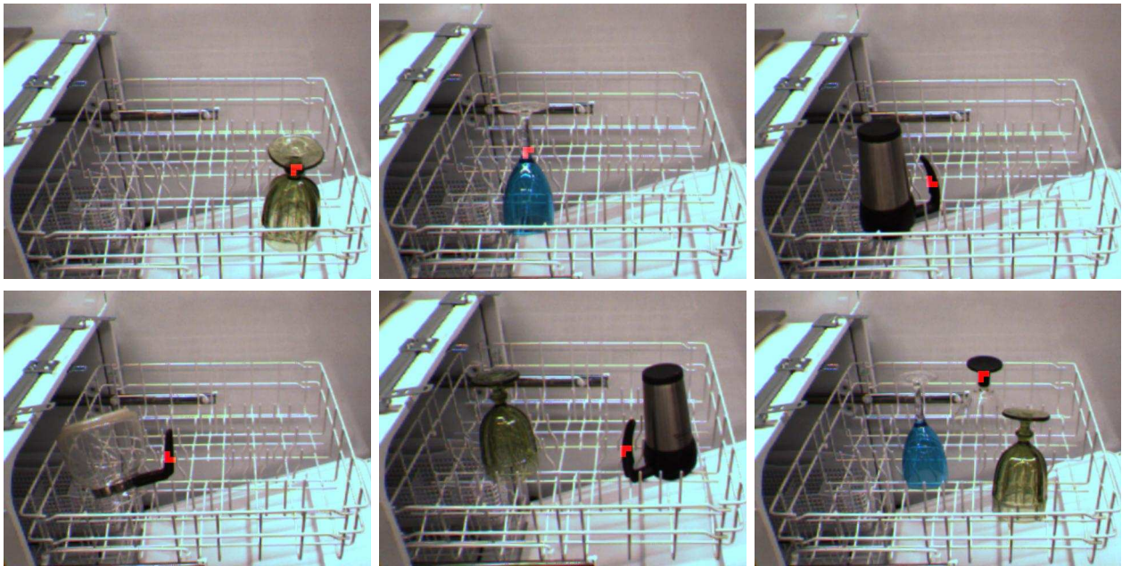
Fig. 6. Grasping point classification (shown in red) for objects placed in dishwasher. In case of multiple objects, the algorithm picks one it thinks is the best.
