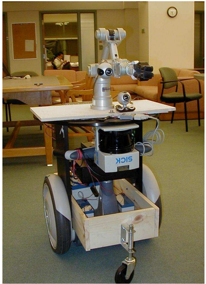
Fig. 7. The robot arm mounted on a mobile base. The 5-dof arm was used to pick up the objects.
