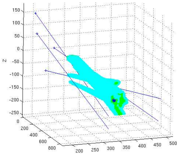
Fig. 4. Statistical Triangulation of the grasping point. The dark blue lines, originating from the camera locations, show the camera direction. Light blue shows the Gaussian cones for the candidate grasp regions. The dark blue spot is the predicted grasping point.
