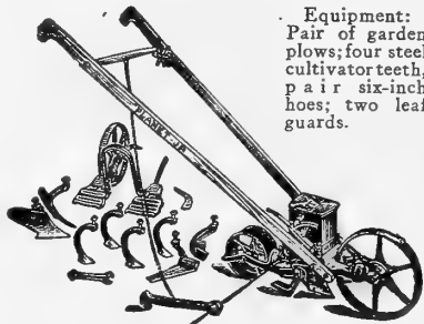
NO. 3 AND NO. 5.—HILL AND DRILL SEEDERS.
