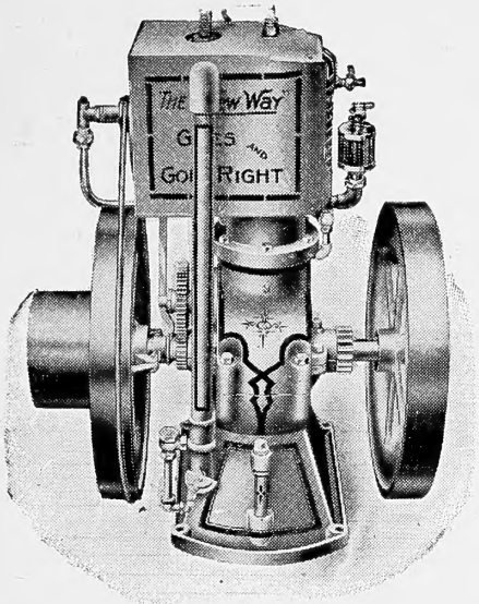
Style of Sizes, 2½, 3¼, 4½ and 6 H. P. 8 and 12 H. P. opposed cylinder
