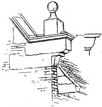
MERSTONE, ISLE OF WIGHT
