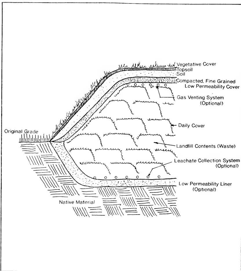
Legend Generalized Landfill Structure (Cross Section) FIGURE 2 LANDFILL REVEGETATION MANUAL
