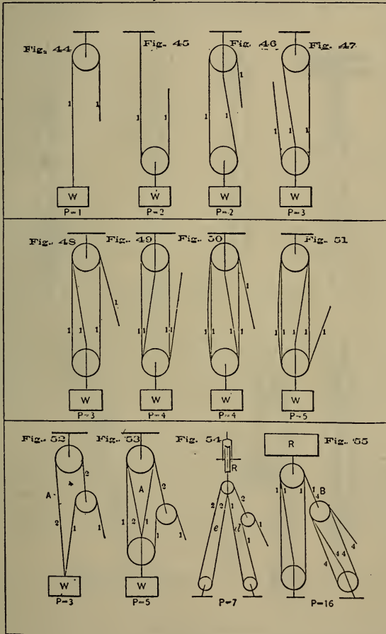
Purchase by Block and Tackle. Plate 1.
