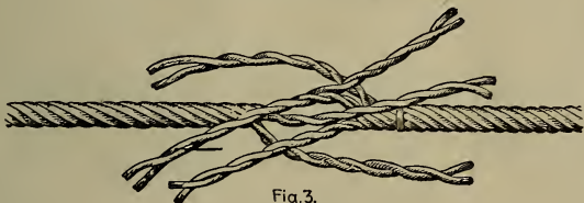
Fig. 3. 2 d Method. Long Splice in Wire.
