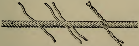
Fig. 4. 2 d Method. Long Splice in Wire.
