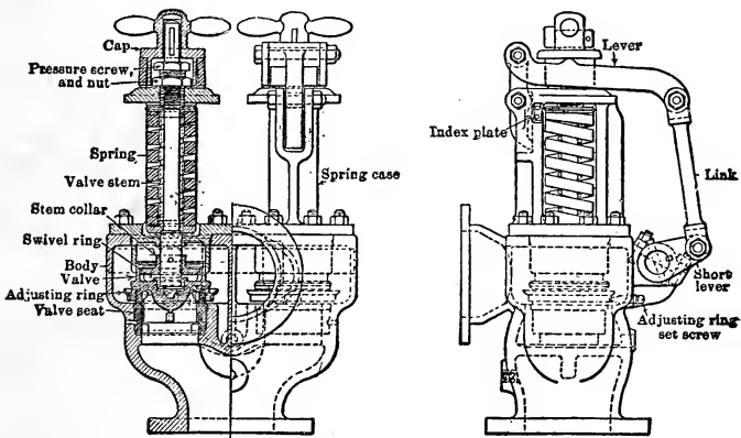
Duplex Safety Valve, showing Names of Parts
