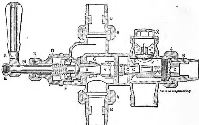
INJECTOR
