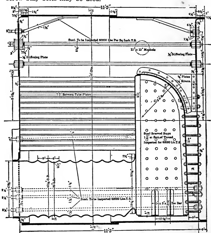
Fig. 11. Scotch Boiler, Longitudinal Section
