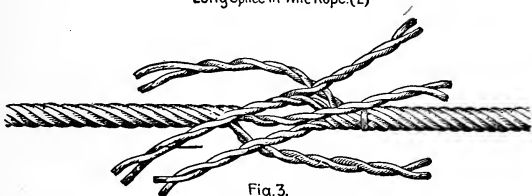
Fig. 3. 2 d Method. Long Splice in Wire.
