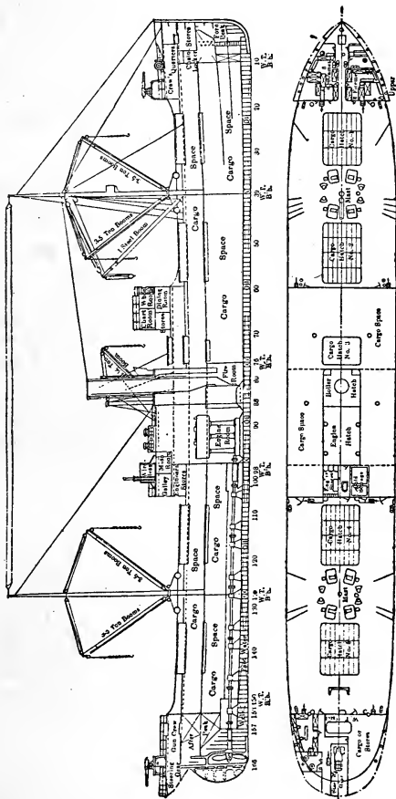
Longitudinal Section. Emergency Fleet Standard Steel Steamship. 7,300 tons dead weight capacity. 11½ knots sea speed.
