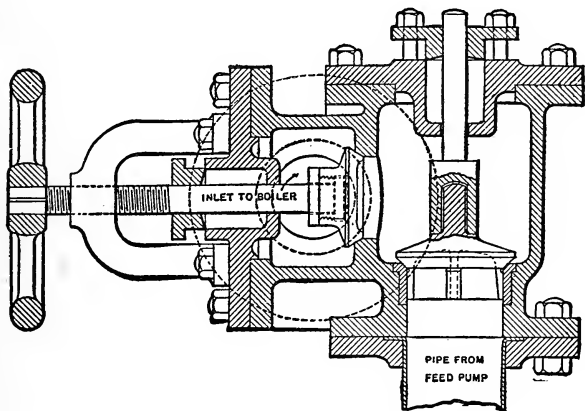
Combined Check and Stop Valve
