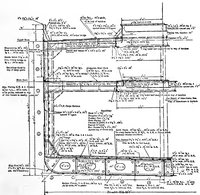
Midship Section. Standard Steel Steamship.
