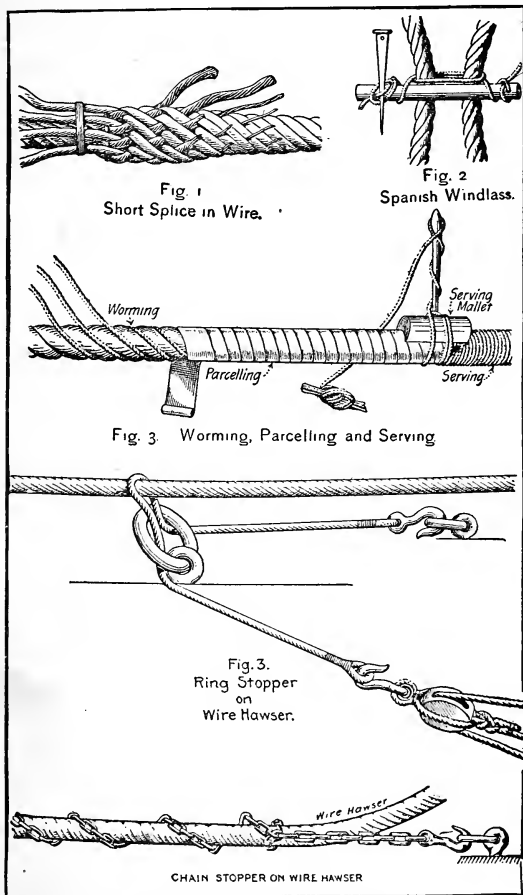
Wire Rope. Plate 3.
