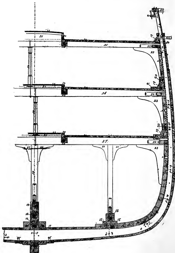
MIDSHIP CROSS SECTION
