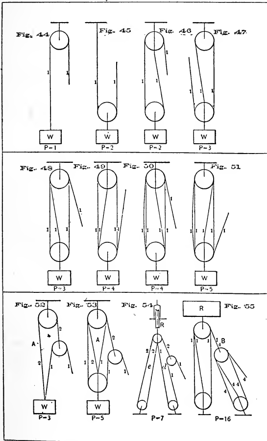
Purchase by Block and Tackle. Plate 1.
