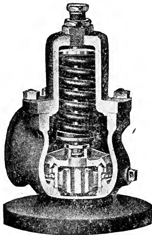
RELIEF VALVE.
