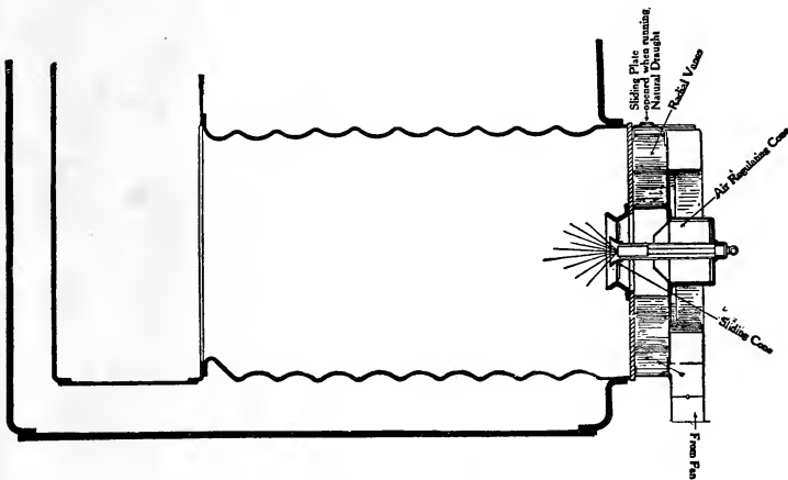
Arrangement of Furnace for Forced Draught.
