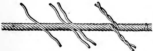
Fig. 4. 2 d Method. Long Splice in Wire.
