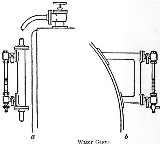
Water Gages
