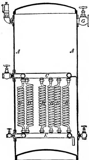
Interior Arrangement of Evaporator, Showing Tube Coils.
