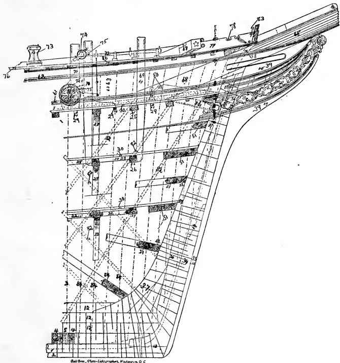
LONGITUDINAL SECTION — BOW
