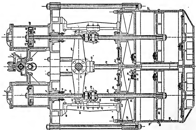
DIAGRAM OF PARTS FOR VERTICAL SINGLE ACTING TWIN BEAM AIR PUMPS
