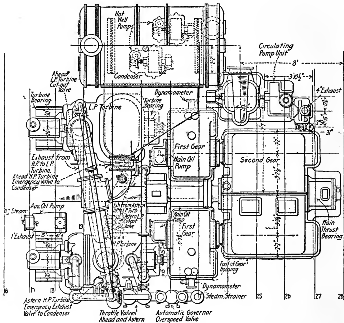
Plan of Engine Room
