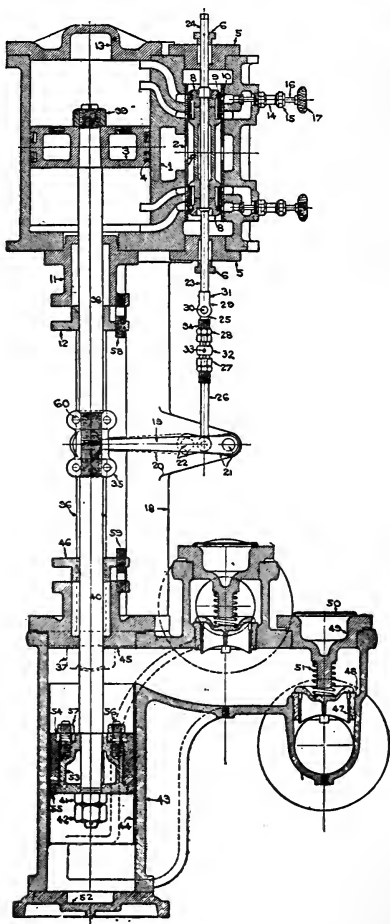
Type of Vertical Duplex Pump Commonly Used.
