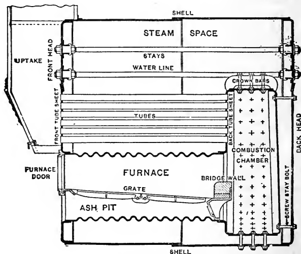
Fig. 9. Scotch Boiler
