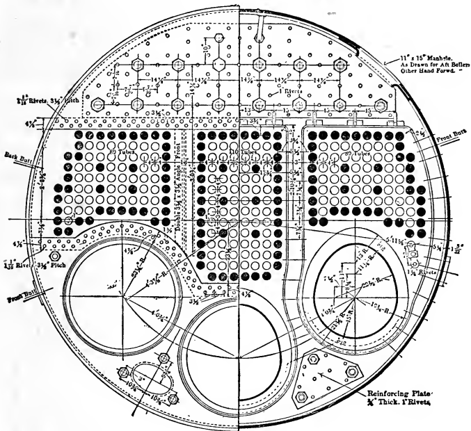
Fig. 10. Scotch Boiler, End View
