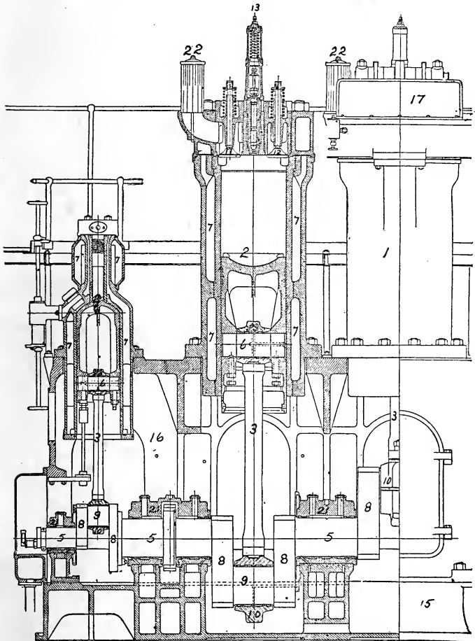
Sectional View, 500 Horse Power Diesel Engine.
