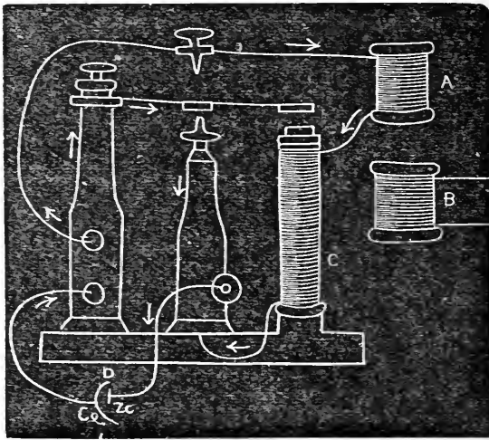
Fig. 30. Diagram of the Course of the Current through the Induction Coil when Helmholtz's Connecting Wire is used.
