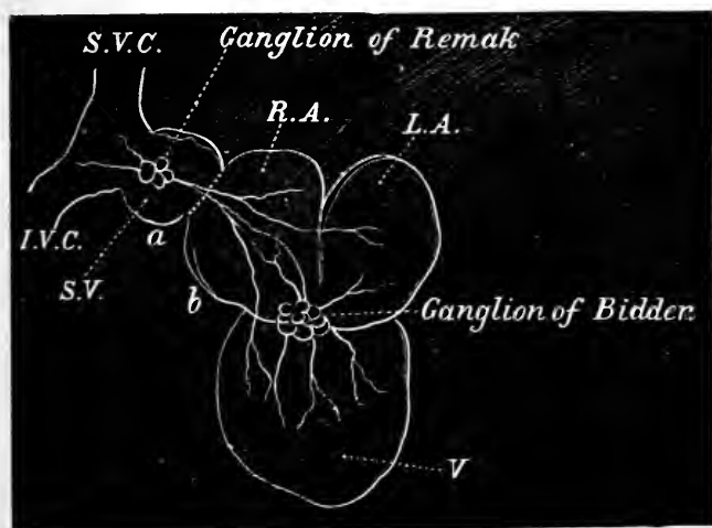
Fig. 37. Ganglia of Frog's Heart. ( After Carpenter's Physiology. )
