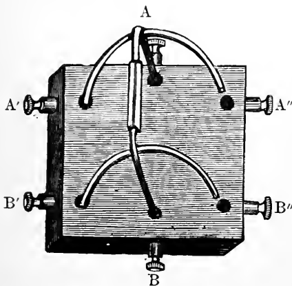
Fig. 34. Reverser. Brass wires (not shown in fig.) connect mercury cups corresponding to A' and B", and A" and B'.
