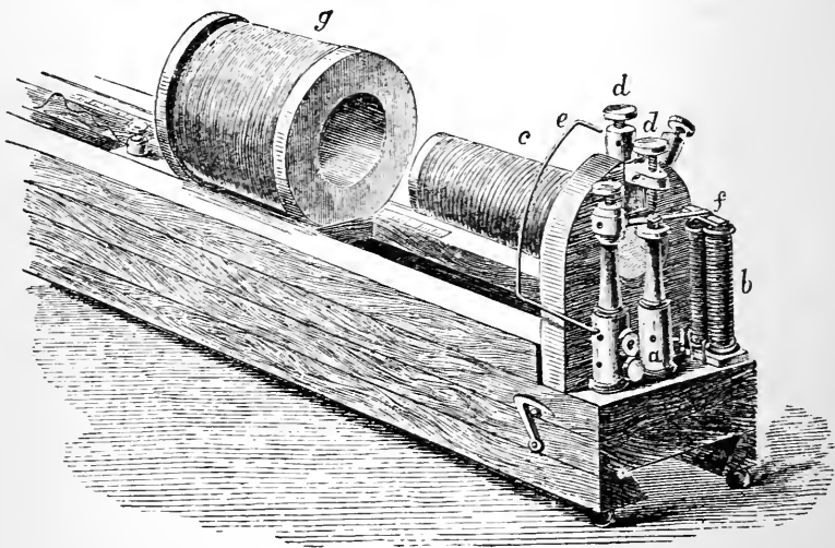
Fig. 29. Du Bois Reymond's Induction Coil.
