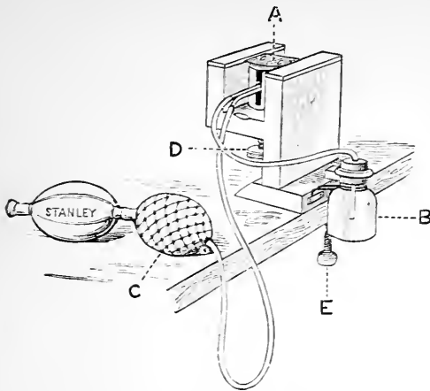
Fig. 14.—Cathcart's Microtome.
