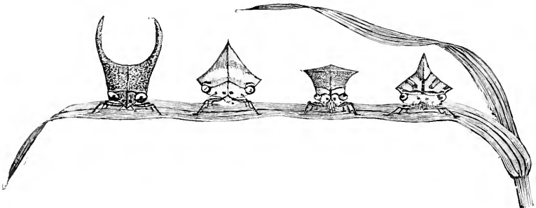
FIG. 190.—Tree-hoppers.
