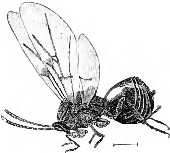
FIG. 745.— Amphibolips spongifica .
