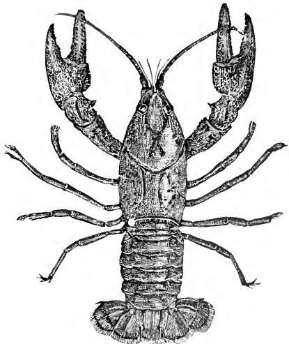
FIG. 3.—A Cray-fish.
