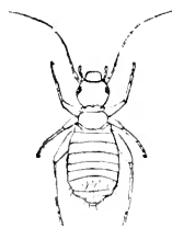
FIG. 108. A Book-lice.
