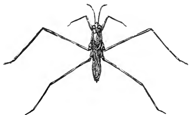
FIG. 157.— Hygrotrechus conformis .
