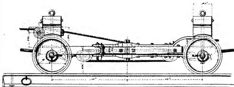
RAILWAY TRUCK.
