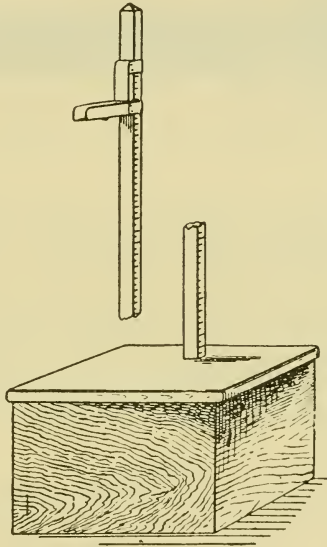
FIG. 4. STADIOMETER, OR HEIGHT STAND.
