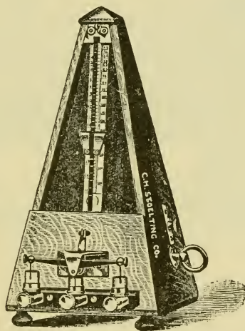
FIG. 21. METRONOME, WITH MERCURY CUPS FOR ELECTRIC CONTACT.
