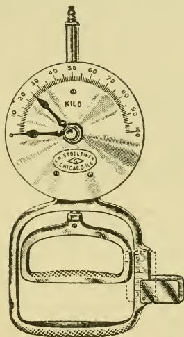
FIG. 14. DYNAMOMETER AND DYNAMOGRAPH, AFTER SMEDLEY, IMPROVED.
