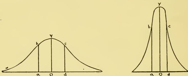
FIG. 3. TYPICAL CURVES OF NORMAL DISTRIBUTION.
