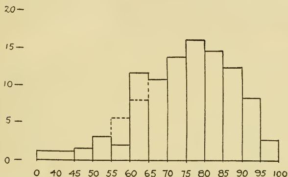
FIG. 2. DISTRIBUTION OF THE MARKS OF 20,348 CORNELL UNIVERSITY STUDENTS. FROM I. E. FINKELSTEIN. The Marking System in Theory and Practice .
