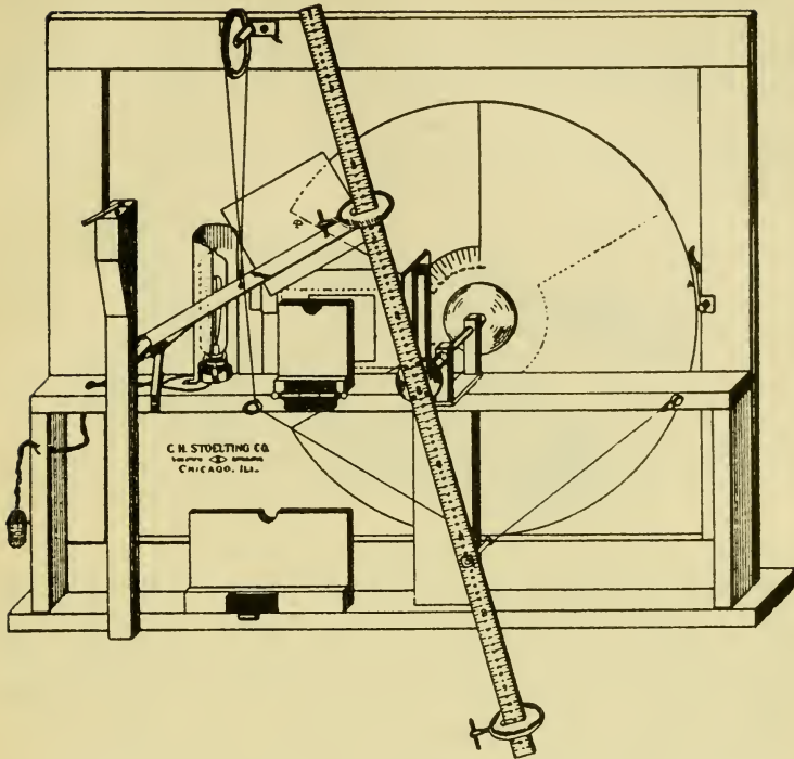
FIG. 57. DISC TACHISTOSCOPE.
