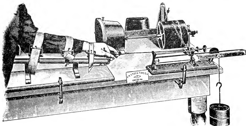
FIG. 25. MOZZO ERGOGRAPH, MODIFIED BY LOMBARD.
