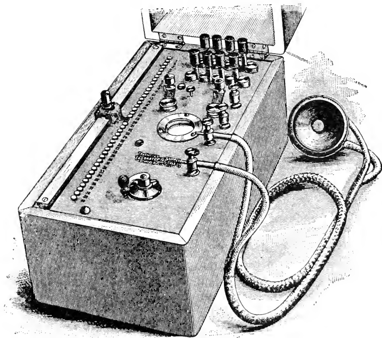
FIG. 50. SEASHORE'S AUDIOMETER.
