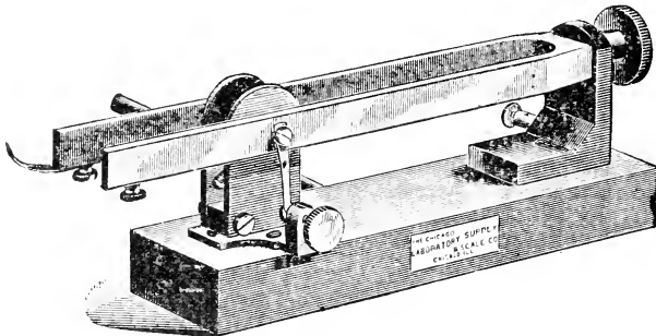
FIG. 58. FIFTY-VIBRATIONS DEBY-CONTACT FORK.
