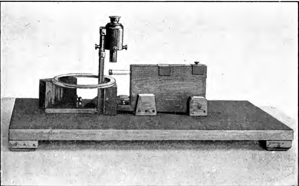
APPARATUS FOR DETERMINING THE MAGNETIC INFLUENCE OF METAL, ADJUSTING DEPARTMENT.
