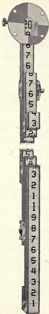
FIG. 63. No. 501-B SELF-READING ROD, THREE PLY
