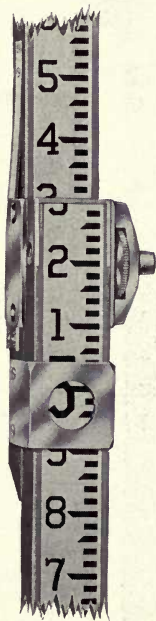
FIG. 75. VIEW OF CLAMP OF PLAIN TWO PLY LEVELING RODS
