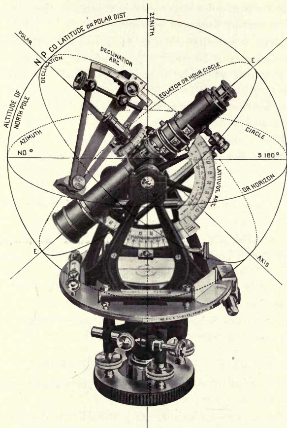
FIG. 36 NO. 30-A PRECISE TRANSIT WITH BURT SOLAR ATTACHMENT ILLUSTRATION ALSO SHOWS BEAMAN STADIA ARC
