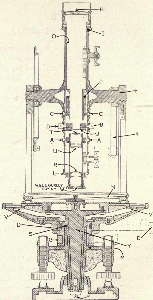
FIG. 1 CROSS SECTION OF TRANSIT
