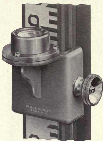
FIG. 91. No. 548 ROD LEVEL
