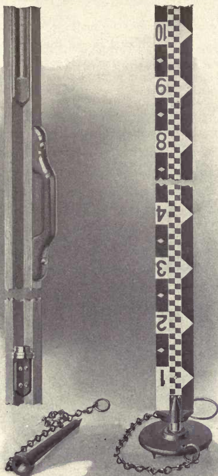
FIG. 82. GURLEY PRECISE LEVELING ROD No. 550-R
