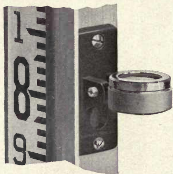
FIG. 89. No. 546 ROD LEVEL
