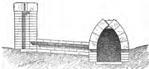
Fig. 41.—Vaulted drain at Khorsabad (after Place).
