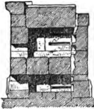
Fig. 199.—The Burj el-Bezzäk. Section (after Renan).
