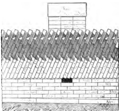
Fig. 42.—Vaulted drain at Khorsabad. Slope of the bricks (after Place).
