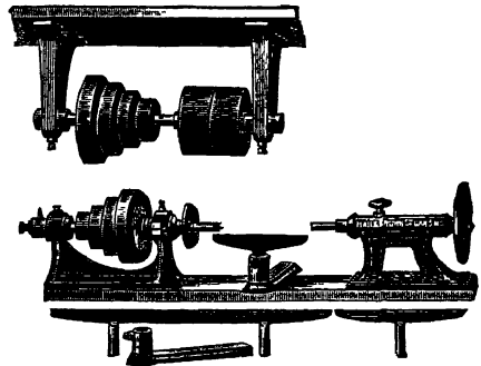
FIG. 36. SPEED-LATHE.
