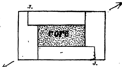
FIG. 122. HORIZONTAL SECTION OF BOX AND CORE.
