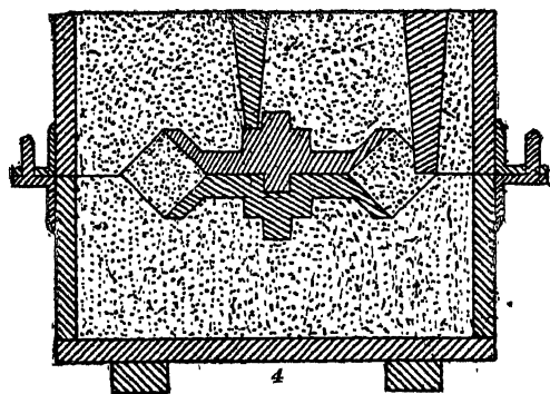
FIG. 117. SECTION OF FLASK, PATTERN, ETC.
