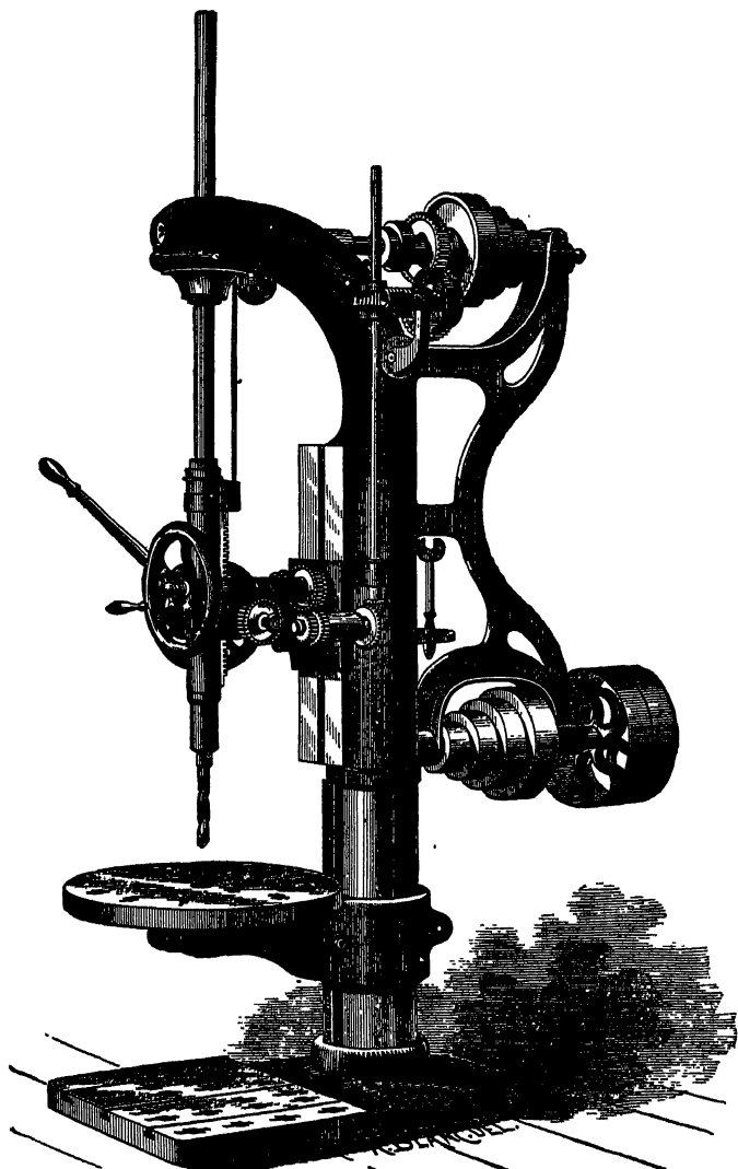
FIG. 125. "GOOSE-NECK DRILL," PUTNAM MACHINE COMPANY, FITCHBURG, MASS.
