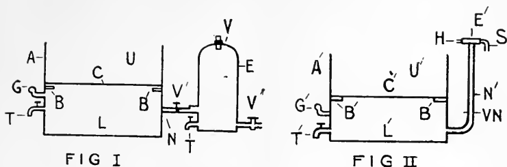
FIGS. 1 and 2.—A and A', \frac{1}{4} in. iron. B and B', Flanges to support C and C'. C and C', \frac{1}{4} in. perforated iron plates. T and T', Taps to run off the filtrate. V V' V'', \frac{1}{2} in. valves. G and G', Vacuum gauges. L, Condensation chamber, \frac{1}{4} in. iron cylinder with steam inlet through V, outlet through B', and connected with A by means of iron pipe N, which can be opened or closed by valve V'. L', a steam ejector connected with boiler by pipe S, and the air by outlet H, and with A by the tube N'.
