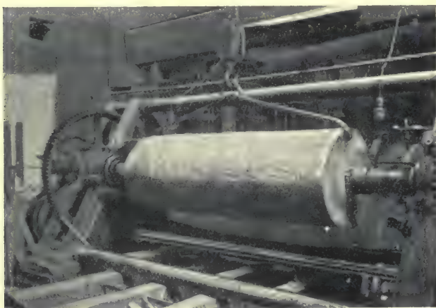
FIG. 1.—CENTRING OF LOG IN ROTARY CUTTER.
