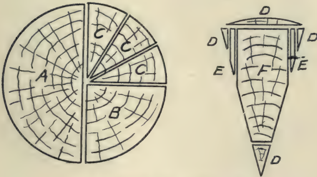
FIG. 5.—METHOD OF CUTTING LOGS.
