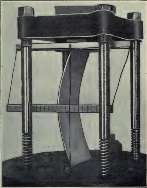
FIG. 11.—A PLYWOOD COLUMN READY FOR TEST.
