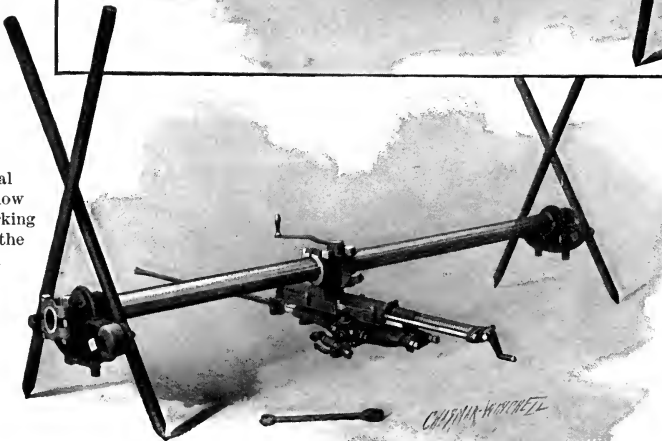
THE SULLIVAN QUARRY BAR, SHOWING ADJUSTABILITY.
