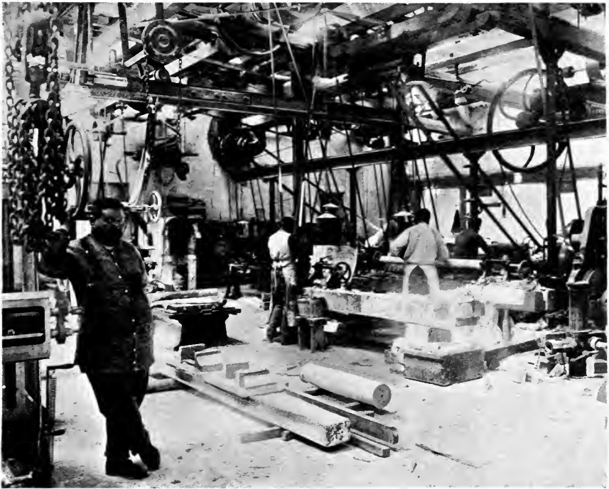
INTERIOR OF MACHINE SHOP, LA BUSSIÈRE, BELGIUM.
