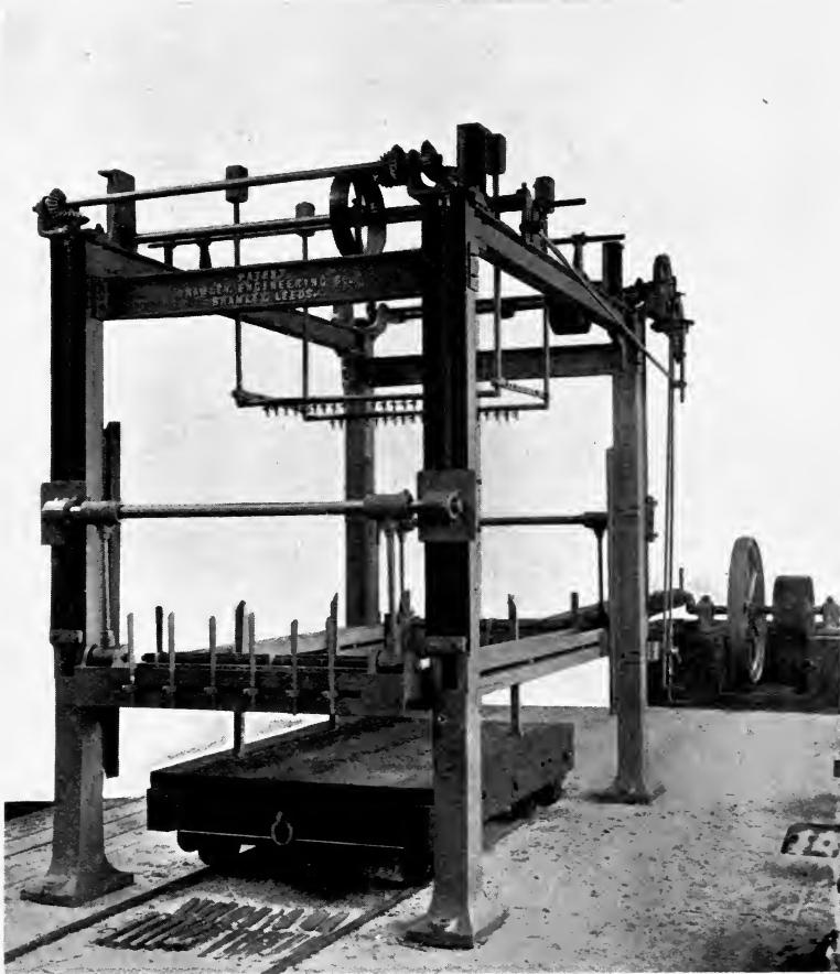
A WELL-KNOWN TYPE OF FRAME SAW.
