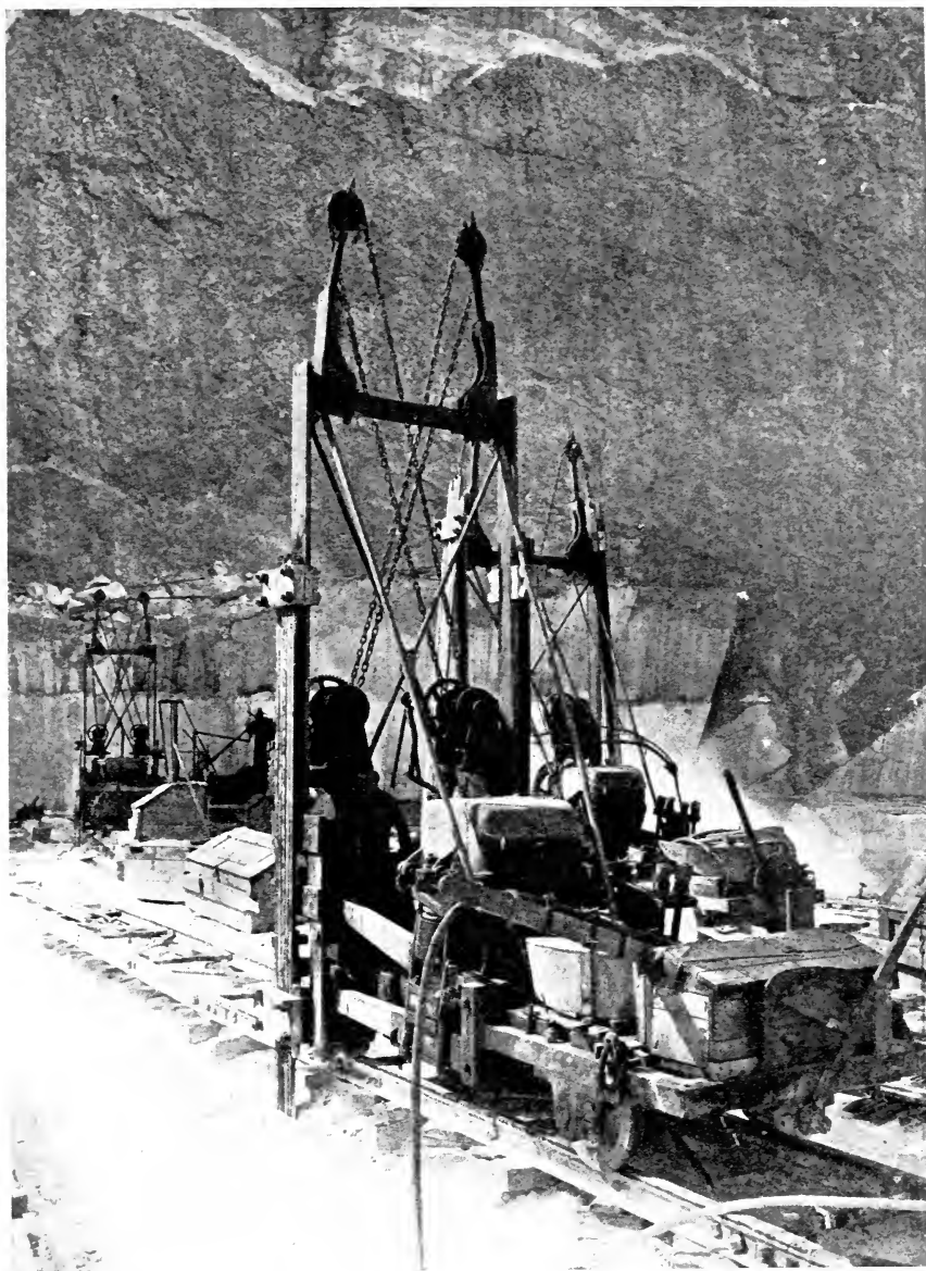
THE WARDWELL CHANNER OPERATING BY ELECTRICITY AT PROCTOR, VERMONT, U.S.A.
