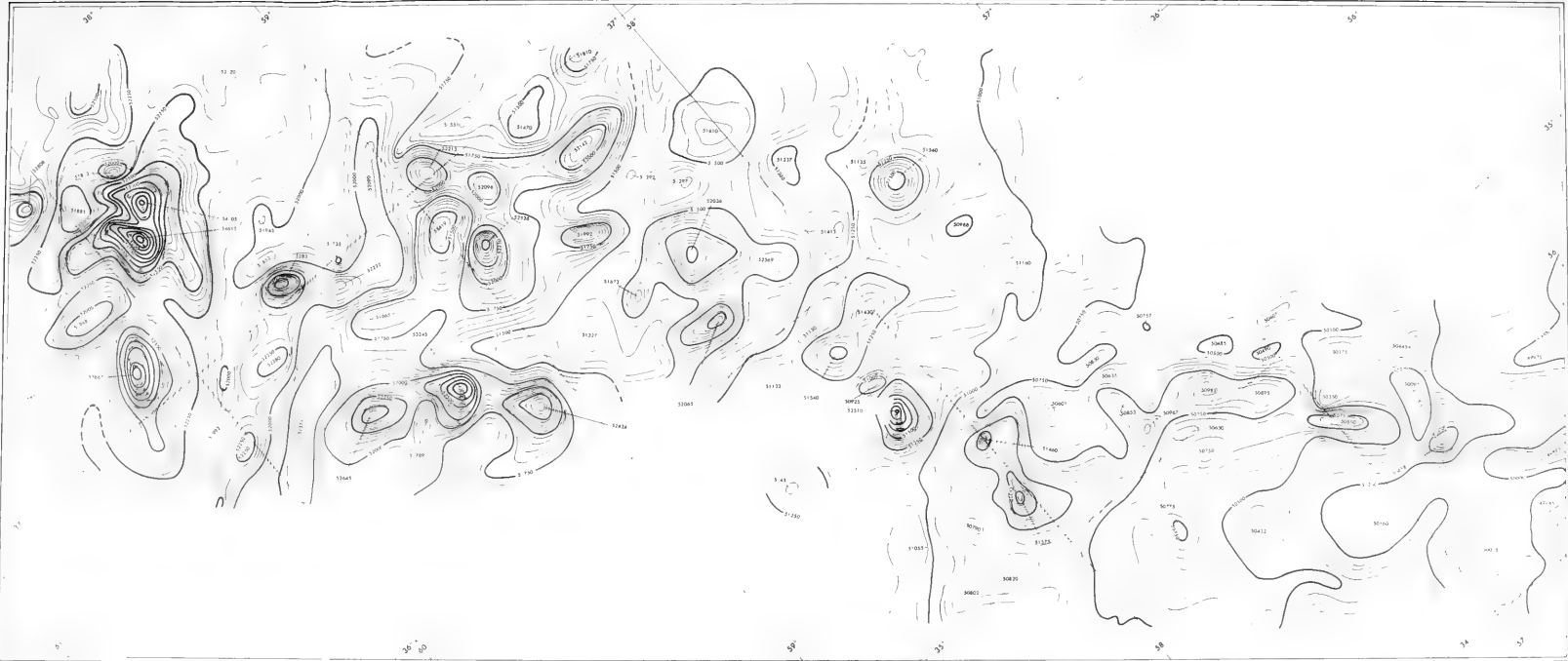
FIGURE 4.—TOTAL MAGNETIC INTENSITY CONTOUR CHART NEW ENGLAND SEAMOUNT CHAIN AREA C CONTOUR INTERVAL 90 GAMMAS
