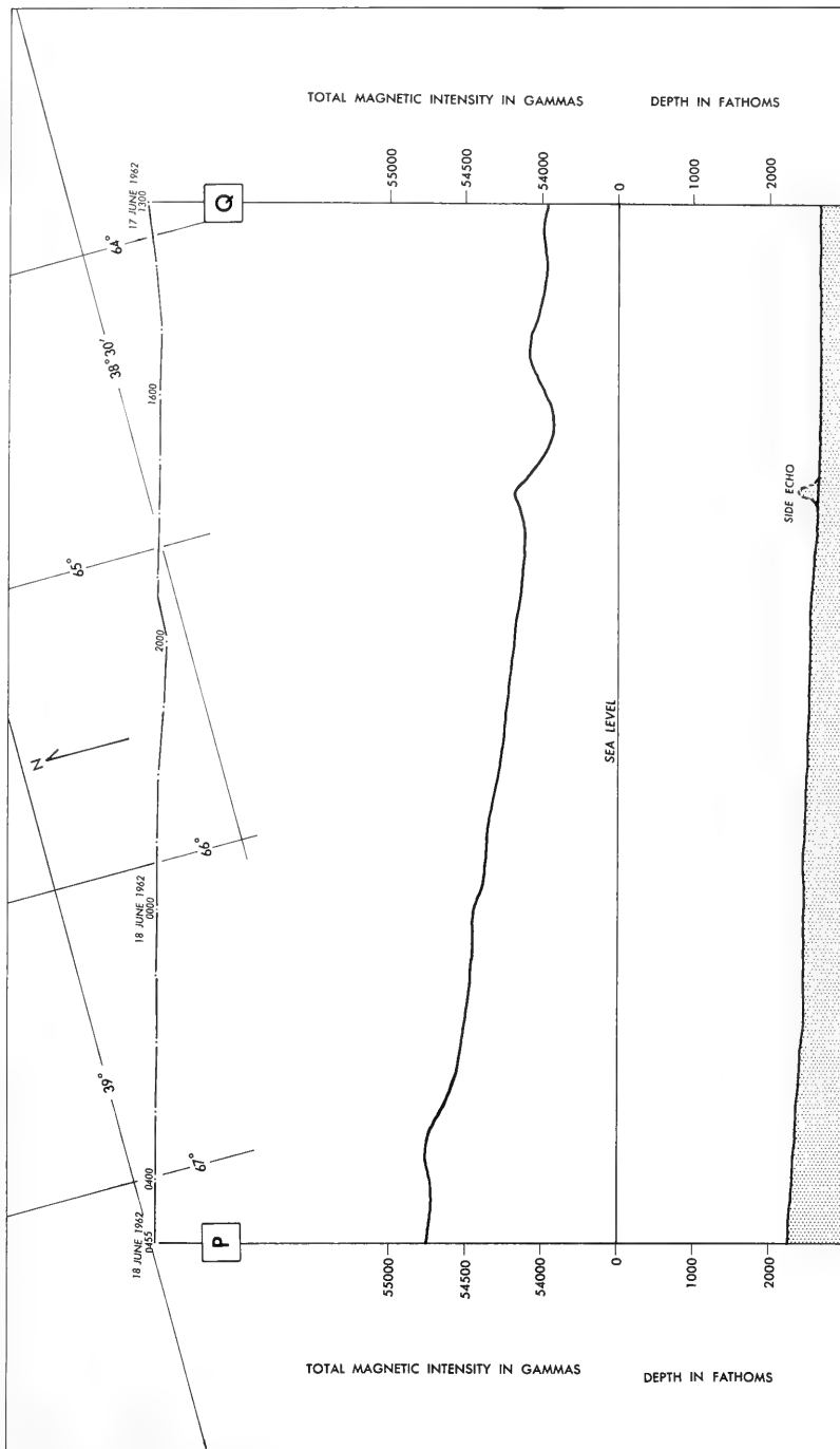
FIGURE 18.—MAGNETIC AND BATHYMETRIC PROFILES P-Q
