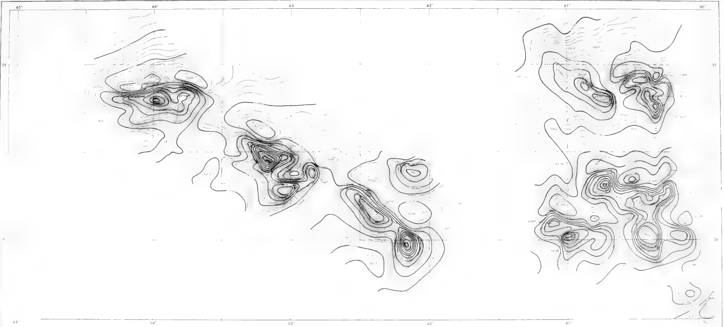
FIGURE 2.—TOTAL MAGNETIC INTENSITY CONTOUR CHART NEW ENGLAND SEAMOUNT CHAIN AREAS A AND B
