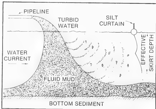
Figure 6-6.—Silt Curtain
