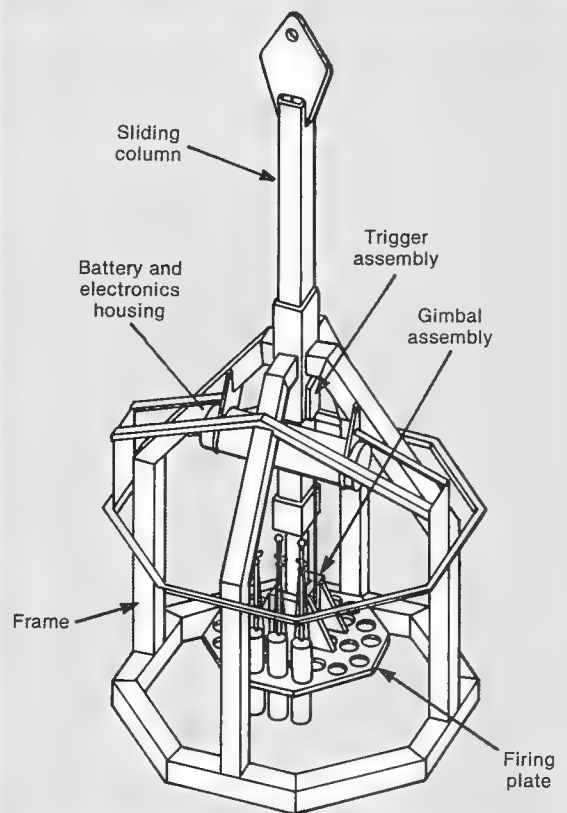
Figure 4-14.—Prototype Crust Sampler
