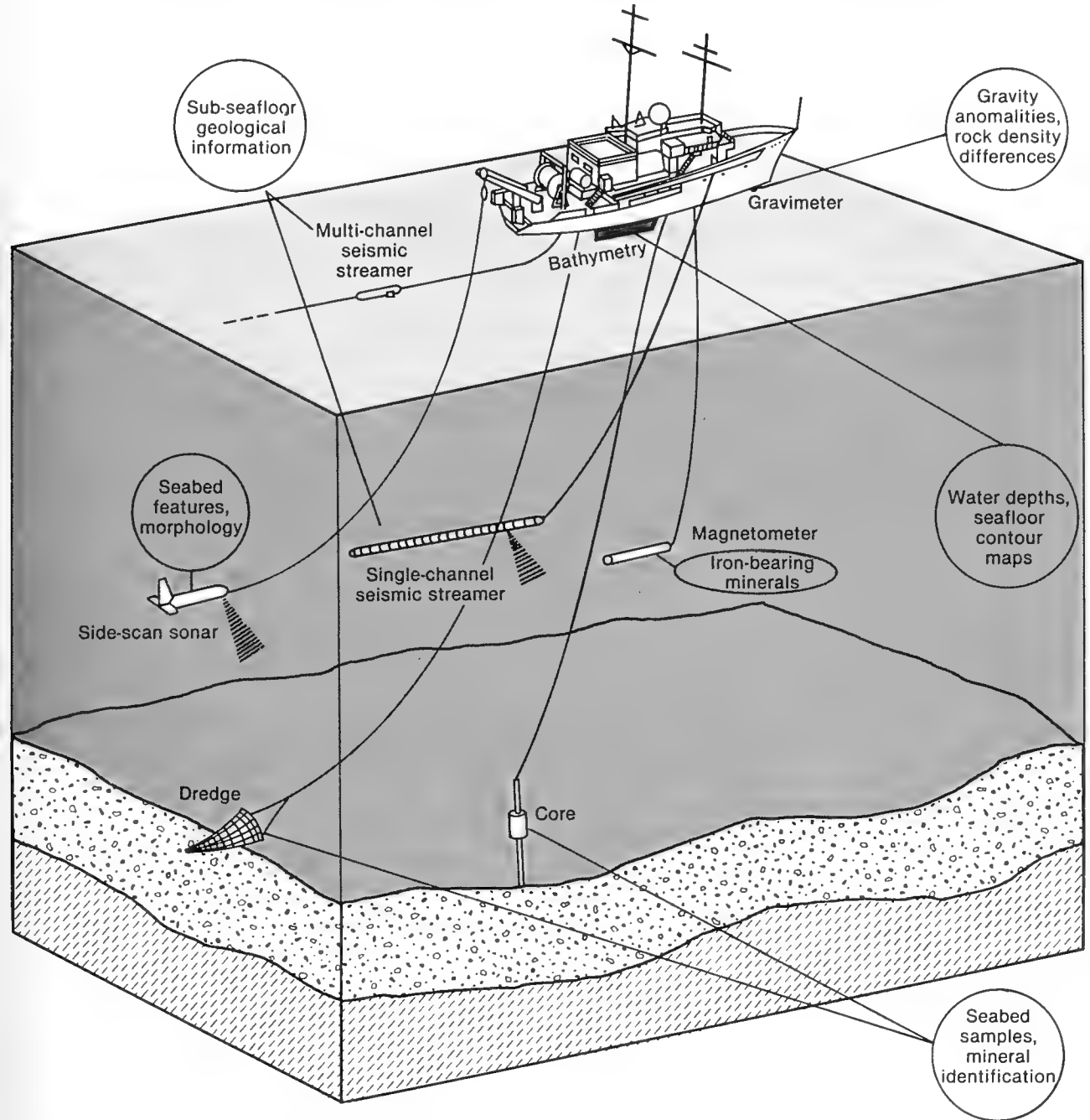
Figure 4-1.—USGS Research Vessel S.P. Lee and EEZ Exploration Technologies
