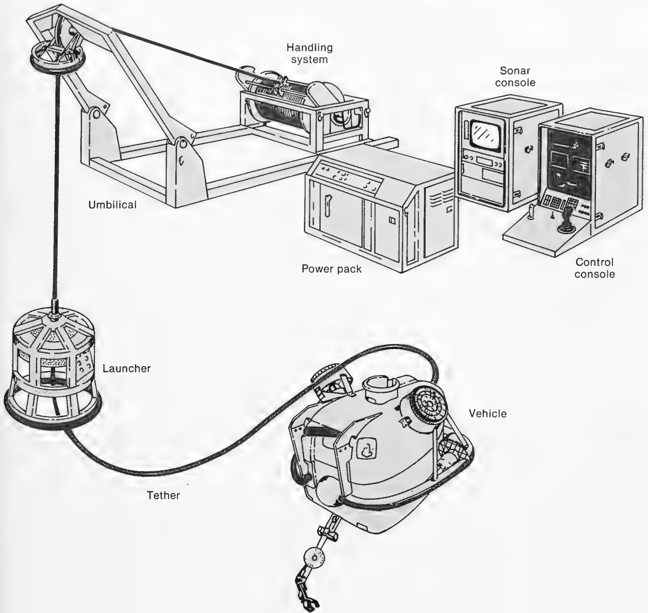
Figure 4-12.—A Tethered, Free-Swimming Remotely Operated Vehicle System
