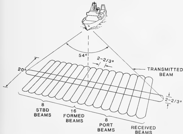
Figure 4-5.—Sea Beam Beam Patterns
