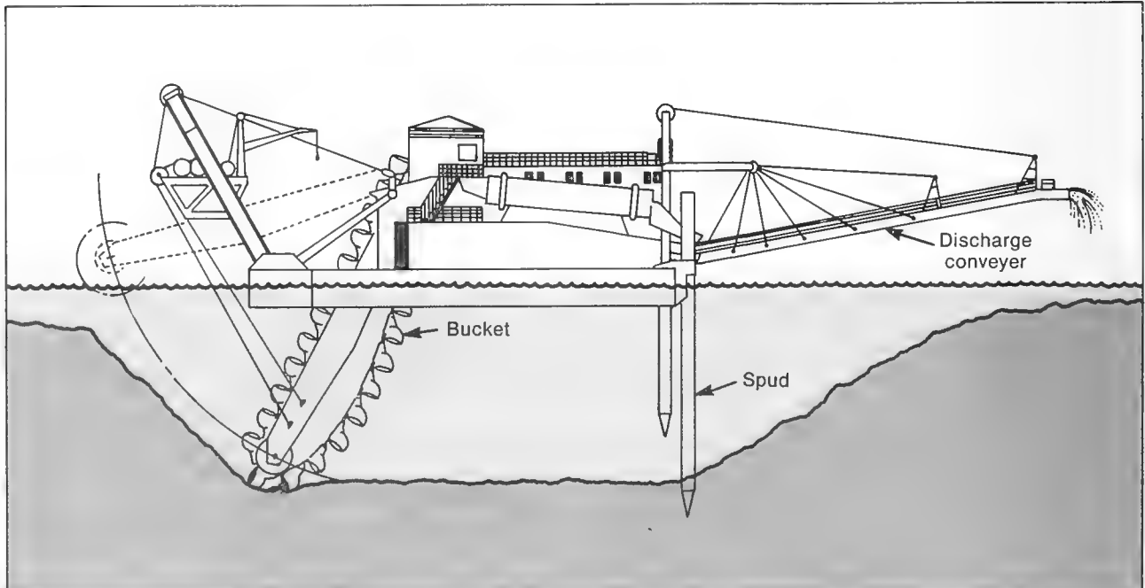
Figure 5-1.—Bucket Ladder Mining Dredge
