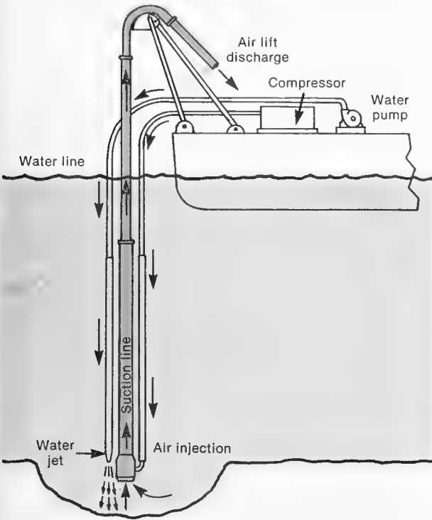
Figure 5-8.—Airlift Suction Dredge Configuration
