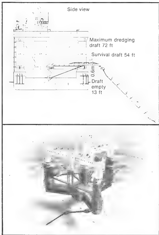
Figure 5-11.—Conceptual Design for Suction Dredge Mounted on Semi-Submersible Platform
