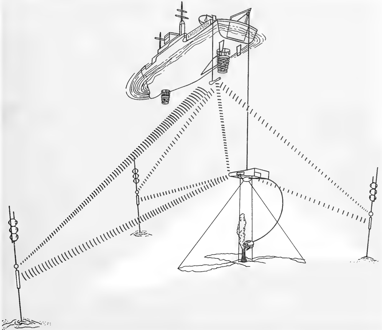
Figure 4-13.—Schematic of the Argo-Jason Deep-Sea Photographic System
