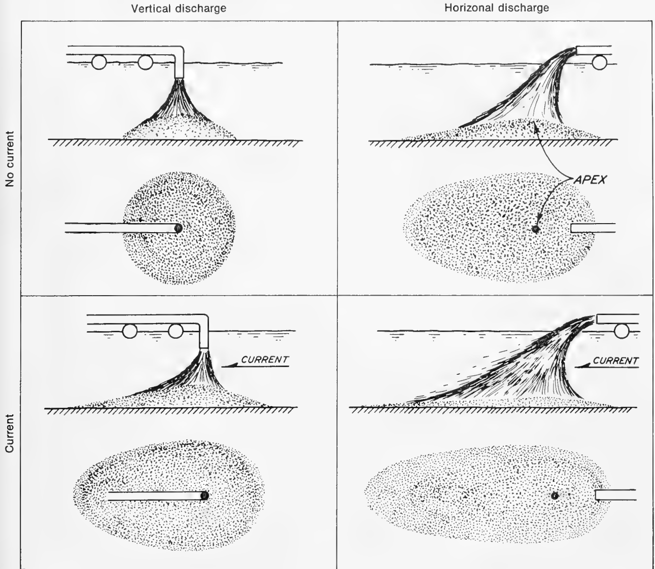
Figure 6-5.—The Effect of Discharge Angle and Water Current on the Shape and Depth of Redeepened Sediments
