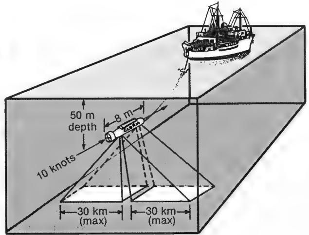
b) Schematic of GLORIA system
