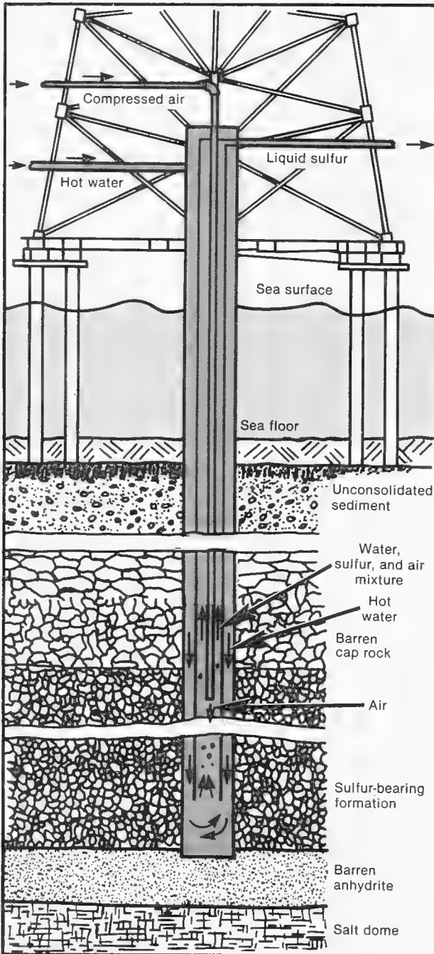
Figure 5-13.—Schematic of Solution Mining Technology (Frasch Process)
