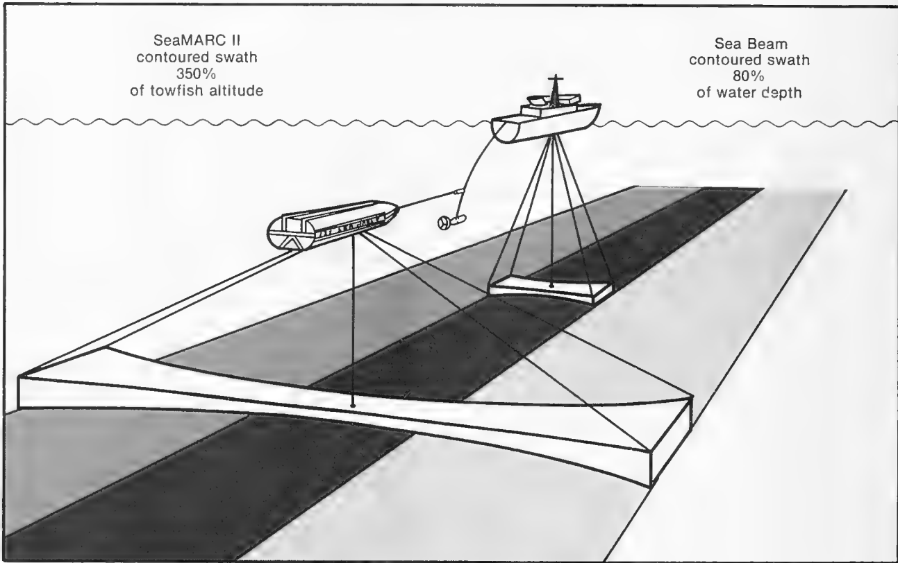
Figure 4-7.—Comparing SeaMARC and Sea Beam Swath Widths
