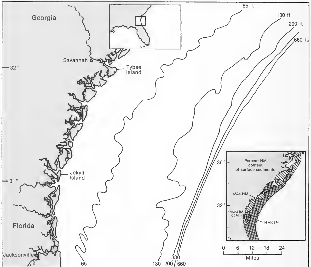
Figure 5-17.—Offshore Titaniferous Mineral Province, Southeast United States
