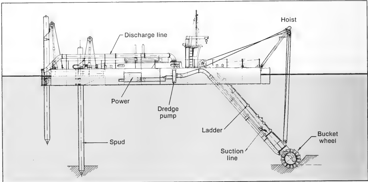
Figure 5-7.—Bucket Wheel Suction Dredge
