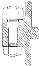
ENLARGED VIEW OF TUBE PLATE JOINT
