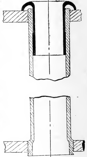
Fig. 35.—Stay Tube.
