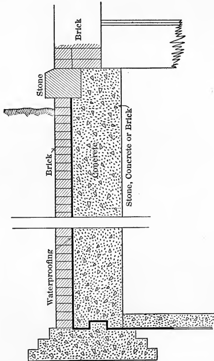
FIG. 78.—Sketch Showing Method of Waterproofing a Basement Wall.
