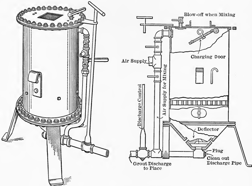
FIG. 104.—Ransome-Cannif Grout Mixer. (Ransome Concrete Machinery Co.)
