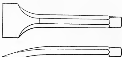
FIG. 23.—Pitching Chisel.
