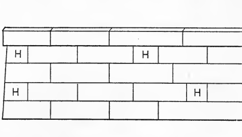
FIG. 65.—Ashlar Masonry with Few Headers.
