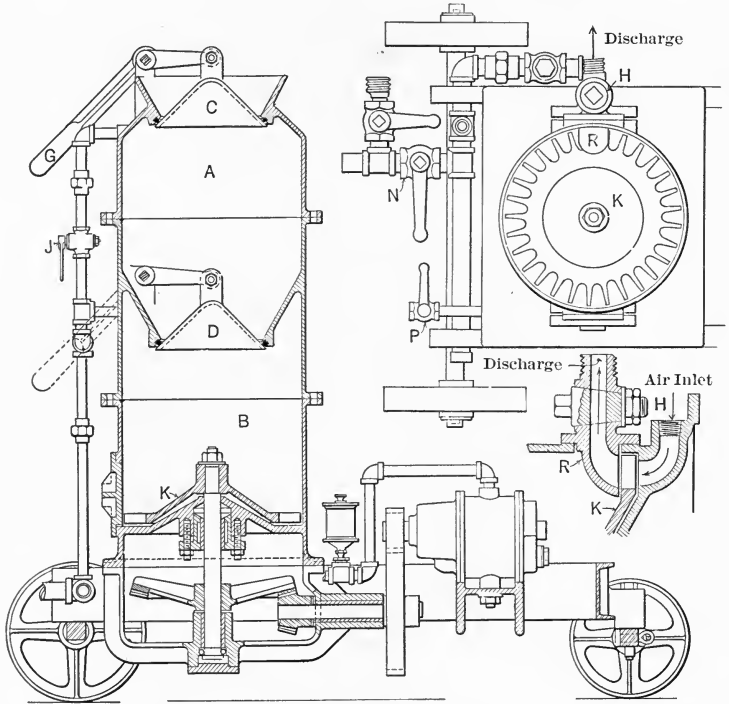
FIG. 110.—Sectional Views of Type G. L. Cement-Gun. Air Pressure, 100 Pounds. (Cement-Gun Company, Inc.)
