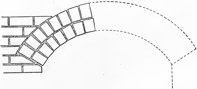
FIG. 89.—Sketch Showing Method of Arranging Common Brick in an Arch. "Row-Lock" Arch.
