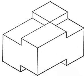
FIG. 70.—Sketch Showing Construction When Structure Is Subjected to Strong Wave Action.
