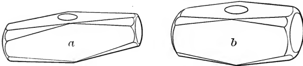
FIG. 6. Drilling or Striking Hammers. ( a ) Nevada Pattern. ( b ) Oregon Pattern.
