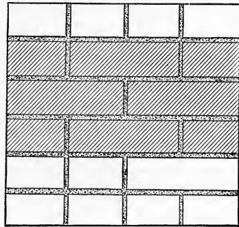
FIG. 81.—Sketch Showing Bonding of Facing and Backing Through the Filling in Brick Masonry.
