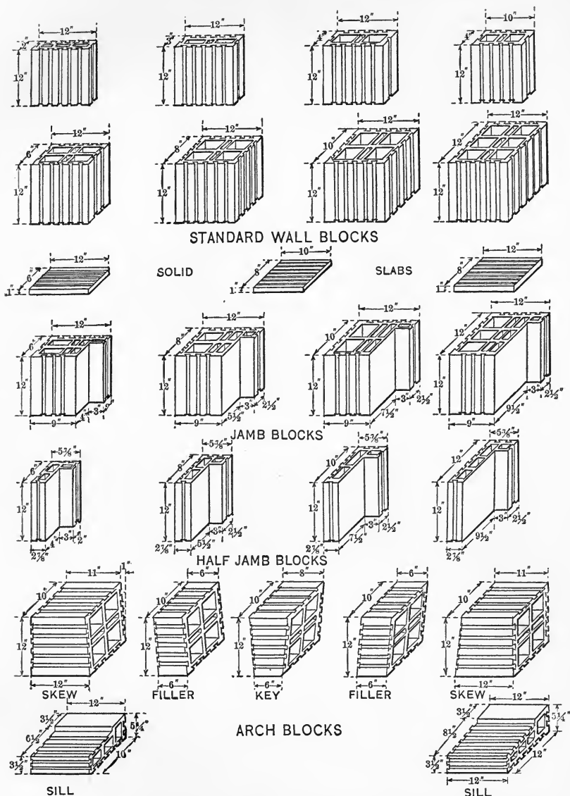
FIG. 51.—A Few Shapes and Sizes of Hollow-Tile Blocks. (National Fire-proofing Co.)
