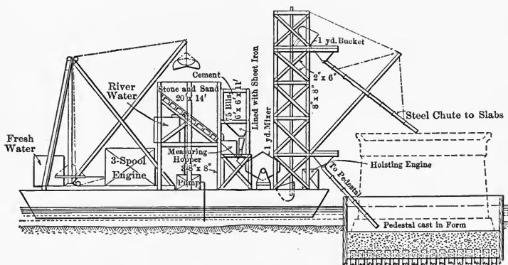
FIG. 102.—Floating Mixer Plant Delivering Concrete Through Chutes. Gunpowder River Bridge. ( Engineering Record , May 2, 1914.)
