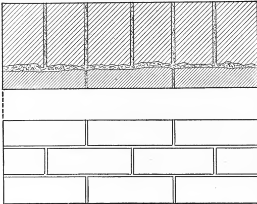
FIG. 83.—Another Type of Secret Bond in Brick Masonry.
