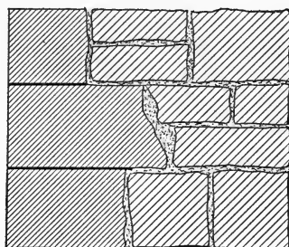
FIG. 62.—Ashlar Masonry with Rubble Backing and Filling.
