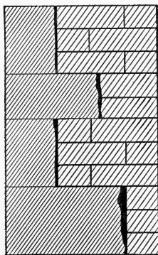
FIG. 61.—Ashlar Masonry with Brick Backing and Filling.
