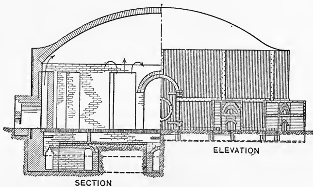
FIG. 45.—Down-Draft Kiln, Circular in Plan, Built of Brick in a Steel Shell.
