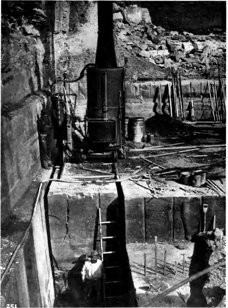
FIG. 10.—Channeling a 9-foot Key Block. Ingersoll-Sergeant Track Channeler. (Ingersoll-Rand Co.)
