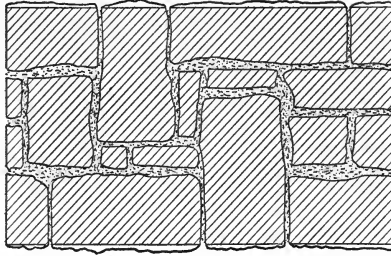
FIG. 68.—Sketch Showing Proper Arrangement of Headers.
