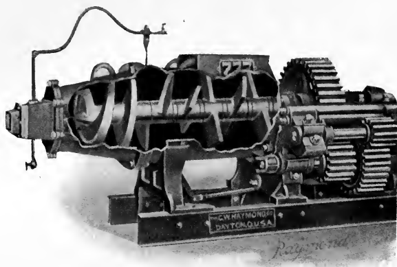
FIG. 41.—Interior of Brick Machine. (The C. W. Raymond Co.)
