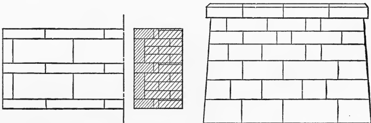
FIG. 59.—Coursed Ashlar, Using Two Sizes of Stone.
