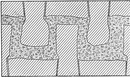
FIG. 69.—Sketch Showing Stretchers and Headers Dovetailed.
