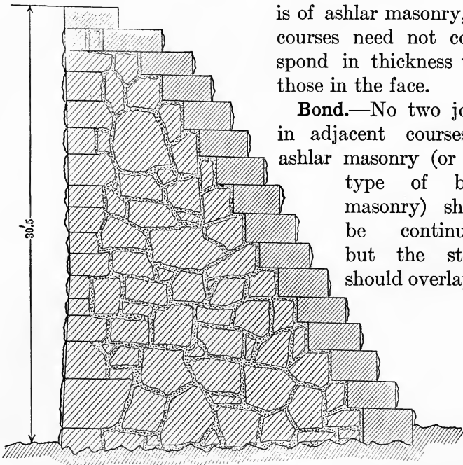
FIG. 64.—Ashlar Face Masonry and Rubble Filling without Horizontal or Vertical Joints. (Muscoot Dam. Reports on the New Croton Aqueduct, etc., 1895-1907.)
