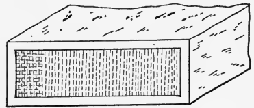
FIG. 36.—Crandalled Face Finish. Cross-Crandalled at Left End.
