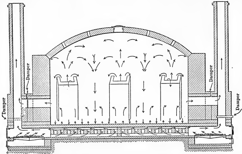
FIG. 46.—Section of a Circular Up-and-Down Draft Kiln. (Ohio Kiln Co.)
