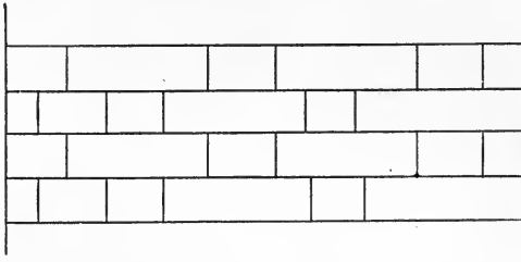
FIG. 66.—Ashlar Masonry with an Equal Number of Headers and Stretchers.
