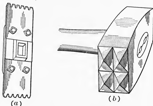
FIG. 107.—Tools for Finishing Concrete Surfaces. (a) Ransome Concrete Axe. (b) Bush Hammer with Four Points.
