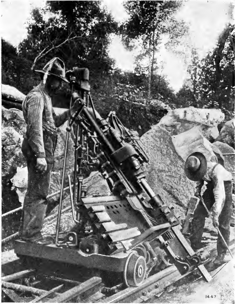
FIG. 11.—Swing Back Type of Ingersoll-Sergeant Track Channeler as Illustrated in a 5-inch "Marble" Channeler. (Ingersoll-Rand Co.)
