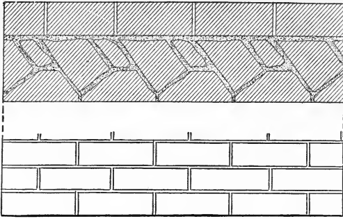
FIG. 82.—Diagonal Secret Bond in Brick Masonry.
