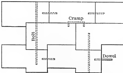
FIG. 70.—Sketch Showing Construction When Structure Is Subjected to Strong Wave Action.
