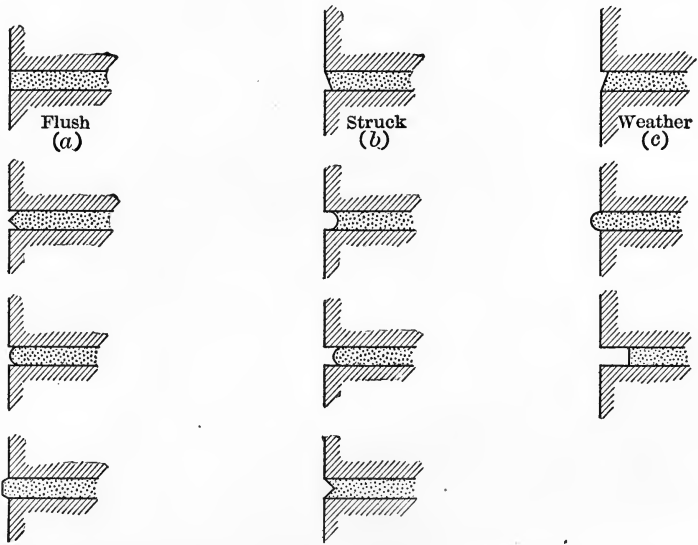
FIG. 79.—Finish of Joints in Brick Masonry. (a) Flush Joint. (b) Struck Joint. (c) Weather Joint.
