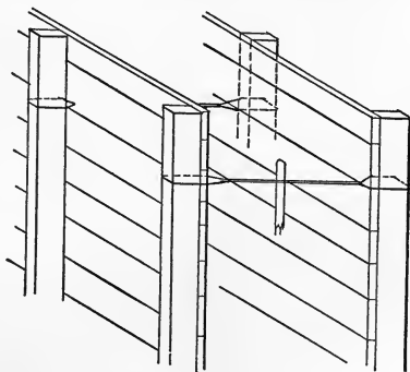
FIG. 112.—Sketch Showing Wire Ties in Concrete Forms.
