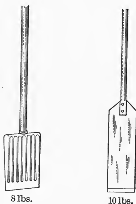
FIG. 108.—Ransome Tamper.
