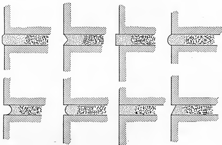
FIG. 75.—Joint Facings for Stone Masonry.
