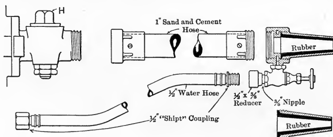
FIG. 111.—Details of Hose Connections and Nozzles Used with the Cement-Gun. (Cement-Gun Company, Inc.)
