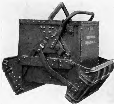
FIG. 105.—Bottom Dump Bucket. Capacity, in Cubic Feet, 15 to 75. (Insley Manufacturing Co.)
