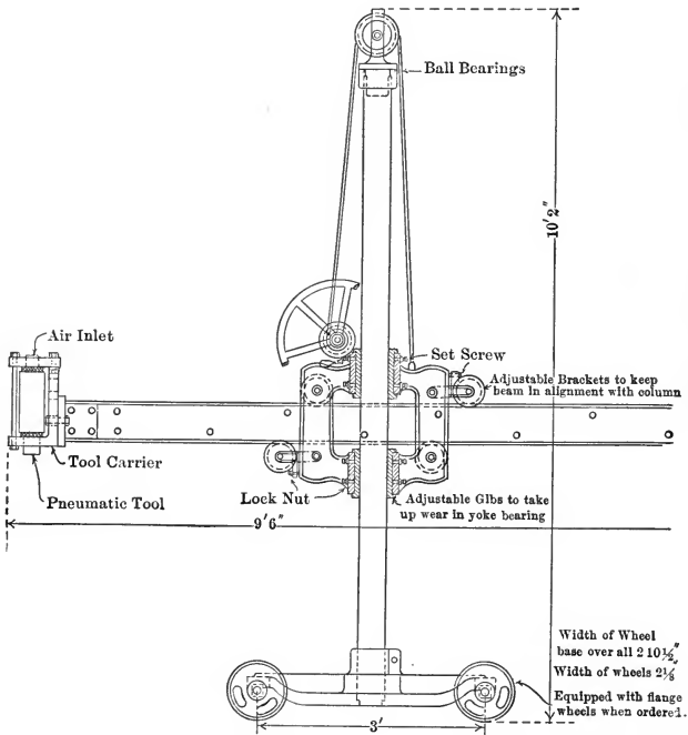
FIG. 29.—Portable Surfacing Machine Using Pneumatic Tools. (George Oldham & Son Co.)
