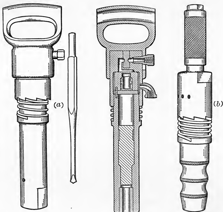
FIG. 26.—Pneumatic Hammers. (a) "Barre" Pneumatic Plug Drill. (b) "Barre" Pneumatic Bushing Tool. (Trow and Holden.)
