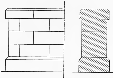
FIG. 58.—Regular Coursed Ashlar. All Stones of the Same Height.
