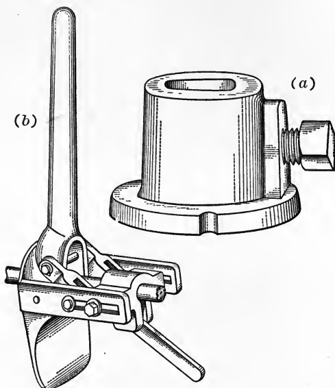
FIG. 114.—Universal Form Clamp Used with Round Rods with Nut on One End. (a) Clamp on Free End of Rod. (b) Device for Pulling Rod when Forms are Removed. (Universal Form Clamp Co.)
