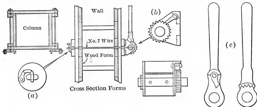
FIG. 113.—Ratchet Form Clamp. (a) Anchor for One End of Wire. (b) Ratchet Tightener at Other End of Wire. (c) Lever for Operating Ratchet. (Peerless Form Clamp Co.).
