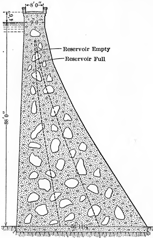
FIG. 115.—Cross-Section of Shirawata Dam, Showing Large Stones Embedded in Concrete. (For Description see Engineering Record , November 8, 1913.)
