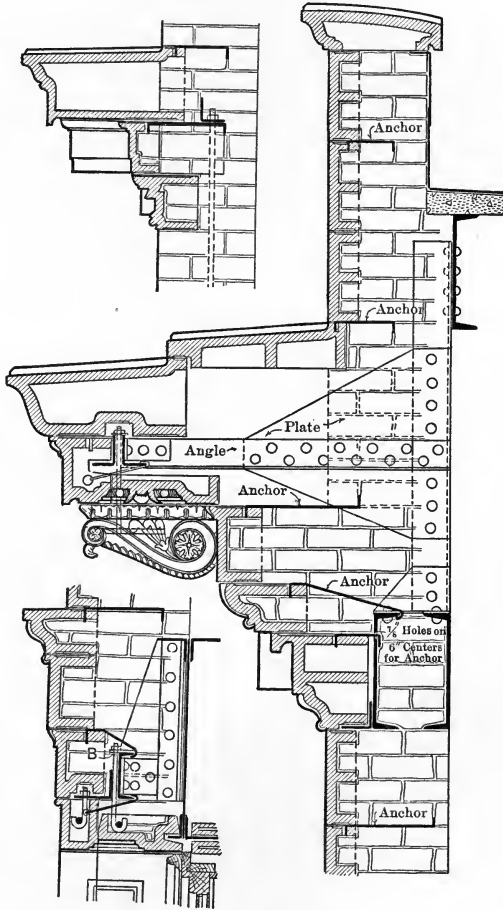
FIG. 93.—Details of Terra-Cotta Construction as Used in Steel Skeleton Buildings.
