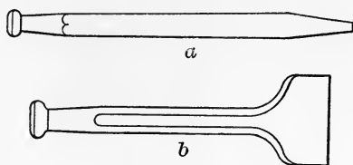
FIG. 25.—Stonecutters' Chisels. (a) Splitter. (b) Drove.
