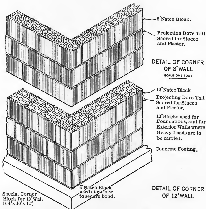
FIG. 91.—Detail of Foundation and Exterior Wall Construction. Exterior to be Finished with Stucco and Interior Plastered. (National Fire-proofing Co.)
