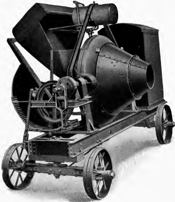
FIG. 95.—No. 104 Smith "Mascot" Mixer on Truck with Gasoline Engine, Power Charger, and Water-Tank. Skip in Discharging Position. (The T. L. Smith Co.)
