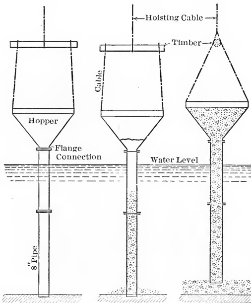
FIG. 106.—Tremie Empty, Sealed, and Ready to be Raised. ( Engineering Record , August 15, 1914.)
