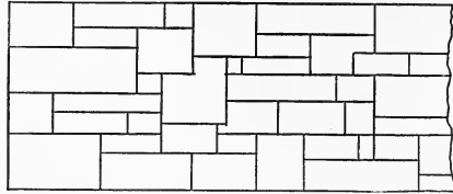
FIG. 56.—Sketch Showing Arrangement of Stone in Broken Range Masonry.
