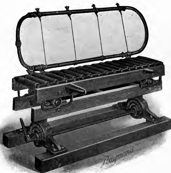
FIG. 42.—The Raymond Combination Cutting Table. "The Simplest Form of Cutter Made." (The C. W. Raymond Co.)
