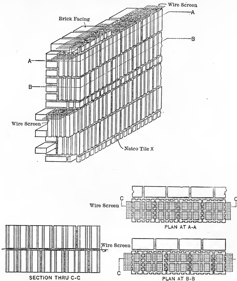
FIG. 92.—Section of Exterior Wall with Brick Facing and Hollow-Tile Backing. Showing Method of Bonding and Sealing Vertical Holes. (National Fireproofing Co.)
