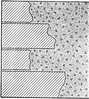
FIG. 63.—Ashlar Masonry with Concrete Backing and Filling.
