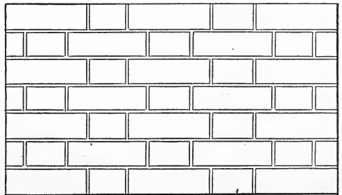
FIG. 87.—Sketch Showing Brick Wall with an Equal Number of Headers and Stretchers. Flemish Bond.
