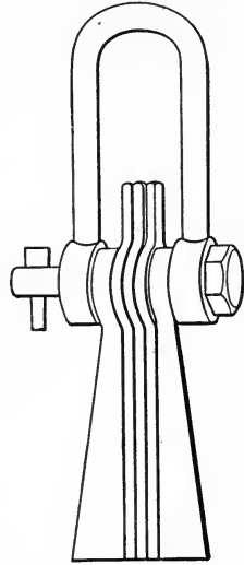
FIG. 73.—Lewis for Lifting Cut Stone.
