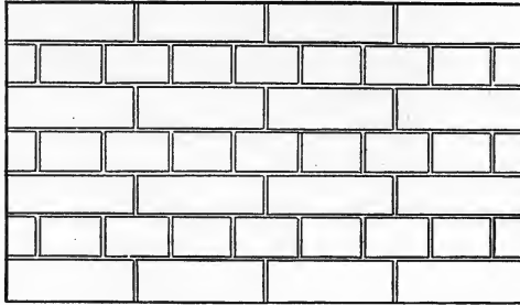
FIG. 88.—Sketch Showing Arrangement of Headers and Stretchers in a Brick Wall. English Bond.
