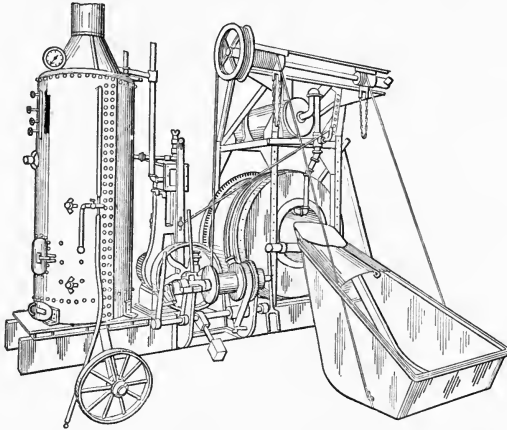
FIG. 94.—Ransome Concrete Mixer. (Ransome Concrete Machinery Co.)
