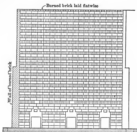
FIG. 43.—Cross-Section of Three "Arches" of a Clamp Kiln.
