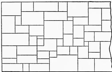
FIG. 57.—Sketch Showing Arrangement of Stone in Random Masonry.
