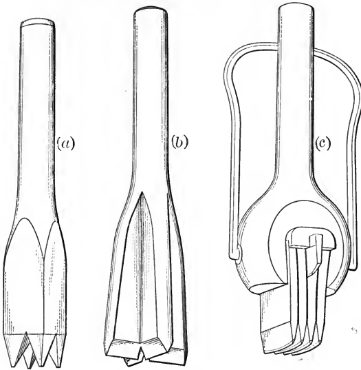
FIG. 28.—Pneumatic Surfacer Tools. (a) Tooth Chisel. (b) Cross Chisel. (c) Boltless Bush Chisel. (Trow and Holden.)
