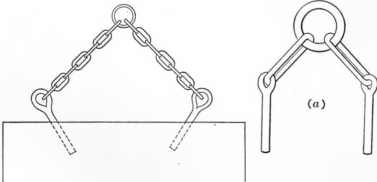
FIG. 74.—Dowels for Lifting Cut Stone. (a) Pin Lewis; Capacity, 1,000 to 6,000 Pounds.
