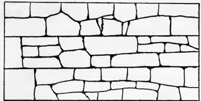
FIG. 77.—Sketch Showing Arrangement of Stones in Coursed Rubble.
