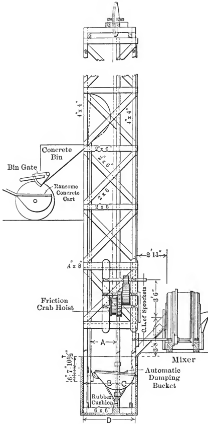
FIG. 101.—“Ransome” Plant for Mixing and Hoisting Concrete.
