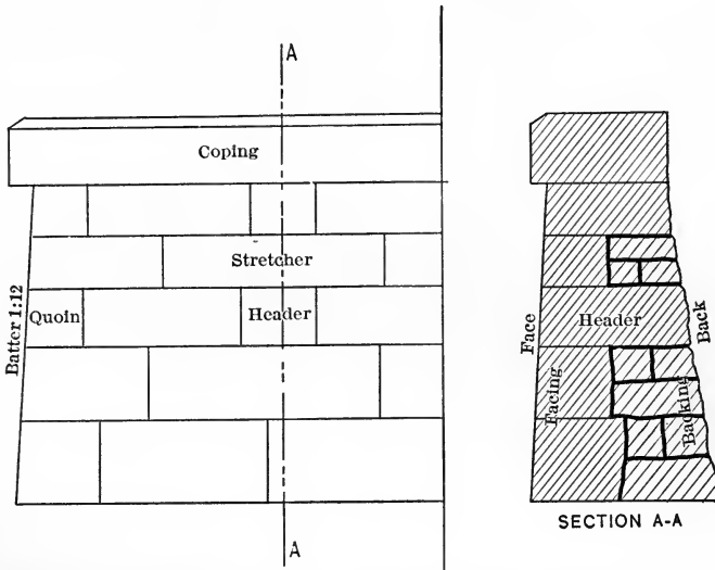
FIG. 55.—Range Masonry. Sketch Showing Arrangement and Names of Parts.
