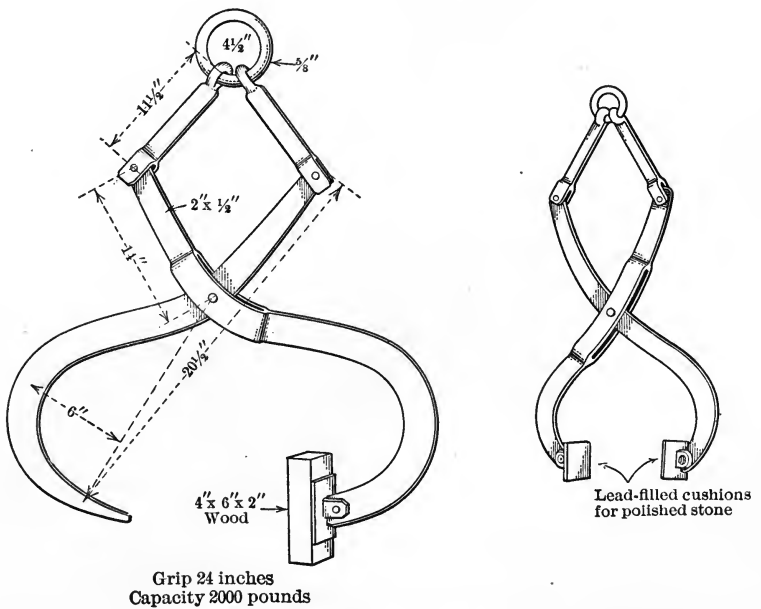
FIG. 72.—Clamps for Lifting Cut Stone.
