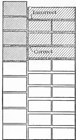
FIG. 84.—Sketch Showing Metal Tie Used to Bond Face Brick with Backing.
