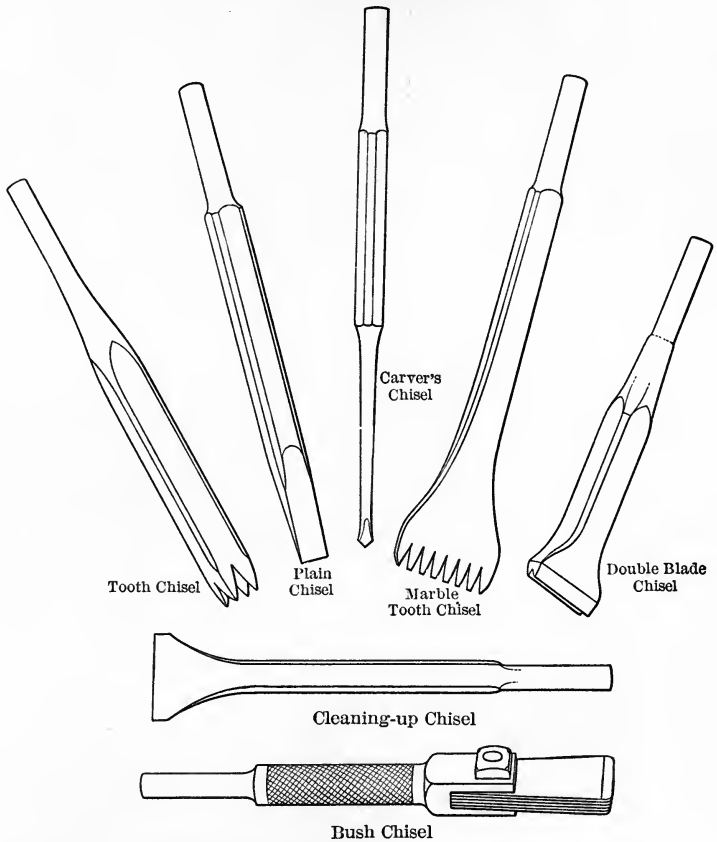
FIG. 27.—Pneumatic Tool Chisels. (George Oldham & Sons Co.)
