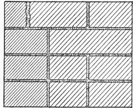
FIG. 85.—Sketch Showing Use of Secret Bond in Brick Masonry.
