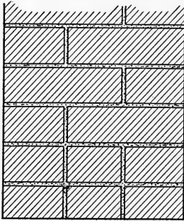
FIG. 80.—Sketch Showing Direct Bonding of Facing and Backing in Brick Masonry.
