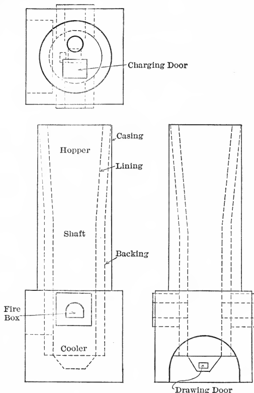
FIG. 53.—Round Kiln with Shaft Drawn In. Lime Kiln.
