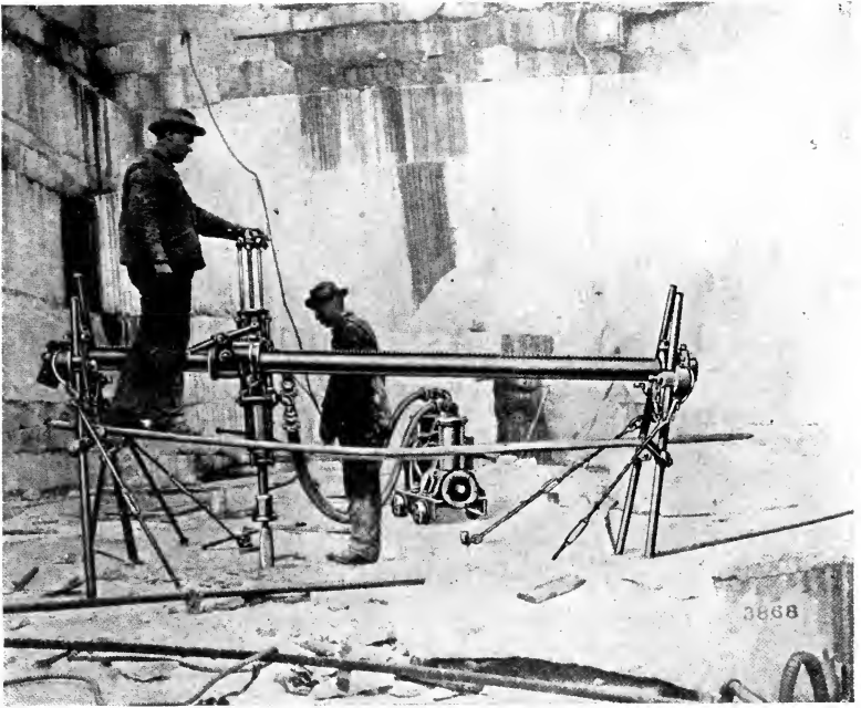
FIG. 12.—“Electric Air” Drill on a Quarry Bar Working in Barre Dark Granite. (Ingersoll-Rand Co.)
