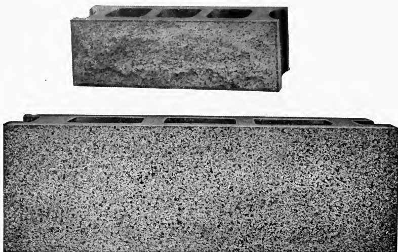
FIG. 96.—Concrete Block 8 x 8 x 24 Inch Granite Faced. Zagelmeyer Process. (Zagelmeyer Cast Stone Block Machine Co.)
