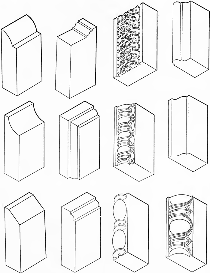
FIG. 50.—A Few Shapes in Which Building Bricks Are Made.
