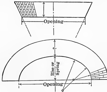
FIG. 90.—Sketch Showing the Use of Special Arch Brick.
