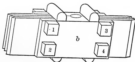
FIG. 19.—Bush Hammers. (a) Solid. (b) With Leaves. "Patent Hammer."
