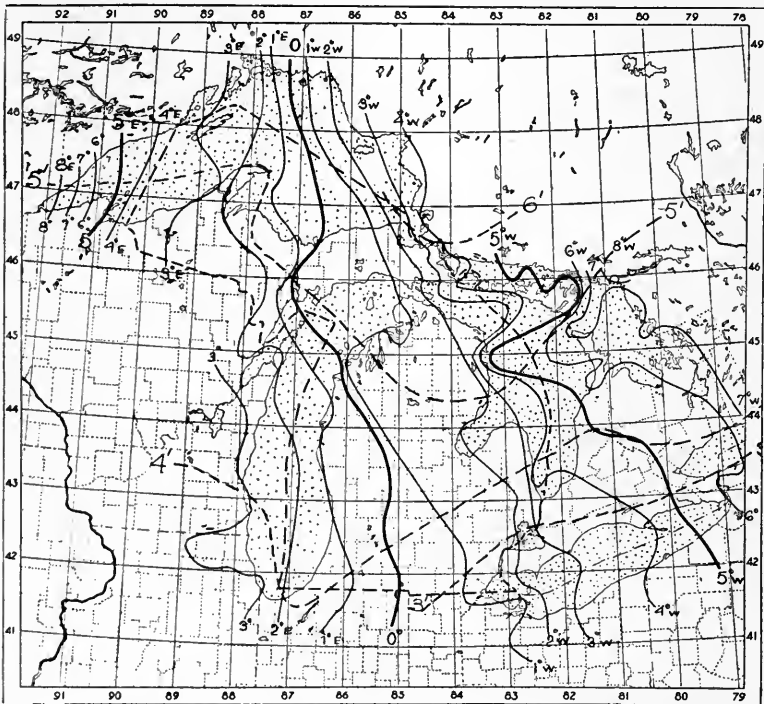
FIG 61 Lines of equal magnetic variation for 1905 giving the number of degrees that the compass points east and west of true north by the solid lines and the change in this variation per year by the dotted line, west variation increasing, east diminishing
