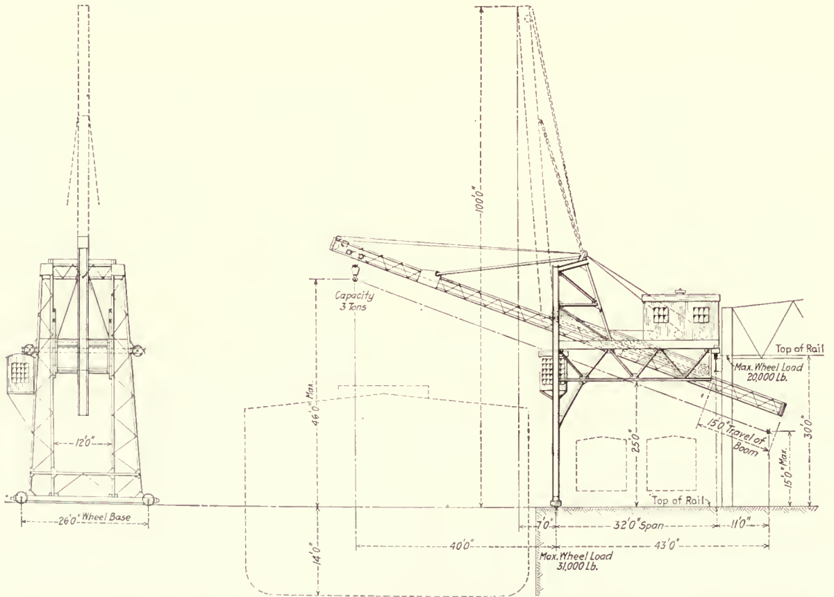
Semi-Portial Wharf Crane with Inclined Boom Equipped with Hoisting Trolley for Delivery Inside of Pier Shed
