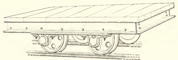
Fig. 1—Four-Wheel Platform Car
