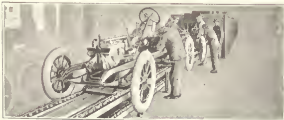
Chassis Assembly.
