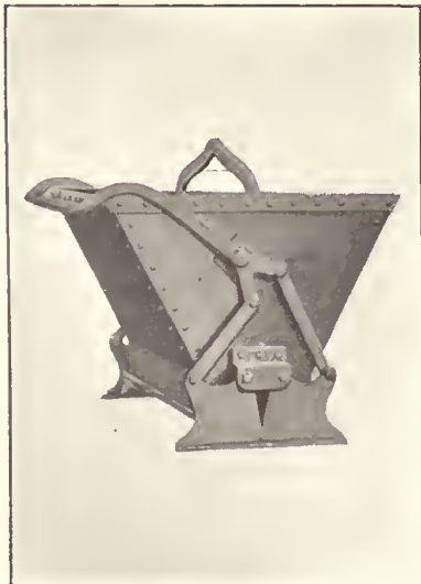
Controllable-Discharge Center-Hinged Bottom-Dump Bucket. Bell-crank Crossbar-Lever Operation
