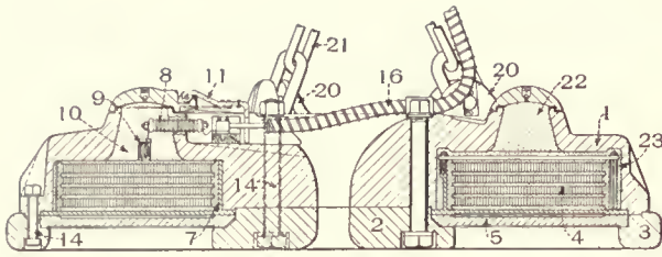
Circular Magnet
