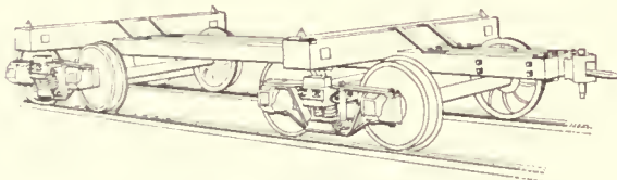
Fig. 38—Logging Car, Wooden Frame
