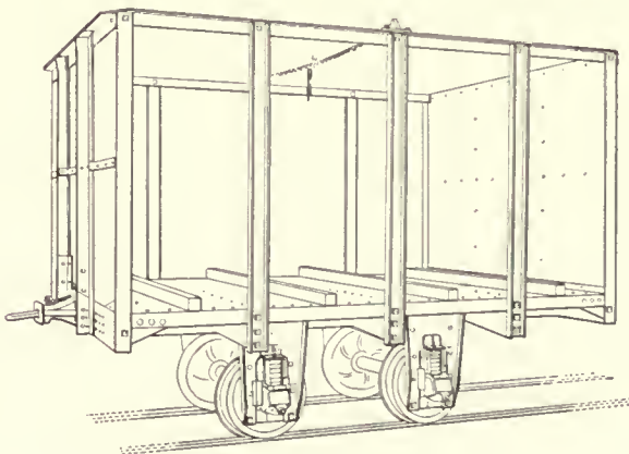
Fig. 50—Cane Car, Top Unloading
