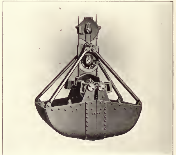
Rope-Reeved Grab Bucket Operated in Bigfts of Line on Hoisting Towers, Cableways, etc.
