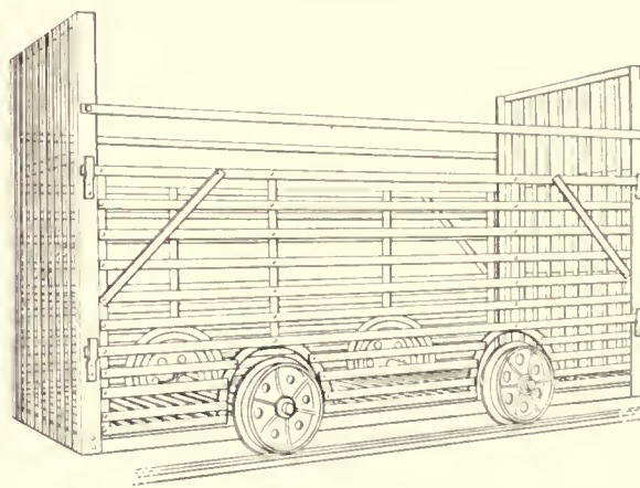
Fig. 37—Charcoal Car
