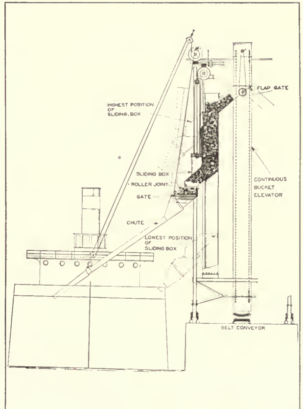
Coaling from a Traveling Tower
