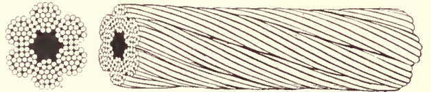
Type H, Flattened Hoisting Rope—Langs' Lay
