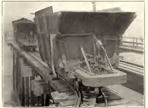
Cable Car With Automatic Dump Attachment
