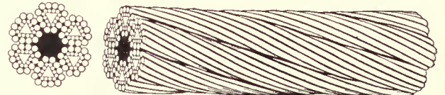
Type B, Flattened Strand Hoisting Rope
