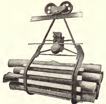
Cordwood Carrier
