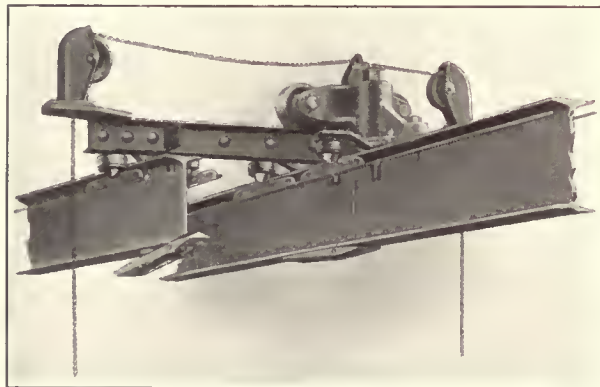
Two-Way Switch
