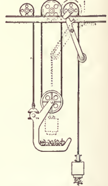
Magnet with Tilting Device
