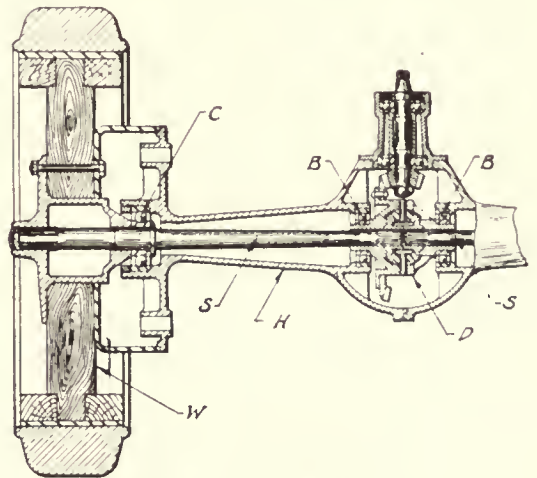
Fig. 6—Semi-Floating Axle
