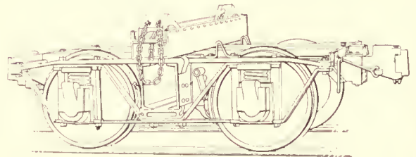
Fig. 40—Logging Truck
