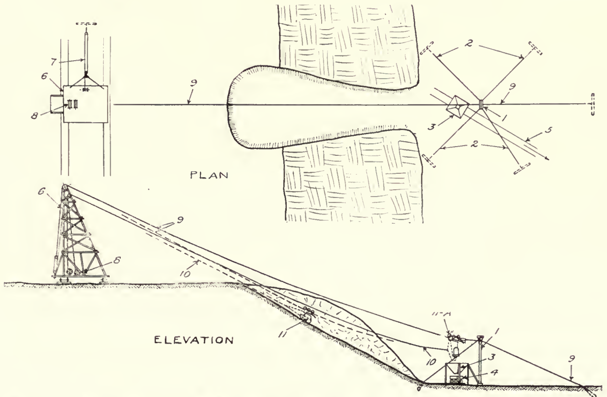
Semi-Gravity Dragline Cableway with Movable Head Tower and A-Frame Tail Tower Handling Clay at a Brick Plant. Rigged for Low-End Dump Into Receiving Hopper for Discharge Into Industrial Cars
