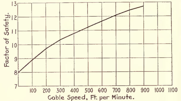
Curve 2—Factors of Safety for Hoisting Cables for Traction Machine Freight Elevators. (Drum Machine Freight Elevators May Use Factors of Safety of 80 Per Cent Given in This Curve)
