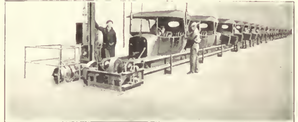
Body Assembly.
