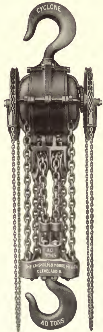
Cyclone 40-Ton High-Speed Chain Hoist. Cyclone Hoists are the only single-unit hoists built for capacities above 3 tons.
