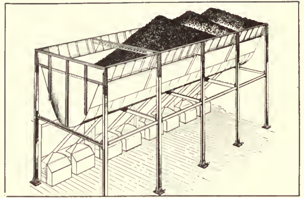
Fig. 2—Suspended Bunker
