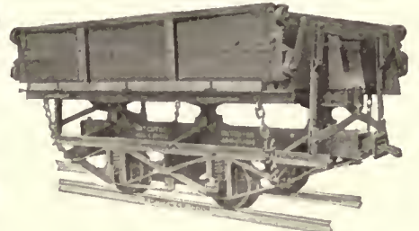
Koppel Square Box Dump.
