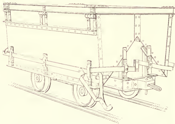
Fig. 28—Gable Bottom Car, Automatic Dumping
