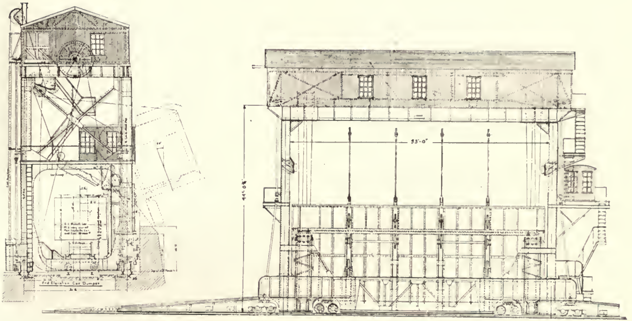
Movable Car Dumper with Portable Inclined Rail Sections
