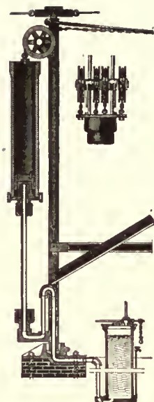
Steam-Hydraulic
