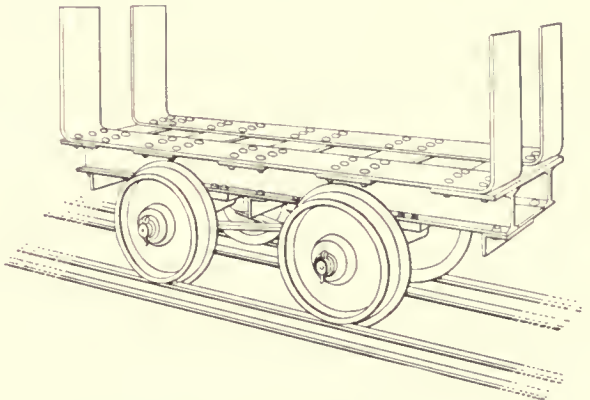
Fig. 67—Car for Short Bars and Coils
