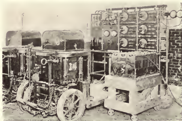
6-Circuit Battery Charging Switchboard in Operation.
