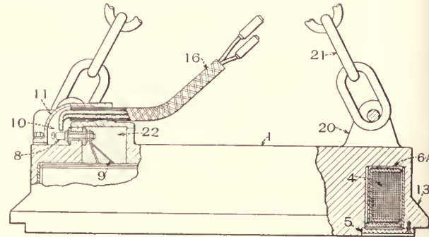
Rectangular Magnet
