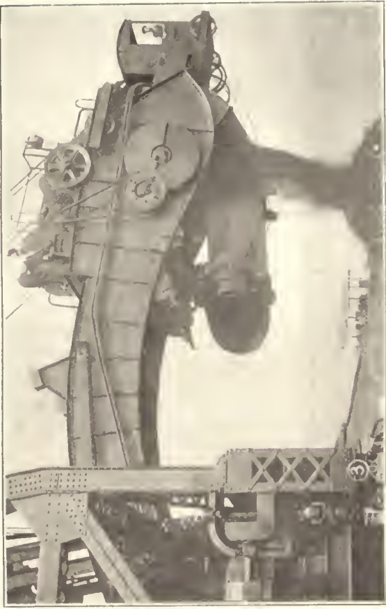
Discharge Nozzle of Coal Dumper and Vessel Loader
