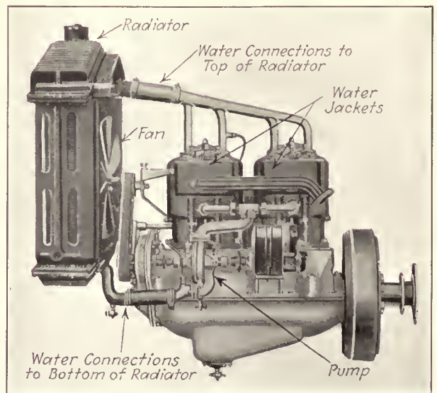
Fig. 33—Cooling System
