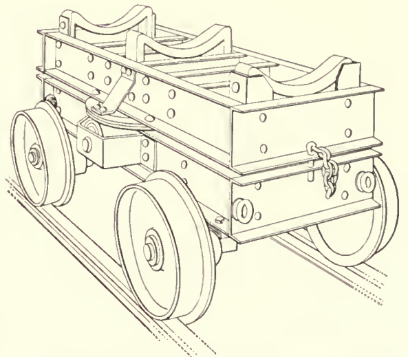
Fig. 68—Swivel Top Car for Forgings
