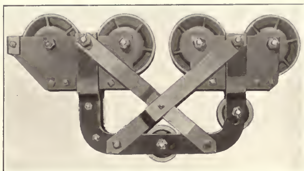
4-Wheel Bar-Frame Carrier with Rocker Wheel Frames
