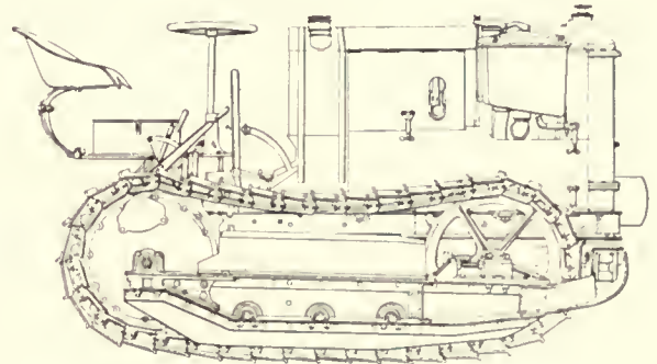
Track-Laying Tractor
