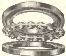
Single-acting Thrust Bearing with Flat Seats (Grooved Races). 1100F Series
