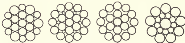
3-sized-wire Construction 1-sized-wire with Fillers 1-sized-wire without Fillers Scale Construction
