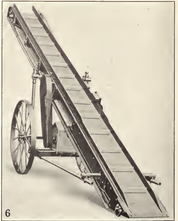
Types of Portable Belt Conveyors: (1) Tronghing Type 60 ft. Span; (2) Self-Propelled Snow Loader; (3) Equipped with Hooks for Attachment to Car or Elevated Track; (4) Hand Wheel Height Adjustment; (5) Equipped with Screening Hopper; (6) Scoop Type
