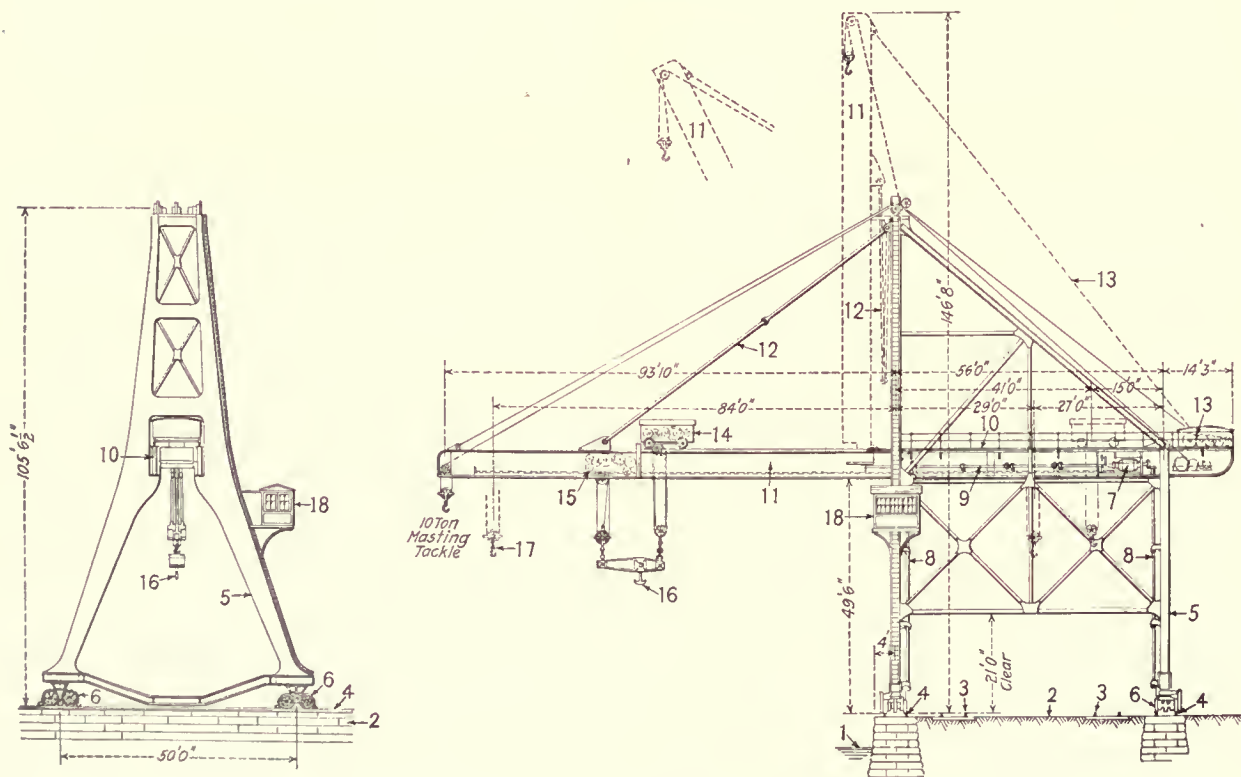
Electric Traveling Double-Cantilever 15-Ton Capacity Shipyard Gantry Crane on Elevated Runway
