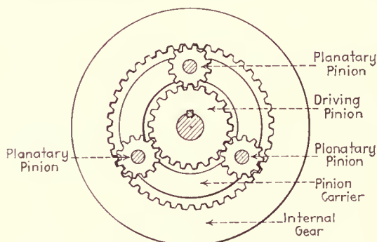
Fig. 16—Planetary Gearing
