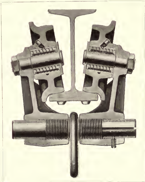
Hyatt equipped I-beam trolley manufactured by Curtis Pneumatic Machinery Company, St. Louis, Mo.
