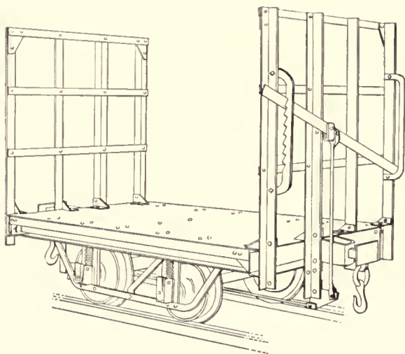
Fig. 47—Cane Car with End Racks
