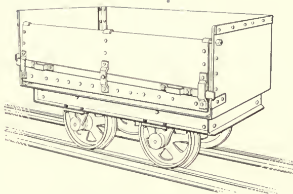
Fig. 77—Coke Charging Car
