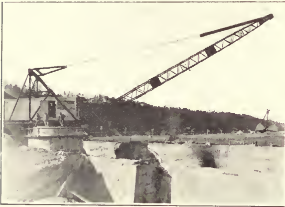
Full Circle Derrick, mounted on concrete base. Capacity up to 4 yd. bucket.
