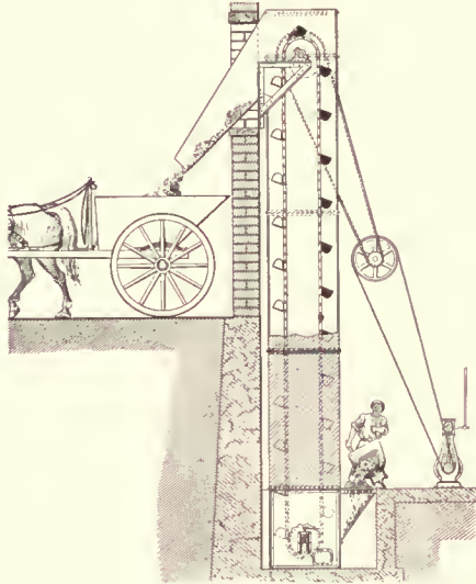
Ash Elevator
