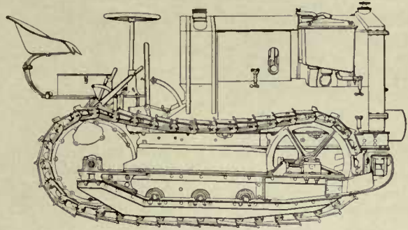
Track-Laying Tractor
