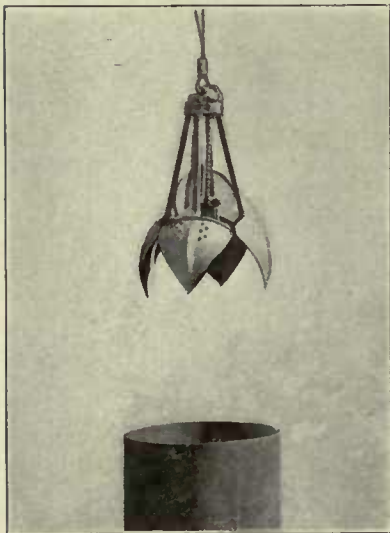
Dwarf Orange-Peel Bucket without Hammer Attachment
