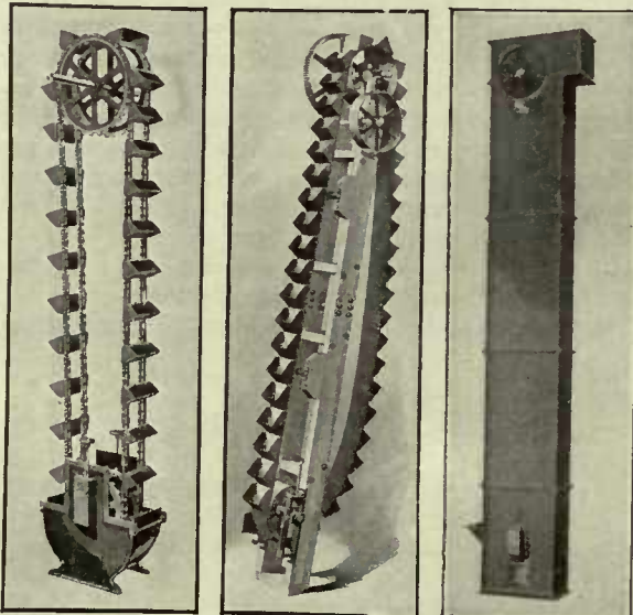
Three Standard Types of Bucket Elevators.
