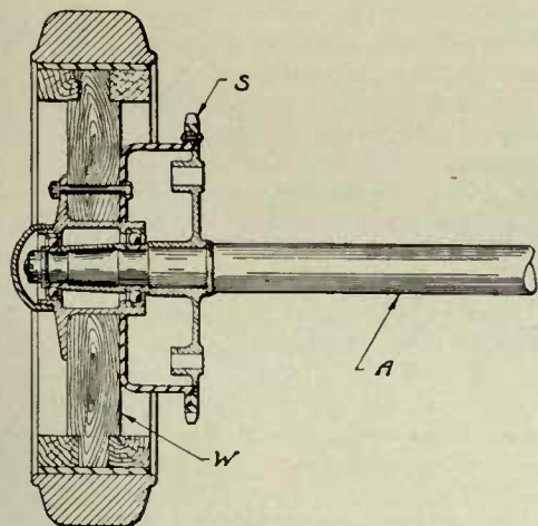
Fig. 4—Simple Form of Dead Axle
