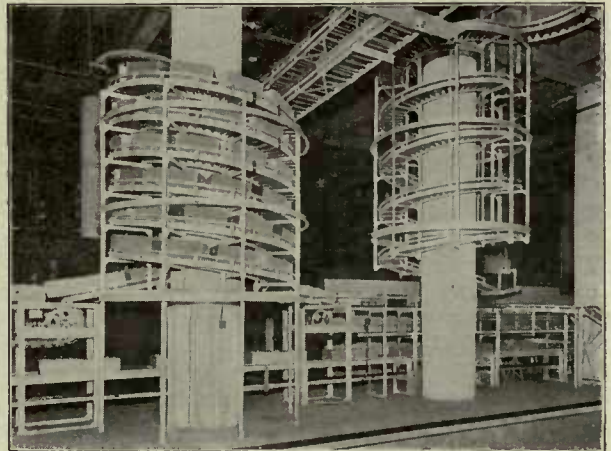
Spiral Located to Conserve Space
