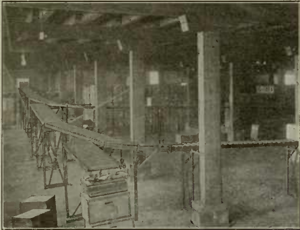
Distribution by Adjustable Curve Sections
