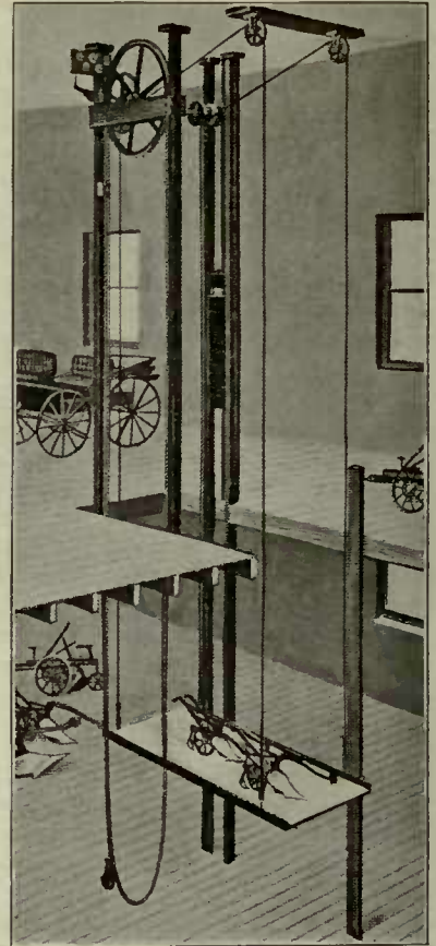
Carriage Elevator
