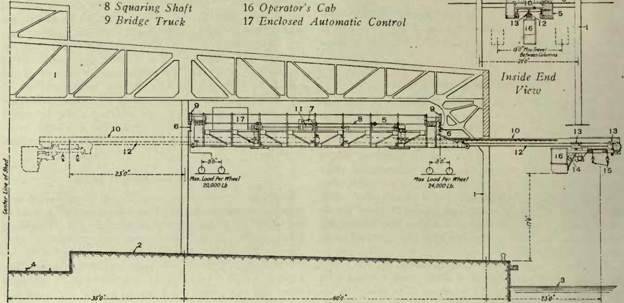
Electric Traveling-Bridge Racking-Cantilever Crane with 4-Ton Capacity Monorail Trolley
