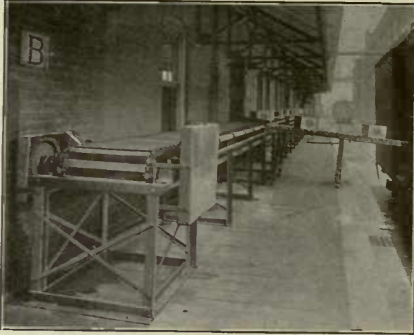
Automatic Discharge to Any Car Door
