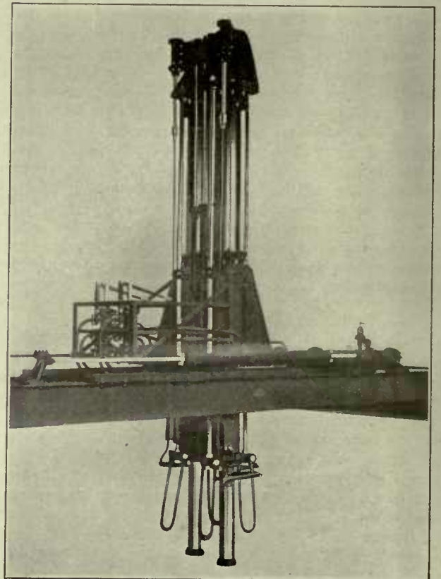
Hydraulic Ingot Stripping Trolley
