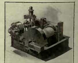
Skip Hoist Engine.
