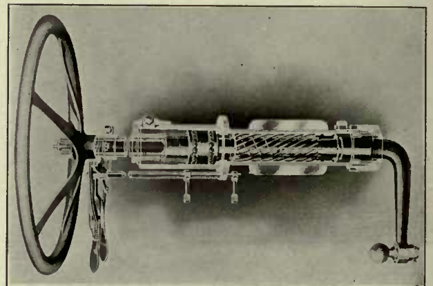
Fig. 26—Double Thread Type
