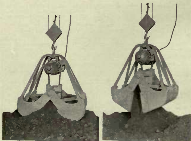
Hayward Electric Motor Bucket. Digging.
