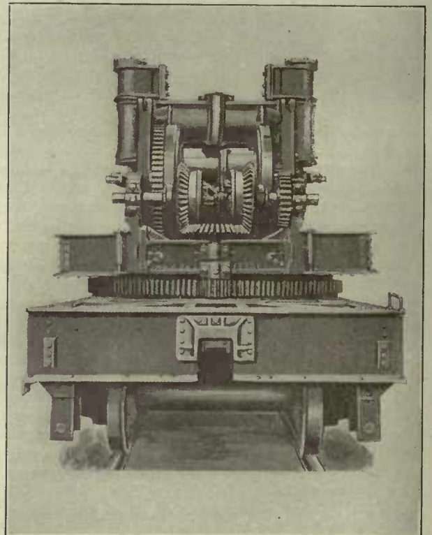
Turntable of Locomotive Crane Showing Hoisting Drums, Rotating Mechanism and Clutch
