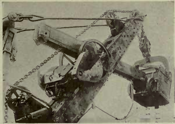
Crowding Motor and Controller on a 65-Ton Electric Shovel Equipped with Four G-E Motors.
