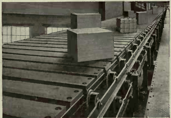
Link-Belt Apron Conveyor Handling Boxes.
