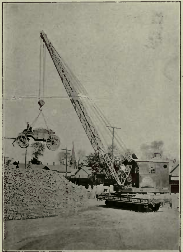
Steam Locomotive Crane Handling Paving Blocks in Dump Wagon with Fall Block, Hoisting Hook, and Chain Grab Hooks
