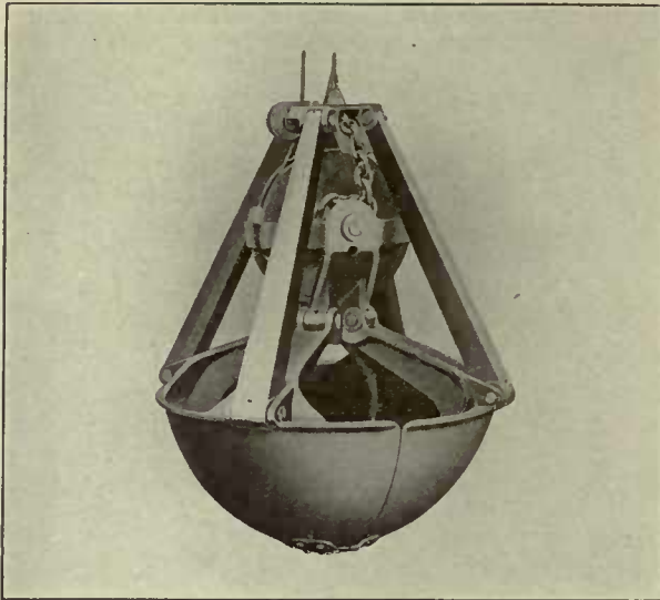
Four-Blade Chain Operated Power-Wheel Orange-Peel Bucket for General Excavation Work
