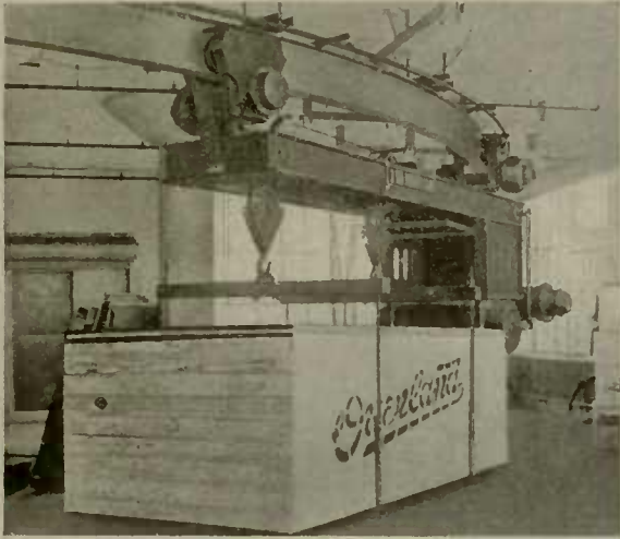
Form 18 Hoist.
