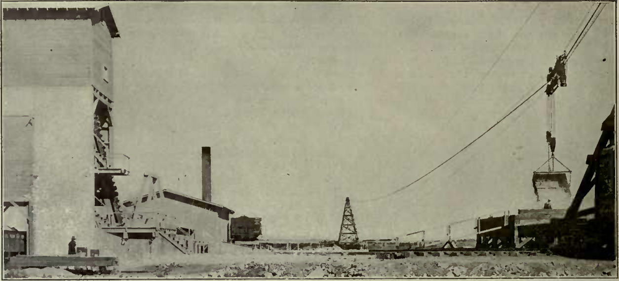
Endless-Rope Suspension Cableway Handling Loose Material with a Skip
