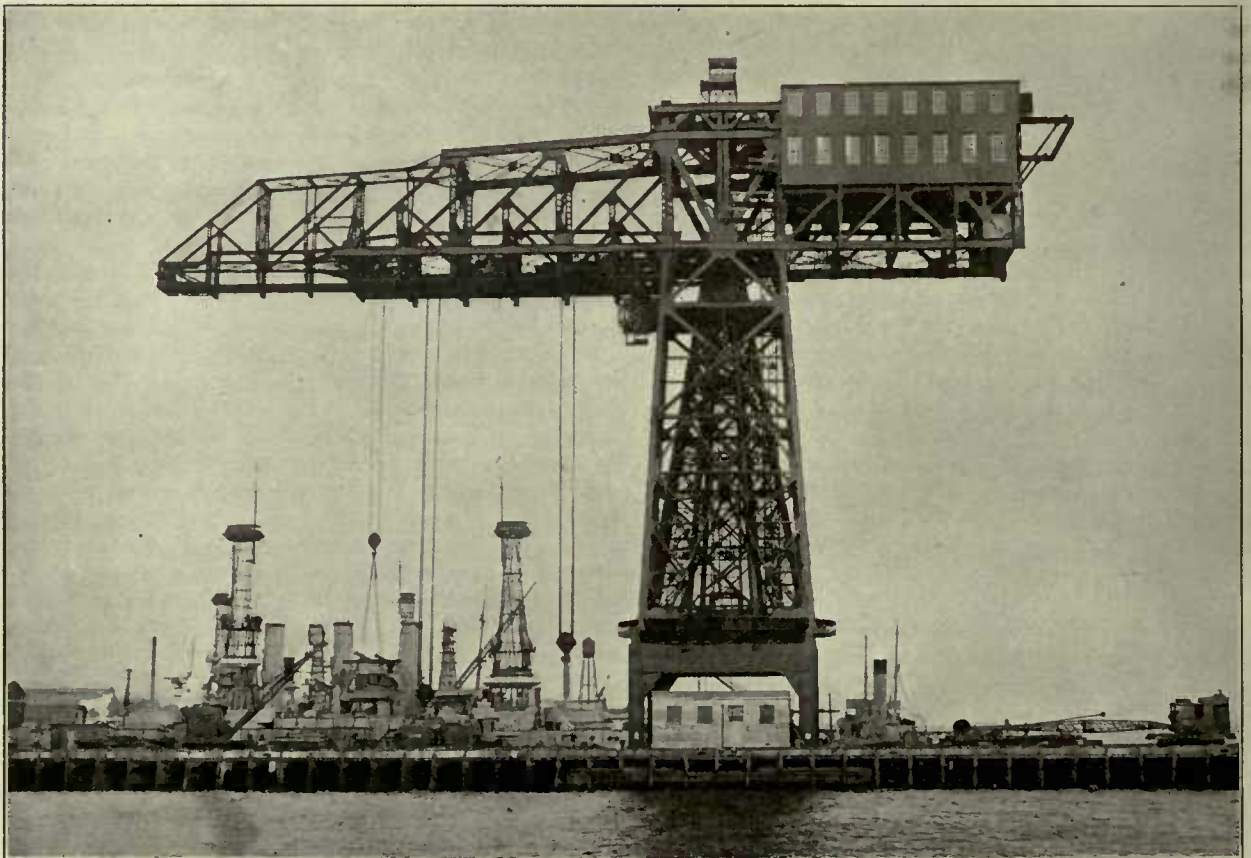
Stationary Hammerhead Portal Crane Installed in Philadelphia Navy Yard. Capacity 350 Tons at 115 ft. Radius; 50 Tons at 90 ft. Radius. Overall Height, 230 ft.
