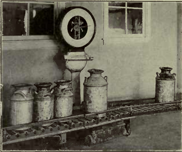
Weighing on Gravity Conveyor
