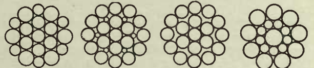
3-sized-wire Construction 1-sized-wire with Fillers 1-sized-wire without Fillers Seale Construction
