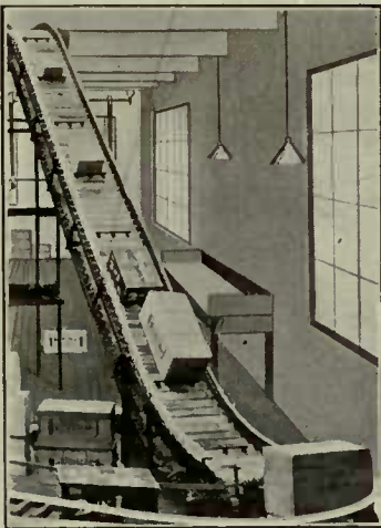
Inclined elevator taking delivery from gravity roller conveyor.
