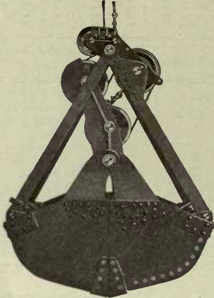
Williams "Favorite" Bucket.
