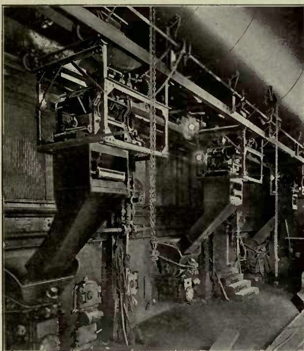
Individual Automatic Scales
