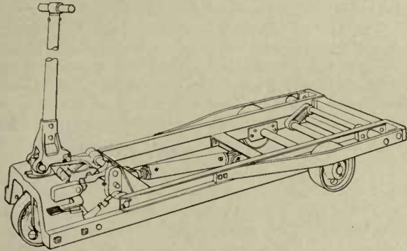
Lift Truck
