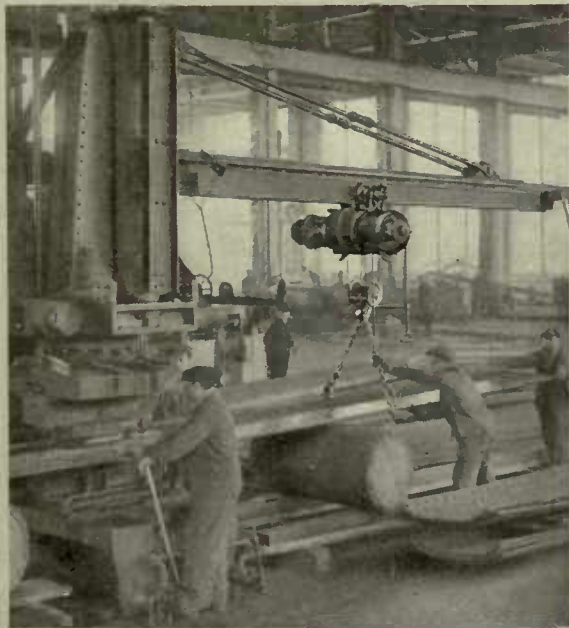
Bracket Crane with Form 1-X Hoist
