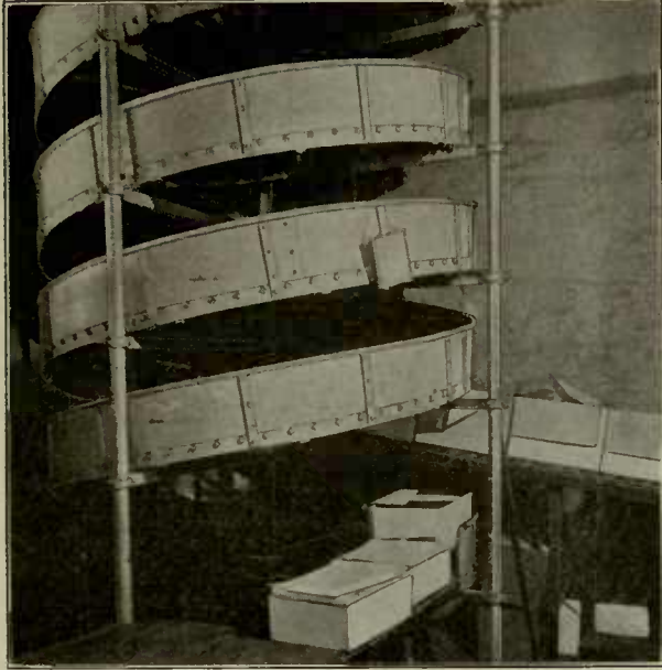
Double Runway with Solid Guard Rails
