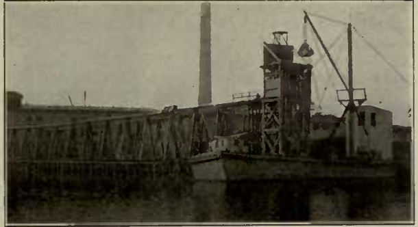
Automatic Railway Delivering Coal from a Barge
