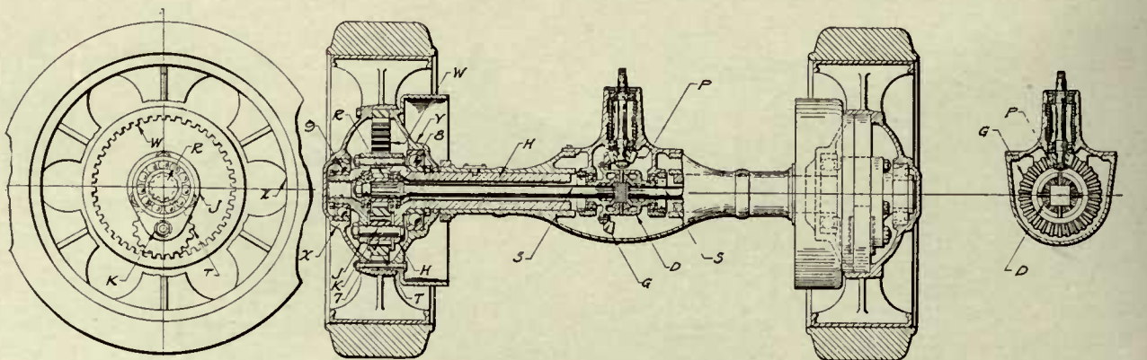
Fig. 15—Double Reduction Internal Gear
