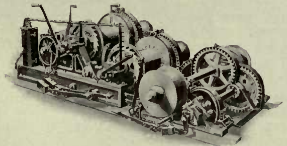
Two Drum Electric Hoist, With Derrick Swinging Gear
