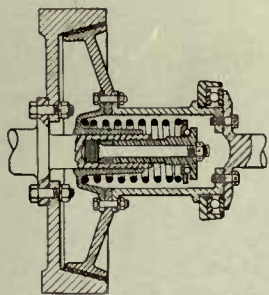
Fig. 27—Cone Clutch
