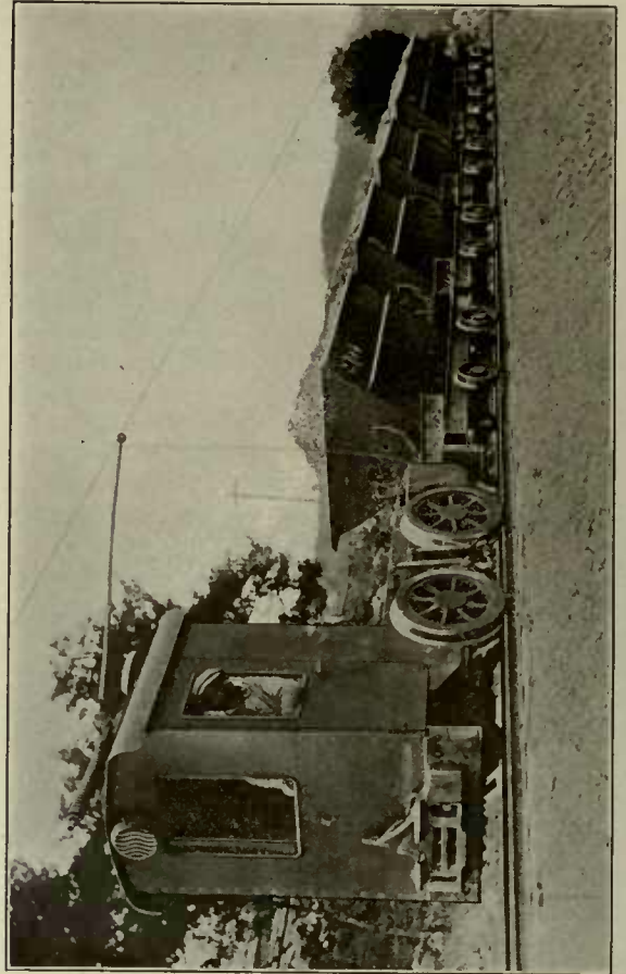
Electric Trolley Locomotive; Fertilizer Works
