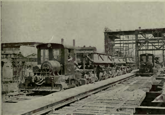
G-E Locomotives at Work in Chemical Plant.
