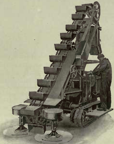
B-G Self-Feeding Bucket Loader (Patented).
