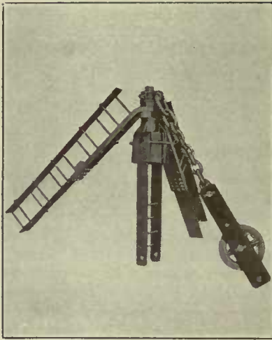
Cast Steel Stiff-Leg Derrick Mast Top with Wrought Iron Timber Straps and Chain Topping-Lift Connection
