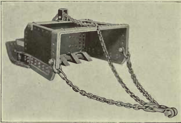
Bottomless Power-Scaper Drag-Line Bucket for Digging Hard-Packed Material
