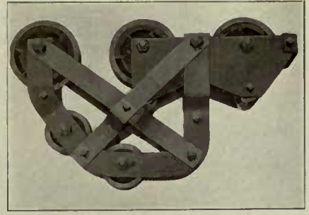
3-Wheel Bar-Frame Carrier
