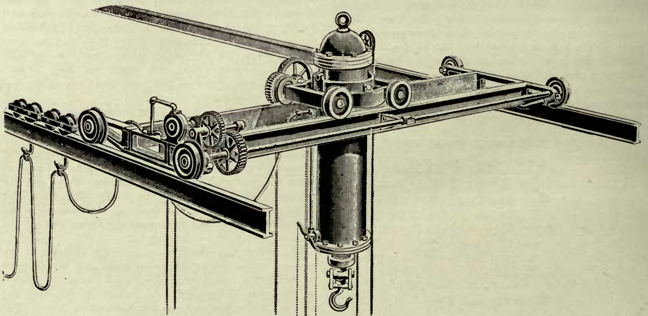
Hand Operated Overhead Travelling Crane With Oil Governed Hoist and Air Hose Trolleys
