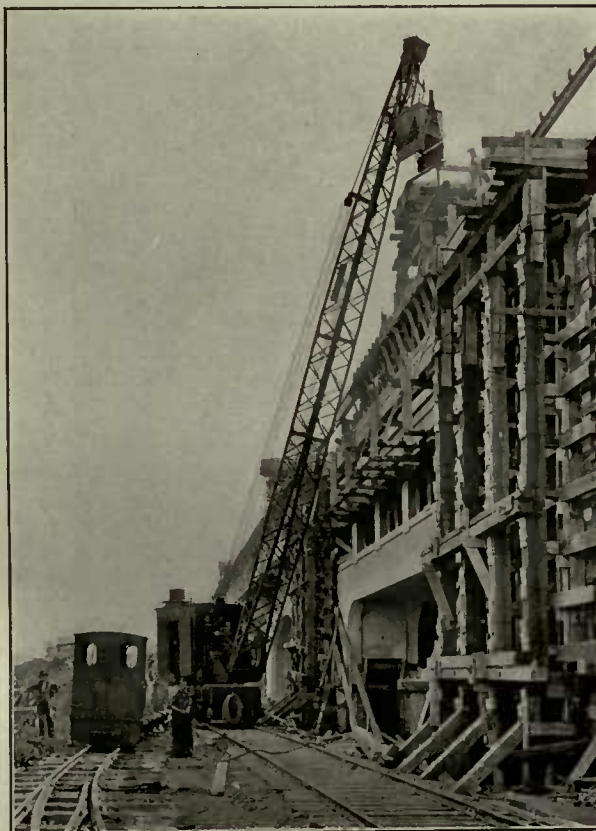
Steam Locomotive Crane Handling Bottom-dump Bucket in Concrete Construction Work
