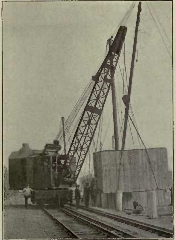
Steam Locomotive Crane Handling Heavy Freight from Car to Lighter for Export. Equipped with Shackle, Chains and Rope Slings
