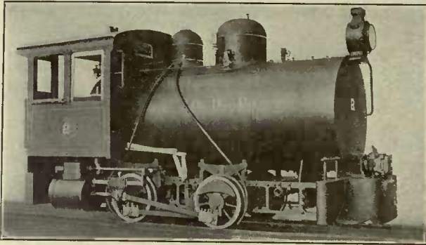
Fireless Locomotive
