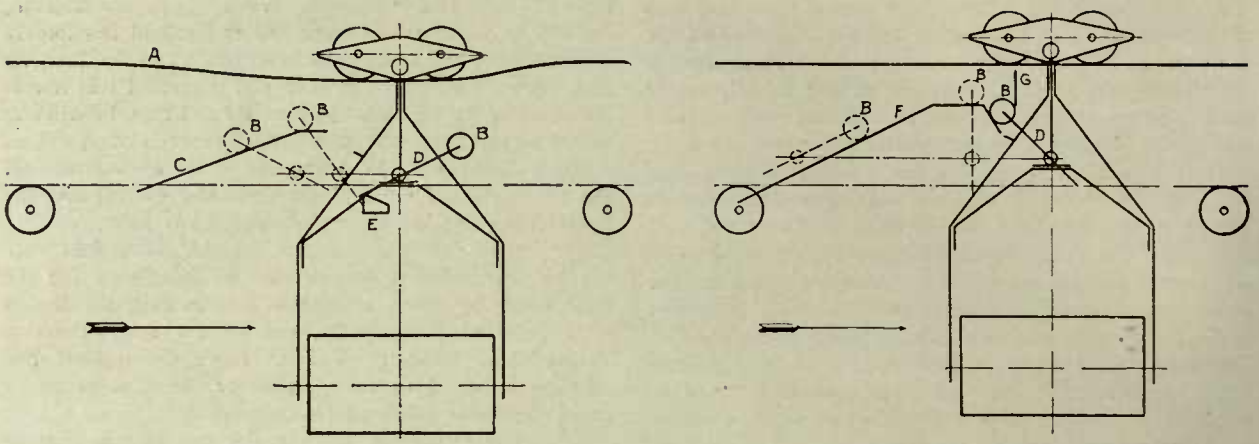
Attaching Detaching Cable Tramway—Carrier Attaching and Detaching Device
