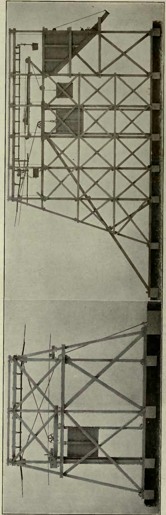
Cable Tramway—Intermediate Anchorage and Tension Station
