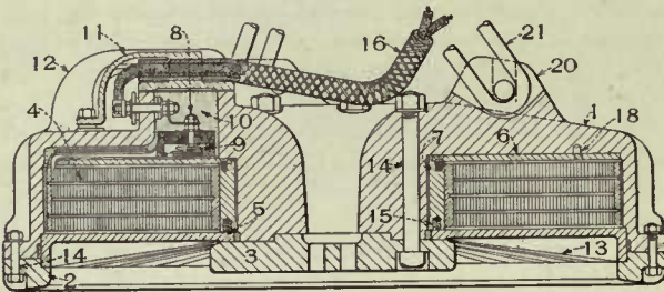
Circular Magnet
