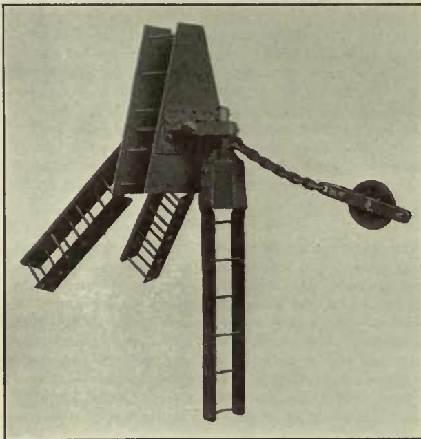
Structural Steel A-Frame Top with Chain Topping-Lift Connection
