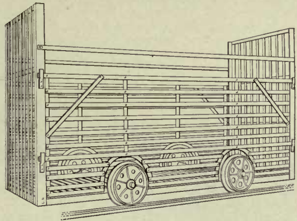
Fig. 37—Charcoal Car
