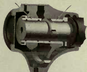
Section of Bearing Housing.
