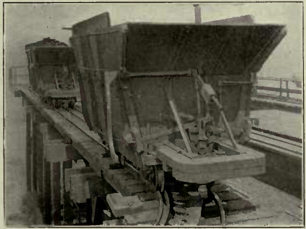
Cable Car With Automatic Dump Attachment
