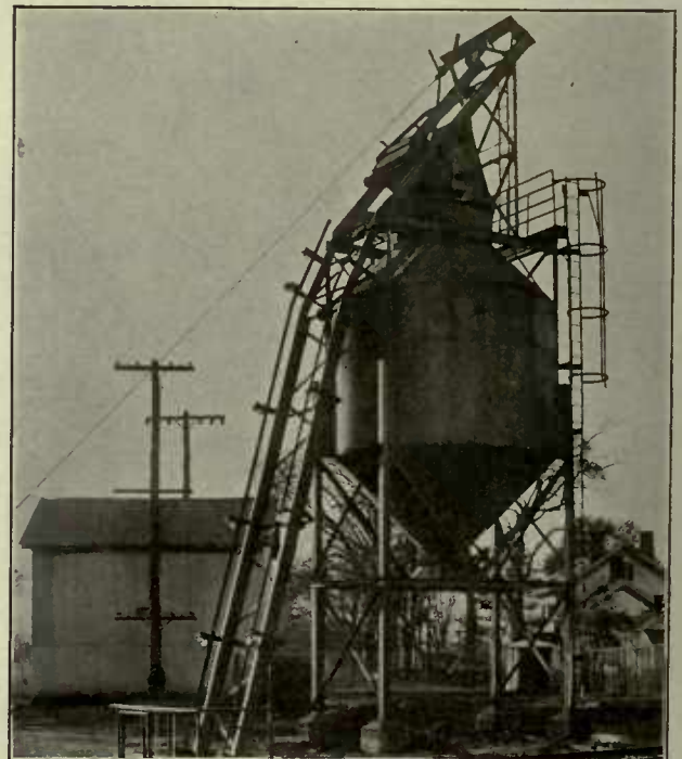
Fig. 6—Single Circular Bin
