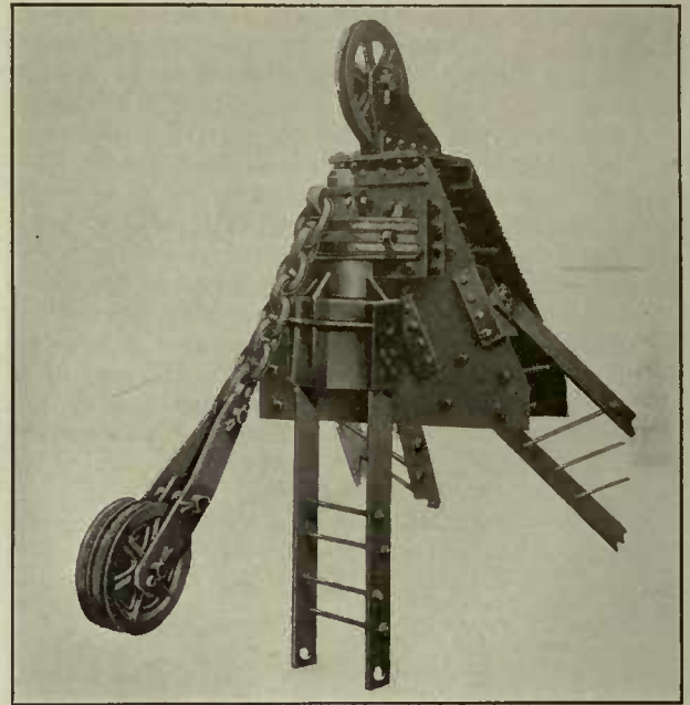
Structural Steel A-Frame Top with Single-Sheave Rooster and Chain Topping-Lift Connection
