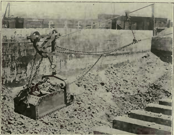
Reclaiming Coal from Storage Pit.
