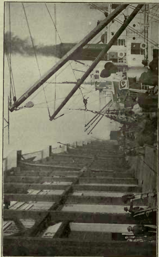
Cargo Handling Gear Rigged with Hook for Handling Package Cargo with a Net
