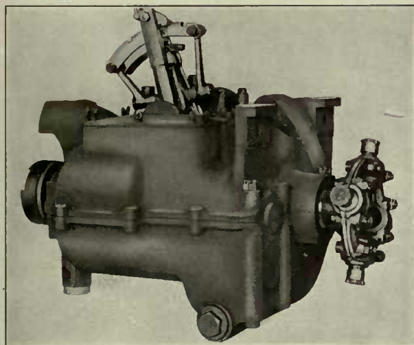
Fig. 18—Amidship Type Transmission
