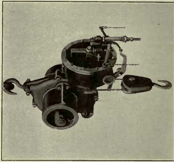
Air-Motor Hoist with Rotating Cylinders, Two-Ton Capacity with Two-Strand Load Cable
