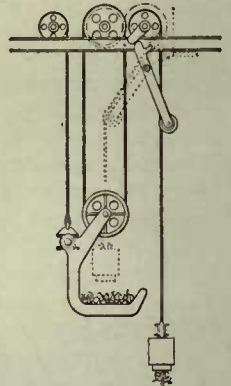
Magnet with Tilting Device
