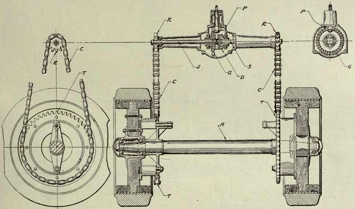
Fig. 10—Chain Drive
