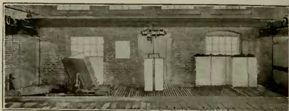
Maris Hand Push Crane with Enclosed Electric Hoist in Can Ice Plant.
