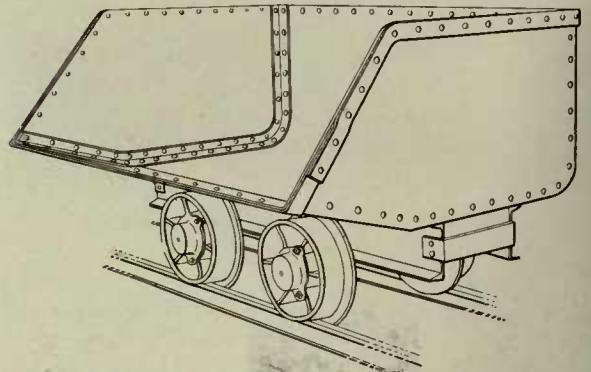
Fig. 16—Charging Car, Inclined Sides
