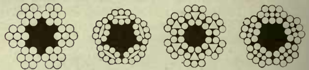
STANDARD TRANSMISSION AND HAULAGE ROPE—6 STRANDS, 7 WIRES EACH—HEMP CORE
