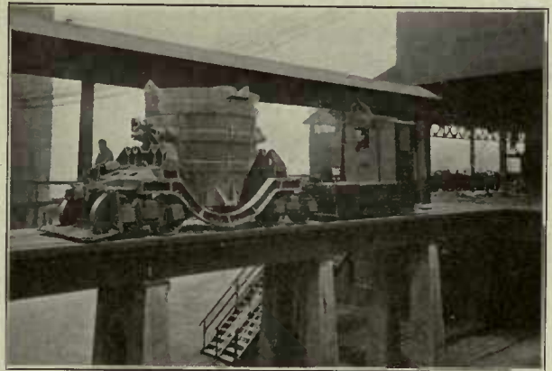
Steel Ladle Car and Electric Locomotive
