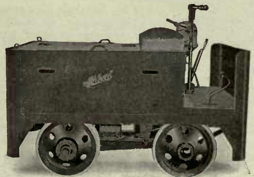
Ideal Tractor Assembled.
