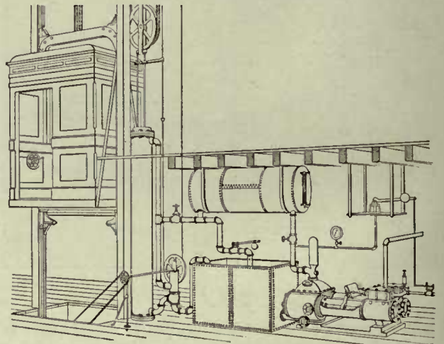
General Arrangement of an Hydraulic Elevator
