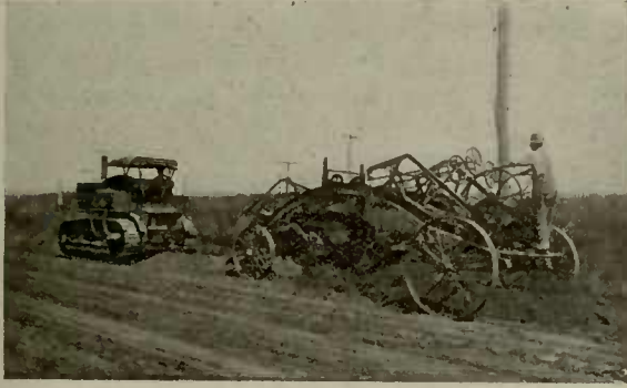
Holt "Caterpillar" Power Is Ideal for Pulling Road Machinery.
