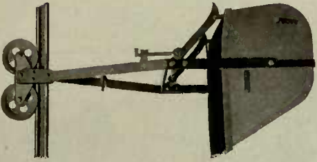
Self-Dumping and Self-Righting Bucket for Reversible Tramway
