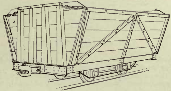
Fig. 49—Cane Car, Drop Side Doors
