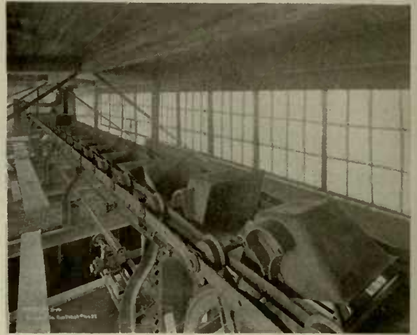
McCaslin Overlapping Pivoted Bucket Conveyor.
