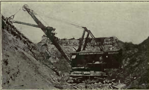
Electric Shovel Digging Power Canal at Niagara Falls, Canada, Operated by A. C. Type MA Motors.
