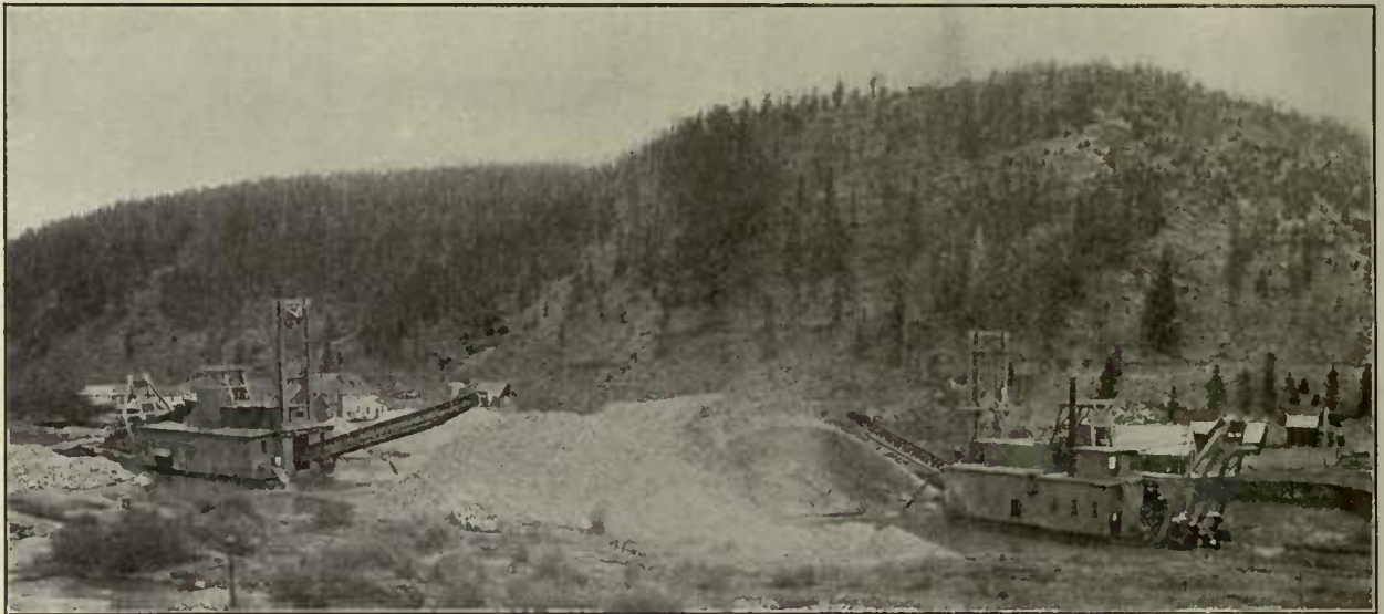
Two Placer Dredges at Work. Elevator or Dredging End Shown at Right, Disposal End at Left
