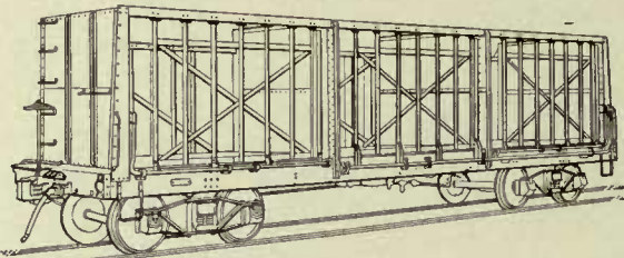
Fig. 42—Side Discharge Cane Car, Hinged Stakes
