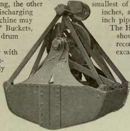
Illustration A-719. Hayward Class "E." Ore Bowl Clam Shell Bucket.
