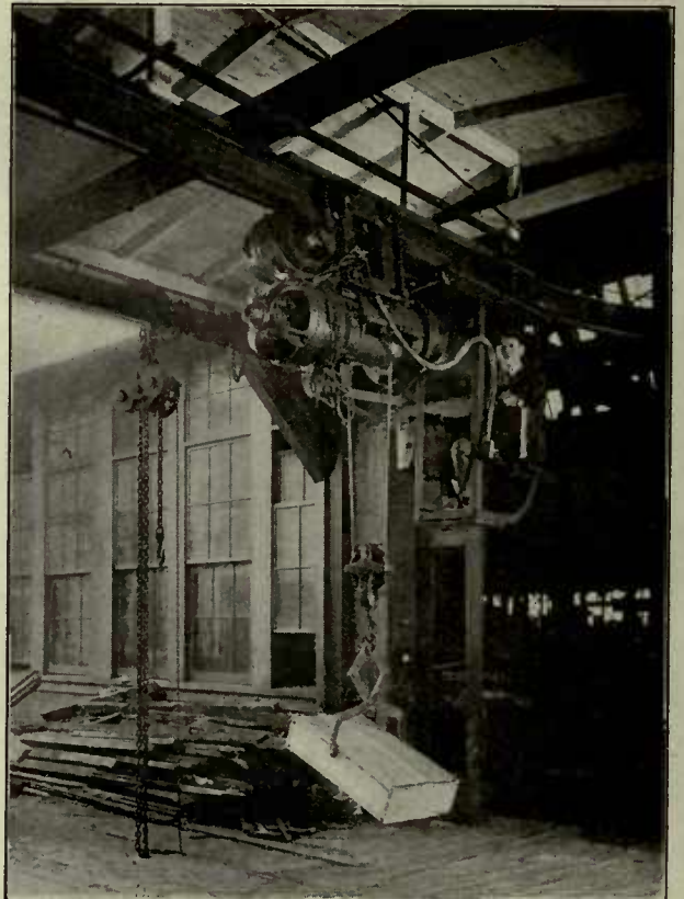
Monorail Hoist Handling Boxed Material with Tongs. Chain Hoist in Background
