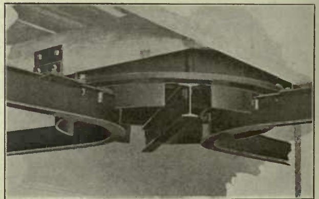
Rotating Switch
