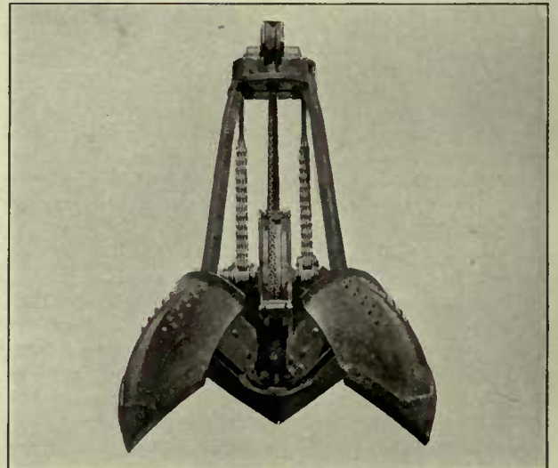
Three-Blade Orange-Peel Bucket with Blades Cut Off for Handling Large Lump Material
