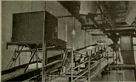
Merrick Conveyor Weightometer Weighing Material in Transit on a Belt Conveyor.
