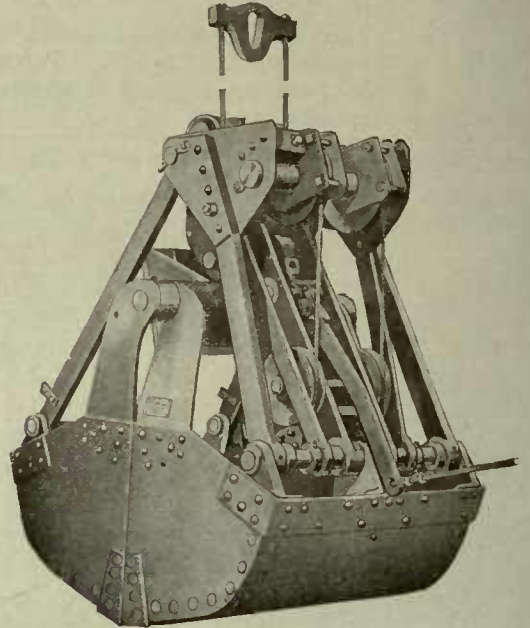
Williams No. 3 Single Hook Foundry Bucket.
