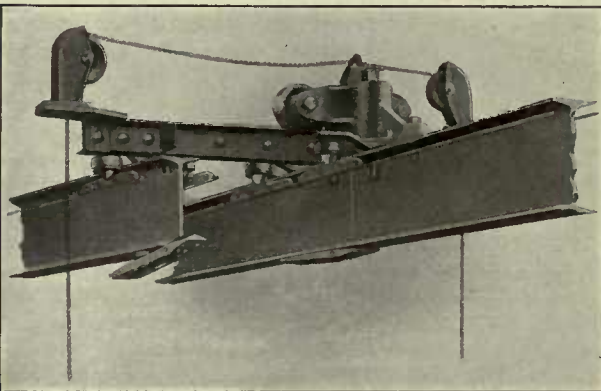
Two-Way Switch
