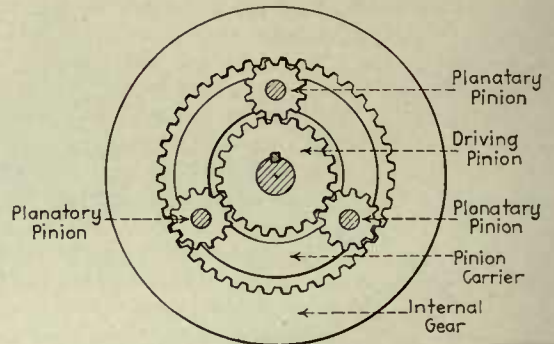
Fig. 16—Planetary Gearing
