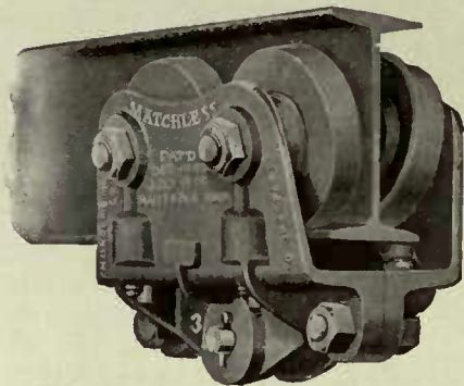
C-M Matchless Adjustable Frame Trolley (also built in geared type). Hoist hook reaches within 1½" of I-Beam.
