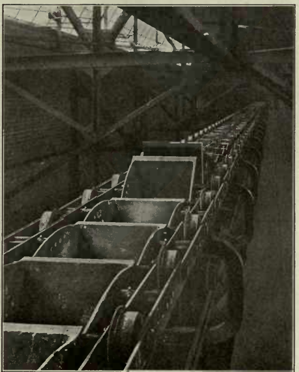
Pivoted Bucket Carriers
