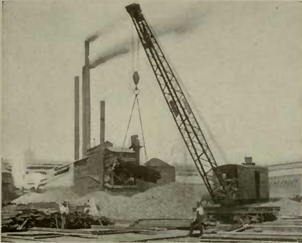
Brownhoist No. 4 Steam Locomotive Crane, Mounted on Standard M. C. B. Trucks, Handling a Bundle of Rails at a Steel Mill.
