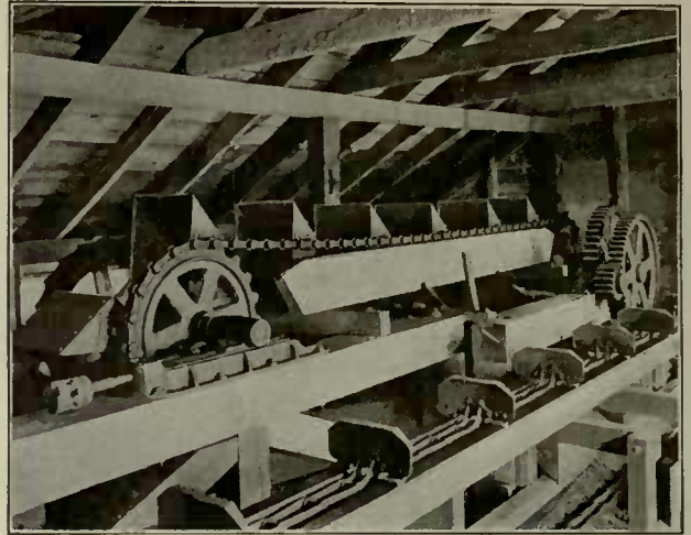
Delivering to Flight Conveyor
