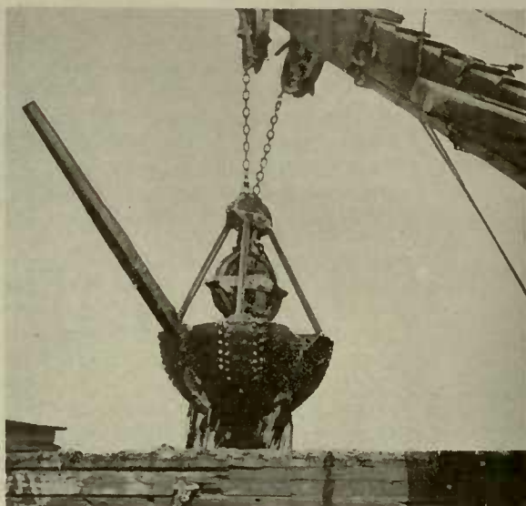
Vulcan Orange-Peel Dredging.
