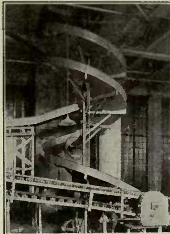
Combination of multiple spiral chute and power driven conveyor.
