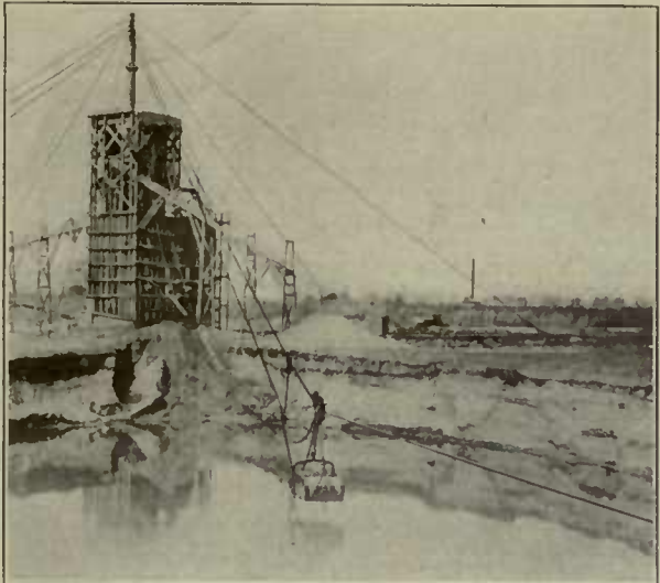
Excavating Gravel from Under Water and Conveying to Screening Plant.
