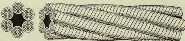
Steel Clad Special Flexible Hoisting Rope
