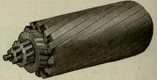
Locked Coil Tramway Cable.
