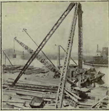
5-Ton Self Slewing Derrick.
