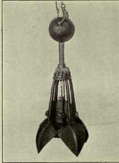
Dwarf Orange-Peel Bucket with Hammer in Raised Position
