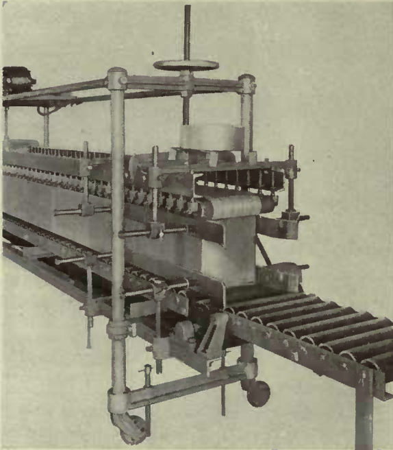
End View of Portable Top and Bottom Sealing Machine.
