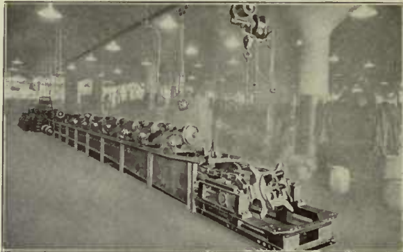
Motor Assembly.
