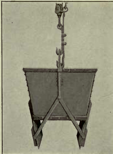
Controllable-Discharge Double-Bail Two-Line Bottom Dump Bucket
