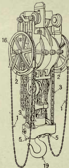
Duplex Gyrotray Gear.
