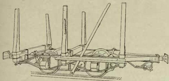
Fig. 41—Lumber Car
