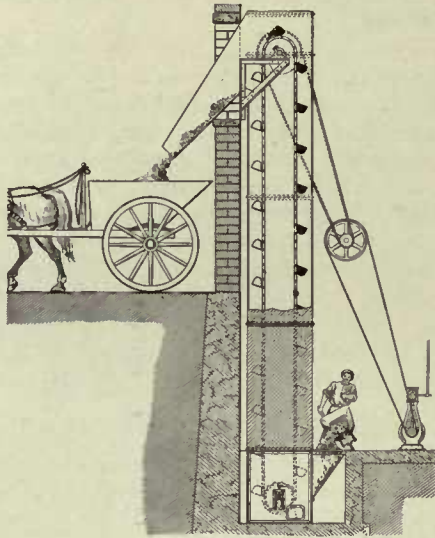
Ash Elevator
