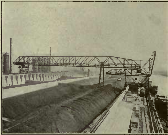
10-Ton Coal Unloader and Bridge and 11-Ton Ore Bridge.
