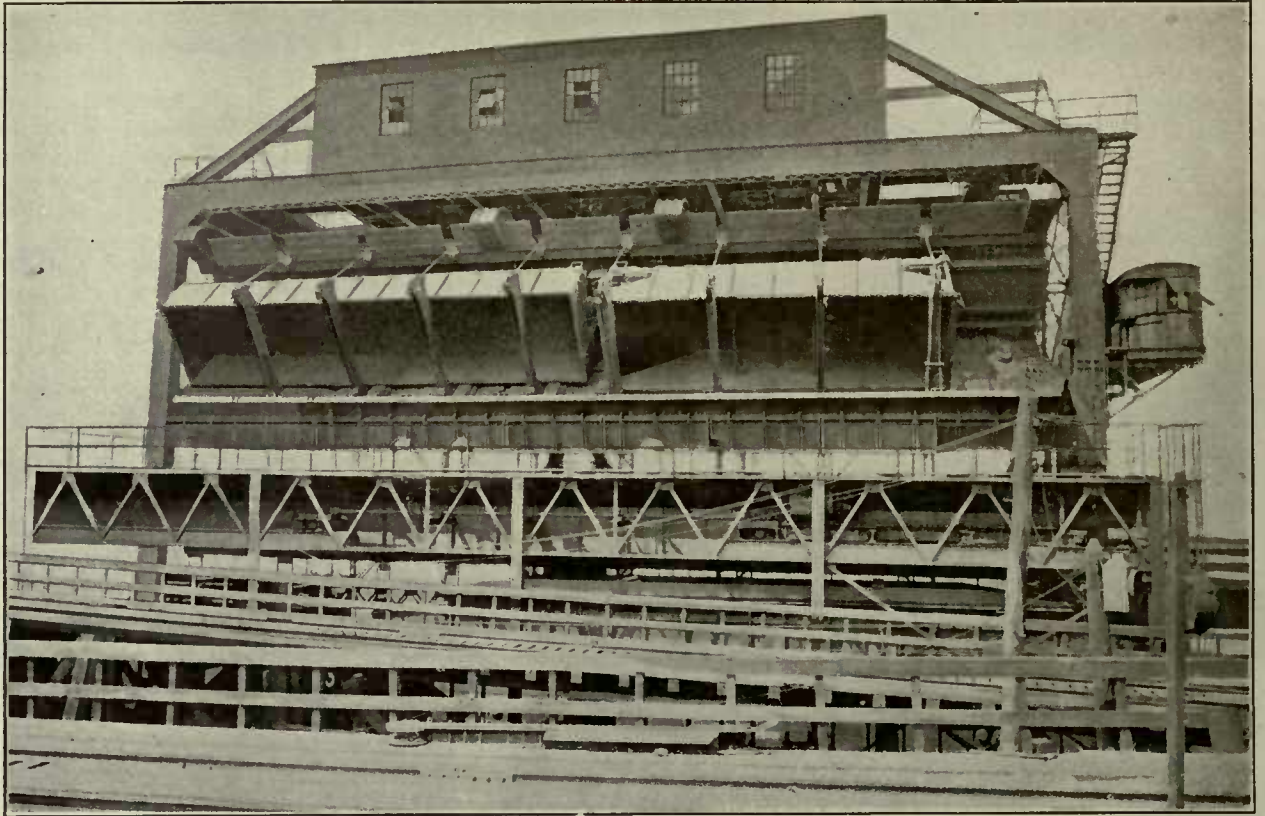
Tandem Car-Dumper with Two Cars in Dumping Position
