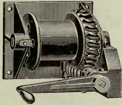
Worm Gear
