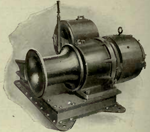
Electric Back Geared Winch.
