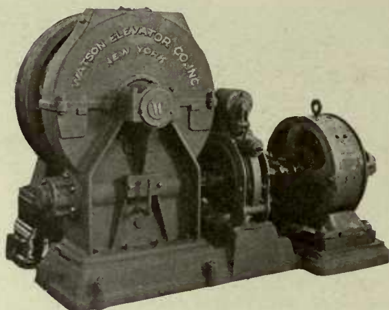
Watson Machine. Note Accessibility of Double Acting Ball Bearing Thrust.
