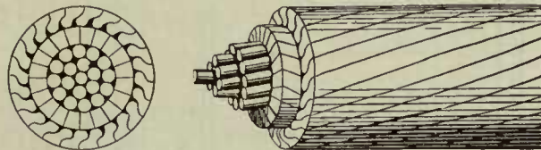
Locked-Coil Track Cable
