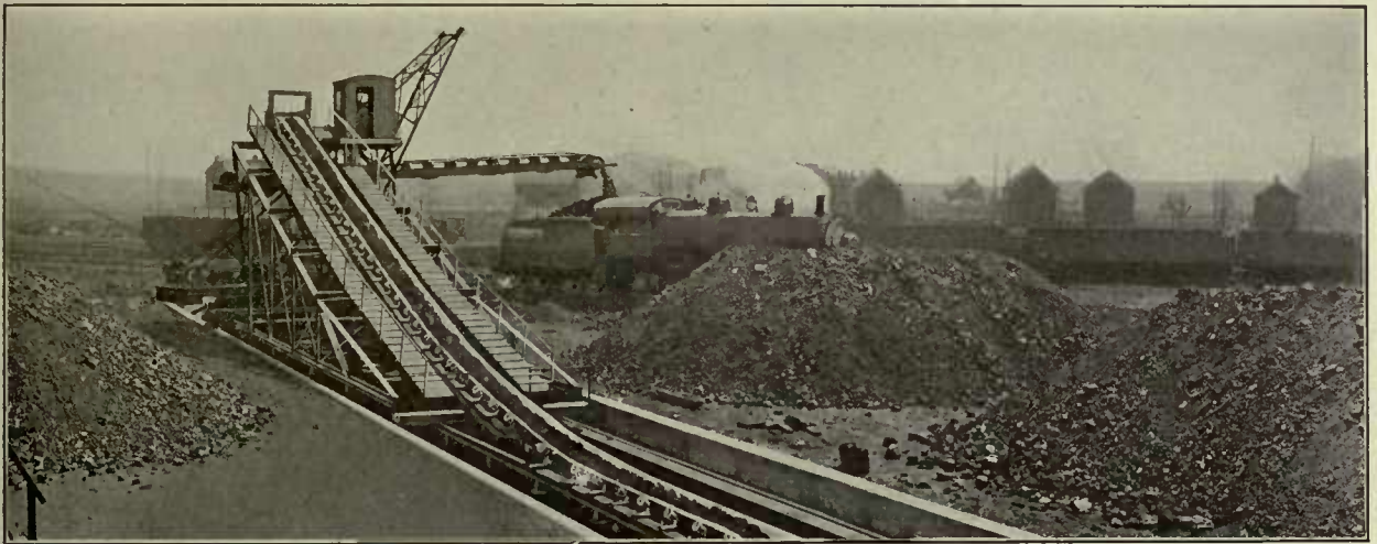
Fig. 18—The Stacker May Be Used for Storing or Coaling Locomotives
