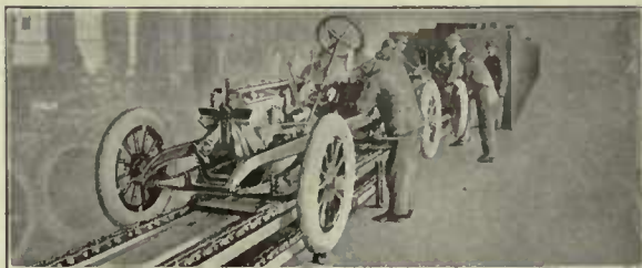
Chassis Assembly.
