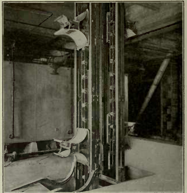
Self-dumping Arms Discharge at Any Floor
