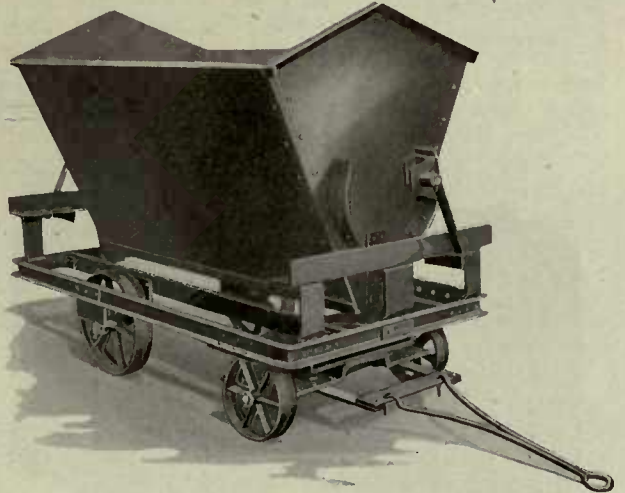
Mercury Side Dump Trailer—Type A-206
