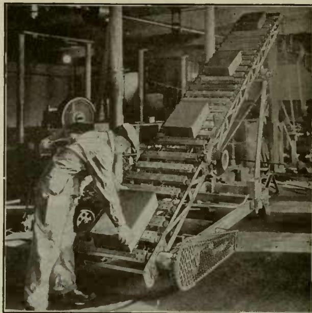
High Type Apron for Boxes
