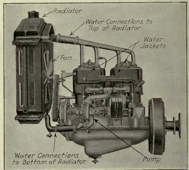
Fig. 33—Cooling System
