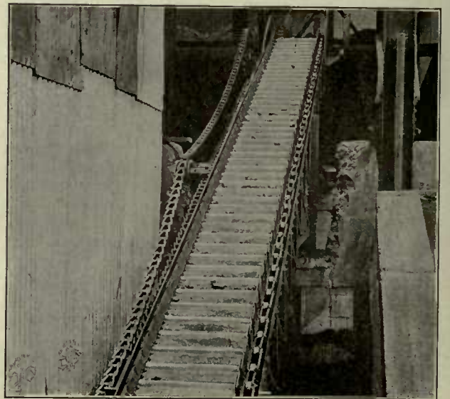
Applications of Apron and Pan Conveyors
