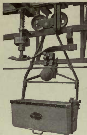
Self Dumping Bucket.
