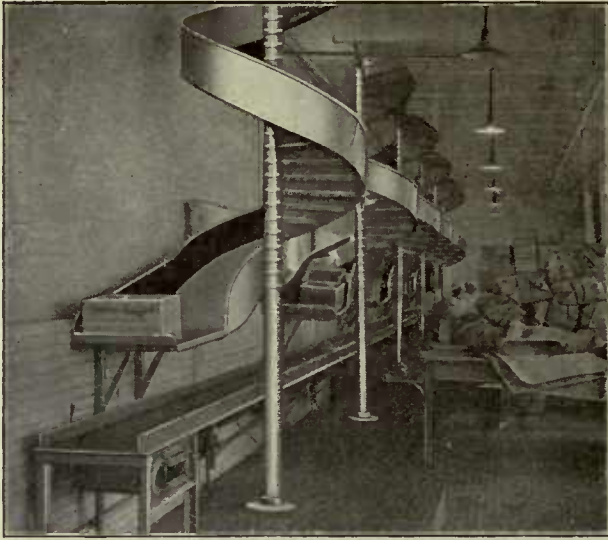
A Bank of Distribution Spirals
