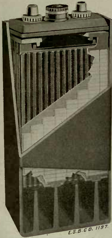
Cut-away Cell Showing New Construction — Positive Plates and Their Supporting Ribs; Negative Plates and Their Supporting Ribs; With Separators Extending Below All Plates.
