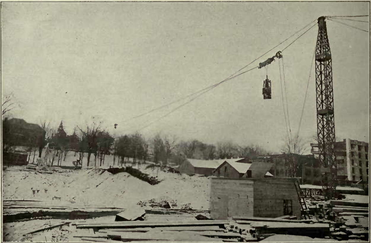
Single Rope Cableway Equipped with Single Line Automatic Grab Bucket for Handling Loose Material
