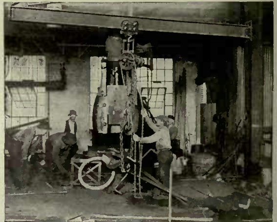
Cyclone Shock Absorber Hoist Suspended from Matchless Trolley Serving a Trip Hammer.
