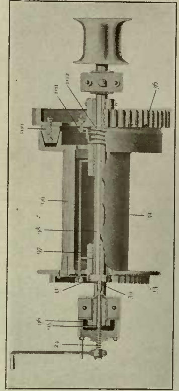
Friction Drum and Drive
