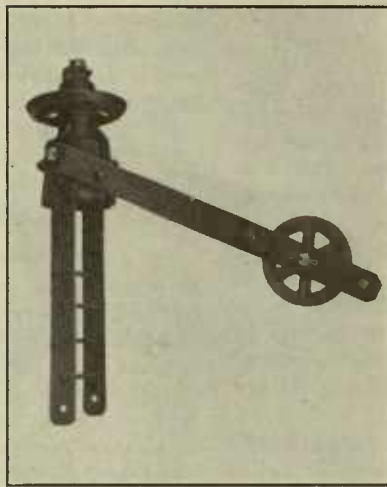
Cast Steel Guy Derrick Mast Top with Wrought Iron Strap Timber and Topping Lift Connections
