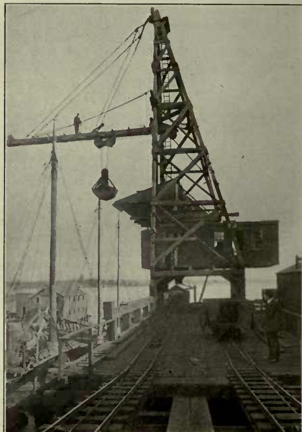
Coal Handling Tower at Power Plant
