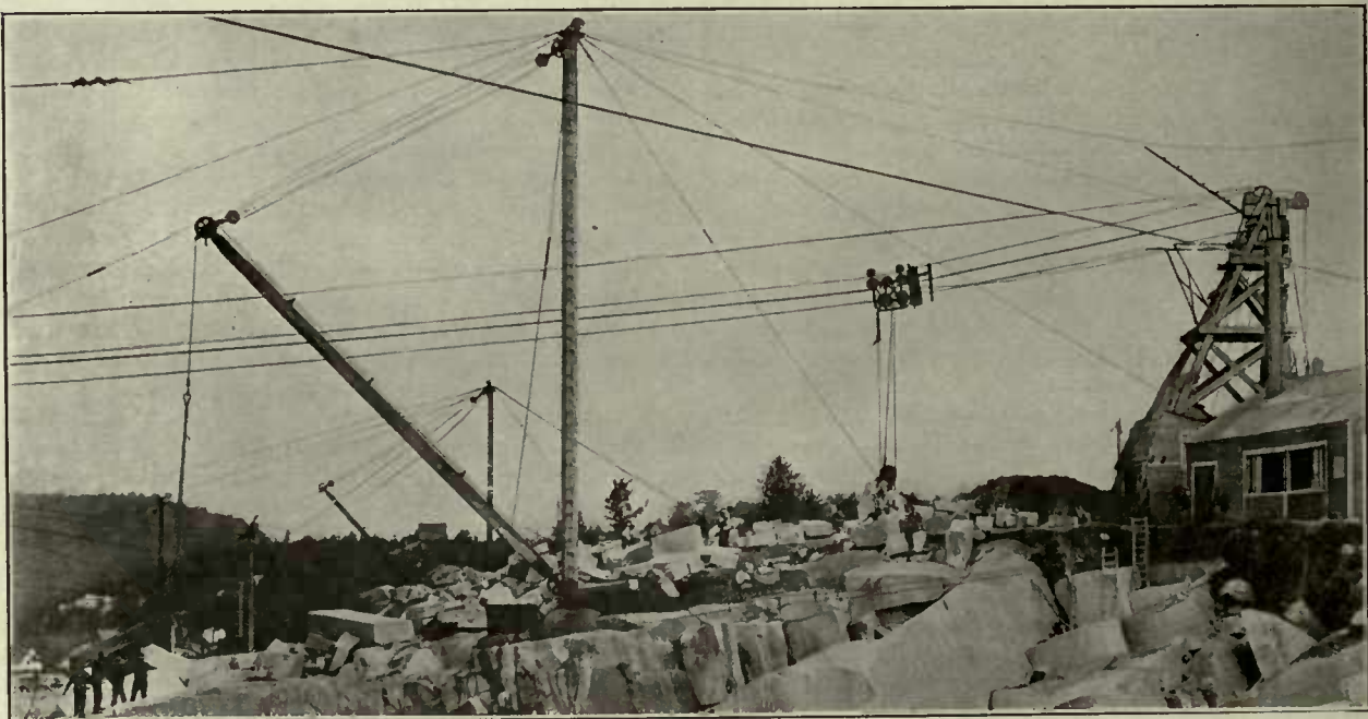
Endless-Rope Suspension Cableway Handling Block Stone in a Quarry
