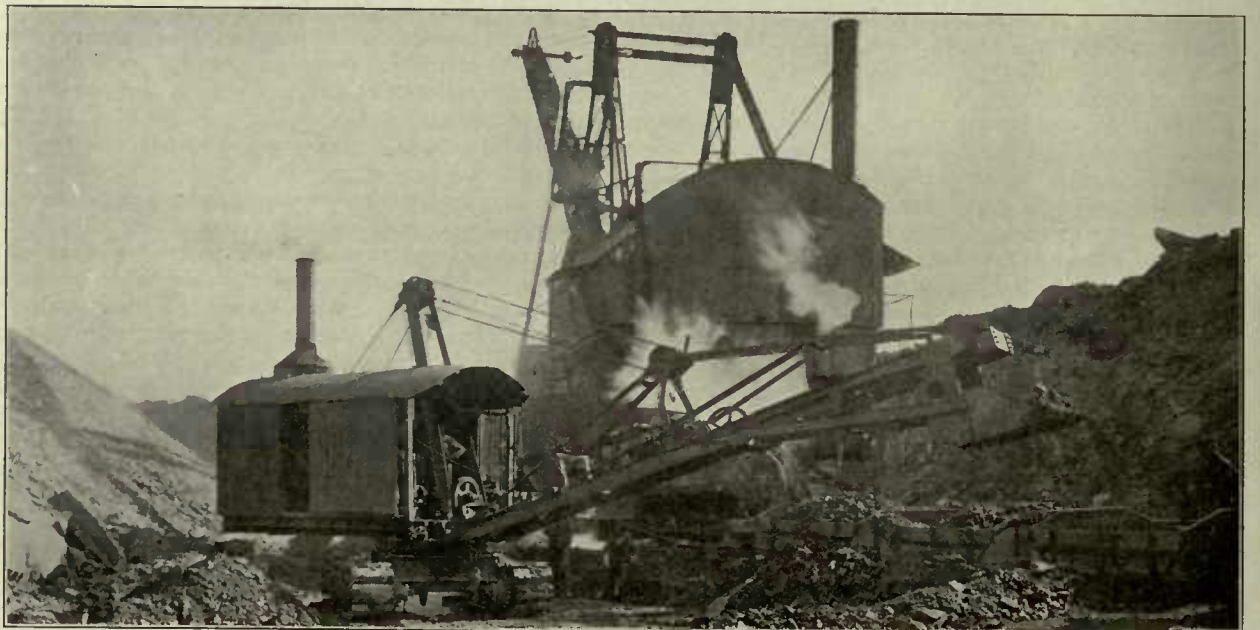
Skimmer or Coal Loader Working in Conjunction with Large Revolving Steam Power Shovel
