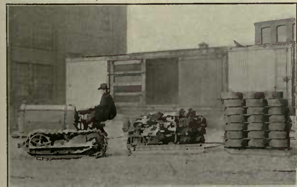
Typical Applications of Gasoline Engine Tractors
