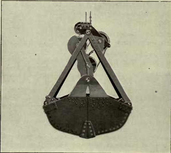
Rope Operated Power-Arm Clam-Shell Bucket for Handling Loose Materials. Two-Line Operation
