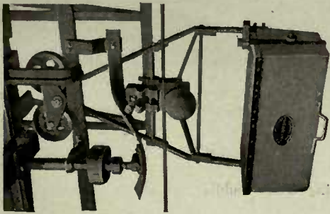
Carrier with Compression Grip Passing Through Automatic Attacher
