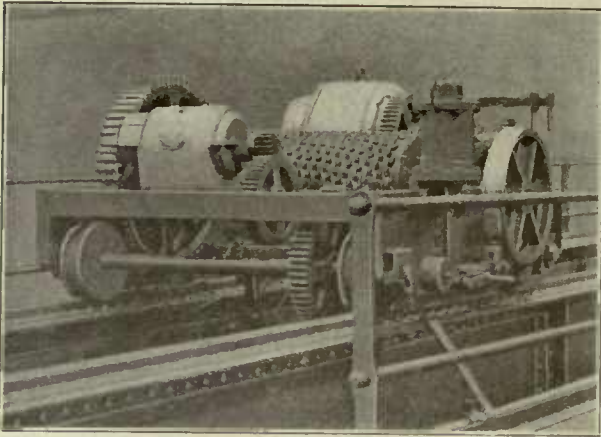
Chain Equipped Three-Motor Trolley
