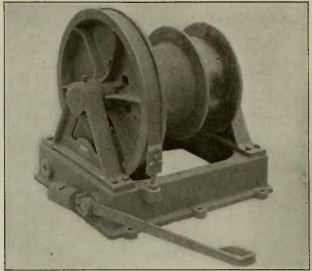
Counterweight Holding-Drum
