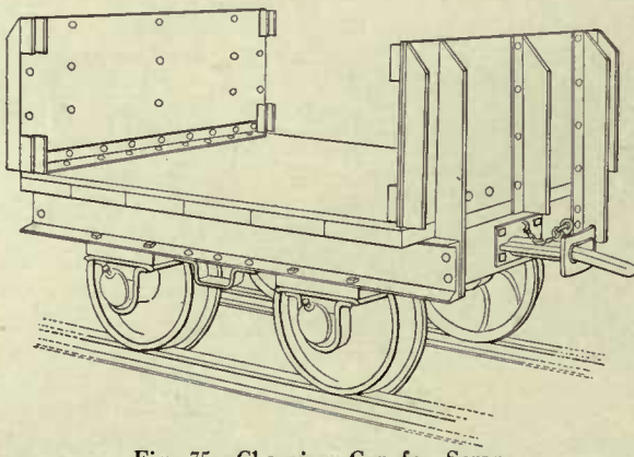
Fig. 75—Charging Car for Scrap
