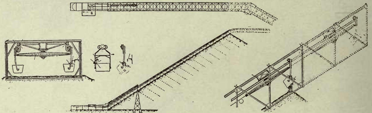
Stacking Tramway Showing Method of Extending Bridge
