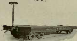
Fig. 1533. Special Double Truck Platform Car.
