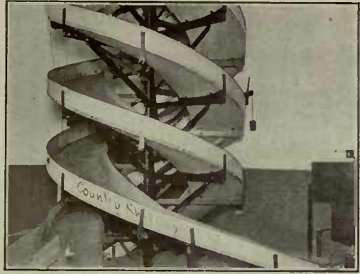
Triple Haslett Spiral for handling baskets of unpacked crockery and glassware.
