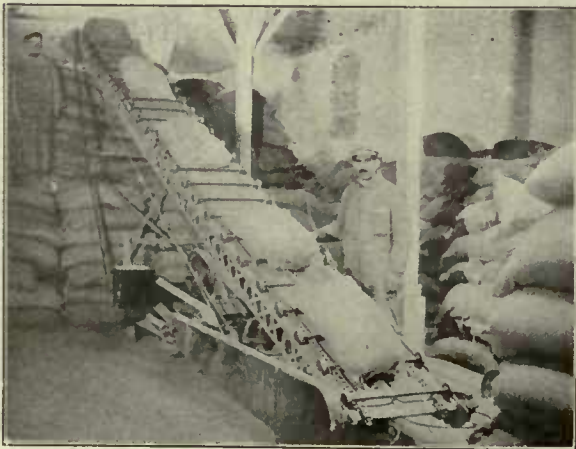
Standard Type Piler at Work in a Rice Mill.
