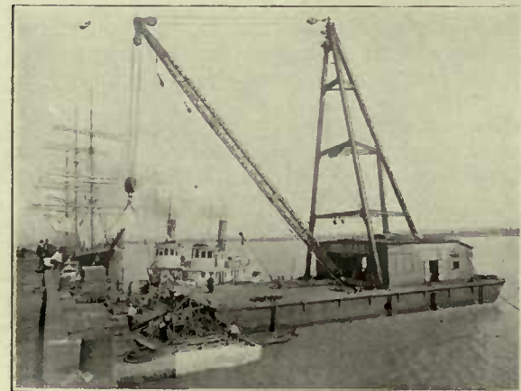
"A" Frame Barge Derricks, 5 to 150 Tons Capacity.
