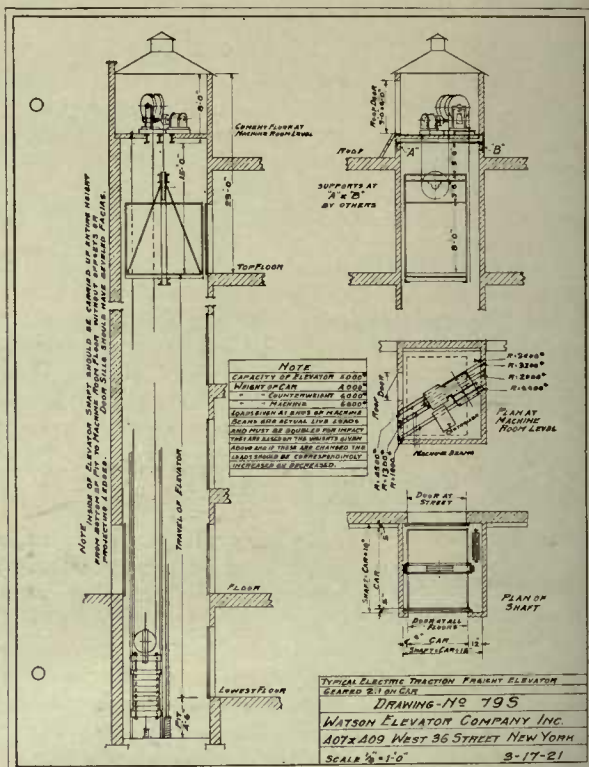
Details of Watson Freight Elevator.
