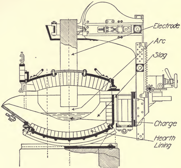
FIG. 101.—Section of a Heroult arc type electric furnace.
