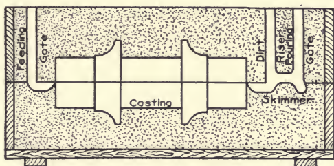
FIG. 86.—Section of a green sand mold.
