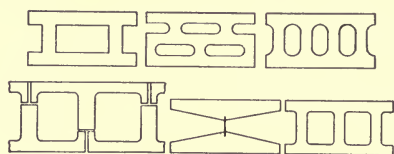
FIG. 21.—Cross sections of some concrete blocks.
