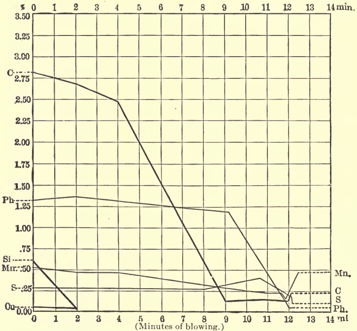
FIG. 96.—Removal of impurities in basic Bessemer process. (Bradley Stoughton.)
