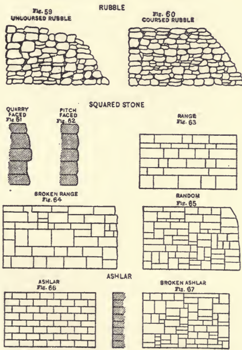
FIGS. 59-67.—Stone masonry.
