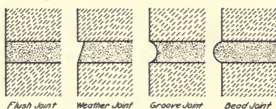
FIG. 68.—Methods of finishing horizontal joints.
