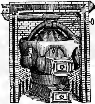
The Boynton Heater.
