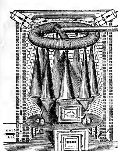
Elevation of Furnace and Section of Brick Walls.
