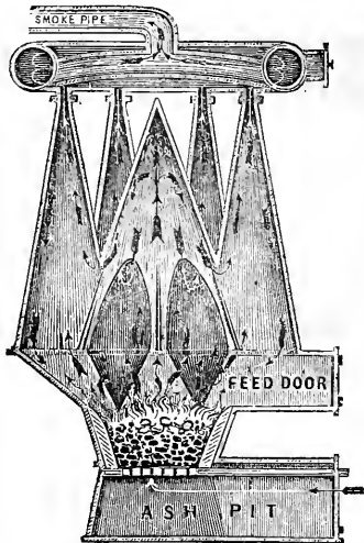
Vertical Section through the Fire Pot, Cones, and Annular Chamber, showing the action of the heat in the Cones.
