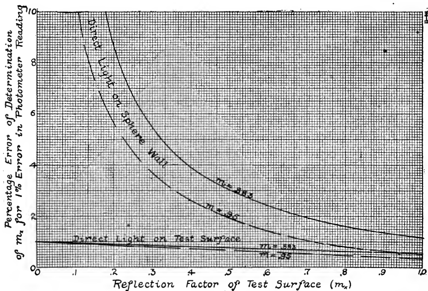
FIG. 3.—Curves showing how the precision of determinations with the new reflectometer varies with different conditions
