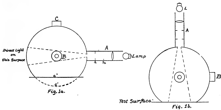
FIG. 1.—The new type "absolute" reflectometer
