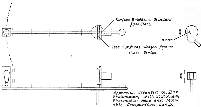
FIG. 2.—Apparatus used in determining reflection factors by measurements of surface brightness at 10^\circ intervals
