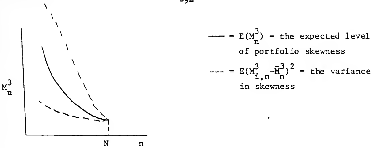
Figure 1: Diversification and its effects upon the variance about a declining mean level of portfolio skew
