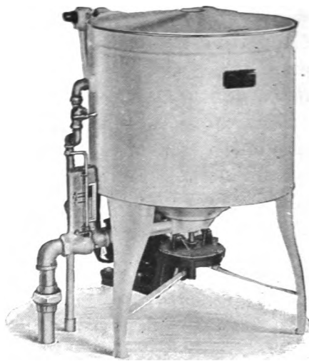
FIG. 119. Dish-washer.
