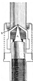
FIG. 49. Bunsen burner for gas light.
