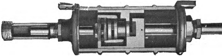
FIG. 150. Sectional view of water motor.
