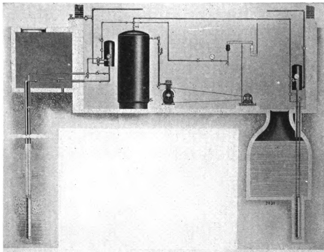
FIG. 70. Compressed-air pump system.
