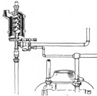
FIG. 74. Water heater and tank. FIG. 75. Booster for hot water.
