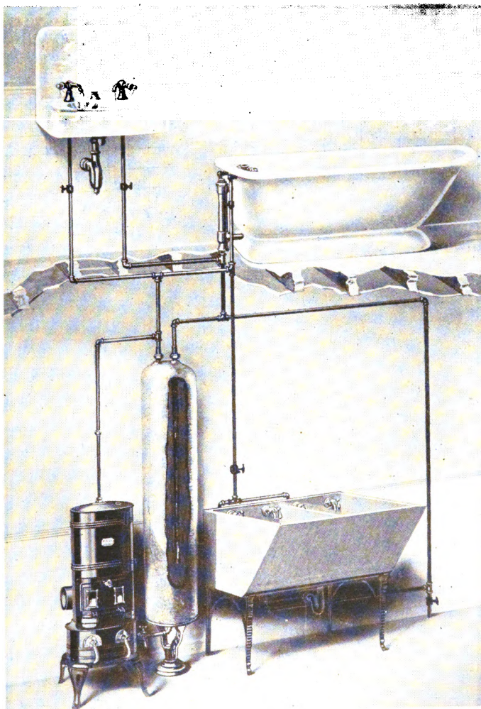
FIG. 76. Water tank and heater.
