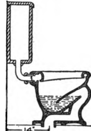
FIG. 83. Section of water closet.
