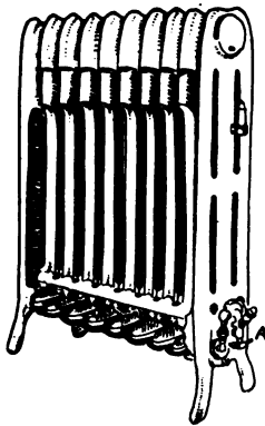
FIG. 42. Gas radiators.
