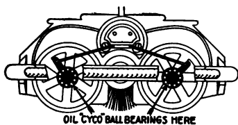
FIG. 101. Section of carpet sweeper.
