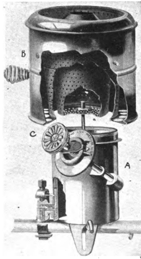
FIG. 11. Parts of oil stove burner.
