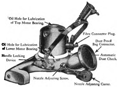
FIG. 99-a. Electric vacuum cleaner, showing parts.
