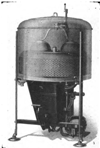
FIG. 91-a. Centrifugal washing machine.
