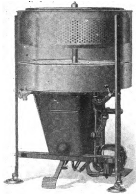
FIG. 92. Washer and dryer.
