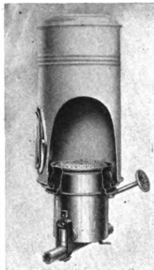
FIG. 13. Burner for oil stove.
