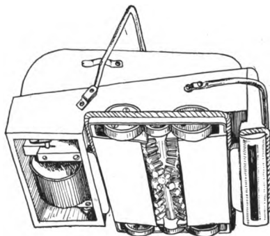
FIG. 98. Brush and vacuum cleaner combined.
