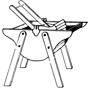
FIG. 90. Oscillating washing machine.
