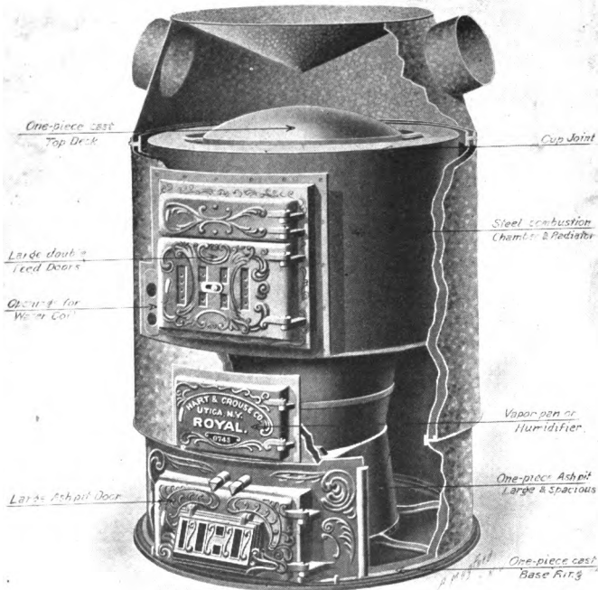
FIG. 26. Warm-air furnace.
