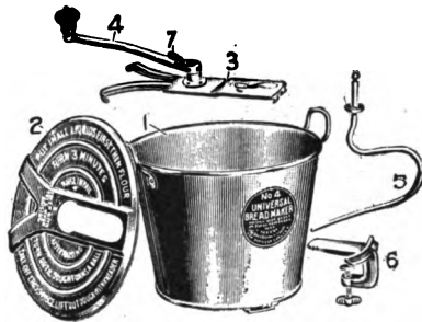
FIG. 115. Parts of bread mixer.
