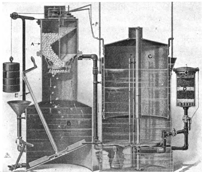
FIG. 156. Acetylene gas plant.
