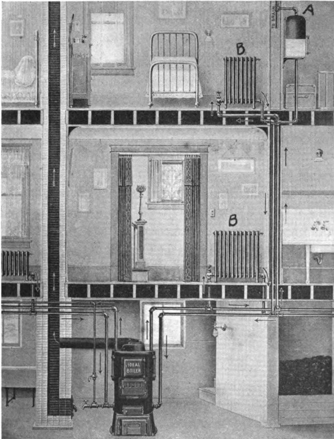
FIG. 31. Hot-water heating system.
