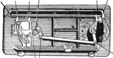
FIG. 133. Under part of machine using a vibrating shuttle.
