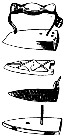
FIG. 95. Parts of electric iron.
