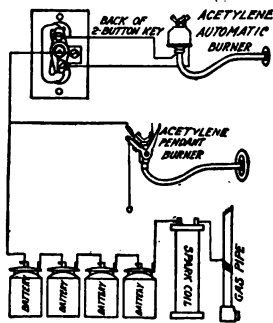
FIG. 50-a. Showing electric lighting device for acetylene burner.
