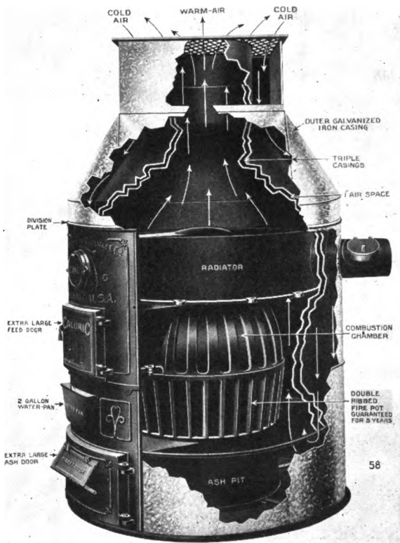
FIG. 28. Pipeless furnace.
