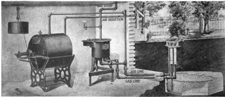
FIG. 155. Gasoline gas plant.
