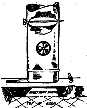
FIG. 2. Drafts and dampers in stove-pipe.
