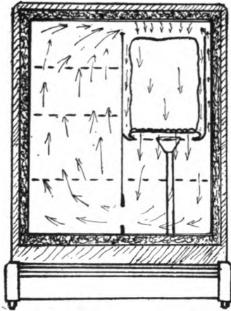
FIG. 57. Diagram showing circulation in a refrigerator.
