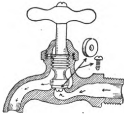
FIG. 77. Faucet showing parts.
