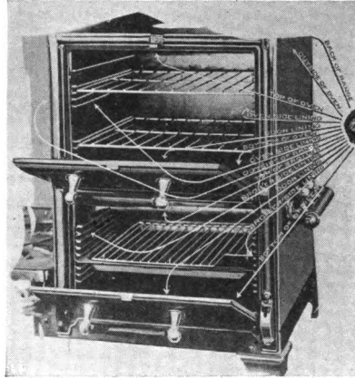
FIG. 7. Gas ovens.
