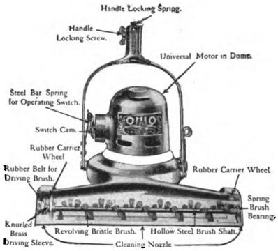
FIG. 99-a. Electric vacuum cleaner, showing parts.
