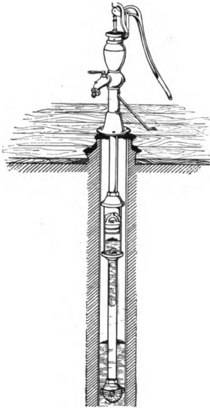
FIG. 68. Suction pump.
