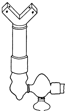
FIG. 50. Open-flame acetylene burner.
