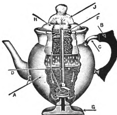
FIG. 118. Percolator.
