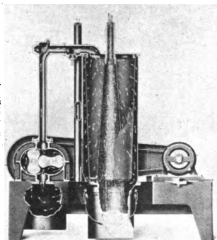
FIG. 100. Stationary vacuum cleaner.
