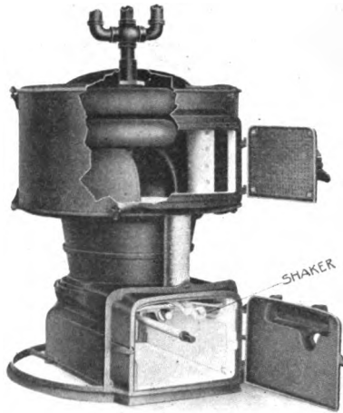
FIG. 30. Garland furnace with hot-water boiler.
