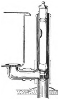
FIG. 79. Cross-section of overflow on bath-tub.
