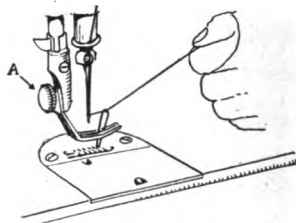
FIG. 137. Pulling up bobbin thread.
