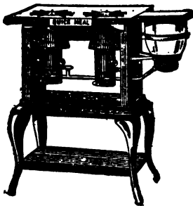
FIG. 11-b. Oil stove without oven.
