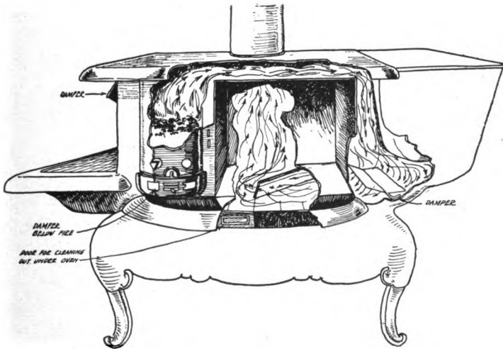
FIG. 1. Cross-section of cooking stove.
