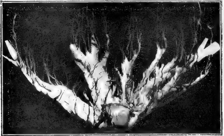
FIG. 42.—An osmotic madre-pore
