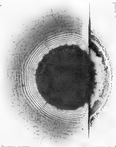
FIG. 13. —Waves of diffusion refracted at a plane surface on passing from a less concentrated into a more concentrated solution. The refracted wave-front is flattened, the wave length being less in the denser medium.
