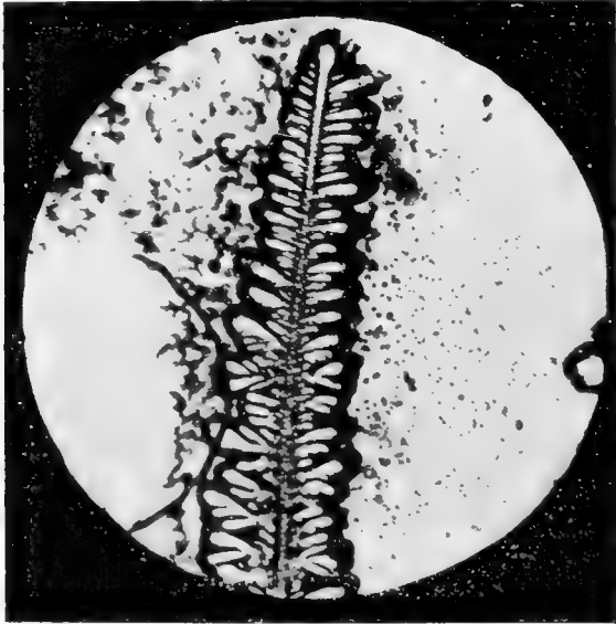
FIG. 30.—Form produced by the crystallization of chloride of ammonium in a colloidal solution.
