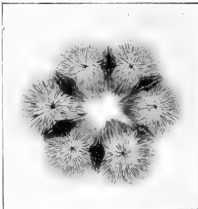
FIG. 5.—Liquid figures of diffusion.
