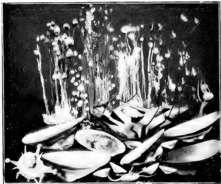
FIG. 61.—A group of osmotic forms.
