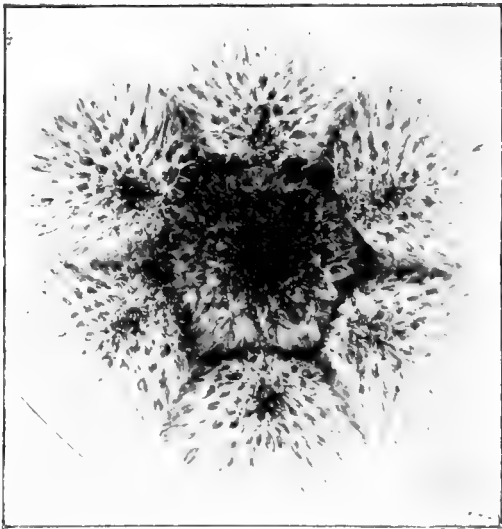
FIG. 21.—The same drops 15 minutes later, showing the granulation appearance.
