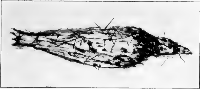
FIG. 52. Amoeboid osmotic growth with long crystalline cilia swimming about in the mother liquor.
