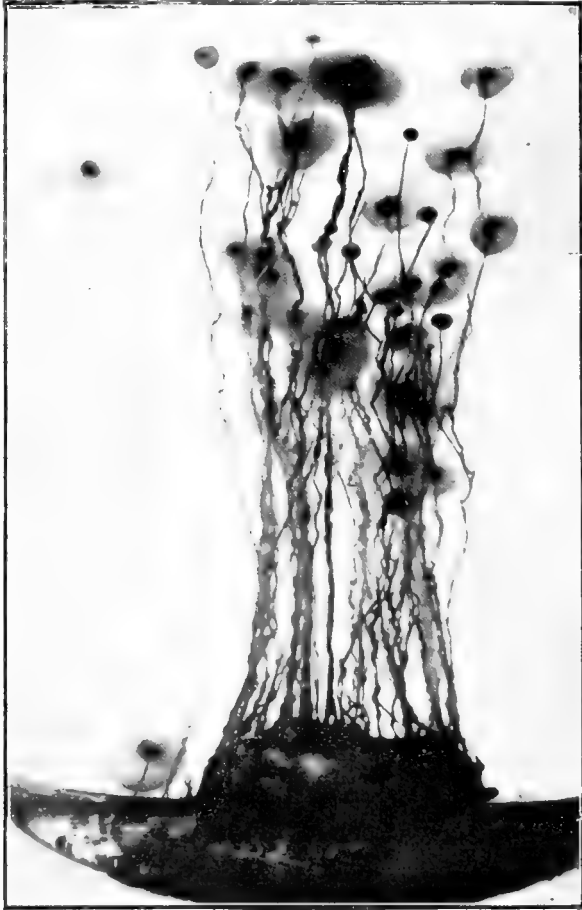
FIG. 30. — An osmotic growth photographed by transverse light to show the construction of the terminal organs.
