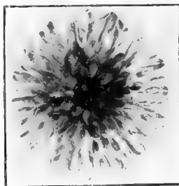
FIG. 19. Uniform cohesion figure formed by a drop of Indian ink in a solution of salt.
