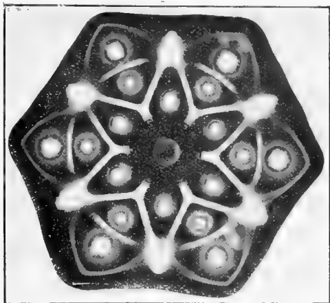
FIG. 7. Pattern produced in gelatine by the diffusion of drops of silver nitrate and sodium carbonate.
