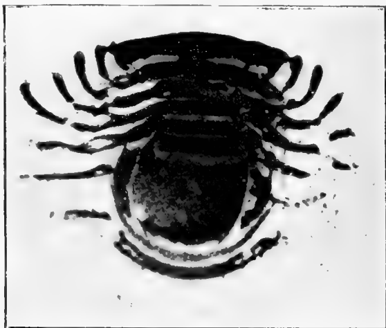
FIG. 18.—Articulate form produced by periodic precipitation.
