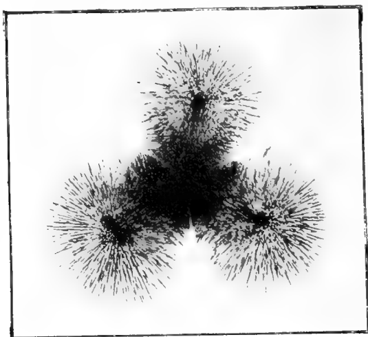
FIG. 34.—A triaster produced by diffusion.
