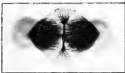
FIG. 33.—Equatorial crown produced by diffusion.
