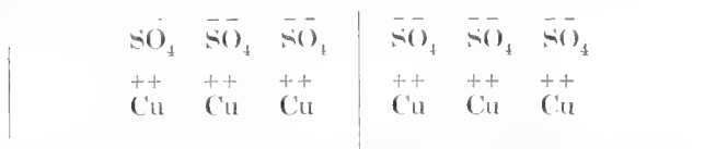
FIG. 1. Before the passage of the current.
