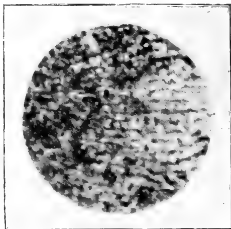
FIG. 58.—Photomicrograph of an osmotic leaf showing the cellular structure.
