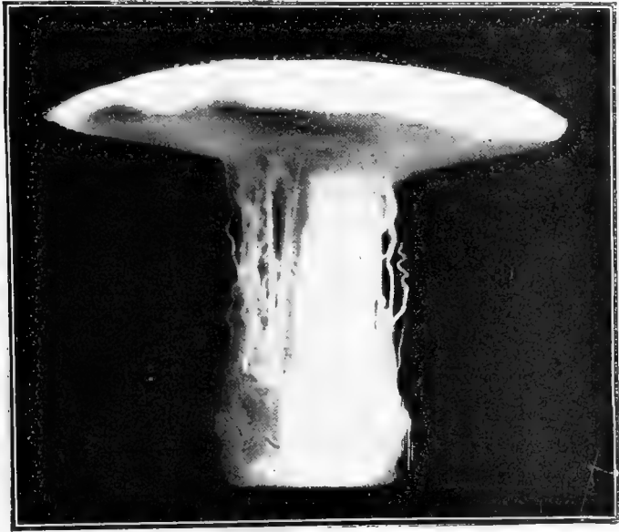
FIG. 43.—An osmotic mushroom form.
