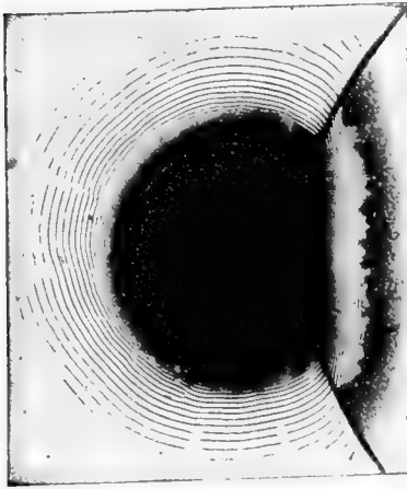
FIG. 14.—Transformation of a spherical wave-front into a plane wave-front by a convergent dipter.
