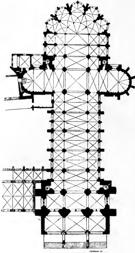
NOYON CATHEDRAL, from V. le-Duc
