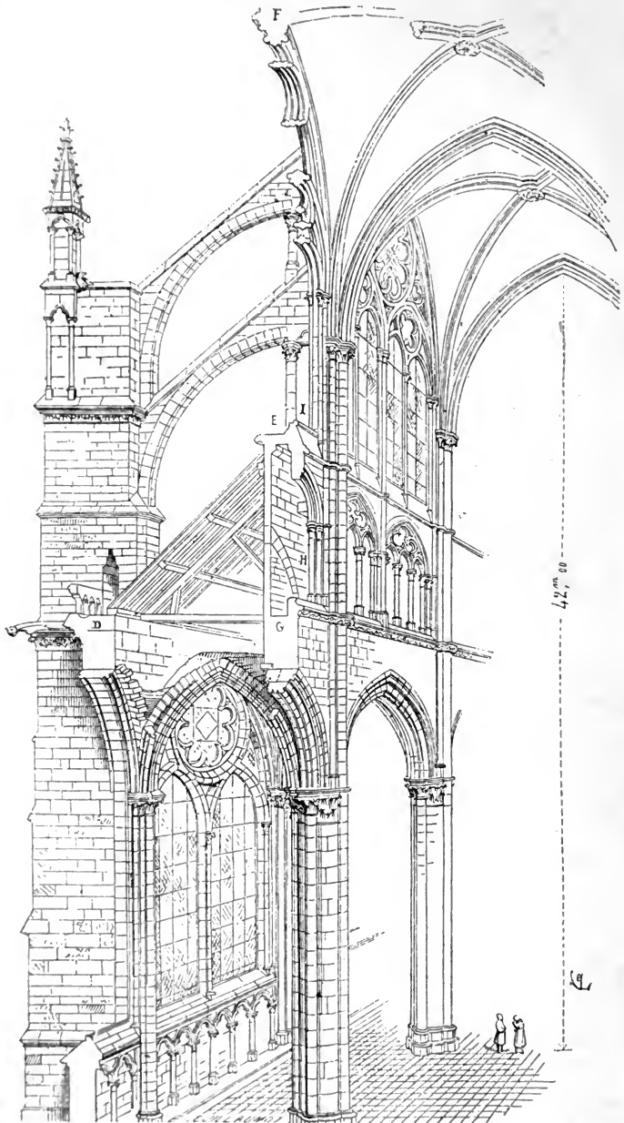
AMIENS—SECTION OF NAVE
