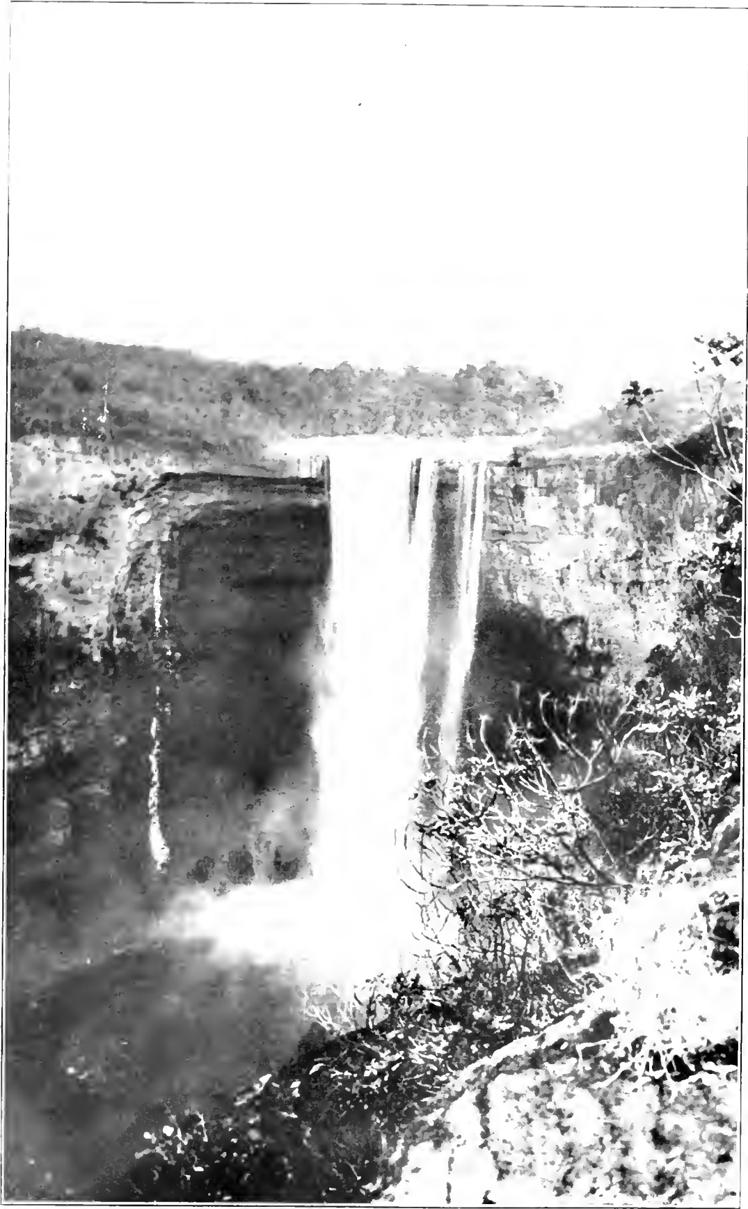
THE KAIBAB FALLS. Height 741 feet.
