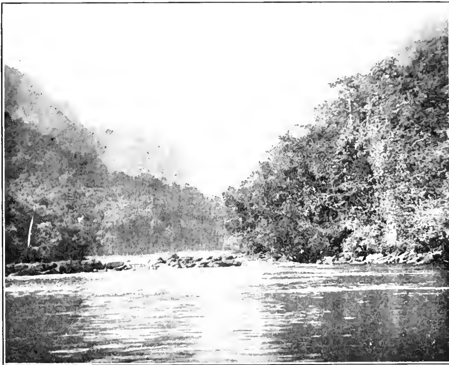
FIG. 17. View on the Potaro River looking up stream at the point where the first glimpse of the Kaieteur Falls is caught.
