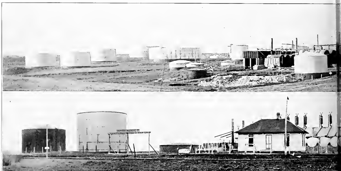
UPPER VIEW—REFINERY OF PONCA REFINING CO., PONCA CITY, OKLA. Capacity 4,500 Barrels per Day Offices 403 Colcord Building, Oklahoma City, Okla.
