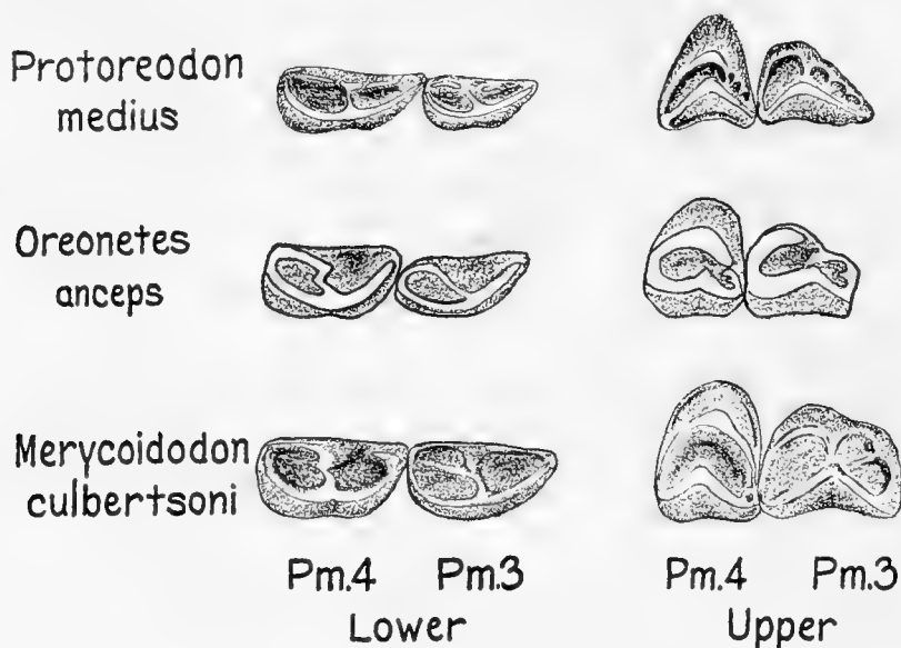
FIG. 3.—Third and fourth premolars of Protoreodon , Oreonetes , and Merycoidodon . (After Loomis, 1924.)
