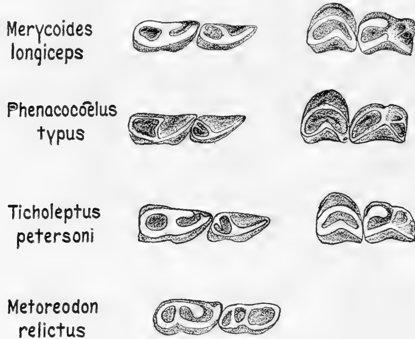
FIG. 5.—Third and fourth inferior and superior premolars of Merycoïdes , Phenacocoëlus , Ticholeptus , and Metoreodon . (After Loomis, 1924.)
