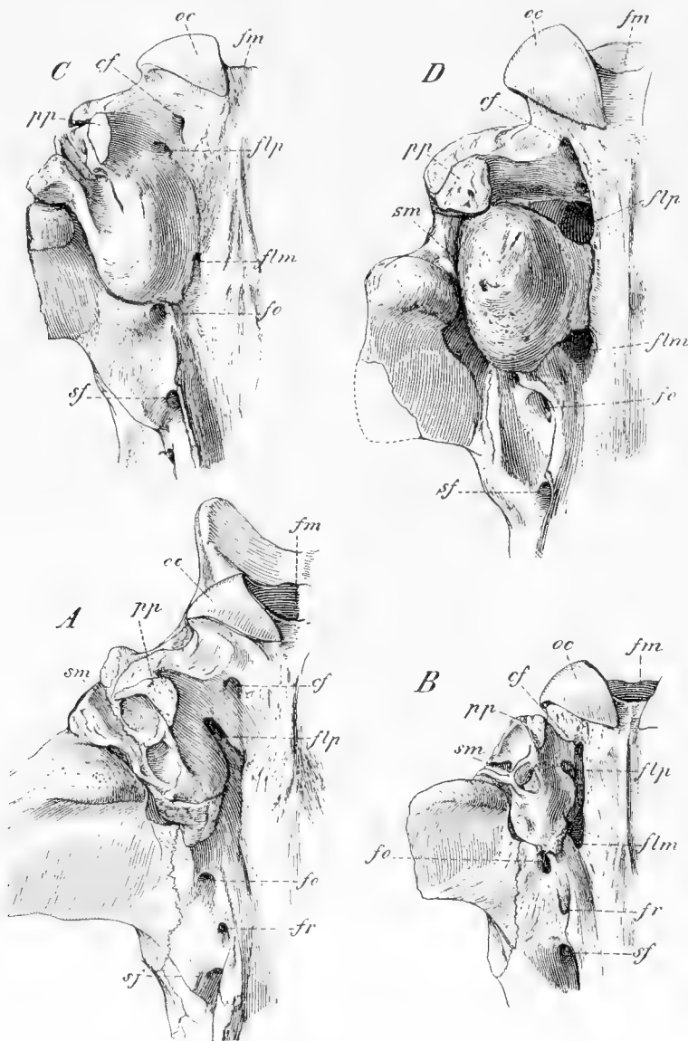
FIG. 7.—Evolution of the basioccipital region in merycoidodonts. A. Merycoidodon culbertsonii , Cat. No. 595. B. Merycoidodon gracilis , Cat. No. 596. C. Eporeodon bullatus , Cat. No. 611. D. Eporeodon major , Cat. No. 1038. All specimens in A.M.N.H. cf , condylar (hypoglossal) foramen; flm , foramen lacerum medium; flp , foramen lacerum posterius; fm , foramen magnum; fr , foramen rotundum; oc , occipital condyle; pp , paroccipital (paramastoid) process; sf , foramen lacerum anterius (sphenoidal fissure); sm , stylomastoid foramen. (After Osborn and Wortman, 1894.)
