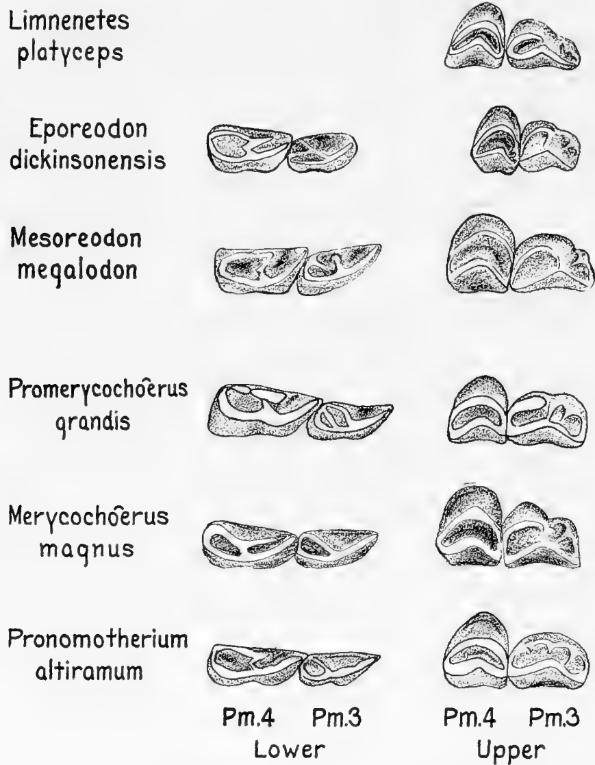
FIG. 4.—Third and fourth premolars of Limnenetes , Eporeodon , Mesoreodon , Promerycochærus , Merycochærus , and Pronomotherium . (After Loomis, 1924.)
