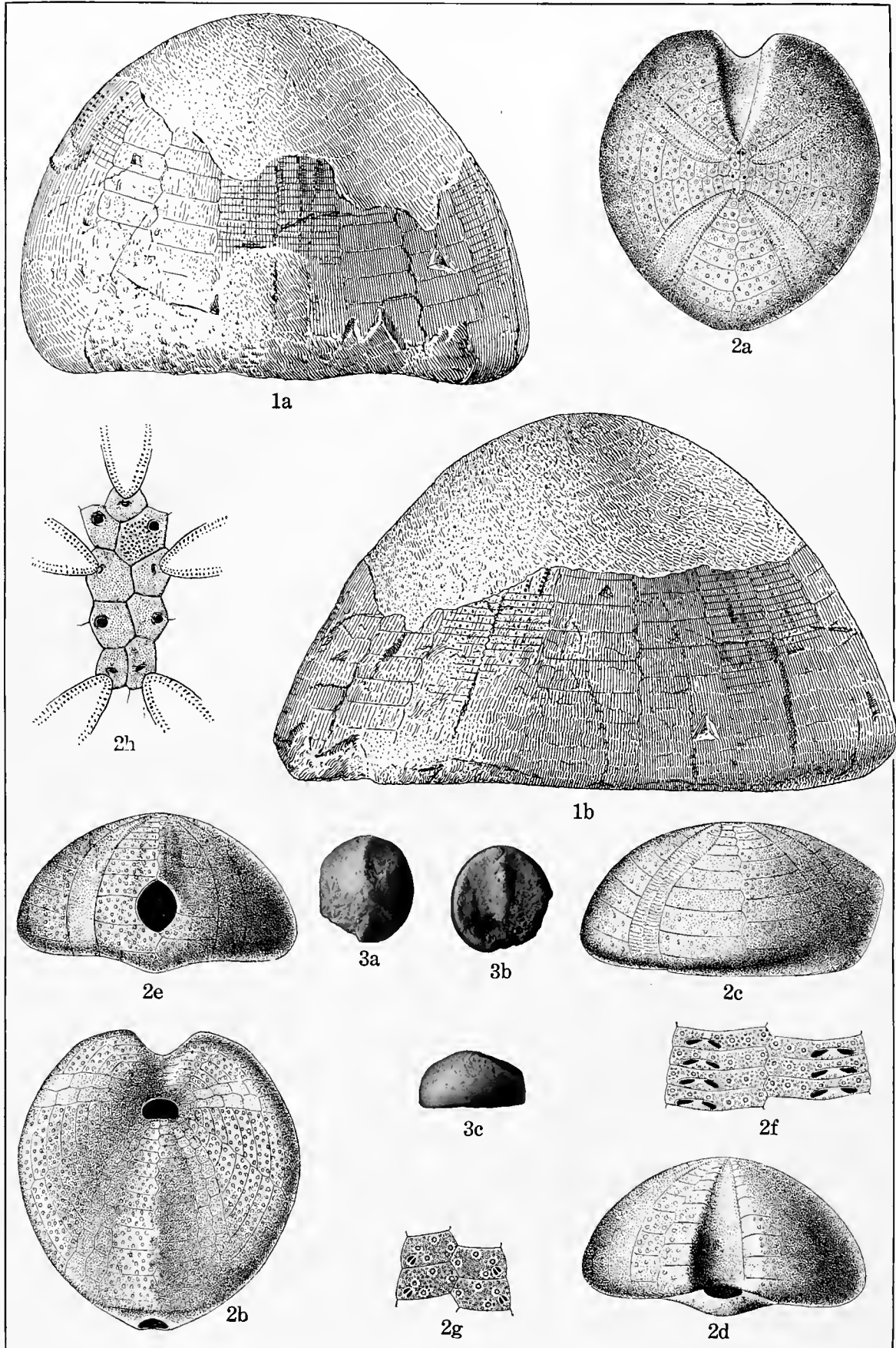
CRETACEOUS ECHINOIDEA.
