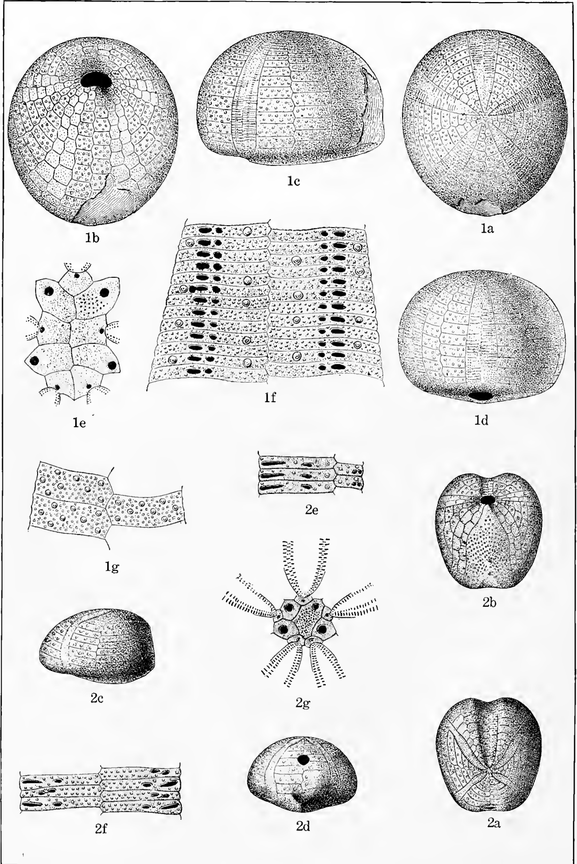
CRETACEOUS ECHINOIDEA.
