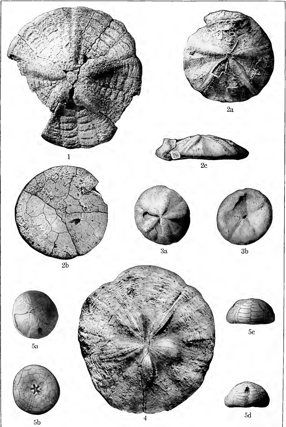
MIOCENE ECHINOIDEA.
