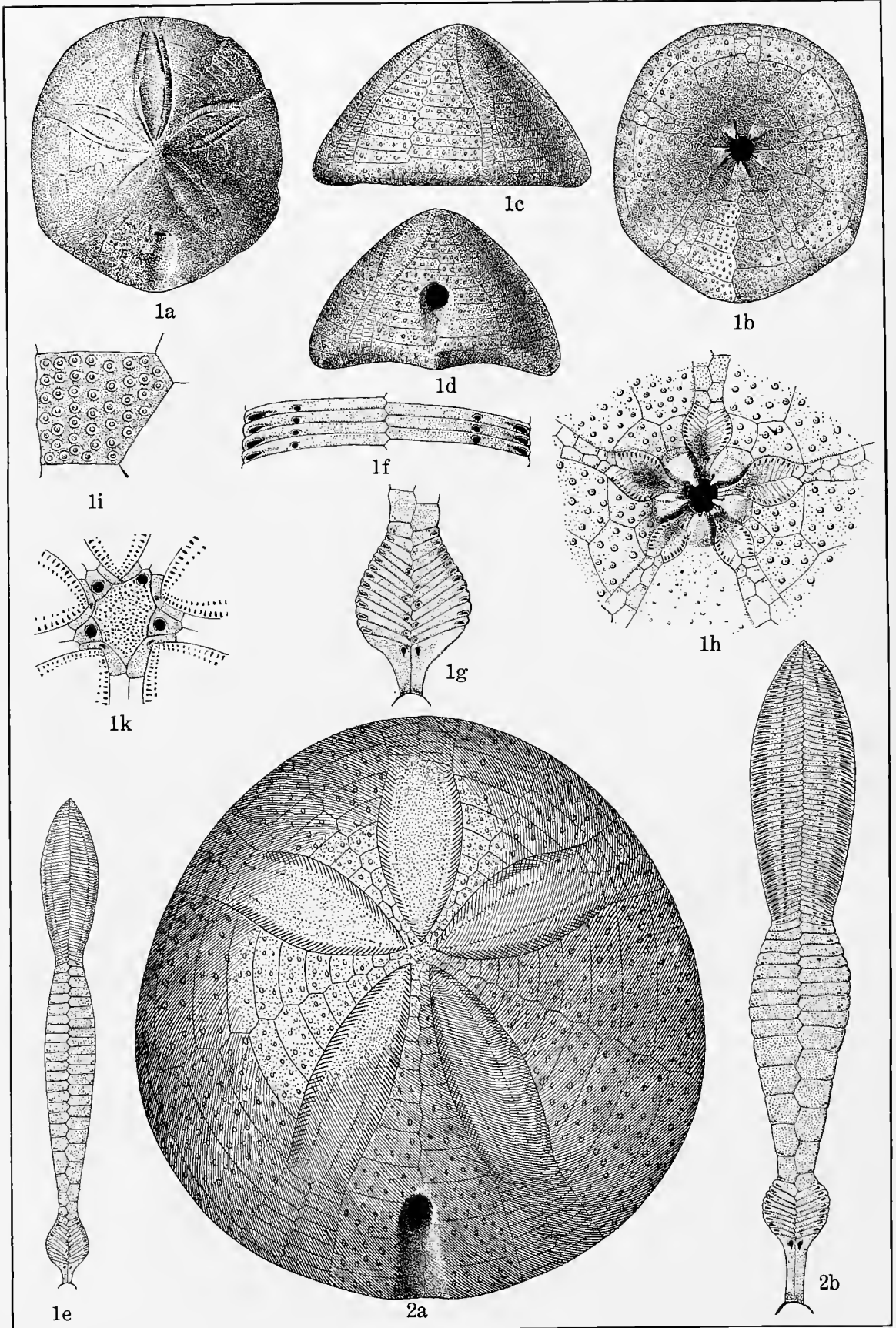
CRETACEOUS ECHINOIDEA.
