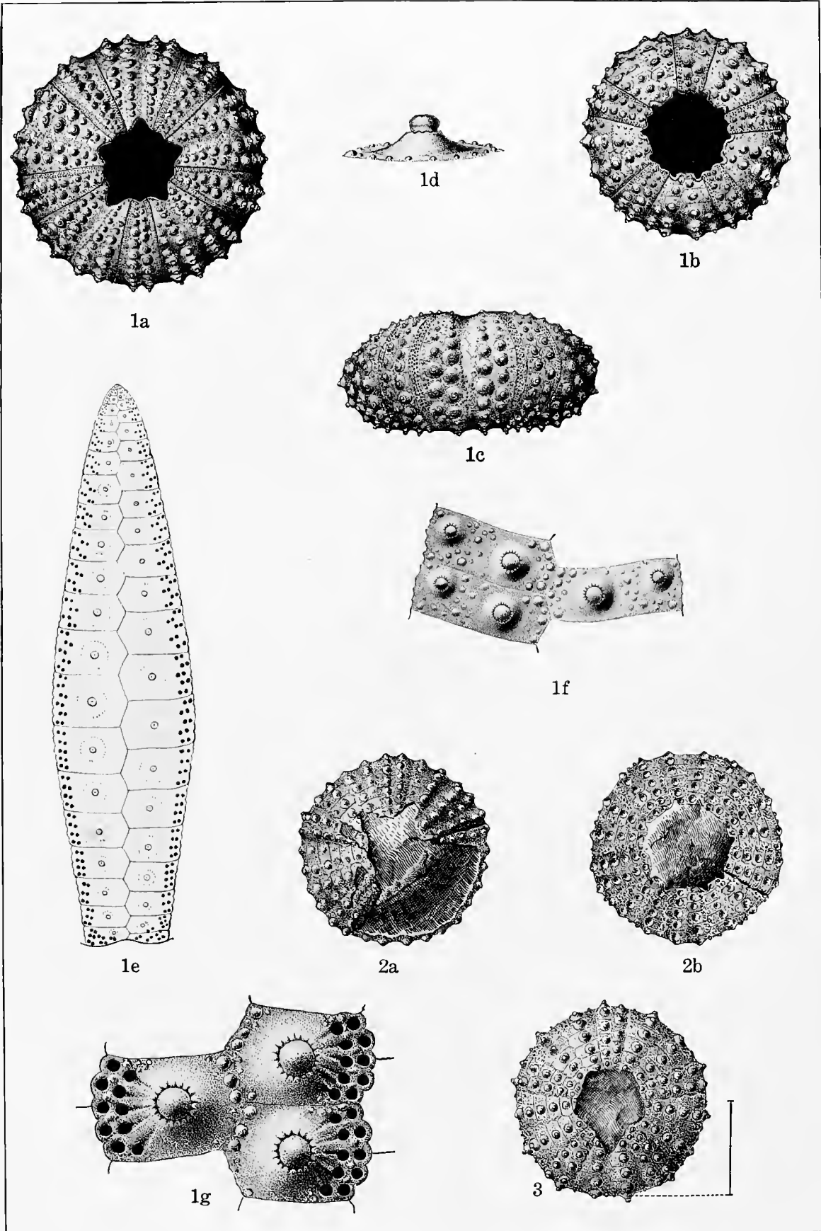
CRETACEOUS ECHINOIDEA.
