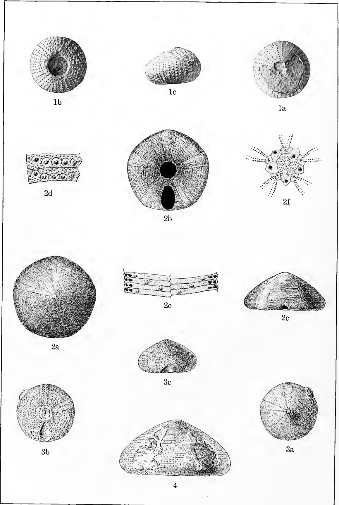
CRETACEOUS ECHINOIDEA.
