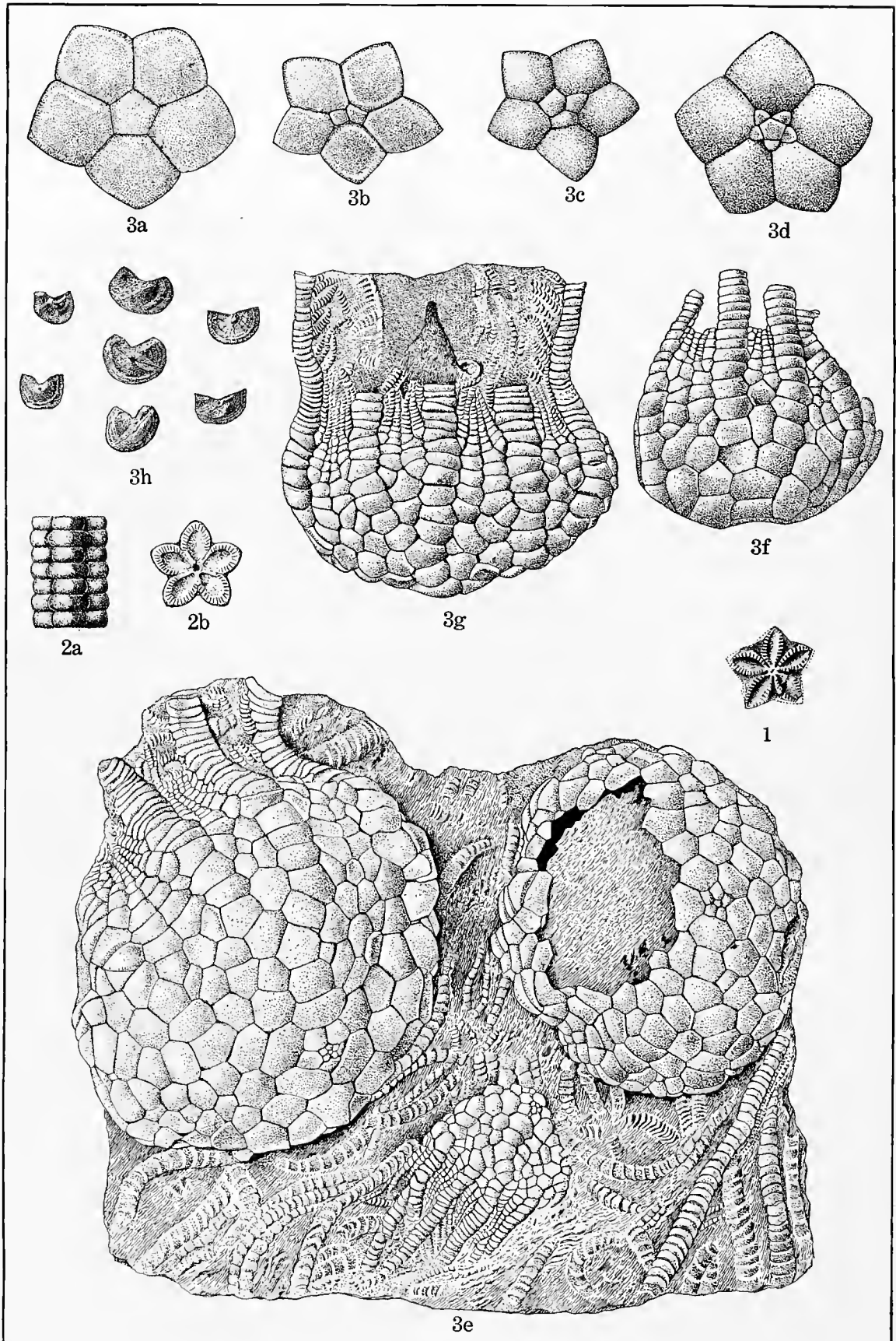
CRETACEOUS CRINOIDEA.
