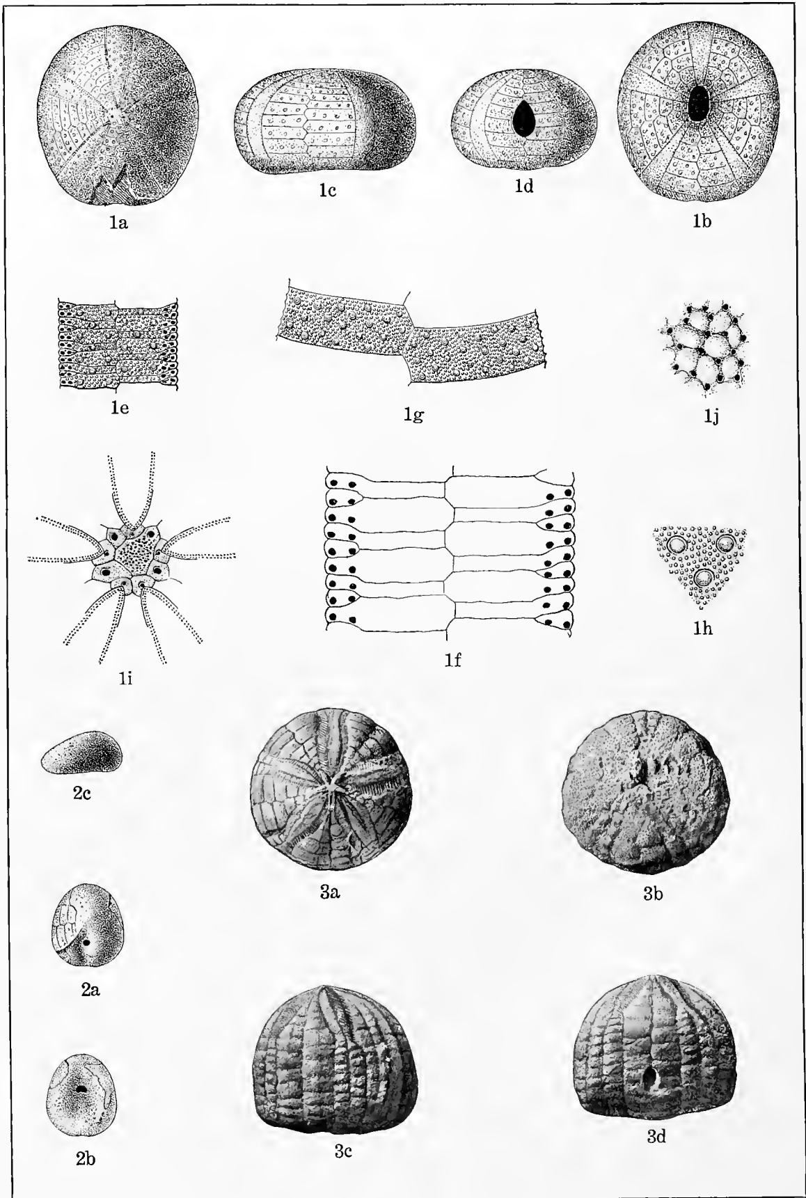
CRETACEOUS ECHINOIDEA.
