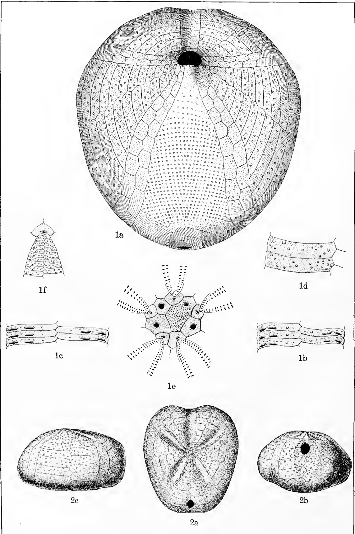
CRETACEOUS ECHINOIDEA.
