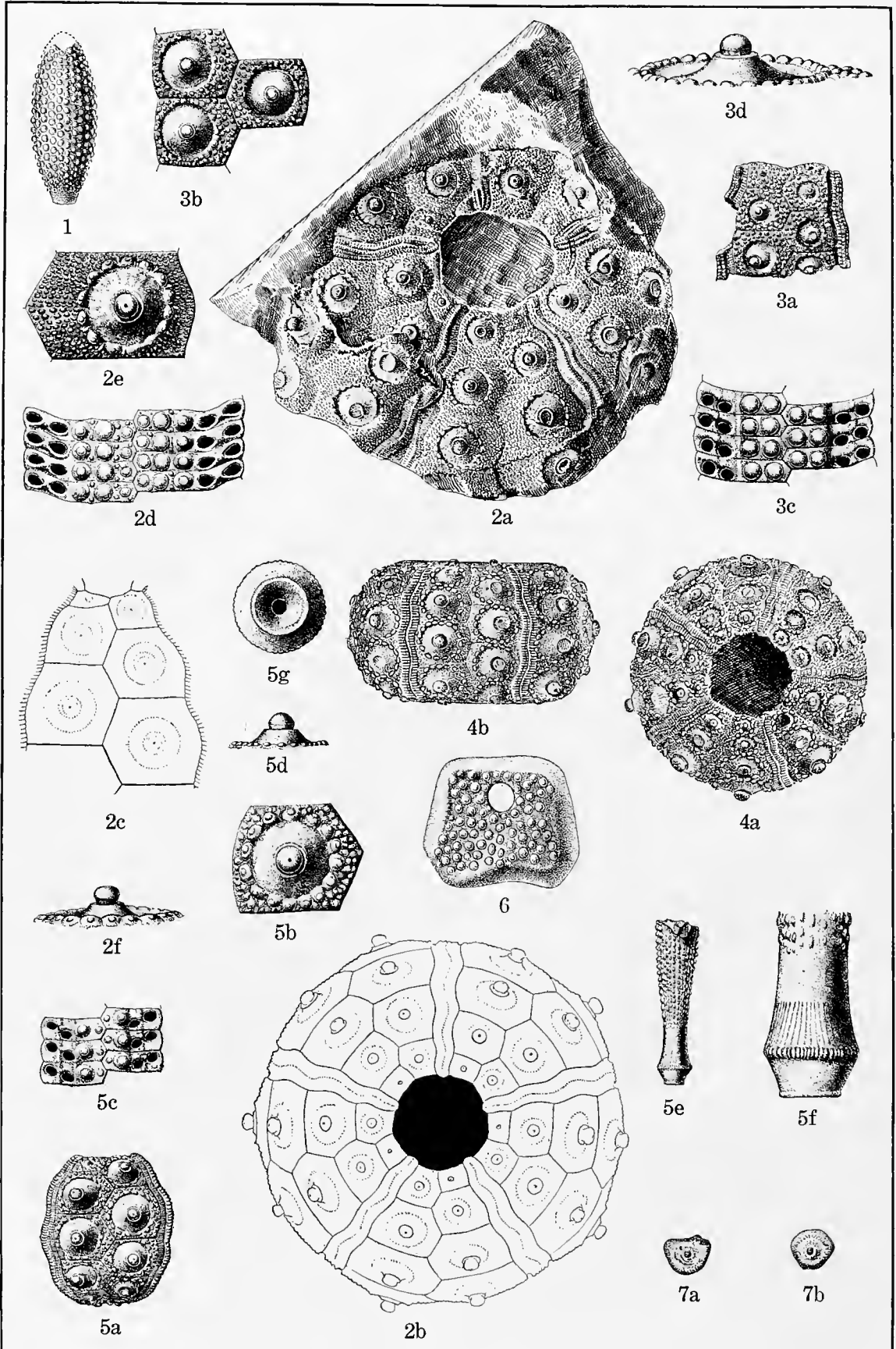
CRETACEOUS ECHINOIDEA.
