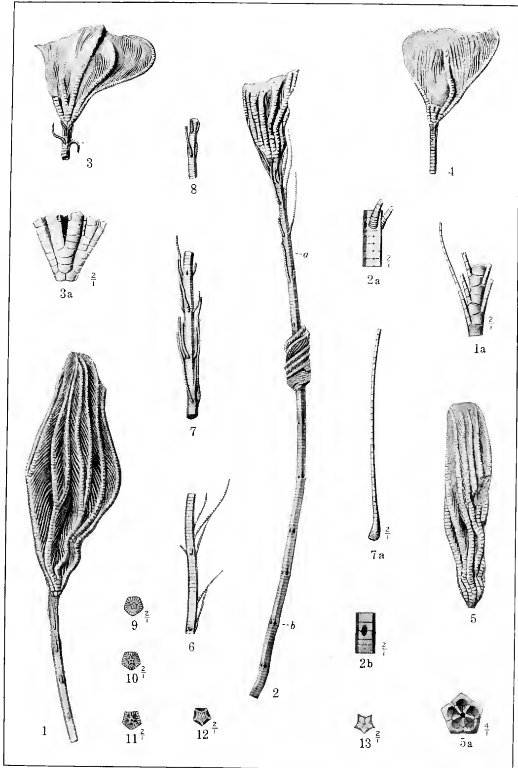
JURASSIC CRINOIDEA.
