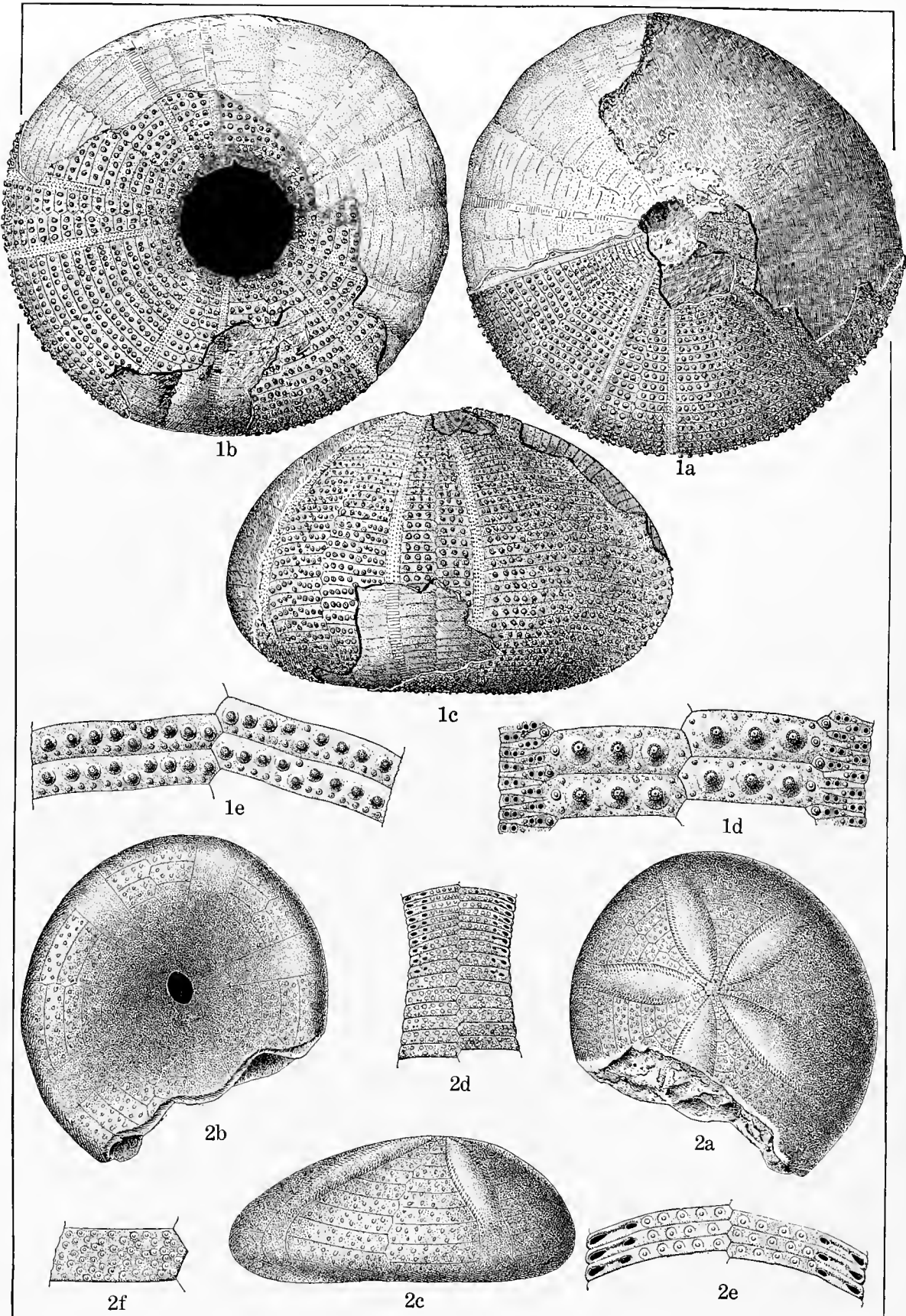
CRETACEOUS ECHINOIDEA.
