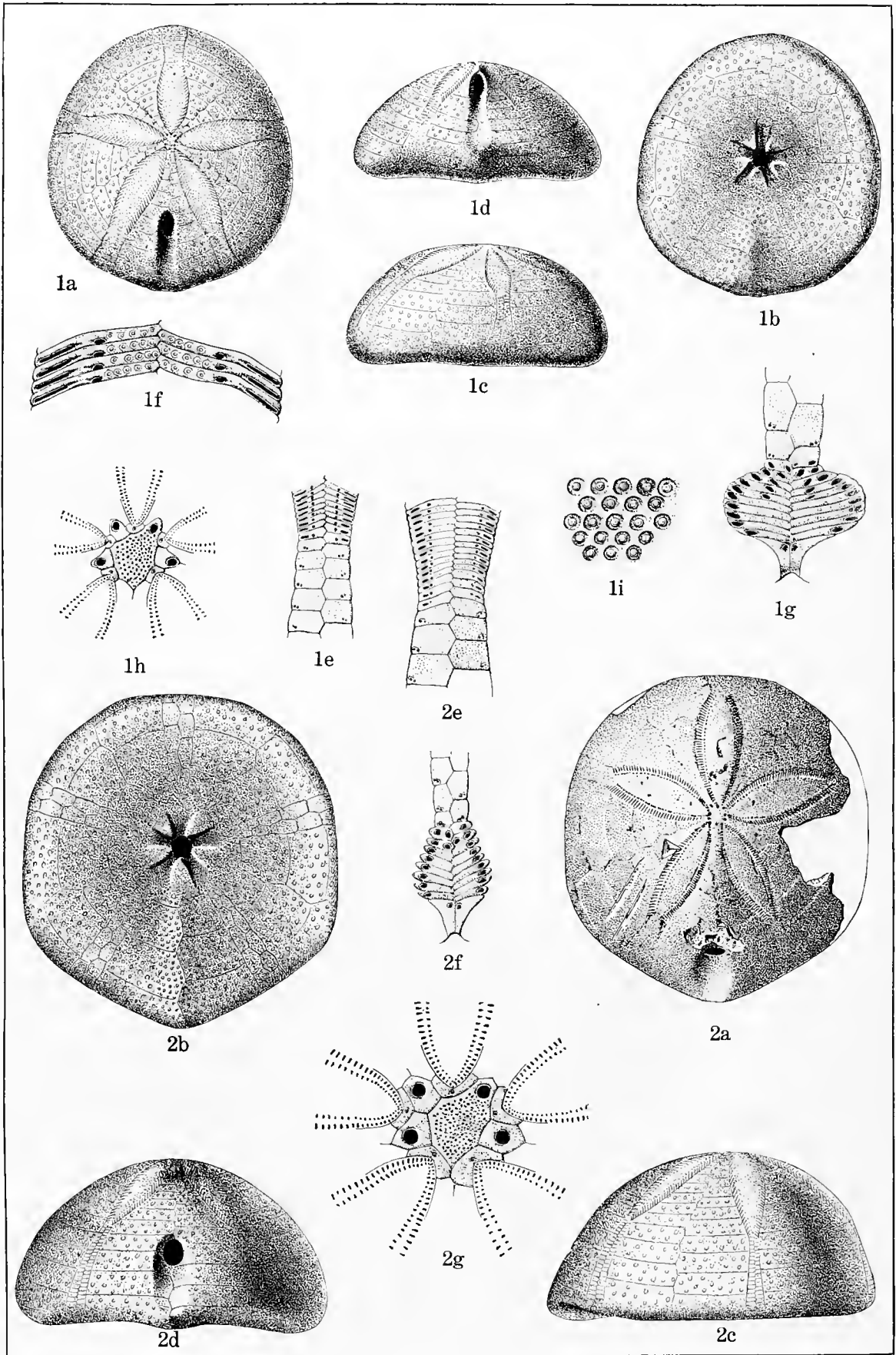
CRETACEOUS ECHINOIDEA.
