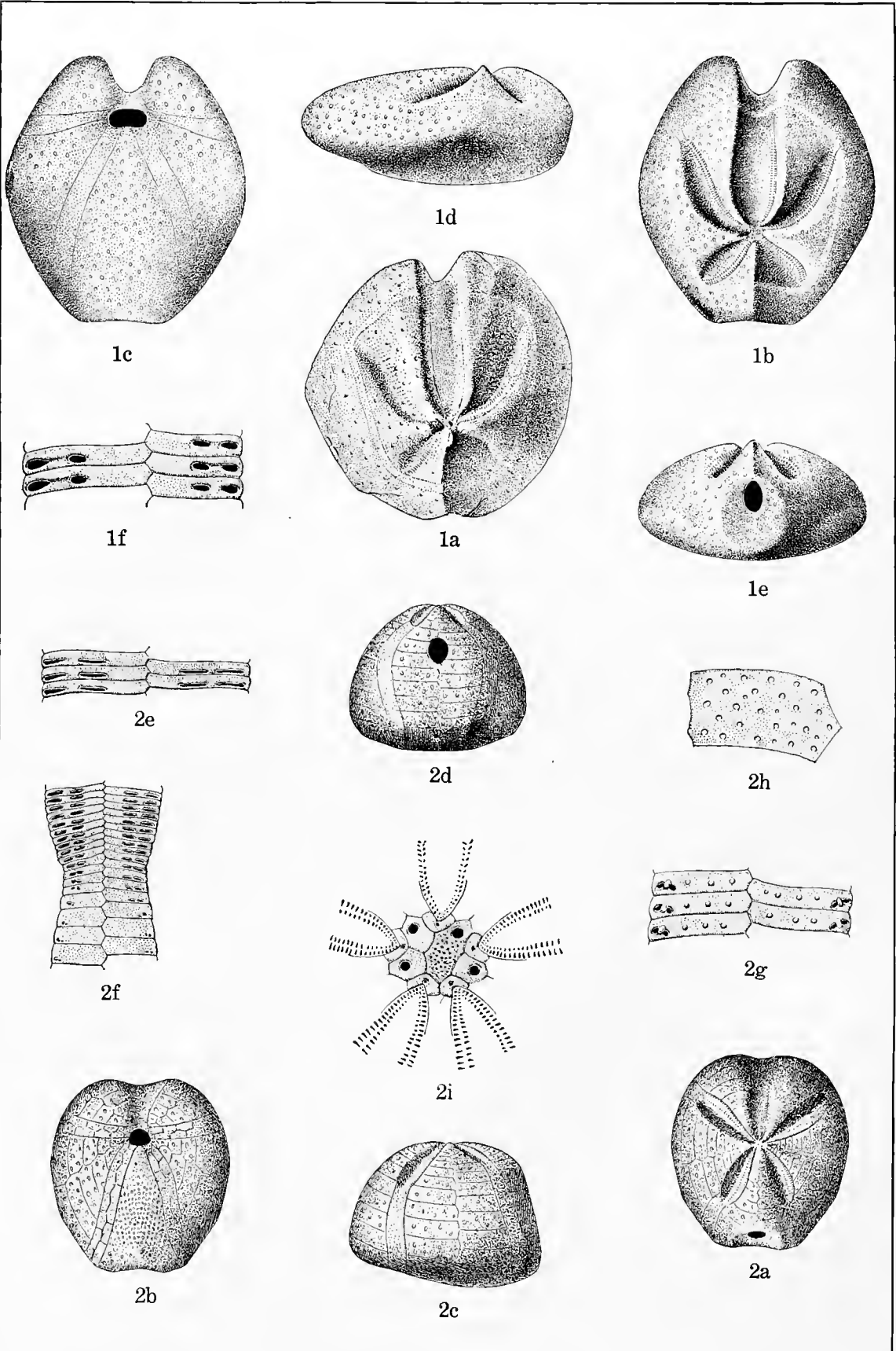
CRETACEOUS ECHINOIDEA.
