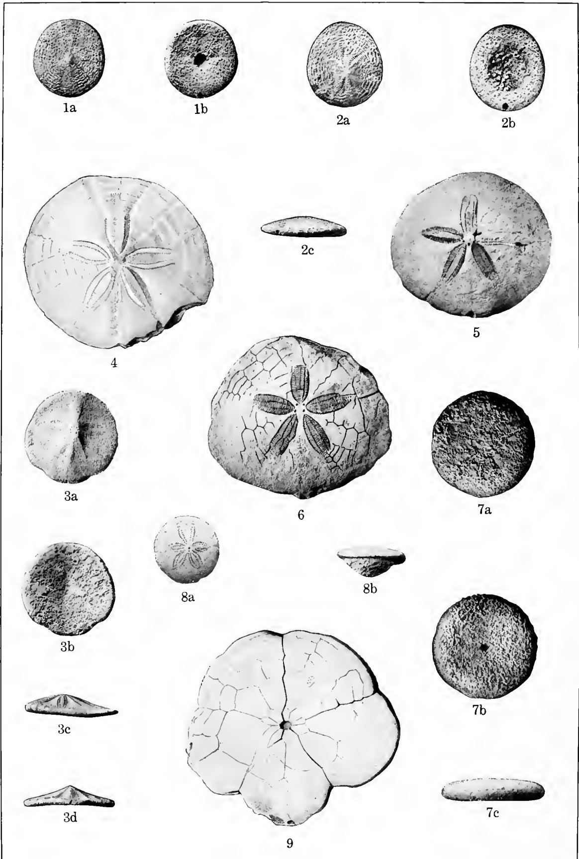
MIOCENE ECHINOIDEA.
