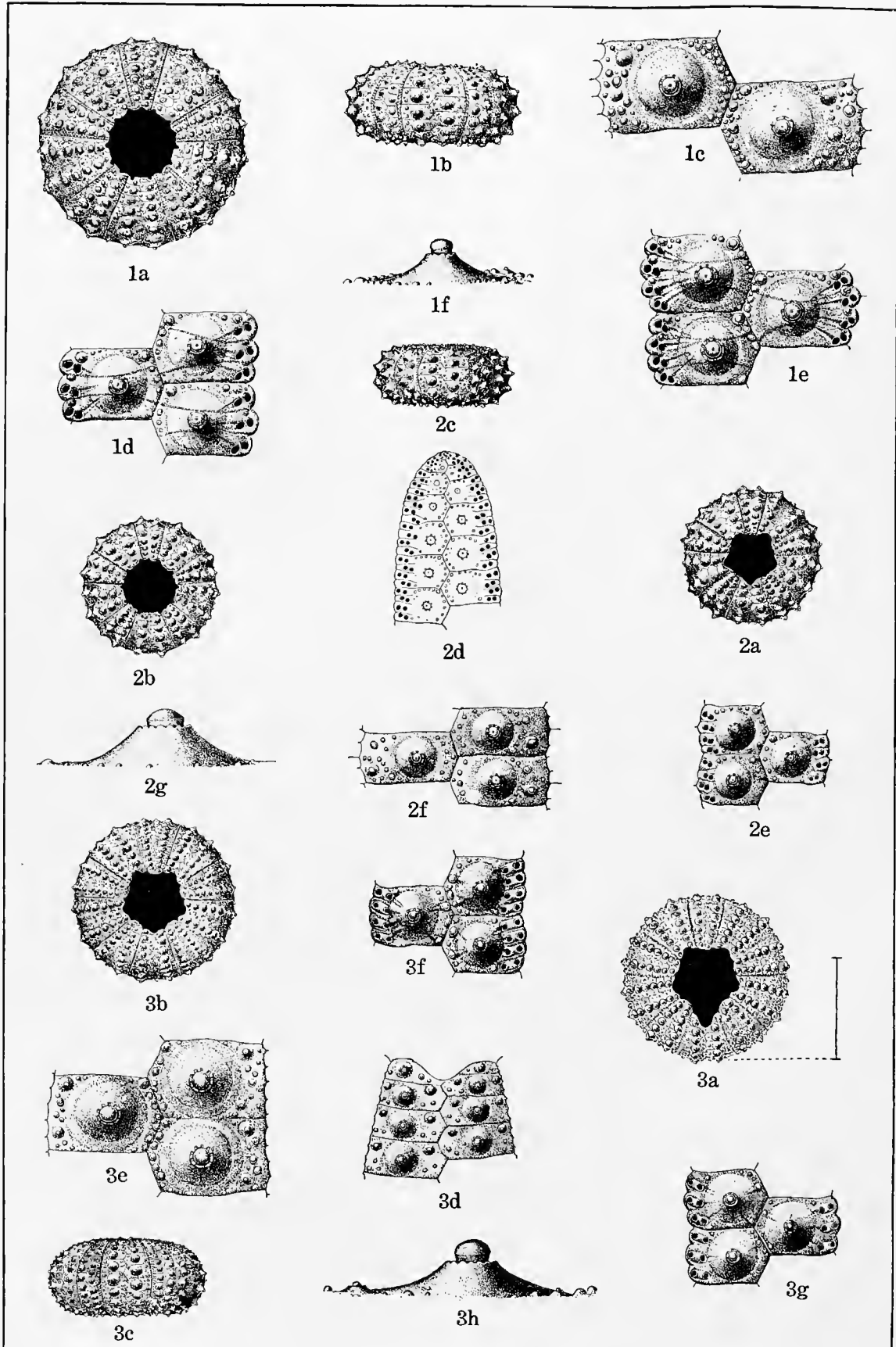
CRETACEOUS ECHINOIDEA.
