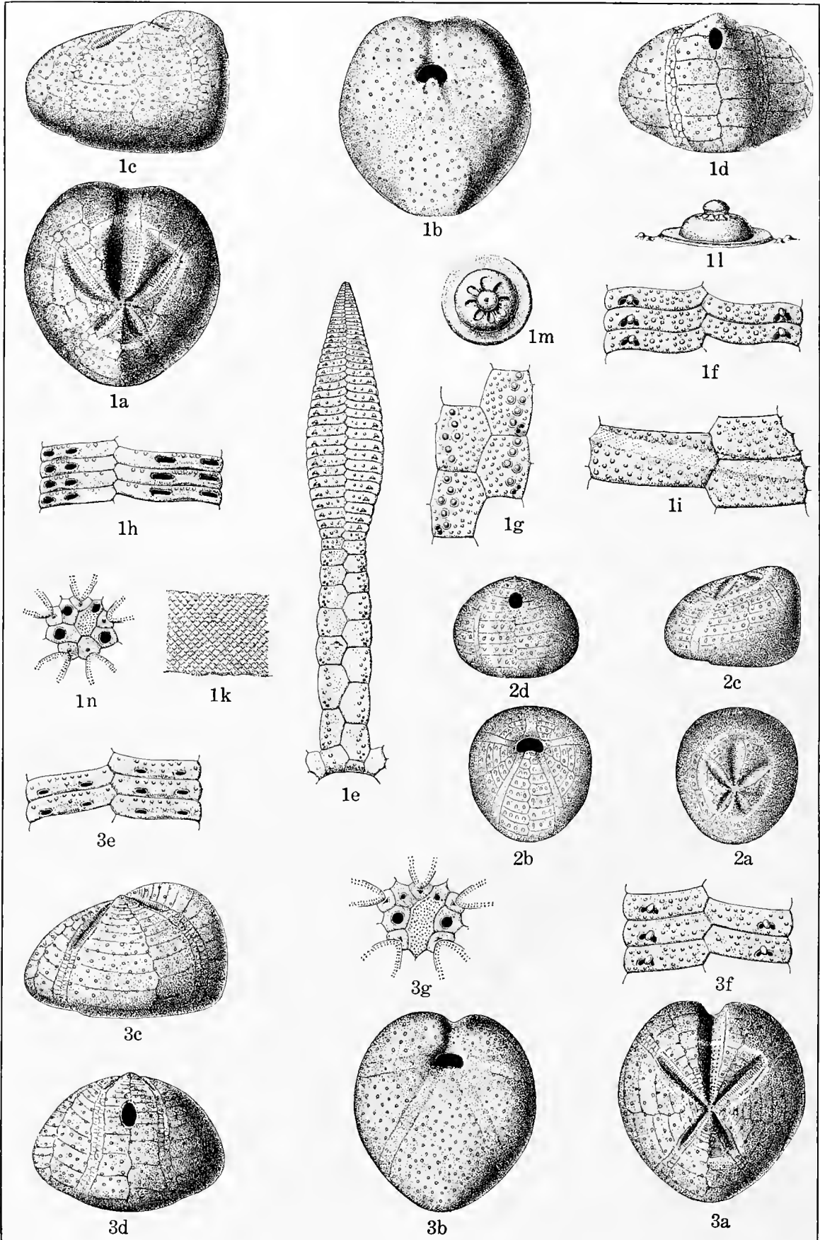
CRETACEOUS ECHINOIDEA.
