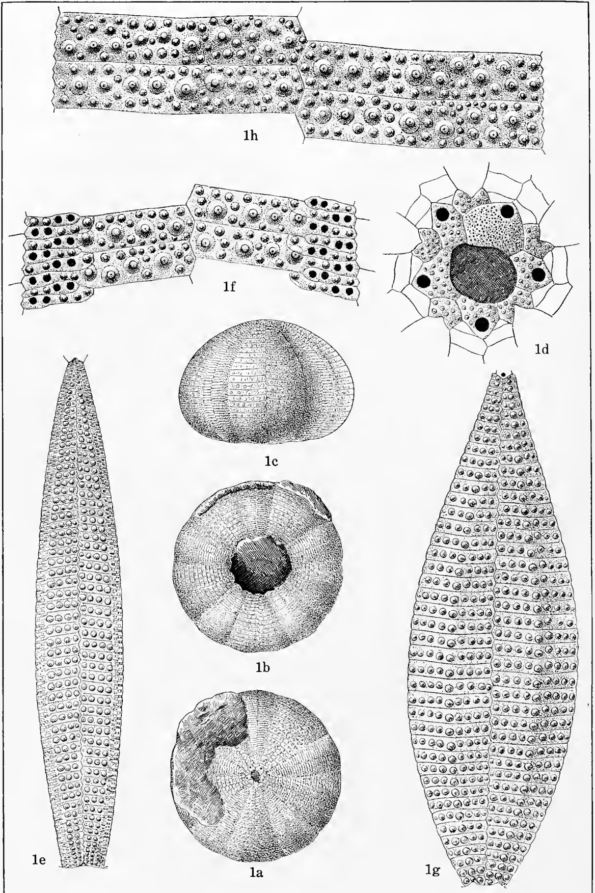
CRETACEOUS ECHINOIDEA.
