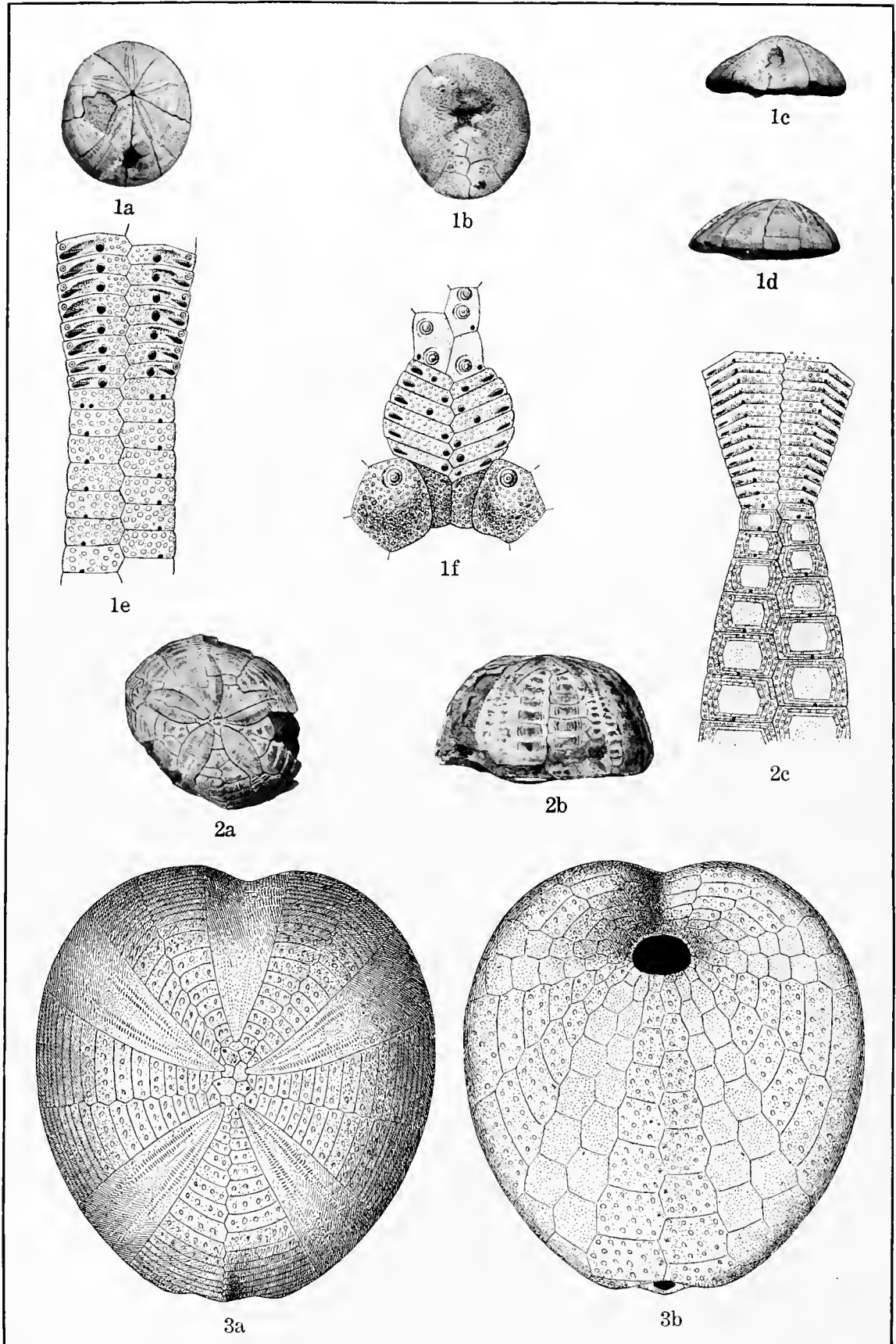
CRETACEOUS ECHINOIDEA.
