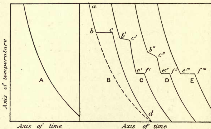
FIG. 1.—Cooling curve without change of state.
