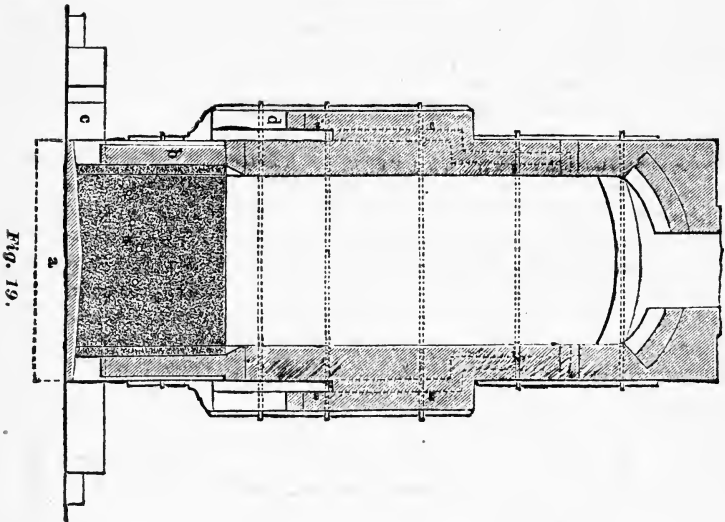
RACHETTE FURNACE AT CLAUSTHAL.
