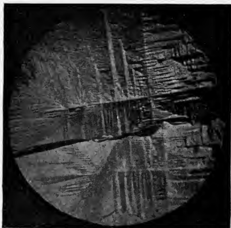
FIG. 76.—Fused Silver. Dendritic Surface ( \times 33 ).
