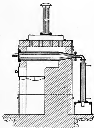
FIG. 68.—Krupp Furnace for Distilling Amalgam.
