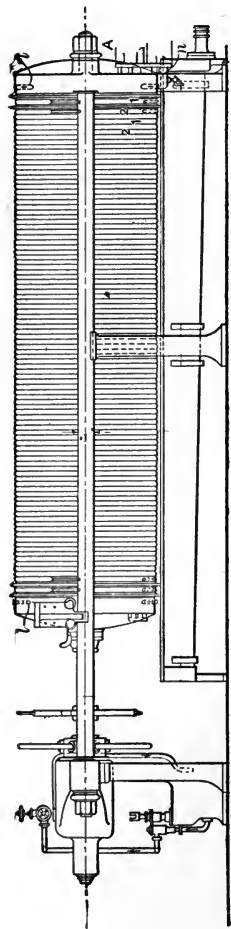
FIG. 24.—Side Elevation.
