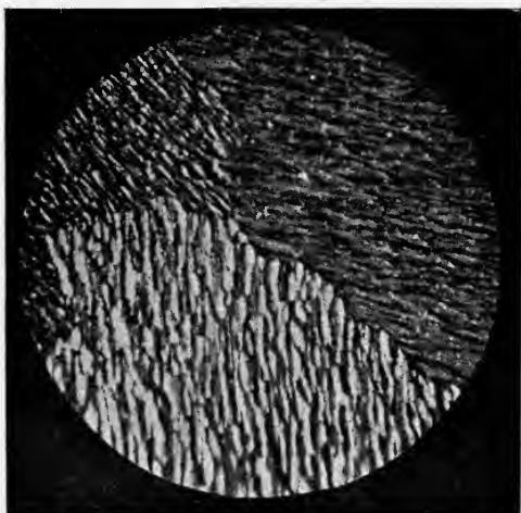
FIG. 159.—Deeply Etched Under-surface of a Cast Tin Ingot.
