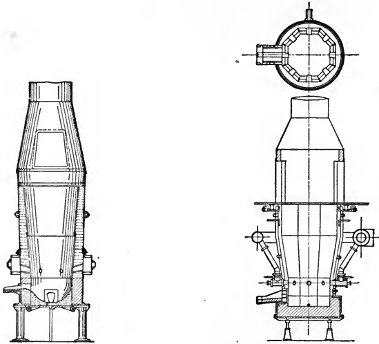
FIG. 100.—Allis-Chalmers.
