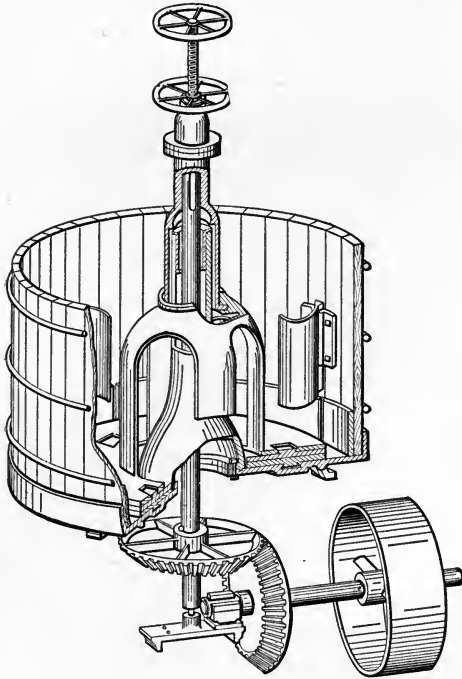
FIG. 65.—American-Amalgamating Pan.
