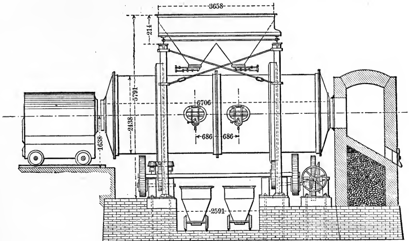
FIG. 93.—Brückner Furnace. Scale 1:150.
