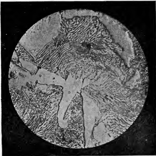
FIG. 178.—White Cast Iron. Cementite (White) with Lamellar Pearlite ( \times 500 ).
