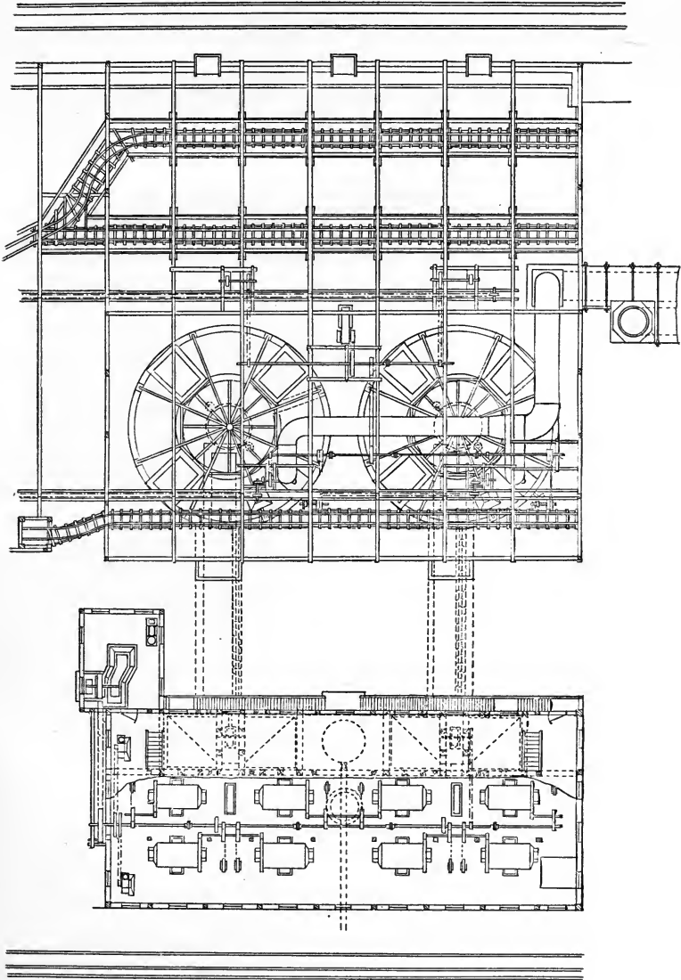
FIG. 6.—Plan of a Chiorinanti Plant.
