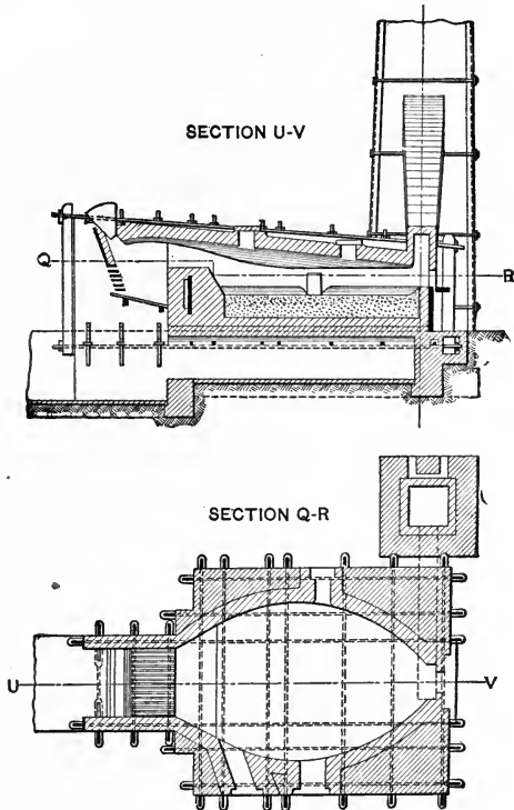
FIG. 108.—Mansfeld Furnaces.
