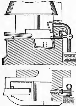
FIG. 181.—Charcoal Hearth.
