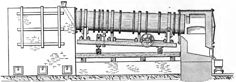
FIG. 94.—White-Howell Furnace.
