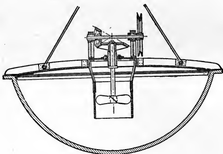
FIG. 51.—Desilverizing Kettle and Auxiliary Apparatus, with stirrer.
