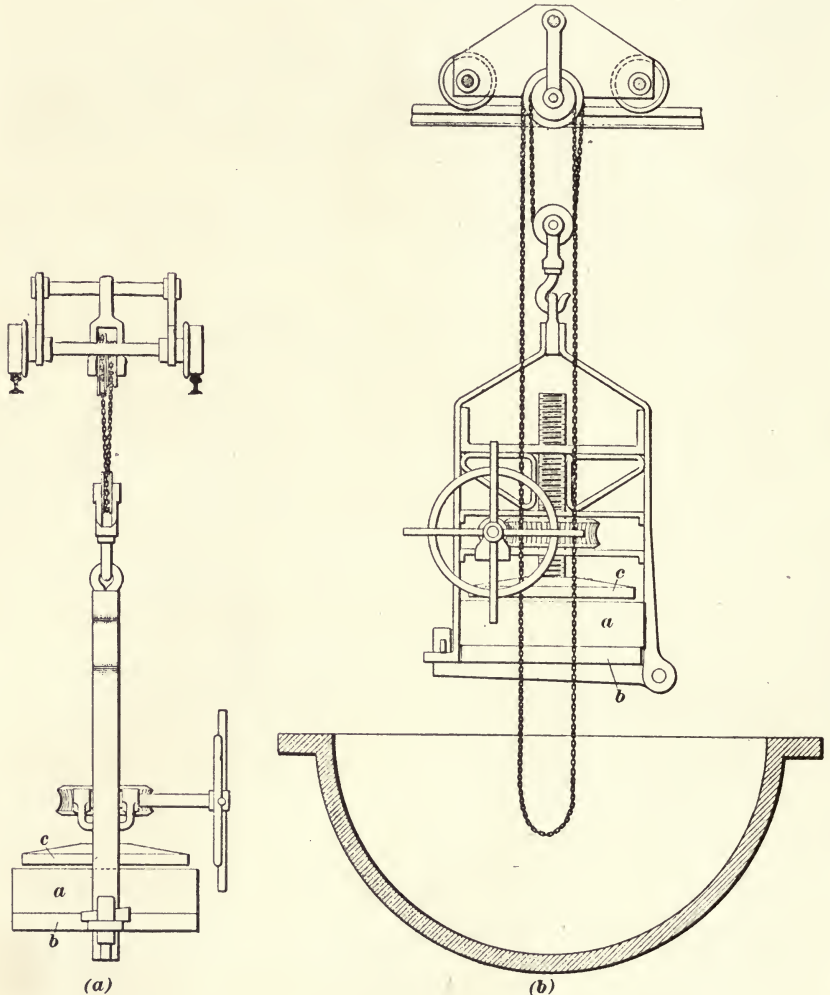
Fig. 173. HOWARD PRESS.
