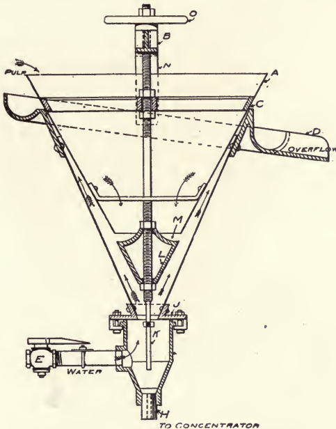
Fig. 84. DOUBLE-CONE CLASSIFIER.
