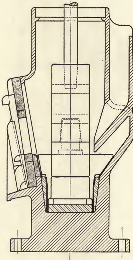
Fig. 47. SINGLE-DISCHARGE MORTAR.
