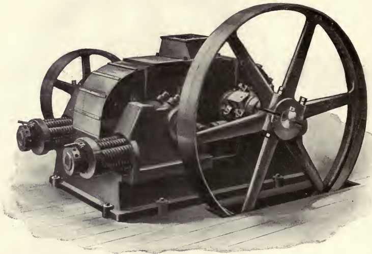
Fig. 24. CRUSHING ROLLS.
