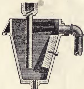
Fig. 52. MERCURY TRAP.
