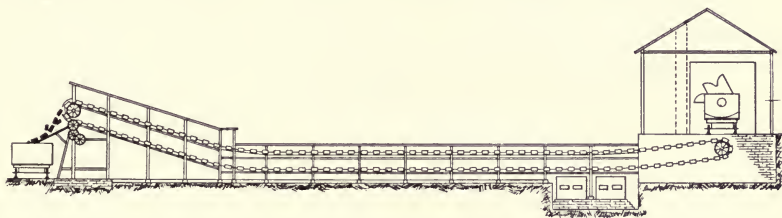
Fig. 126. HEYL AND PATTERSON PIG-CASTING MACHINE.
