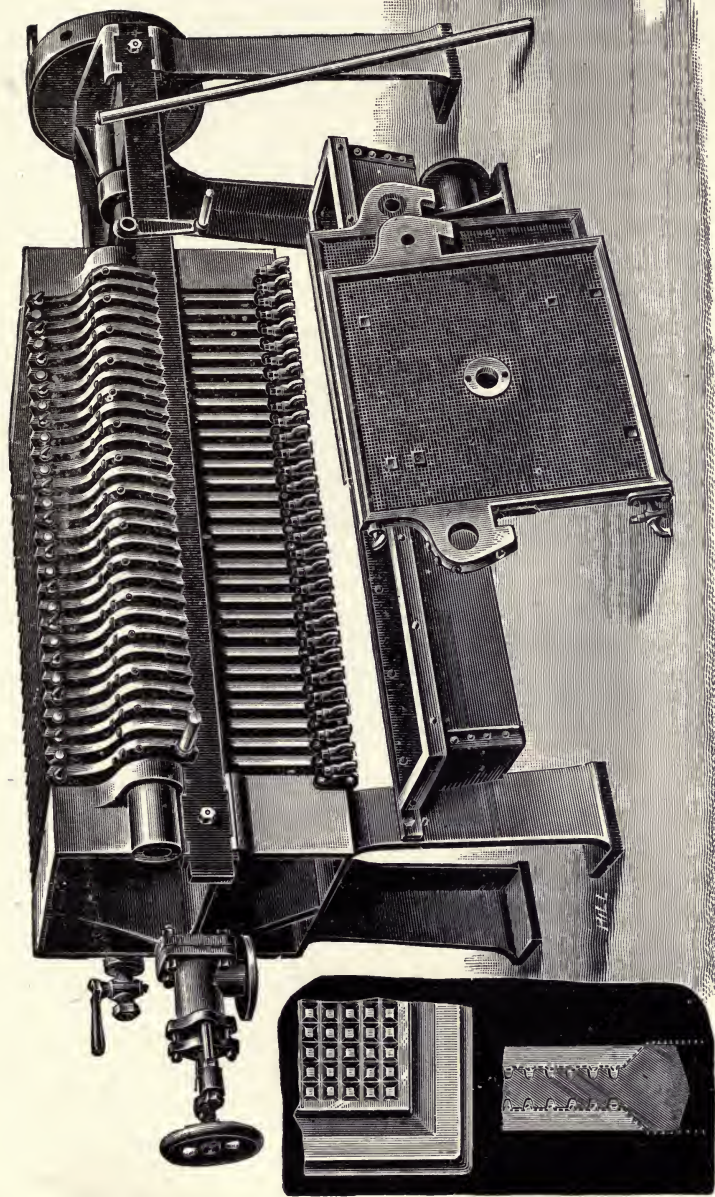
FIG. 78. FILTER PRESS.
