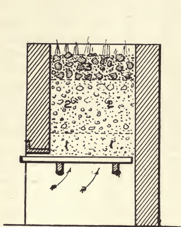
Fig. 2. WIND FURNACE.
