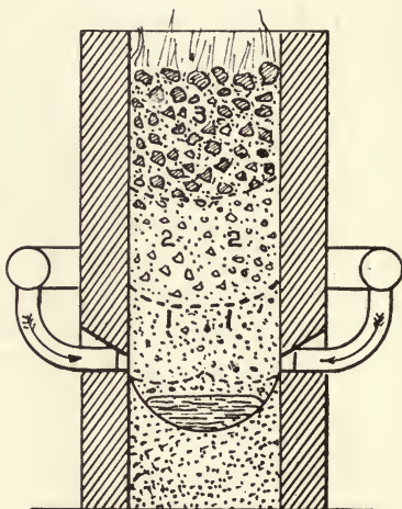
Fig. 3. CUPOLA FURNACE.
