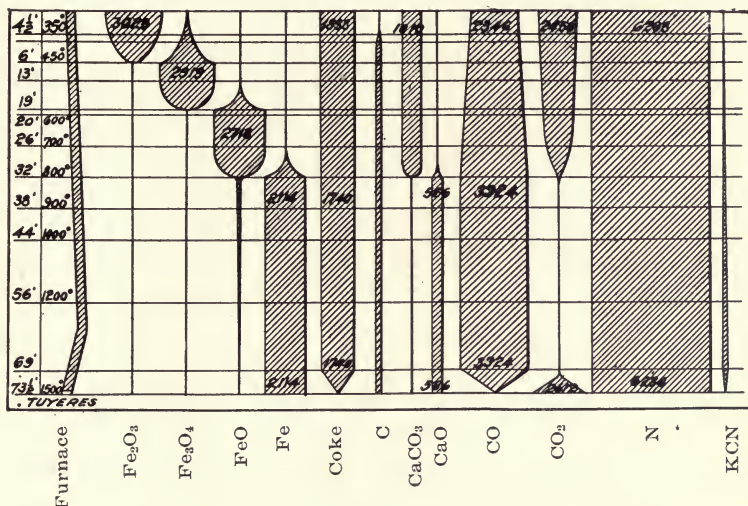
Fig. 127. CHEMICAL REACTIONS OF BLAST-FURNACE.
