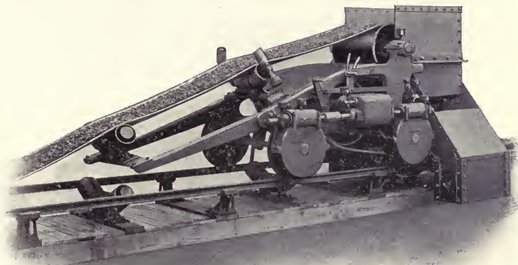
Fig. 193. CONVEYING BELT WITH TRIPPER.
