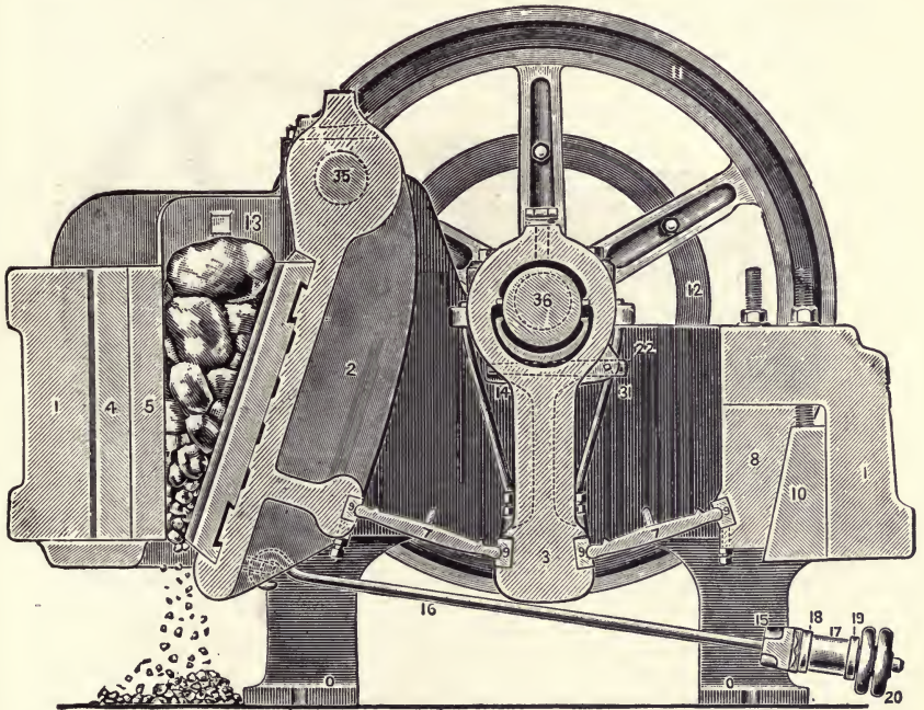
Fig. 23. BLAKE ORE-CRUSHER (SECTION).
