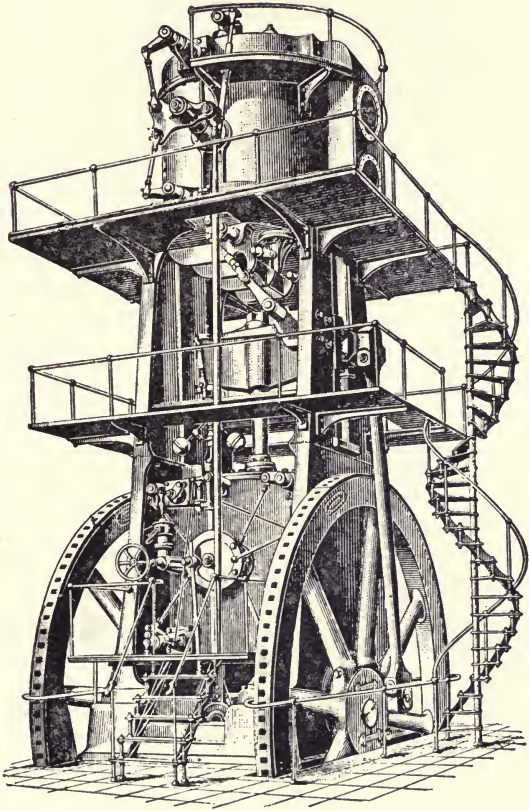
Fig. 125. BLOWING ENGINE.
