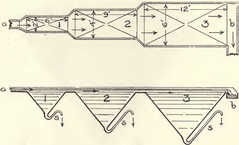
Fig. 82. THREE-COMPARTMENT SPITZKASTEN.
