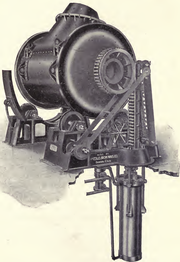
Fig. 142. COPPER CONVERTER.
