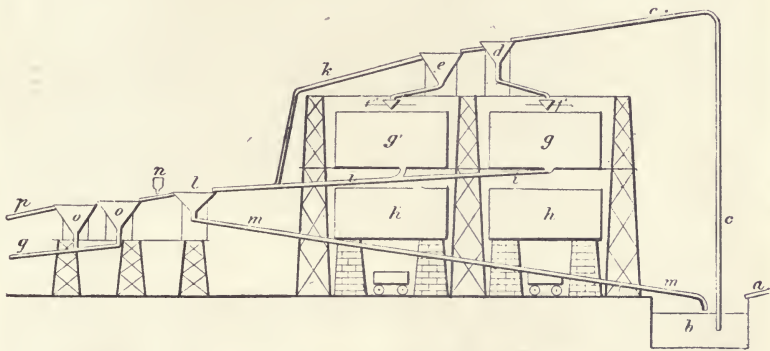
Fig. 85. CYANIDE PLANT FOR DOUBLE TREATMENT.
