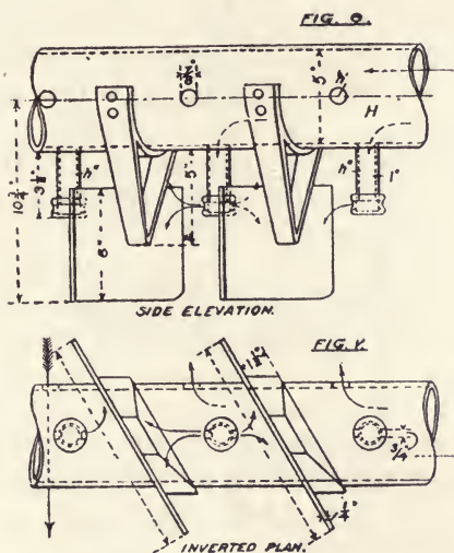
Fig. 42. DETAIL OF RABBLES.
