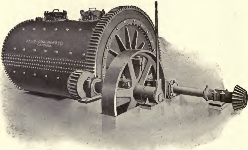
Fig.61. CHLORINATION BARREL.
