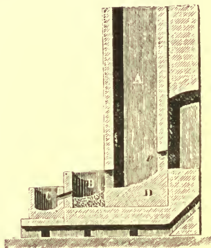
FIG. 51.—Blast-furnace or Blowing-house for smelting Tin Ores.
