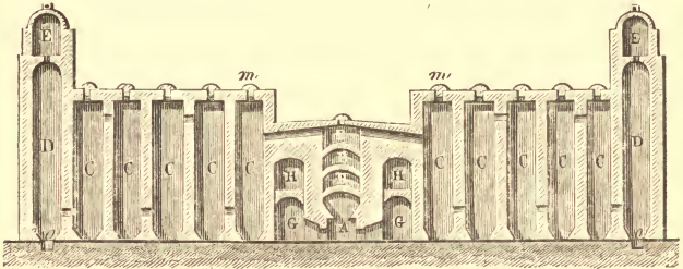
FIG. 98.—Section of Idrian Furnace and Condensing Chambers. A , Fire-place. B , Arches upon which the ore is placed. C D E , Condensing chambers. G H , Air channels.
