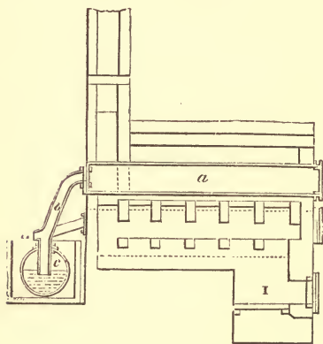
FIG. 101.—Ure's Retort for extraction of Mercury from Cinnabar.
