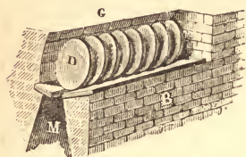
FIG. 78.—Liquation-hearth.
