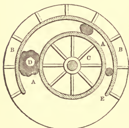
FIG. 15.—Cylindrical Rotating Squeezer for Puddled Balls, seen from above.
