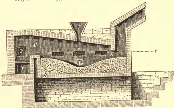
FIG. 62.—Reverberatory Furnace for smelting Galena.
