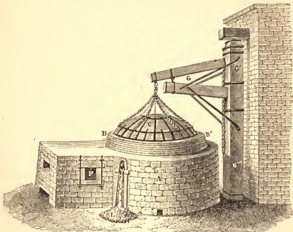
FIG. 76.—German Cupellation-furnace.
