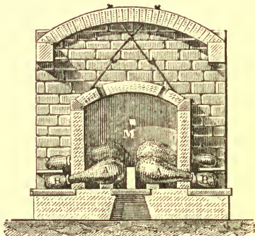
FIG. 100.—Extraction of Mercury in the Palatinate.
