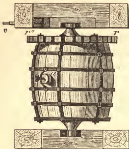
FIG. 81.—Amalgamation Cask. a , Opening for charging and discharging. r r'' , Toothed wheel for receiving motion from the axis (Fig. 82).
