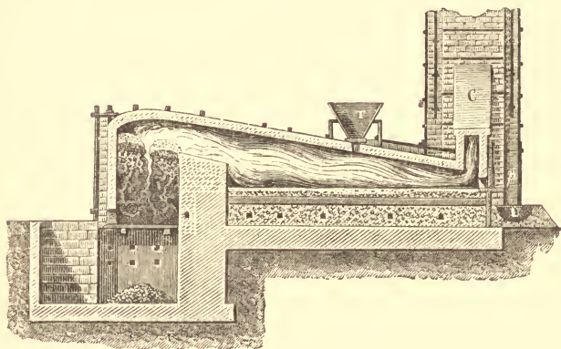
FIG. 33.—Section of Ore-furnace for smelting Copper Ores. T, Hopper for introducing the charge. B, Tap-hole for discharging the slag into the slag-moulds U. C, Flue leading to the chimney.
