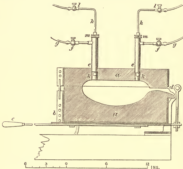
FIG. 104.—Lime Furnace for melting Platinum with the Oxy-hydrogen Blowpipe. a a , Blocks of lime hollowed out to form the furnace. k k , Openings for the oxy-hydrogen blowpipes. e e , Outer tubes conveying the hydrogen or coal-gas. h h , Inner tubes conveying the oxygen. d , Spout for pouring the melted platinum.
