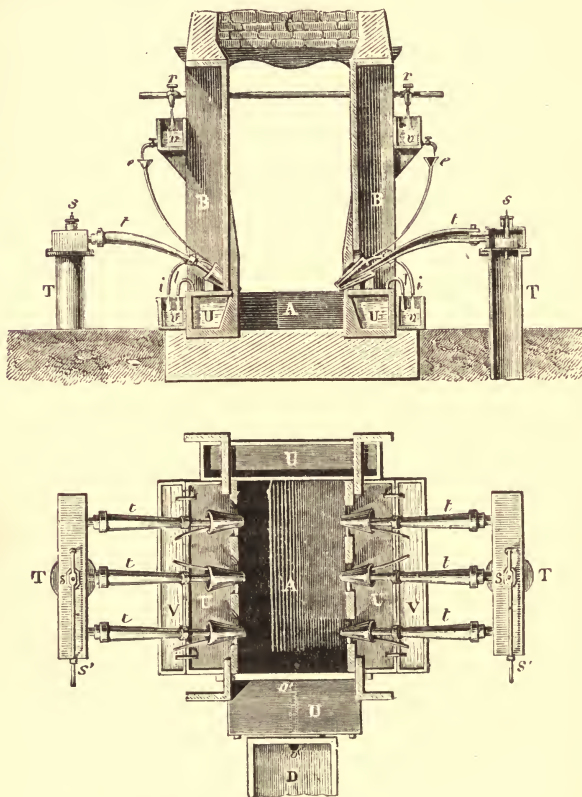
FIG. 10.—Hearth for refining Cast Iron, in section and plan. A, Hearth in which the fuel and pig-iron are placed. B, Hollow iron supports for the chimney C, which is about 18 feet high. D, Flat mould for the refined iron. e, Funnel-pipes for conveying water to the tuyères. i, Pipes for carrying off the heated water from the tuyères. l, Pipes for carrying off the heated water from the hollow walls u. o, Tap-hole for running out the fine metal. r, Stopcocks for supplying water to the cisterns v. s, Valves for regulating the blast issuing from the pipes T.
