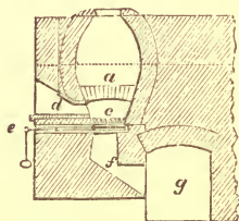
FIG. 61.—Furnace for making Brass. a , Arch upon which the crucibles stand. c , Grate. d , Fire-door. e , Damper. f , Inclined plane for carrying away cinders into the channel g .
