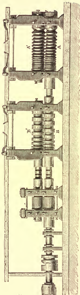
FIG. 12.—Mill for rolling Puddled Bars.
