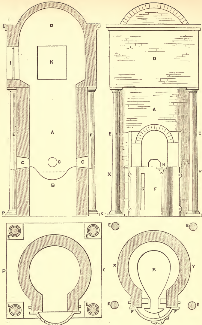
FIG. 68.—Castilian Furnace for Lead-smelting. A, Body of the furnace. B, Crucible for receiving the lead. C, Blast-pipe. D, Masonry enclosing the top of the furnace. E, Cast-iron pillars. F, Receptacle for the lead. G, Slot for the tapping-hole. H, Spout for overflow of slag. I, Charging-door. K, Flue. P Q, Ground line.
