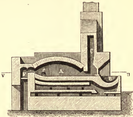
FIG. 41.—Section of Furnace for refining Black Copper, at Mansfeld, made at the line x of the plan, Fig. 42.
