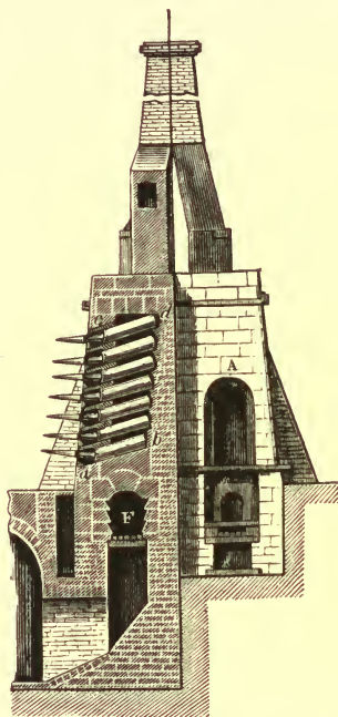
FIG. 56.—Belgian Furnace for distilling Zinc from its Ores.
