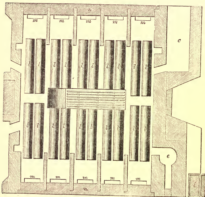
FIG. 58.—Silesian Zinc-furnace; plan. z , Arched retorts. c , Space for heating the retorts before setting them in the furnace. e , Pot for remelting the distilled zinc. i , Iron ingot-moulds for casting the zinc.
