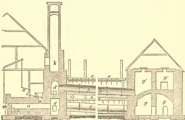
FIG. 99.—Modern Idrian Mercury-furnace.
