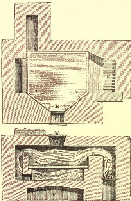
FIG. 53.—Reverberatory Furnace for manufacture of Tungstate of Soda from Tin Ores. B, Opening for introducing the charge. D, Working-door. E, Opening for discharging the contents of the hearth. F, Vault for receiving the finished charge.
