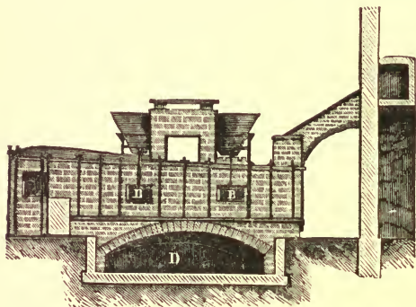
FIG. 30.—Furnace for roasting Copper Ores. BB, Working doors. D, Vault for receiving the roasted ore.
