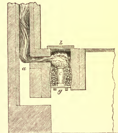
FIG. 22.—Furnace and Pot for melting Steel. g, Grate. c, Crucible. b, Cover of Furnace. a, Chimney.
