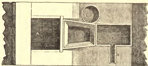
FIG. 67.—Plan of Slag-hearth.
