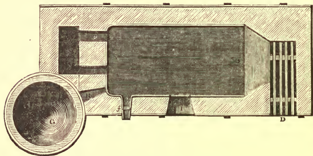
FIG. 70.—Plan of Improving Furnace.
