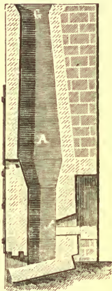
FIG. 38.—Blast-furnace employed for smelting the Bituminous Schists at Mansfeld.
