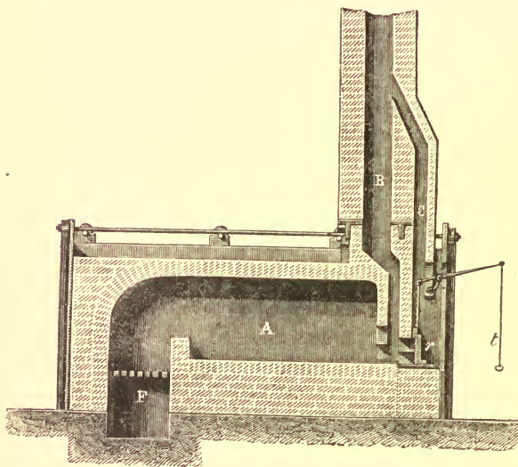
FIG. 16.—Reheating Furnace. A, Hearth upon which the bars are heated. F, Grate. r, Door opened by the lever t, for introducing the bars. o, Opening through which the flame and smoke pass into the flue B. C, Flue through which the air entering by the charging door passes into the chimney.
