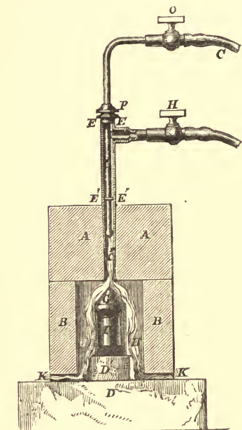
Fig. 103.—Platinum melted in Crucible by the Oxy-hydrogen Blowpipe.
