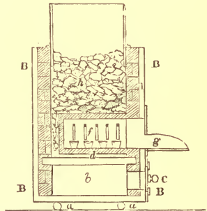
FIG. 93.—Assay by Cupellation. a , Iron castors on which the furnace moves. b , Ash-pit. c , Damper. d , Grate. f , Muffle containing the cupels. g , Mouth-plate. h , Fuel.
