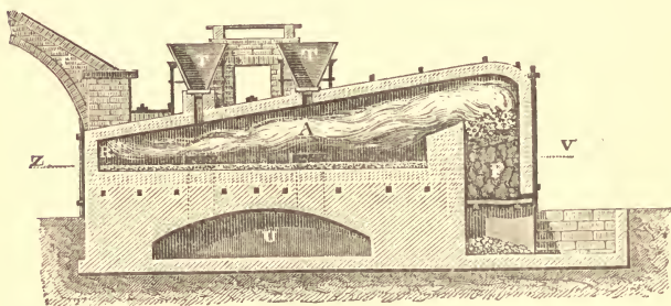
FIG. 31.—Furnace for roasting Copper Ores. Section through the line x y of the plan (fig. 32).
