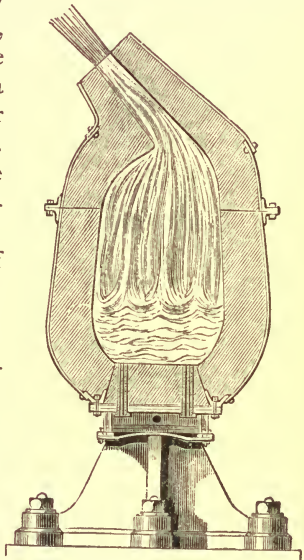
FIG. 23.—Bessemer's Converting Vessel.
