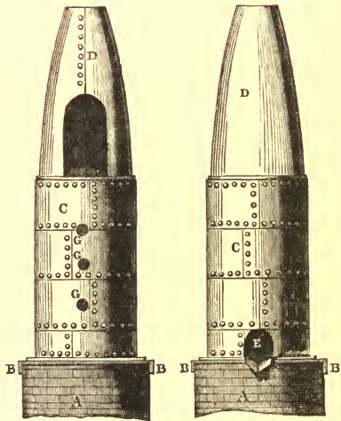
FIG. 9.—Front and Back Views of Cupola Furnace. A , Foundation of Masonry covered with Iron Plates B .
