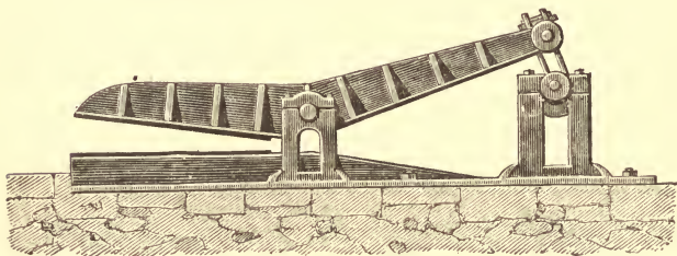
FIG. 13.—Squeezer for Puddled Balls.
