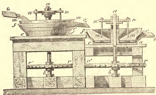
FIG. 89.—Mill for amalgamating Pyrites containing Gold. r r' , Toothed wheels for transmitting motion to the axle a b .
