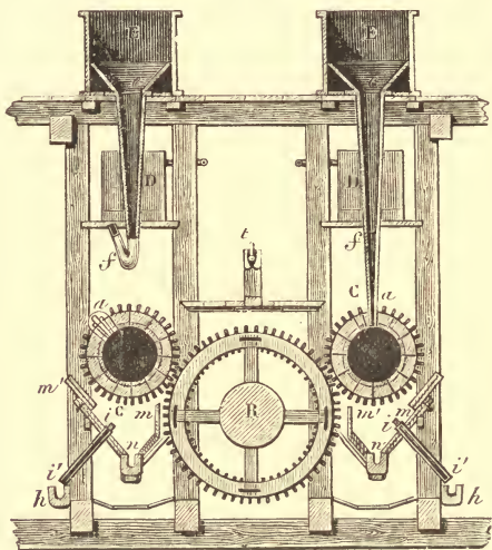
FIG. 83.—Amalgamation of Silver Ores at Freiberg. E , Reservoirs for the ground mineral. f , Leathern pipe for conveying it into the opening a of the cask C . D , Cisterns containing water. m m' , Receptacles for the amalgam and spent charge. i i' , Pipe for conveying the amalgam into the gutter h .
