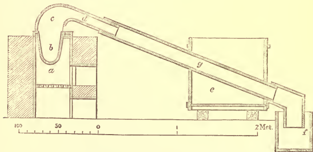
FIG. 85.—Apparatus for distillation of the Amalgam of Silver.
