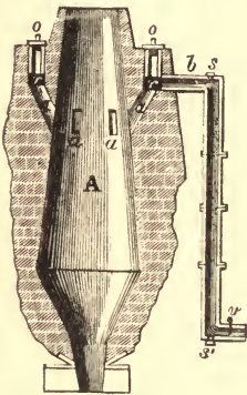
FIG. 6.—Blast-furnace, with openings for drawing off the waste gases.
