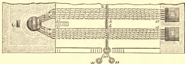
FIG. 95.—Plan of Aludel Furnace for extraction of Mercury.
