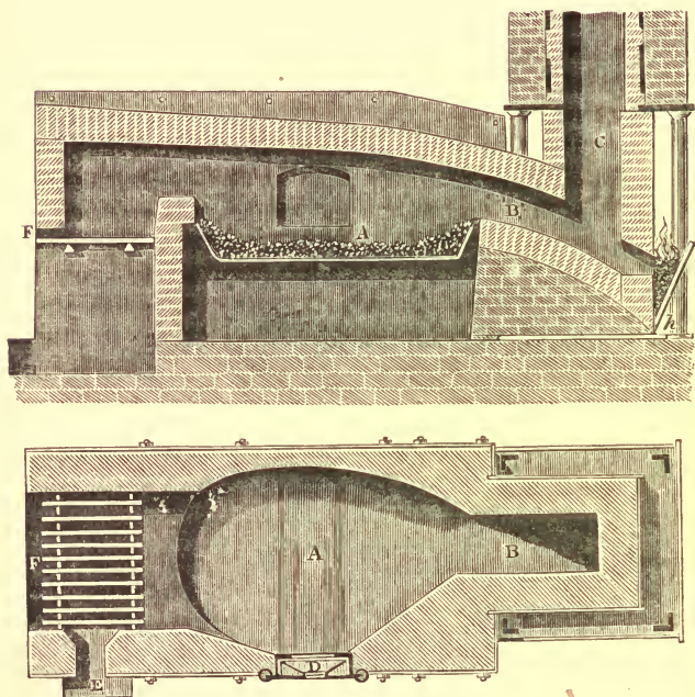
FIG. 11.—Puddling Furnace.
