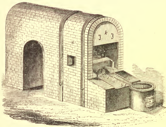
FIG. 65.—Scotch Furnace or Ore-hearth for the extraction of Lead.
