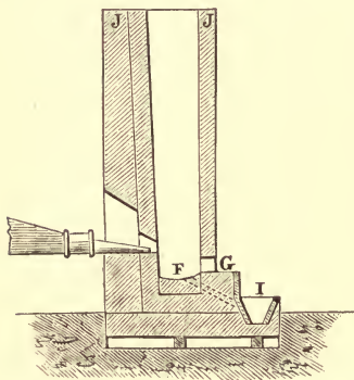
FIG. 52.—Blowing-house at Altenberg. F, Crucible. G, Inclined plane for slag. I, Fore-hearth.
