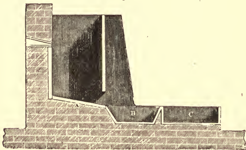
FIG. 66.—Slag-hearth for extracting Lead.
