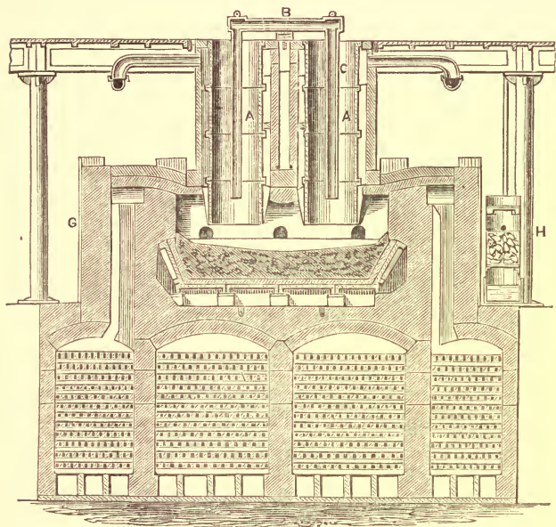
FIG. 28.—Furnace proposed by Siemens, for making cast steel in his Regenerative Furnace. Beneath are shown the chambers containing fire-brick for accumulating the heat of the products of combustion before they pass into the chimney. B, Blast-pipe, from which pipes descend at right angles into the small blast-furnaces A.
