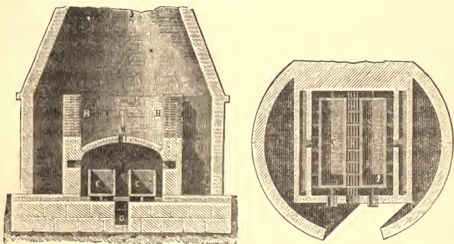
FIG. 20.—Cementation Furnace for converting Bar Iron into Steel.
