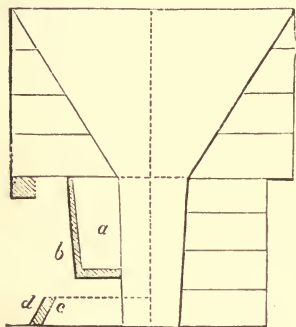
FIG. 2.—Boshes, Hearth, and Crucible of Blast-furnace.
