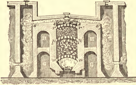
FIG. 97.—Extraction of Mercury at Idria. G H , Passages from which air enters through flues into the space occupied by the ore. c , Condensing chambers.
