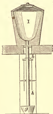
FIG. 54.—Crucible for extraction of Zinc by the English method.
