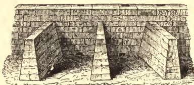
FIG. 40.—Roasting-stalls employed at Mansfeld.
