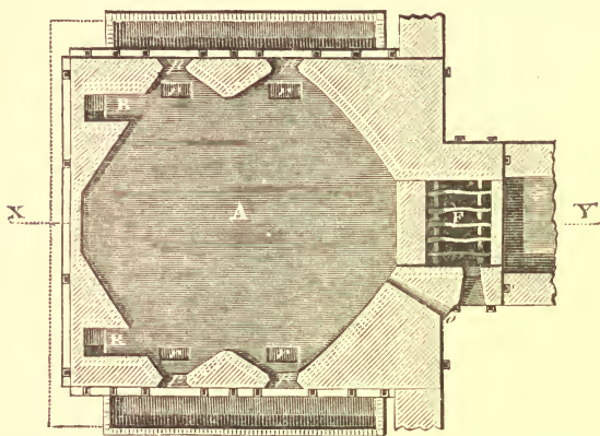
FIG. 32.—Furnace for roasting Copper Ores. Plan at the line z v of the section (fig. 31).
