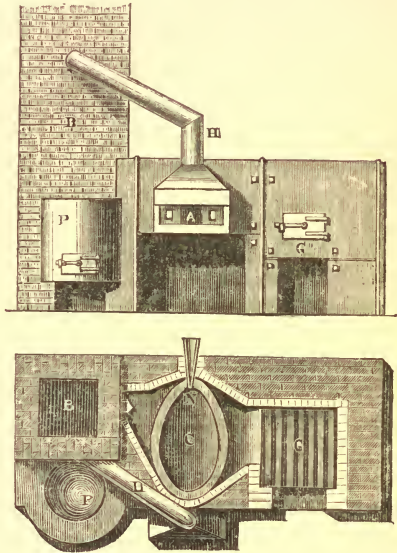
FIG. 75.—English Furnace for the cupellation of Lead.
