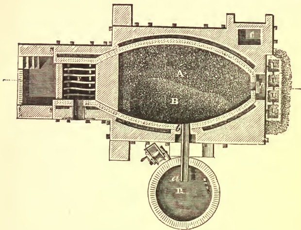
FIG. 34.—Plan of Ore-furnace for smelting Copper Ores. F, The grate. R, Tank for granulating the coarse metal.
