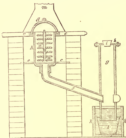
FIG. 90.—Apparatus for distilling the Amalgam of Gold. a , Dishes for receiving the amalgam, attached to the pillar b . A , Iron cylinder heated by a fire on the grate c . d , Iron dome. e , Iron cover of the furnace. f , Tube for vapour of mercury. g , Cylinder in which the mercury condenses, closed by an iron plate h and a wooden plug i . k , Water-tank. l , Vessel for collecting the mercury. m , Chimney.
