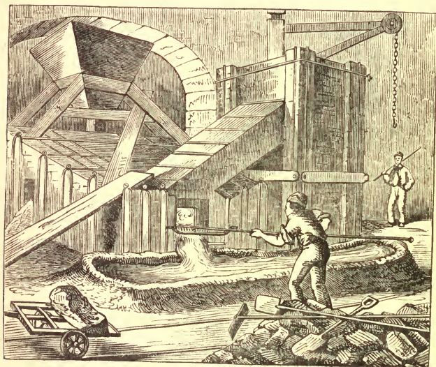
FIG. 36.—Copper Smelting-furnace.
