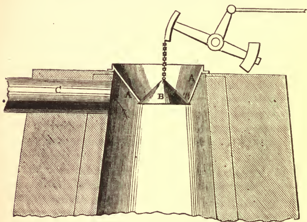
FIG. 7.—Cup and Cone for closing the Blast-furnace, in order that the waste gases may pass into the lateral flue, as shown by the arrow.
