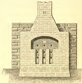
FIG. 8o.—Sweating-furnace. M, Back-wall with flues communicating with the chimney H.
