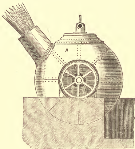
FIG. 26.—Bessemer's globular Converting Vessel.
