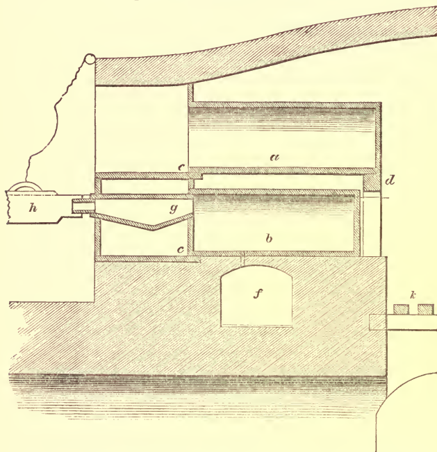
FIG. 60.—Belgian-Silesian Zinc-furnace. a b , Arched retorts. c d , Their supports. f , Flue. g , Condensing tube. h , Receiver suspended by iron-wire. k , Fire-place.
