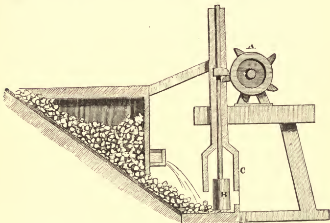
FIG. 45.—Section of Stamping-mill.
