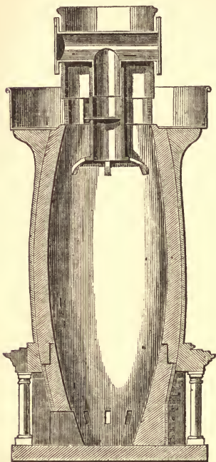
FIG. 8.—Schneider's arrangement for collecting the waste gases from the Blast-furnace by a central pipe.
