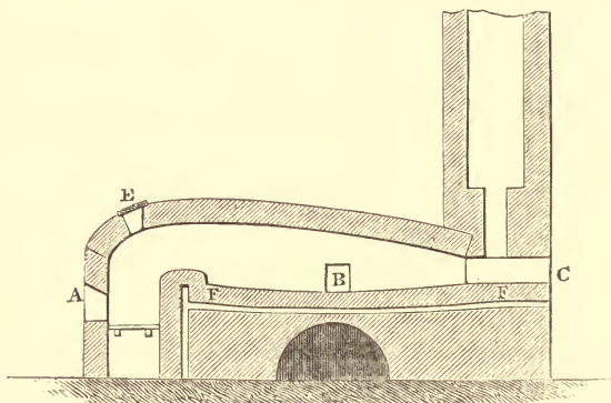
FIG. 50.—Furnace for smelting Tin Ores. A, Fire-door. B, Charging-door. C, Working-door. E, Door for moderating the draught whilst charging the furnace, lest the ore-dust be blown into the flue. F, Air-channel under hearth.
