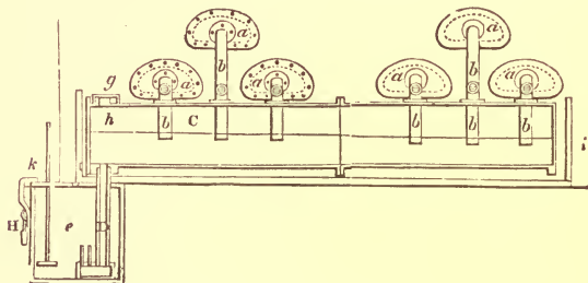
FIG. 102.—Ure's Retorts for extraction of Mercury.
