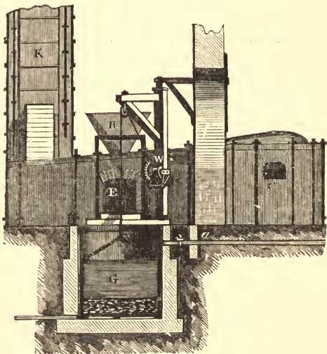
FIG. 35.—Elevation of Ore-furnace for smelting Copper Ores. H, Hopper for introducing the charge. K, Chimney. C, Fire-door. a, Pipe for supplying water to the tank.
