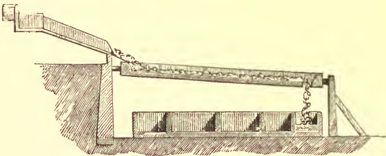
FIG. 47.—Section of Rack for washing Ores.
