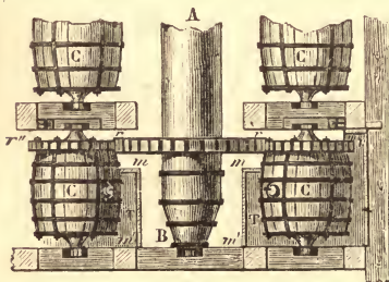
FIG. 82.—Amalgamation of Silver Ores at Freiberg. r r'' , Toothed wheels for transmitting motion from the axis A . m m' , Troughs for receiving the contents of the casks C .
