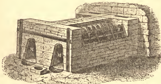
FIG. 79.—Liquation-hearth.
