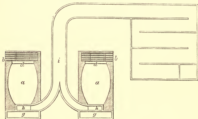
FIG. 49.—Saxon Furnaces for calcining Tin Ore. a , Hearth. b , Grate. d , Fire-bridge. g , Chimney. h , Flue. i , Channel for conveying the fumes into the condensing chambers.
