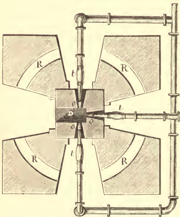
FIG. 4.—Arrangement of Tuyères in Blast-furnace. z , Pipes conveying the blast. o , Openings in the sides of the hearth D . R , Arched passages for the labourers.
