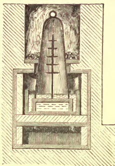
FIG. 84.—Distillation of the Amalgam of Silver.
