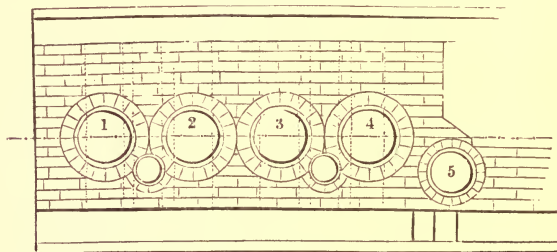
FIG. 71.—Pots for desilverising Lead.
