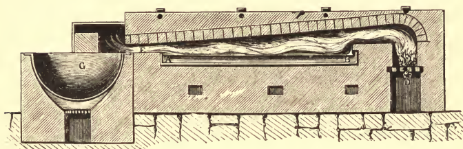
FIG. 69.—Calcining Furnace for improving Hard Lead.
