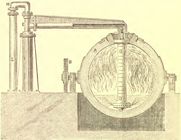
FIG. 27.—Section of Bessemer's globular Converting Vessel. A, The converter. B, Pulley wheel for tipping the converter, connected by a wire rope with a hydraulic ram. G, Pipe conveying the blast. H, Elbow-pipe with telescopic joint.
