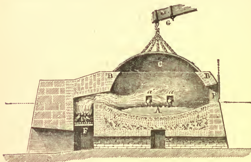
FIG. 77.—Section of German Cupellation-furnace.
