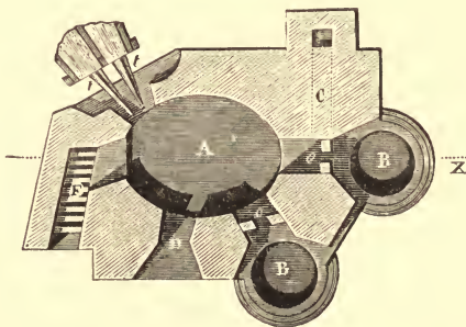
FIG. 42.—Plan of Furnace for refining Black Copper, at Mansfeld, made at the line v u of the section, Fig. 41.
