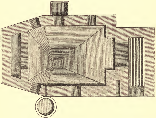
FIG. 64.—Hearth of Reverberatory Furnace for smelting Galena.
