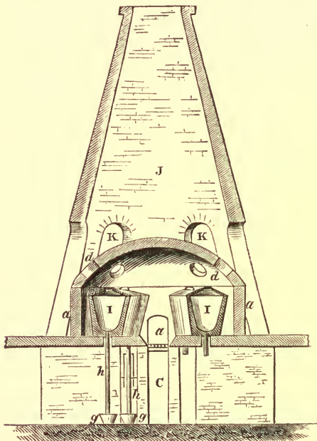
FIG. 55.—Extraction of Zinc by the English method.
