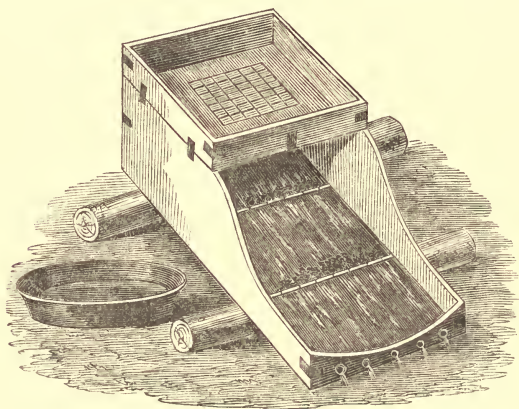
FIG. 88.—Cradle for Gold-washing.
