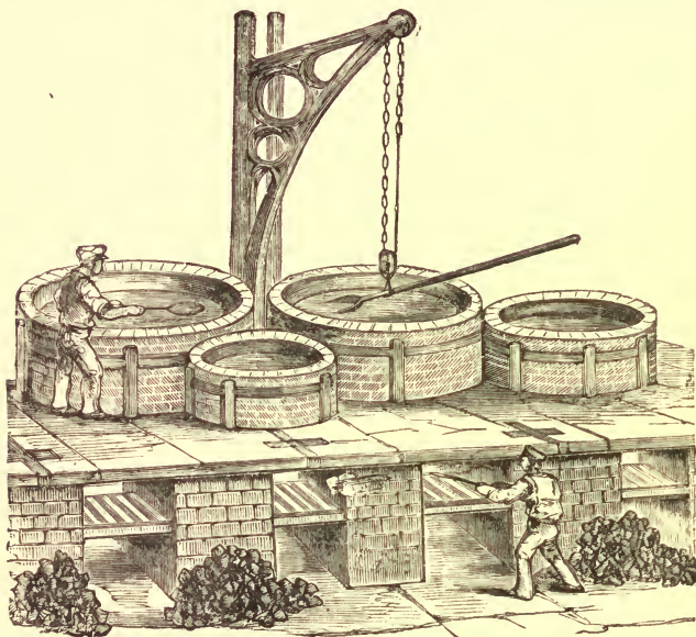
FIG. 73.—Desilverising Lead by Pattinson's Process.
