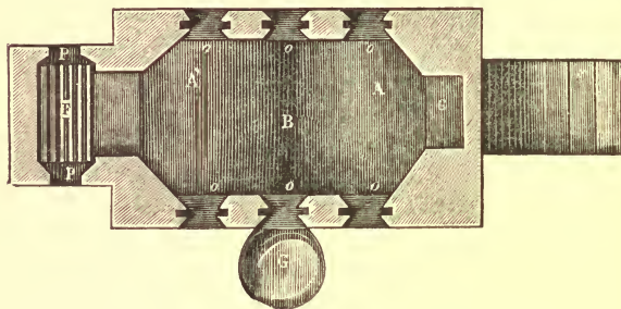
FIG. 63.—Plan of Reverberatory Furnace for smelting Galena.
