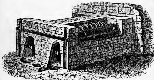
FIG. 79.—Liquation-hearth.
