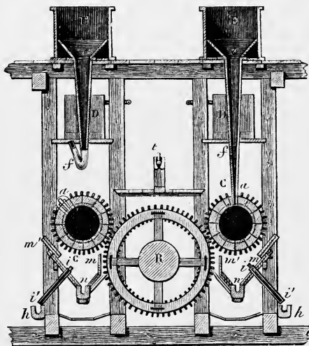
FIG. 83.—Amalgamation of Silver Ores at Freiberg. f , Reservoirs for the ground mineral. f , Leathern pipe for conveying it into the opening a of the cask c . d , Cisterns containing water. m m m ', Receptacles for the amalgam and spent charge. i i' ', Pipe for conveying the amalgam into the gutter h .
