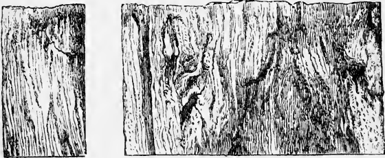
FIG. 19.--Structure of Puddled Bar.
