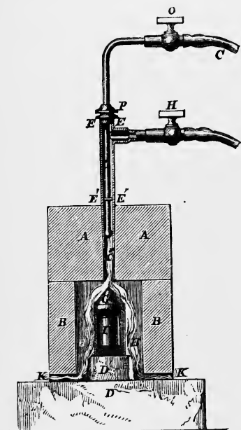
Fig. 103.—Platinum melted in Crucible by the Oxy-hydrogen Blowpipe.
