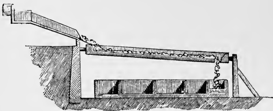
FIG. 47.—Section of Rack for washing Ores.
