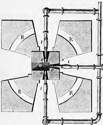
FIG. 4.—Arrangement of Tuyères in Blast-furnace. t , Pipes conveying the blast. o , Openings in the sides of the hearth D . R , Arched passages for the labourers.
