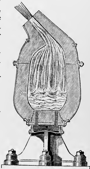
FIG. 23.—Bessemer's Converting Vessel.
