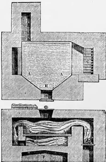
FIG. 53.—Reverberatory Furnace for manufacture of Tungstate of Soda from Tin Ores. B, Opening for introducing the charge. D, Working-door. E, Opening for discharging the contents of the hearth. F, Vault for receiving the finished charge.
