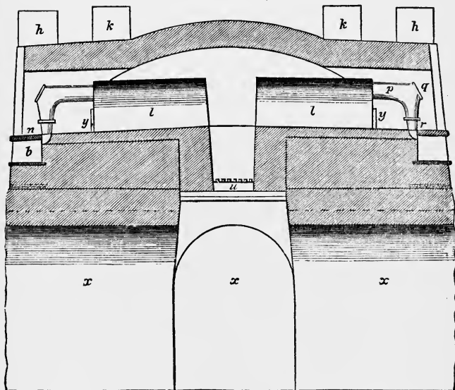
FIG. 57.—Silesian Zinc-furnace; section. l , Arched retorts. y , Door for removing the exhausted ore. q , Door for charging the retorts. p r , Tube for condensing the zinc. b , Receptacle for condensed zinc. h k , Flues. n , Fire-grate. x , Vaults.
