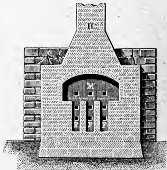
FIG. 80.—Sweating-furnace. M, Back-wall with flues communicating with the chimney H.
