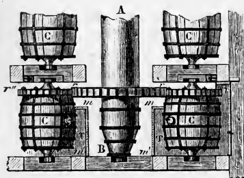
FIG. 82.—Amalgamation of Silver Ores at Freiberg. r r'' , Toothed wheels for transmitting motion from the axis A B. m m' , Troughs for receiving the contents of the casks C.
