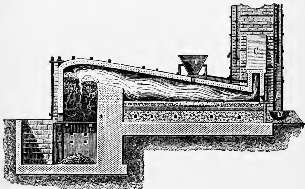
FIG. 33.—Section of Ore-furnace for smelting Copper Ores. T, Hopper for introducing the charge. P, Tap-hole for discharging the slag into the slag-moulds U. C, Flue leading to the chimney.
