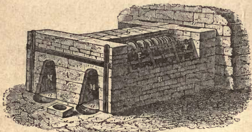
FIG. 79.—Liquation-hearth.
