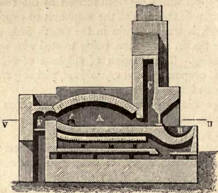
FIG. 41.—Section of Furnace for refining Black Copper, at Mansfeld, made at the line x of the plan, Fig. 42.
