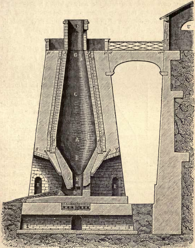
FIG. 1.—Blast-furnace for Smelting Iron Ores.
