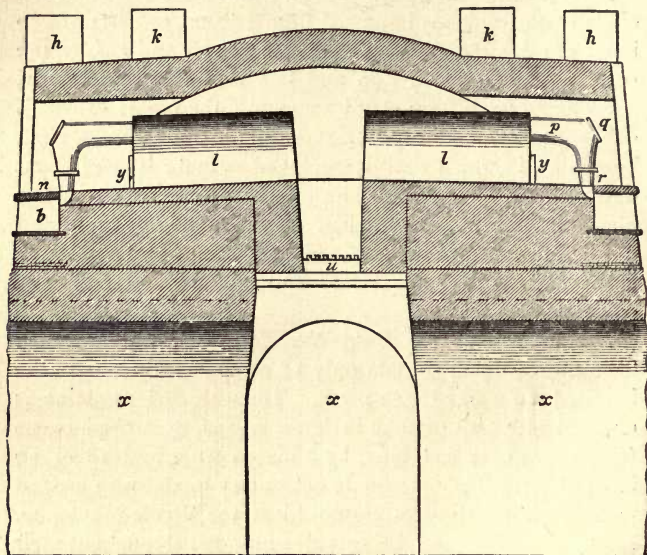
FIG. 57.—Silesian Zinc-furnace; section. l , Arched retorts. y , Door for removing the exhausted ore. q , Door for charging the retorts. p , r , Tube for condensing the zinc. b , Receptacle for condensed zinc. h , k , Flues. z , Fire-grate. x , Vaults.
