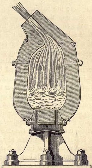
FIG. 23.—Bessemer's Converting Vessel.
