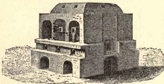
FIG. 59.—Silesian Furnace for distilling Zinc from its Ores. z , Condensing tube. z , Openings beneath the hearth for receiving the condensed zinc.
