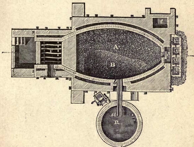
FIG. 34.—Plan of Ore-furnace for smelting Copper Ores. F, The grate. R, Tank for granulating the coarse metal.
