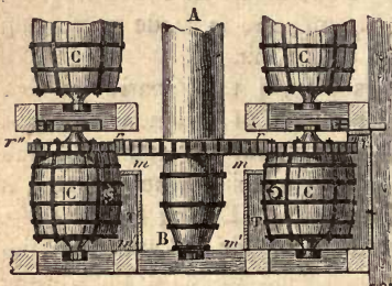
FIG. 82.—Amalgamation of Silver Ores at Freiberg. \gamma \gamma' , Toothed wheels for transmitting motion from the axis A. B, Troughs for receiving the contents of the casks c.
