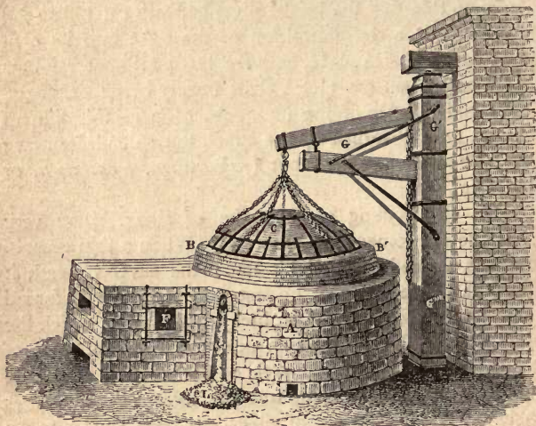
FIG. 76.—German Cupellation-furnace.
