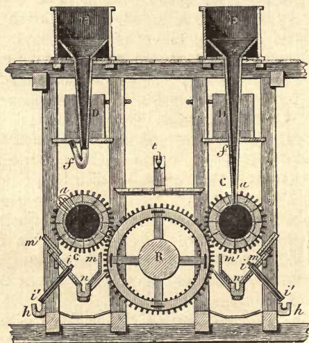
FIG. 83.—Amalgamation of Silver Ores at Freiberg. E, Reservoirs for the ground mineral. f, Leathern pipe for conveying it into the opening a of the cask c. D, Cisterns containing water. m n m', Receptacles for the amalgam and spent charge. i i', Pipe for conveying the amalgam into the gutter h.
