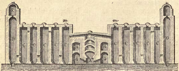
FIG. 98.—Section of Idrian Furnace and Condensing Chambers. A, Fire-place. B, Arches upon which the ore is placed. C D E, Condensing chambers. G H, Air channels.
