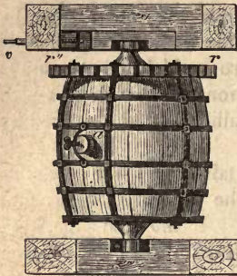
FIG. 81.—Amalgamation Cask. \alpha , Opening for charging, and discharging. \gamma \gamma'' , Toothed wheel for receiving motion from the axis (Fig. 82).
