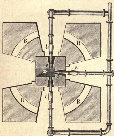
FIG. 4.—Arrangement of Tuyères in Blast-furnace. t , Pipes conveying the blast. o , Openings in the sides of the hearth. R , Arched passages for the labourers.
