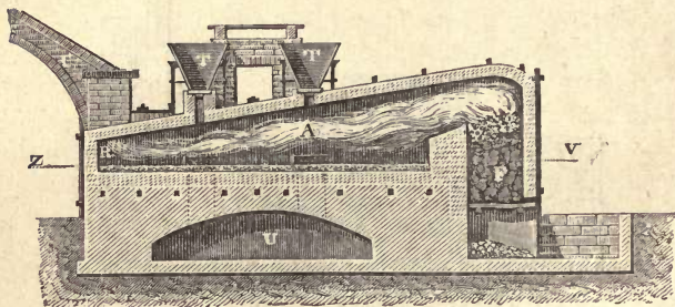
FIG. 31.—Furnace for roasting Copper Ores. Section through the line x v of the plan (fig. 32).
