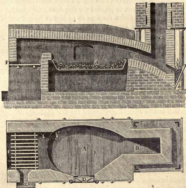
FIG. II.—Puddling Furnace.
