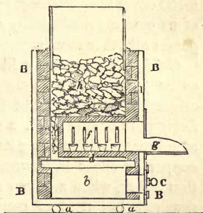
FIG. 93.—Assay by Cupellation. a , Iron castors on which the furnace moves. b , Ash-pit. c , Damper. d , Grate. f , Muffle containing the cupels. g , Mouth-plate. h , Fuel.
