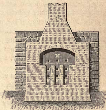
FIG. 8o.—Sweating-furnace. M, Back-wall with flues communicating with the chimney H.
