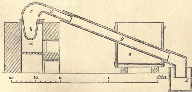
FIG. 85.—Apparatus for distillation of the Amalgam of Silver.
