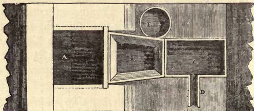
FIG. 67.—Plan of Slag-hearth.
