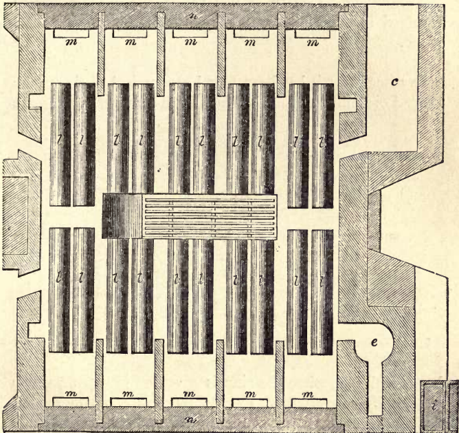
FIG. 58.—Silesian Zinc-furnace; plan. l , Arched retorts. c , Space for heating the retorts before setting them in the furnace. e , Pot for remelting the distilled zinc. i , Iron ingot-moulds for casting the zinc.
