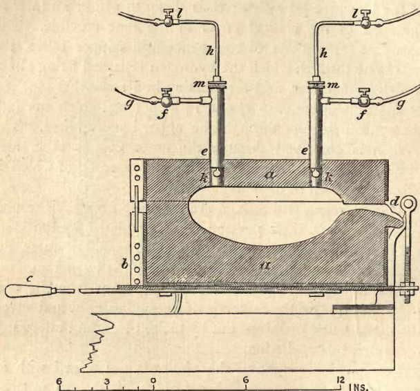
FIG. 104.—Lime Furnace for melting Platinum with the Oxy-hydrogen Blow-pipe. a a , Blocks of lime hollowed out to form the furnace. k k , Openings for the oxy-hydrogen blowpipes. e e , Outer tubes conveying the hydrogen or coal-gas. h h , Inner tubes conveying the oxygen. d , Spout for pouring the melted platinum.
