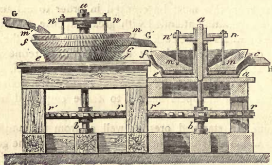
FIG. 89.—Mill for amalgamating Pyrites containing Gold. r' , Toothed wheels for transmitting motion to the axle a b .
