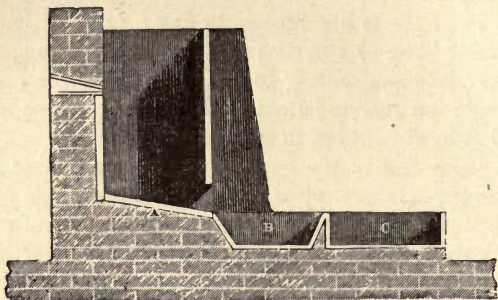
FIG. 66.—Slag-hearth for extracting Lead.
