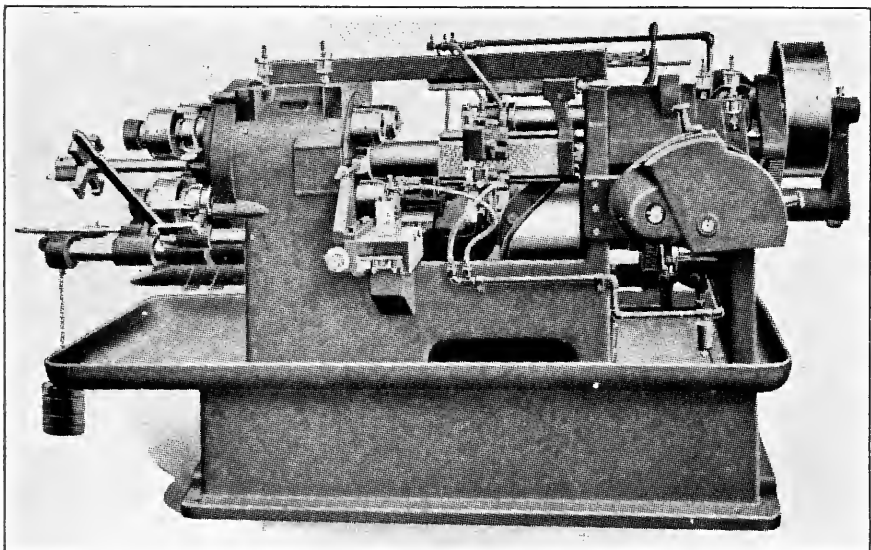
Multiple-spindle automatic screw machine
