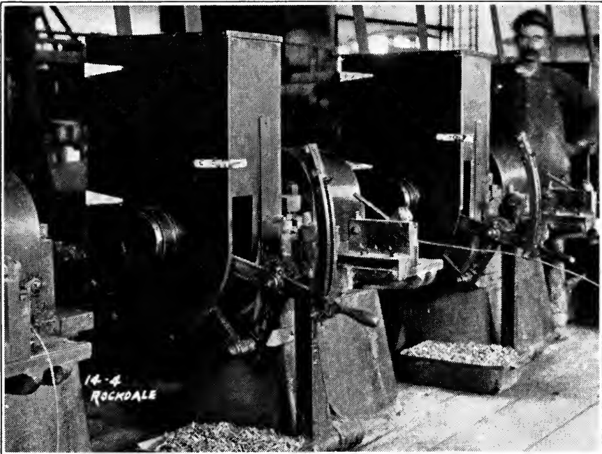
Fence staple machines
