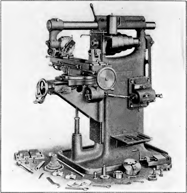
Universal milling machine
