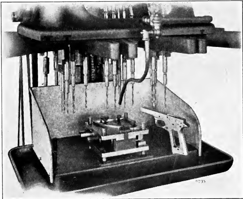
Multiple-spindle drill operating upon automatic pistol frames
