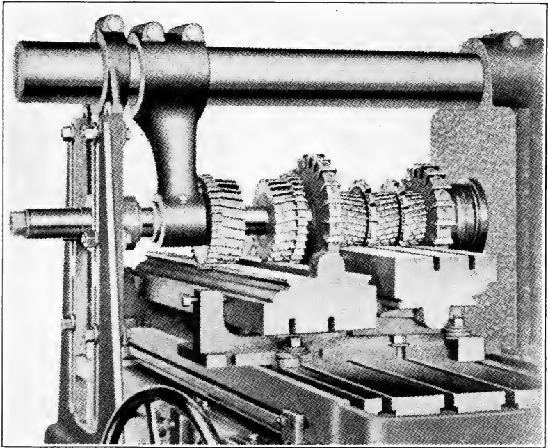
Gang cutters milling two sides at once
