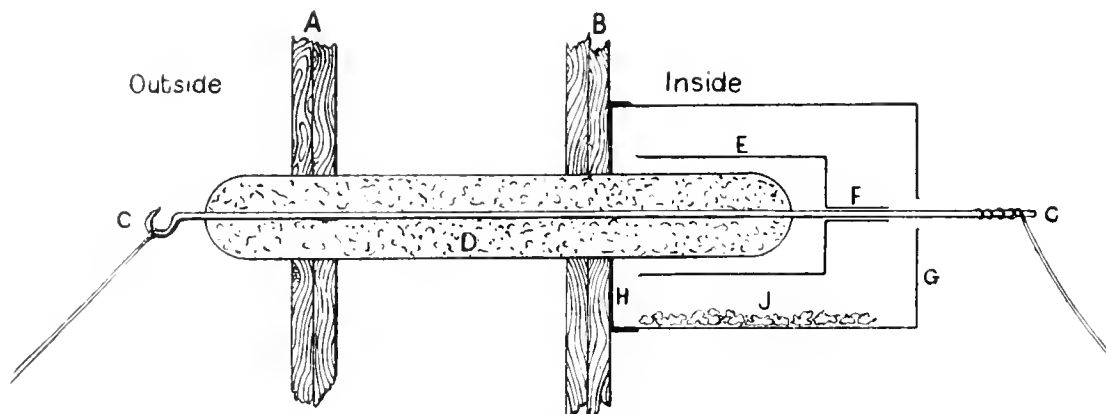
FIG. 90. Insulator through wall.
