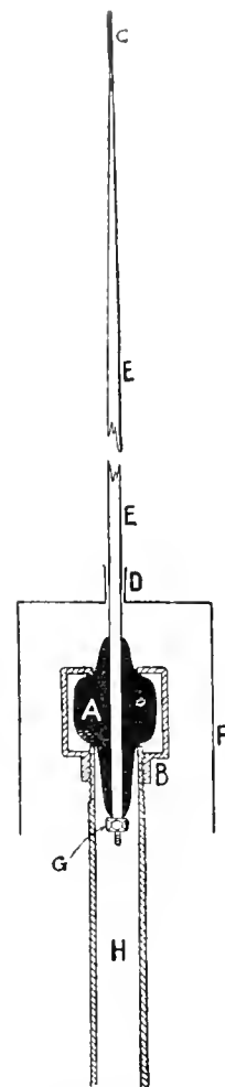
FIG. 89. Insulator for collector rod.
