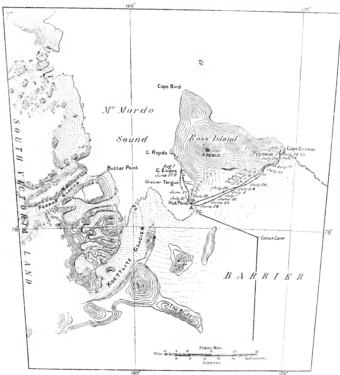
FIG. 2. Map of the Surroundings of Cape Evans.
