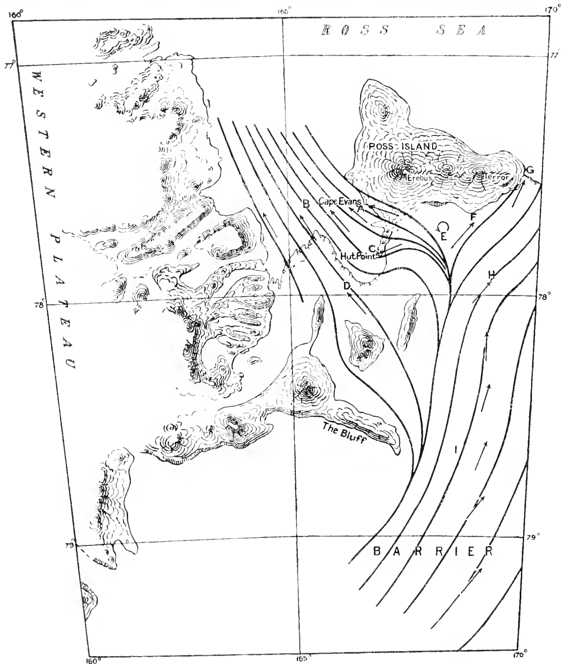
FIG. 37. Wind directions.
