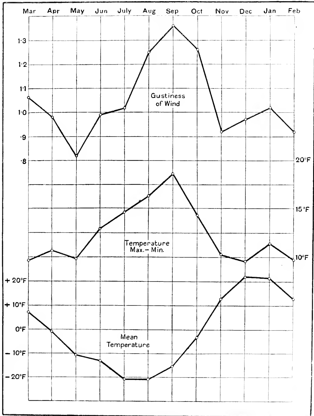
FIG. 40. Gustiness of wind.
