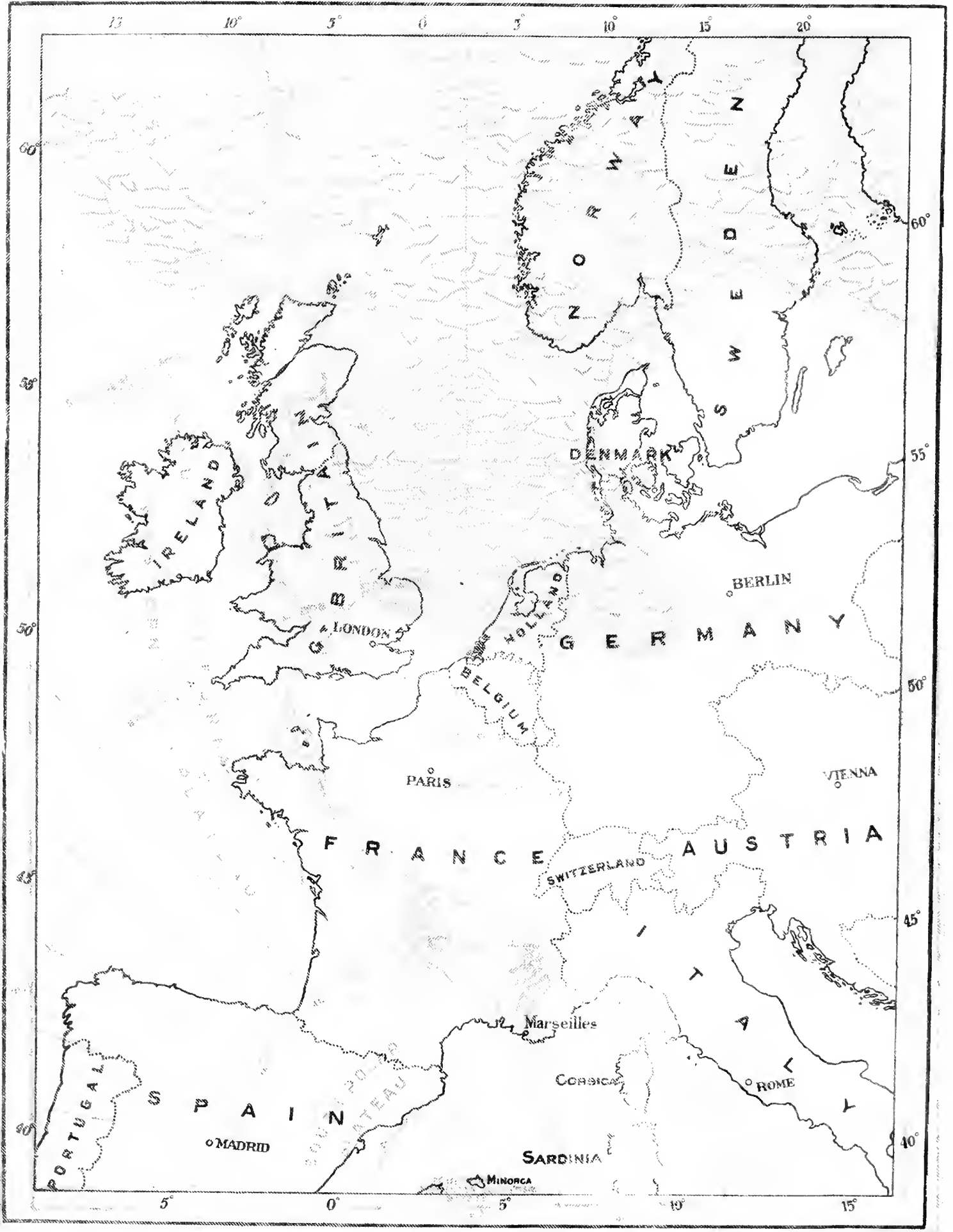
Sketch map of part of Europe drawn to the same scale as the map of the Ross Sea area to which it is attached.
