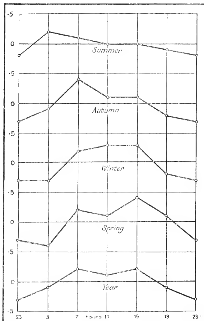
FIG. 52. Daily variation of cloud.
