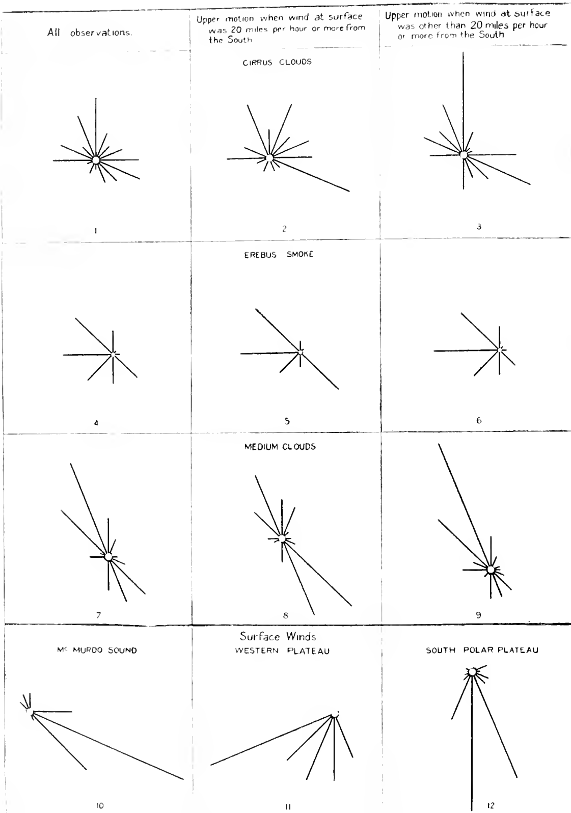
FIG. 47. Motion of atmosphere. Percentage frequency.
