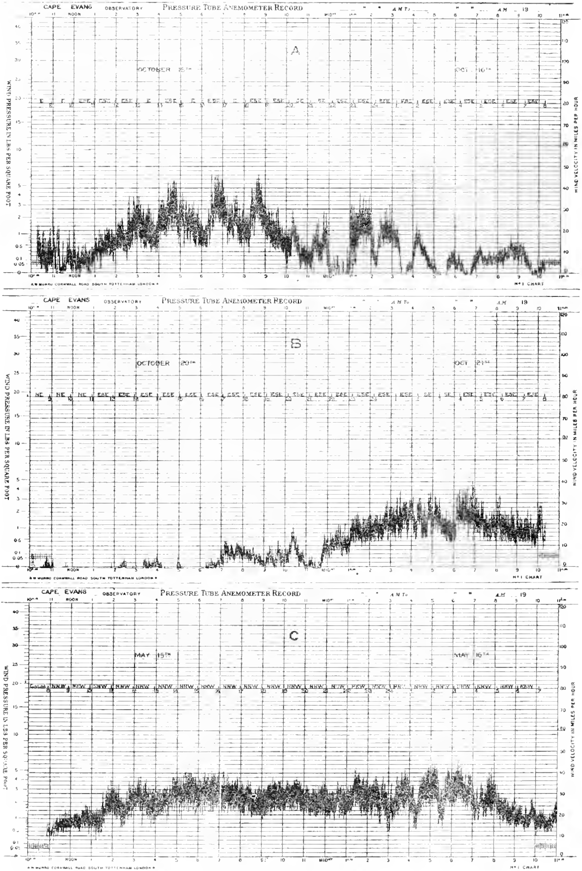
FIG. 11. Anemograms, squalls.
