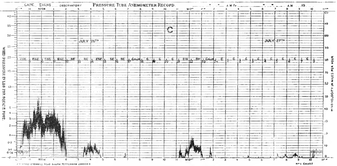
FIG. 42, Anemograms, recrudescences.
