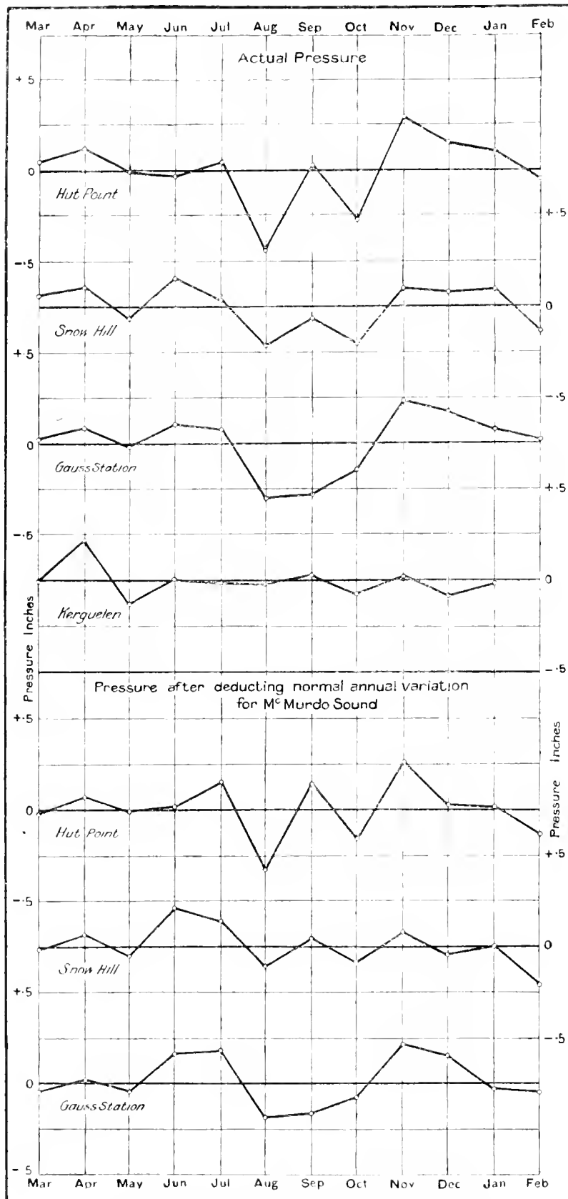
FIG. 60. Comparison of monthly pressure in Antarctic.
