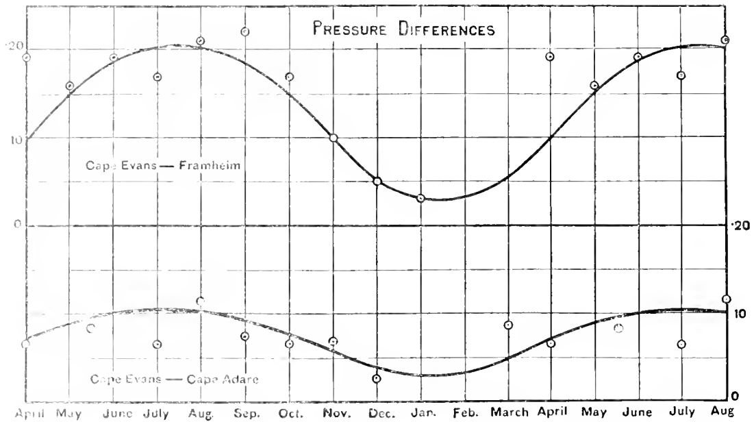
FIG. 57. Pressure differences.
