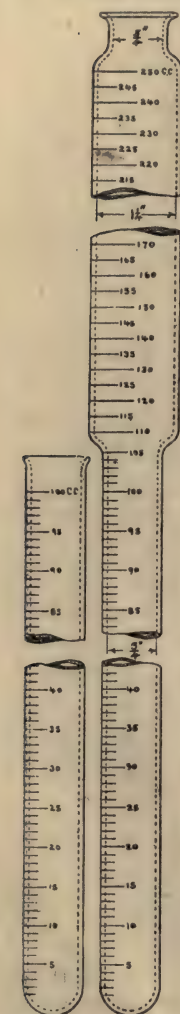
COMPARISON TUBES FOR COLORIMETRIC MANGANESE DETER- MINATIONS.
