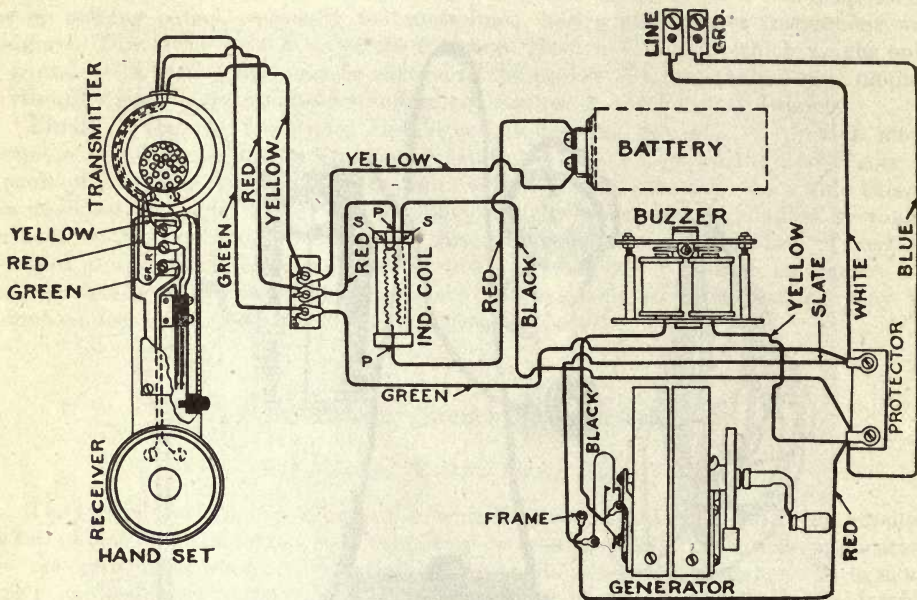
Fig. 63 Wiring diagram of Forestry Branch portable telephone
