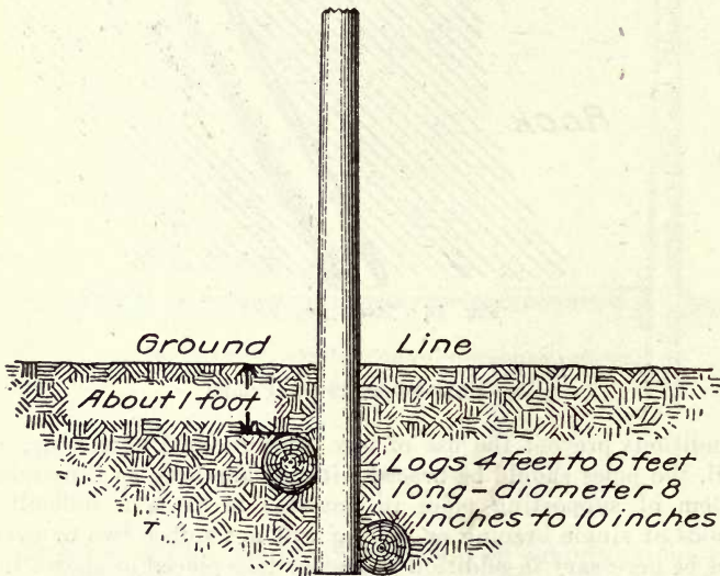
Fig. 17 Method of using guy stub
