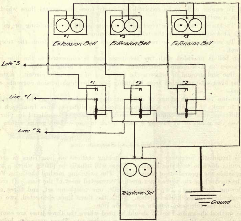
Fig. 55 Switching station, second method
