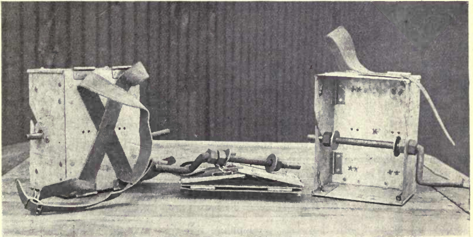
Fig. 36 Emergency wire reel, open and folded
