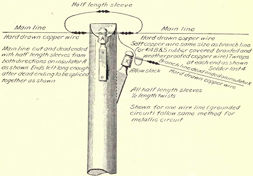
Fig. 39 Method of connecting branch line to main line when both are hard-drawn copper wire
