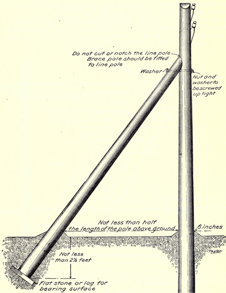
Fig. 14 Method of bracing
