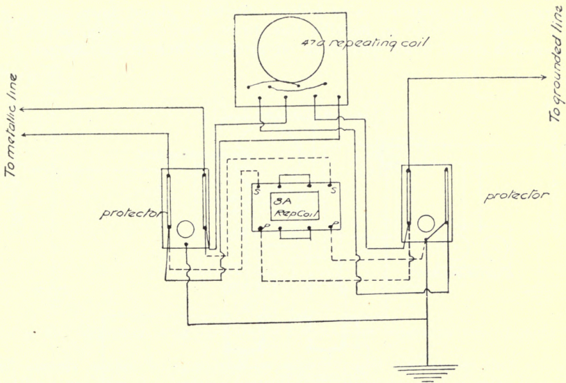
Fig. 58 Connecting grounded line to metallic line through a repeating coil without switches. Dotted lines indicate connections when an 8-A coil is used
