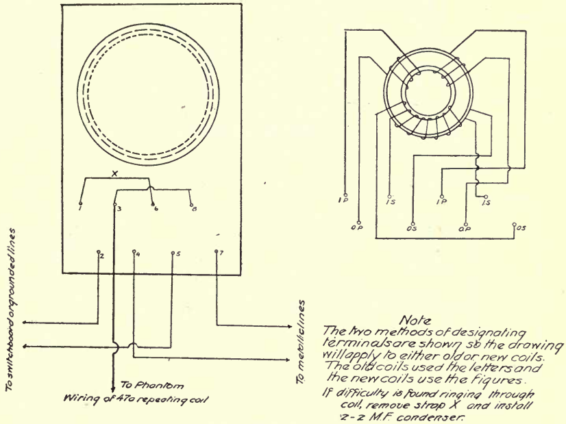
Fig. 56 Wiring and connections on 47-A repeating coil
