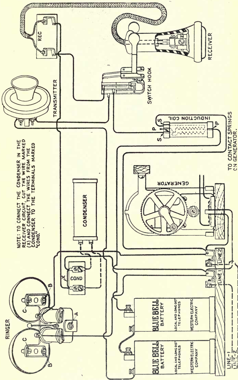
Fig. 47 Wiring diagram of lookout station telephone set
