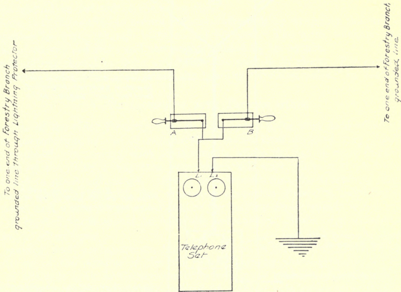
Fig. 92 Method of installing test-station indoors
