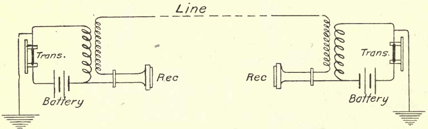
Fig. 77 Diagram of telephone circuit, third stage
