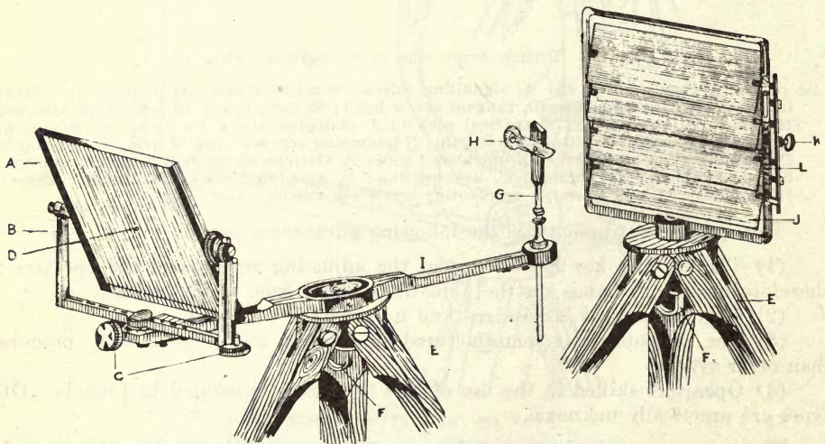
Fig. 101 American Army type of heliograph, two-mirror
