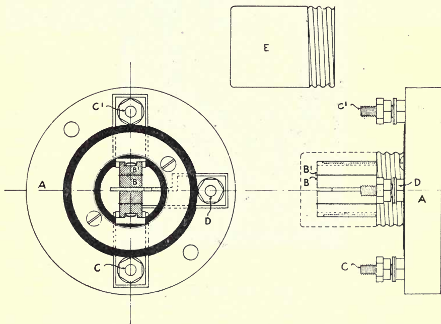
Fig. 83 Lightning protector for use where there are no power or light wires
