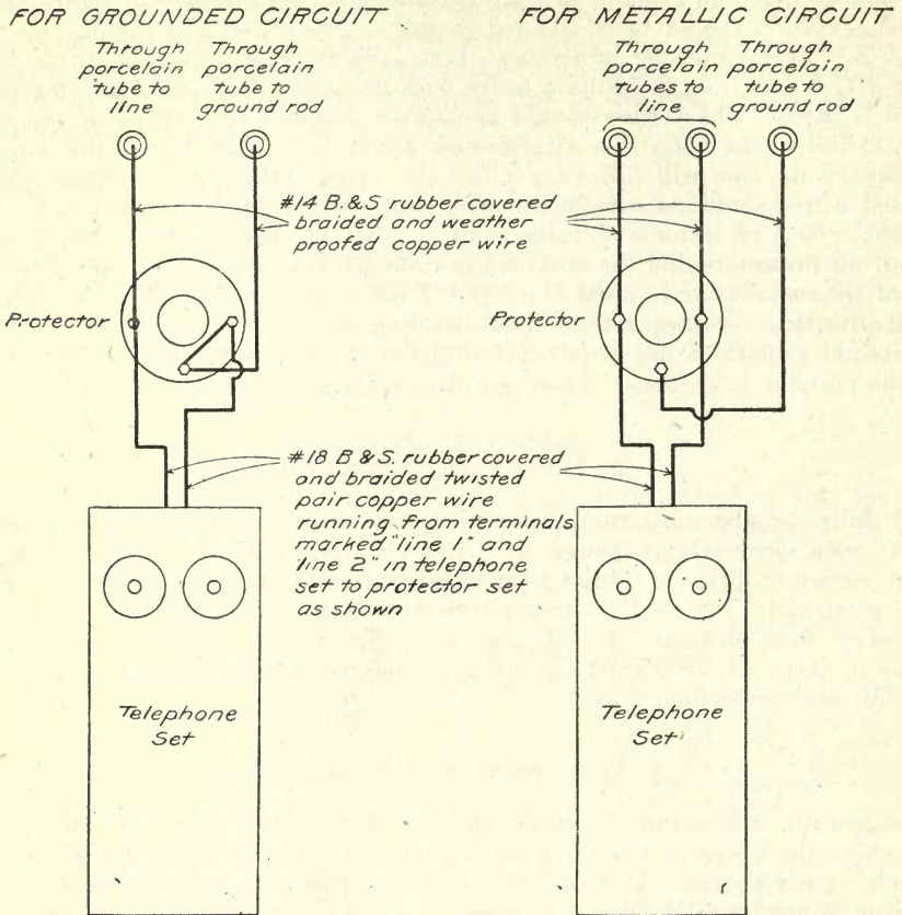
Fig. 45 Wiring diagram for telephone station
