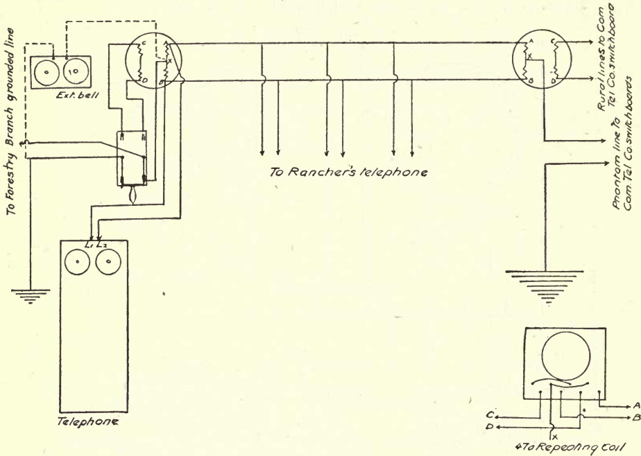
Fig. 57 Phantom circuit
