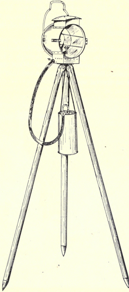
Fig. 106 Acetylene signal-lantern with tripod
