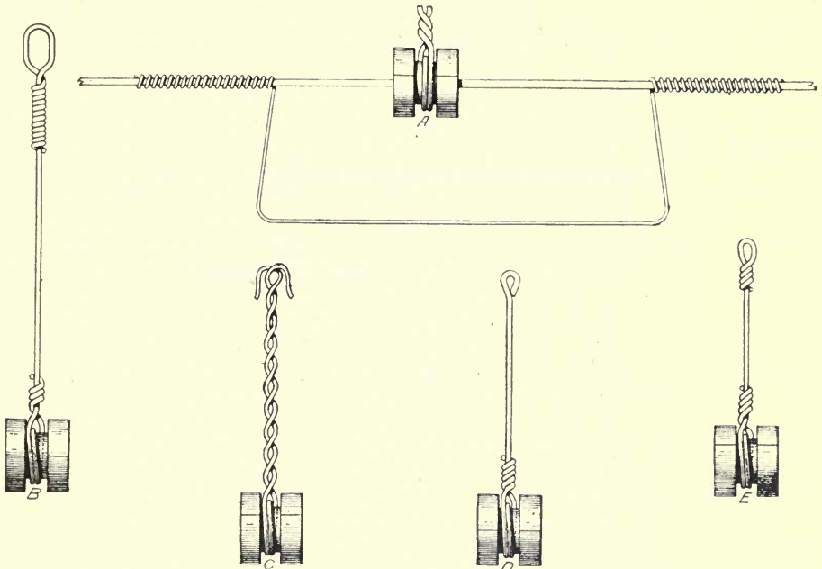
Fig. 32 Split tree insulator attachment and crosstie
