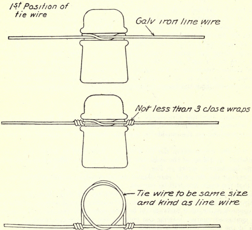
Fig. 23 Method of making "figure 8" tie for iron wire
