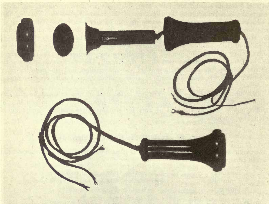
Fig. 70 Bipolar hand receiver
