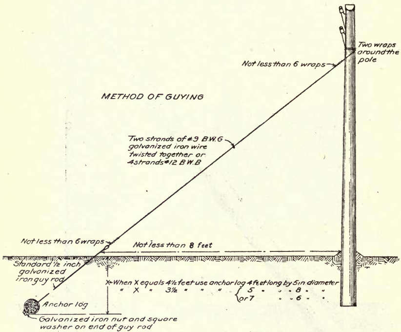
Fig. 15 Method of guying
