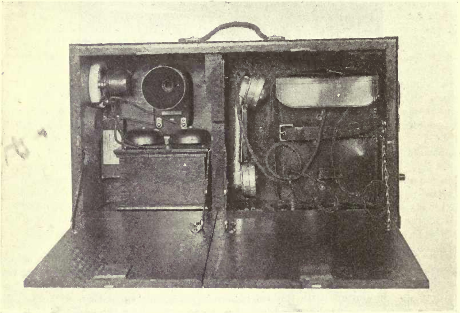
Fig. 67 Forestry Branch emergency communication kit No. 1-A
