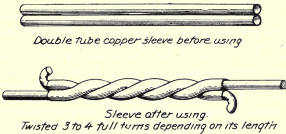
Fig. 29 Method of splicing hard-drawn copper wire
