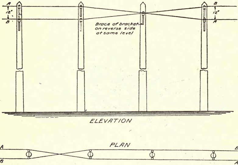
Fig. 21 Transposition of wires, metallic circuit
