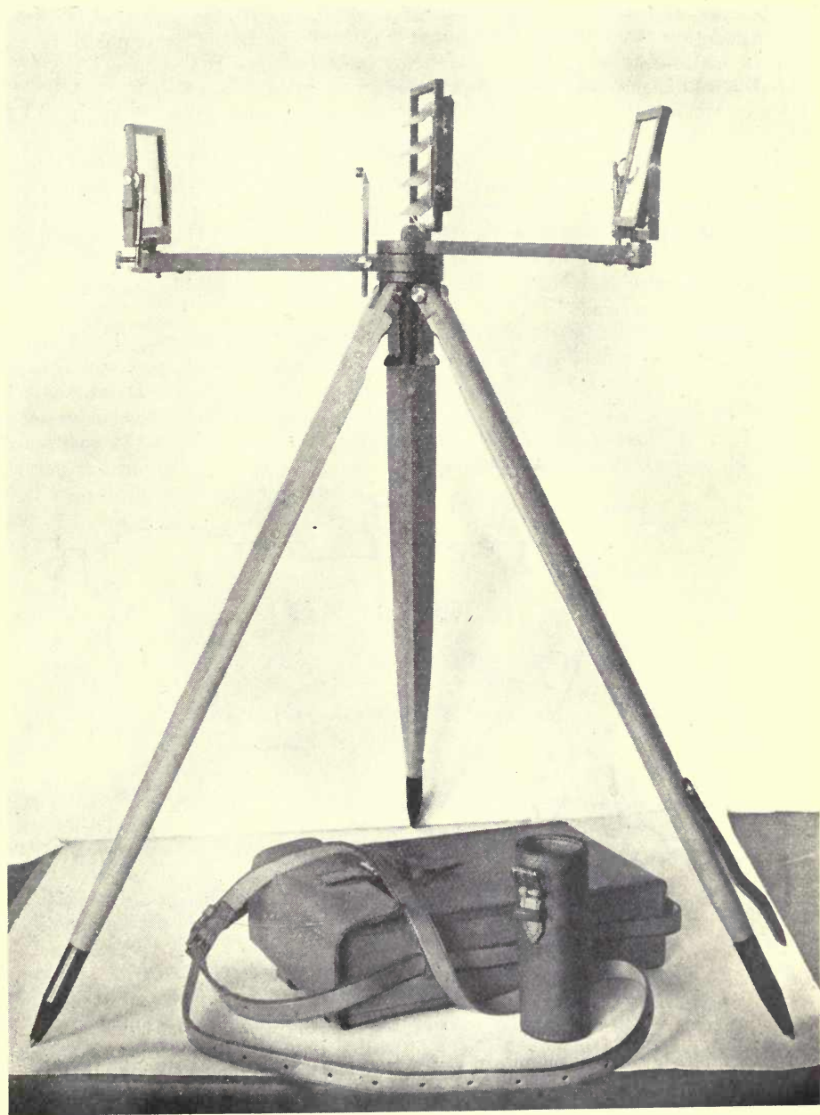
Fig. 103 Forest Service type of heliograph, two-mirror
