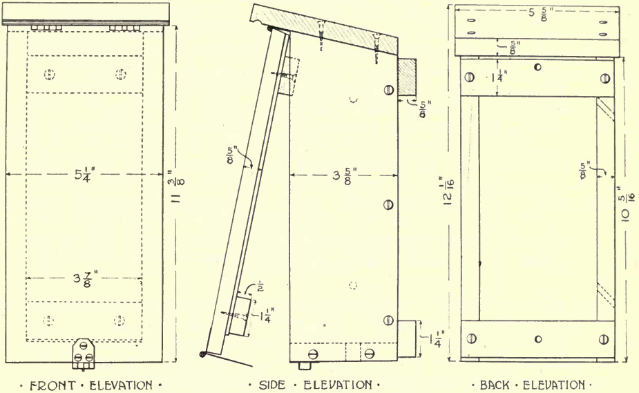
Specifications 12 Design of outdoor protector mounting-box
