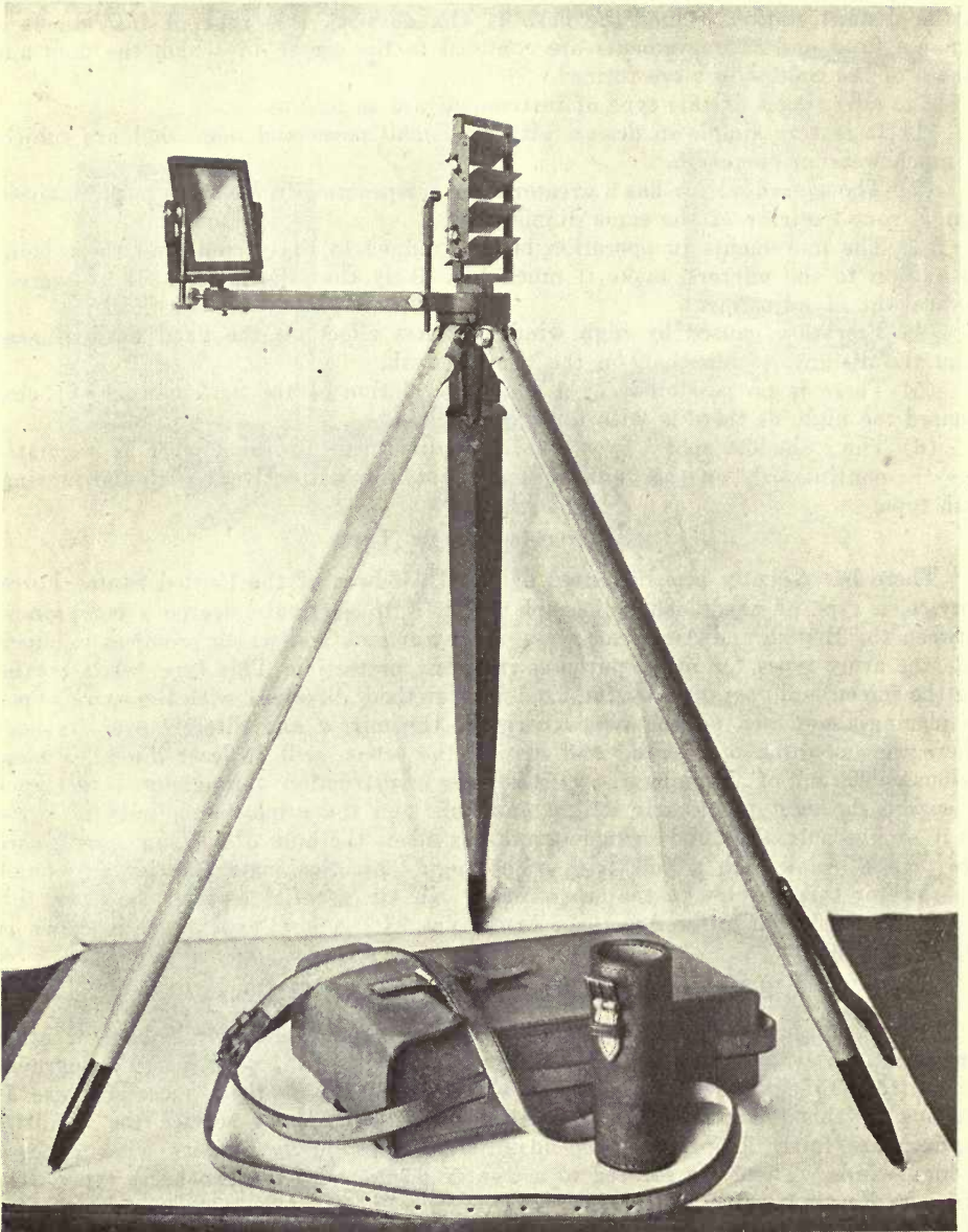
Fig. 102 Forest Service type of heliograph, one-mirror
