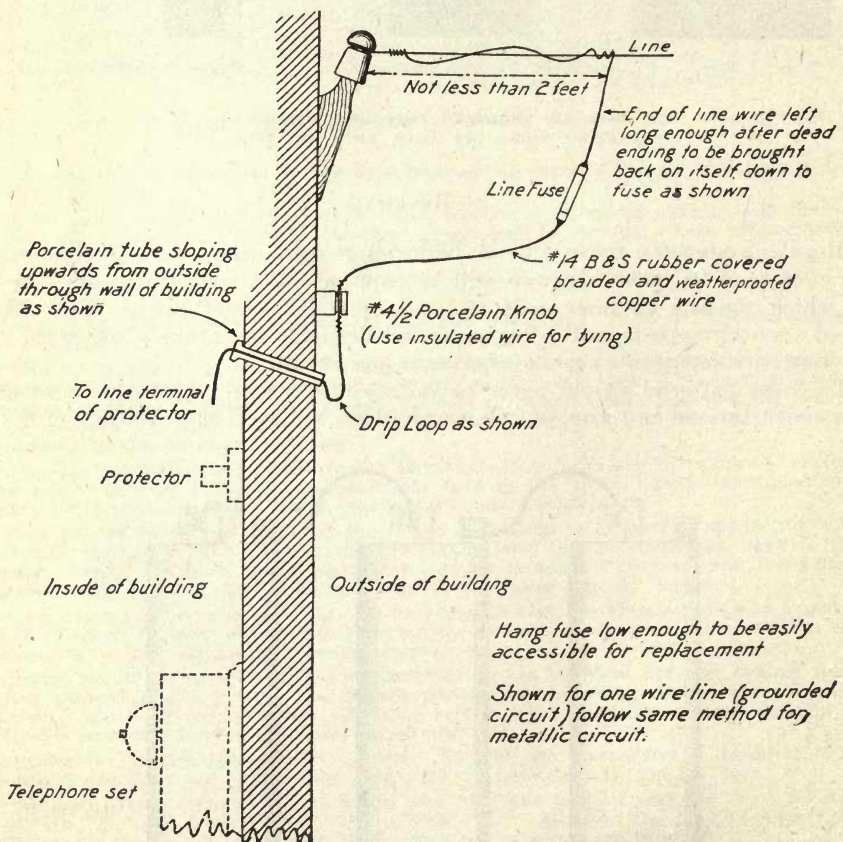
Fig. 44 Method of installing line fuse when required
