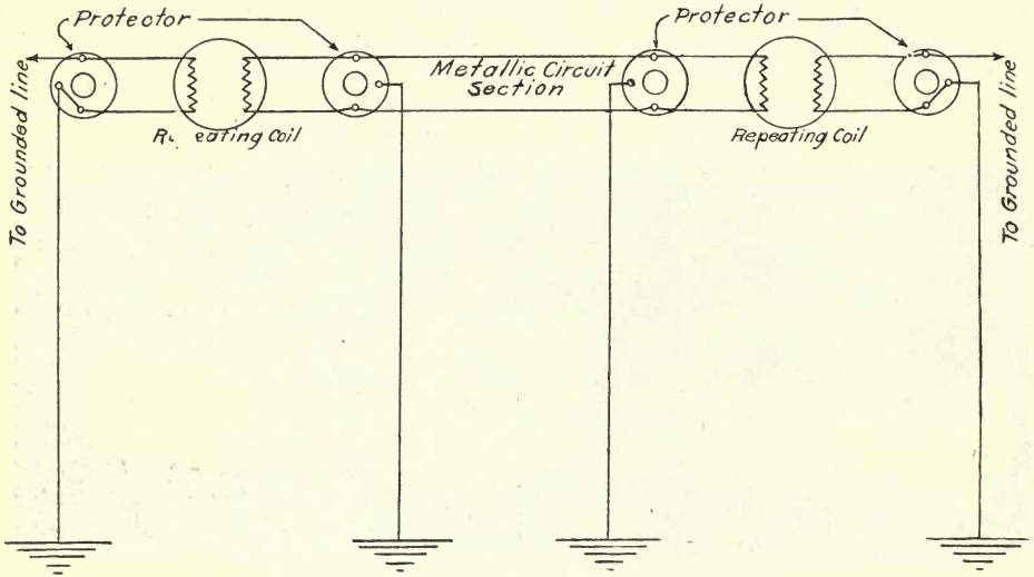
Fig. 86 Method of inserting a metallic circuit section in a grounded line to overcome induction disturbances
