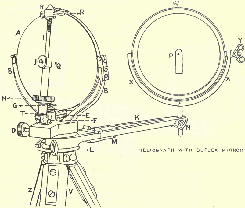
Fig. 99 British Army type of heliograph, two-mirror
