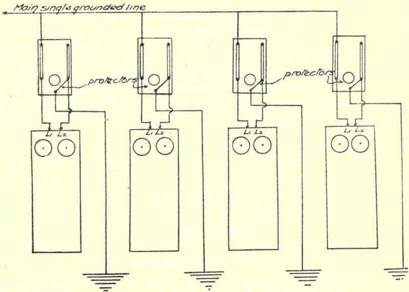
Fig. 90 Connecting bridging telephone on a grounded line
