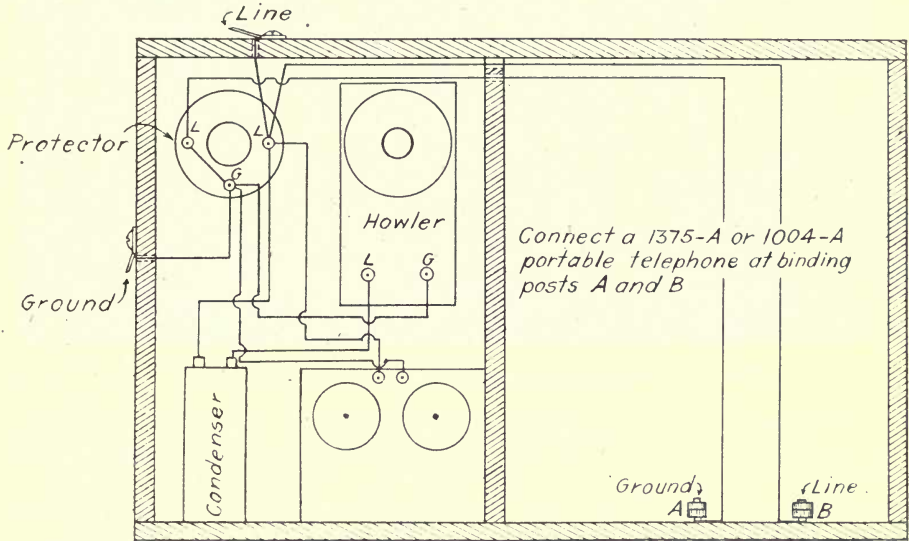
Fig. 68 Wiring diagram of the No. 1-A kit
