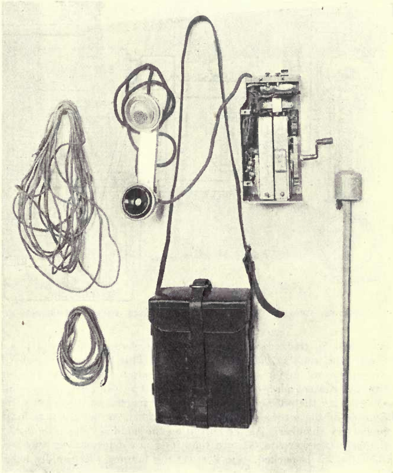
Fig. 62 Forestry Branch portable telephone set (1375-A) with ground rod and connector
