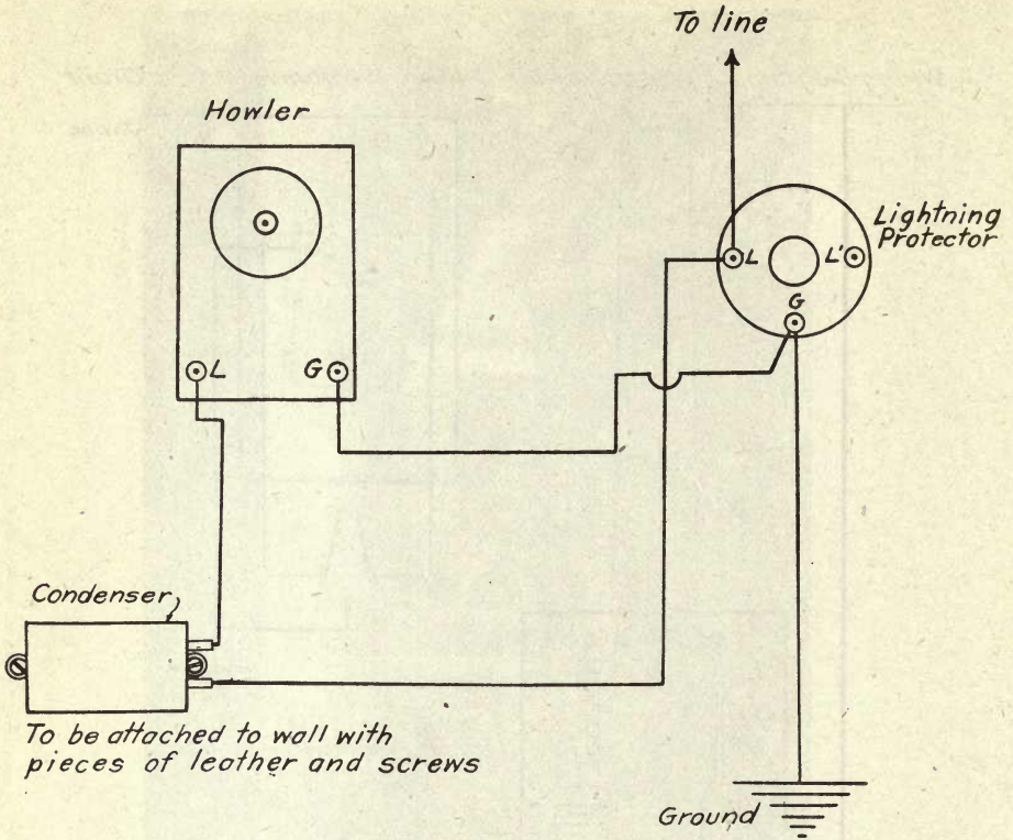
Fig. 50 Method of connecting howler and condenser
