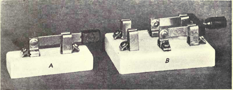
Fig. 85 Baby knife-switches. (A) Single pole, single throw (S.P.S.T.). (B) Double pole, double throw (D.P.D.T.)
