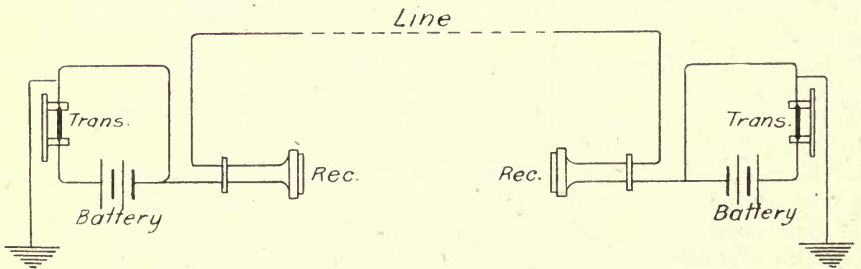
Fig. 75 Diagram of telephone circuit, second stage
