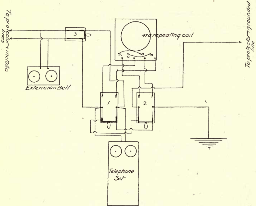
Fig. 60 Connecting grounded to metallic line by use of switches and one telephone
