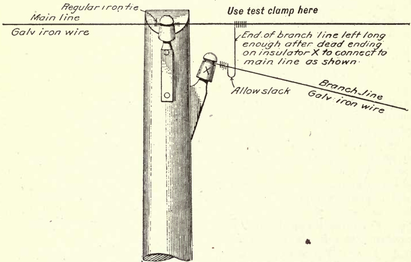
Fig. 38 Method of connecting branch line to main line when both are galvanized-iron wire
