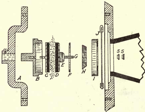
Fig. 74 Details of the solid-back transmitter
