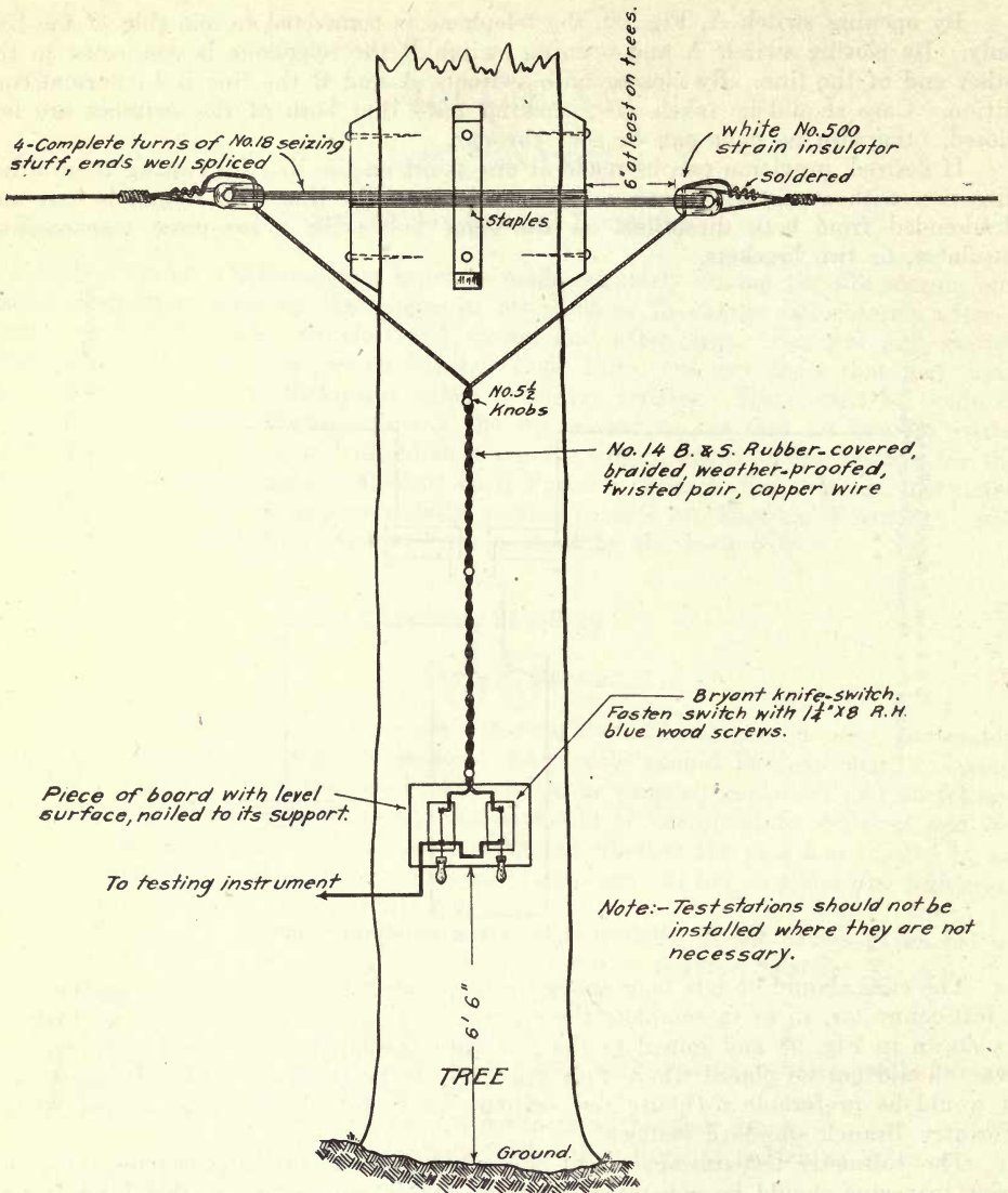
Fig. 93 Method of installing test-station on a tree
