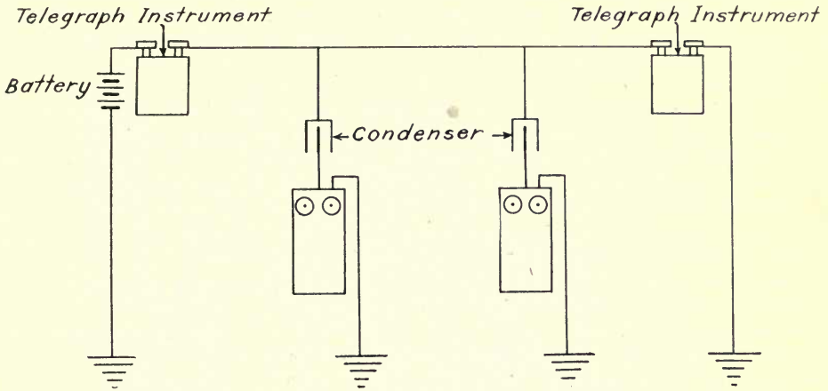
Fig. 61 Method of using one wire for simultaneous telegraphy and telephony
