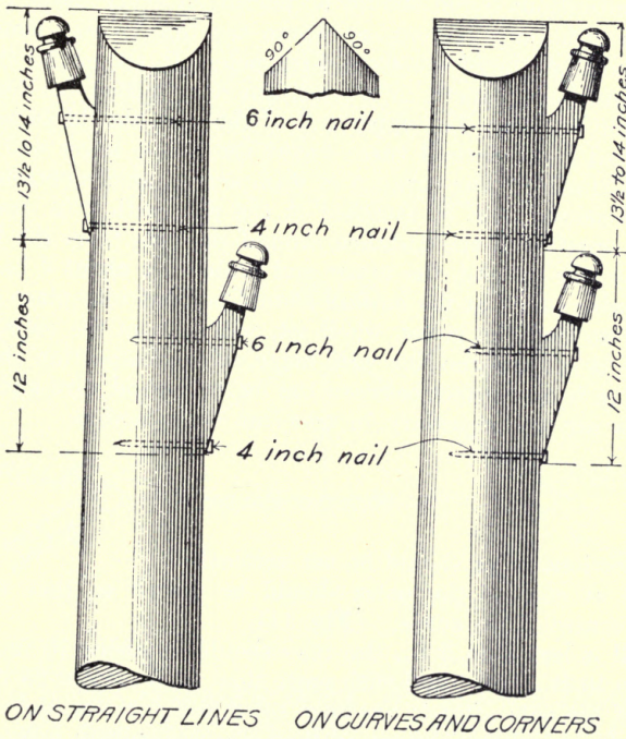
Fig. 10 Location of brackets on pole
