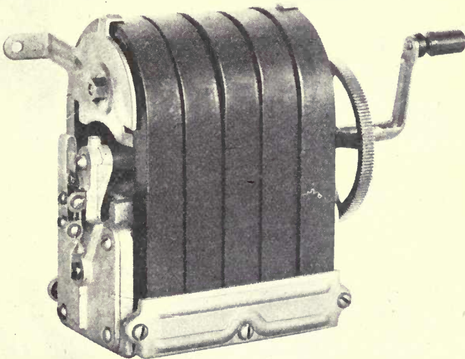
Fig. 78 Magneto generator, five bar
