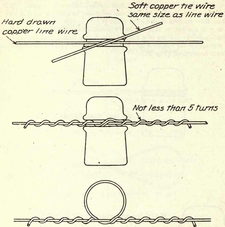
Fig. 26 Method of making regular tie for hard-drawn copper wire
