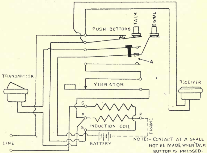
Fig. 65. Wiring diagram of the Adams hand set (1004-A)
