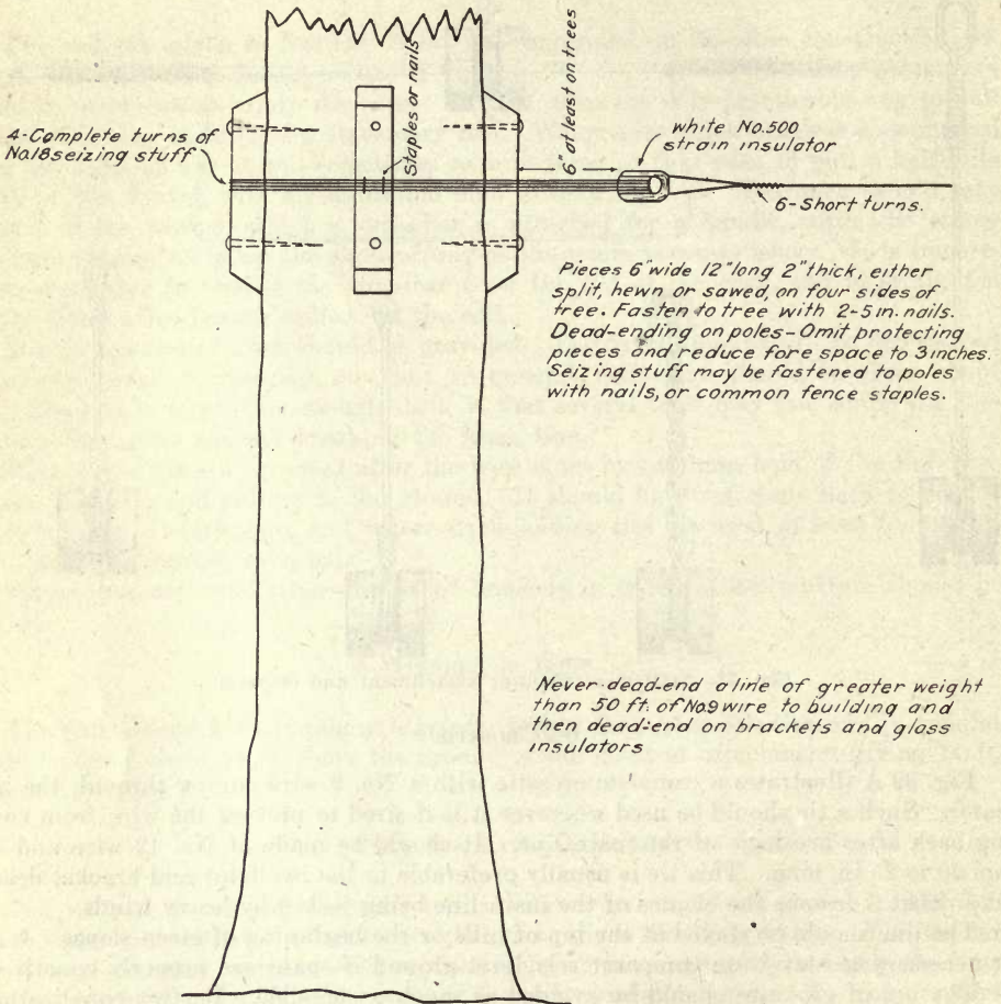
Fig. 33 Method of dead-ending on tree lines
