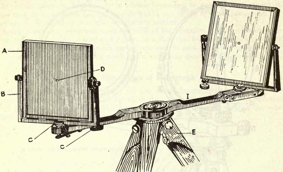
Fig. 100 American Army type of heliograph, one-mirror
