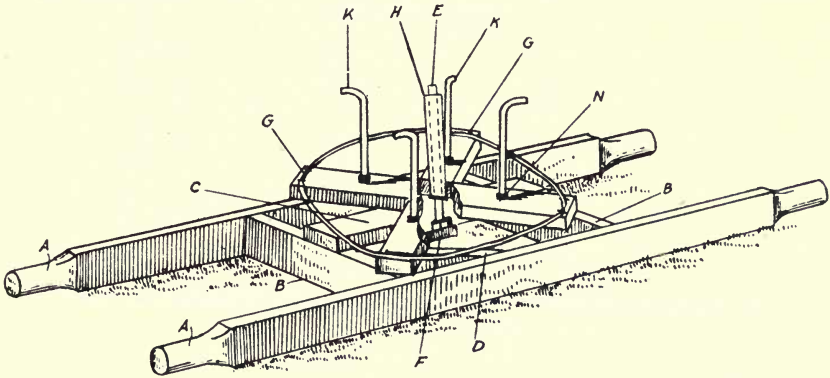
Fig. 20 Home-made reel
