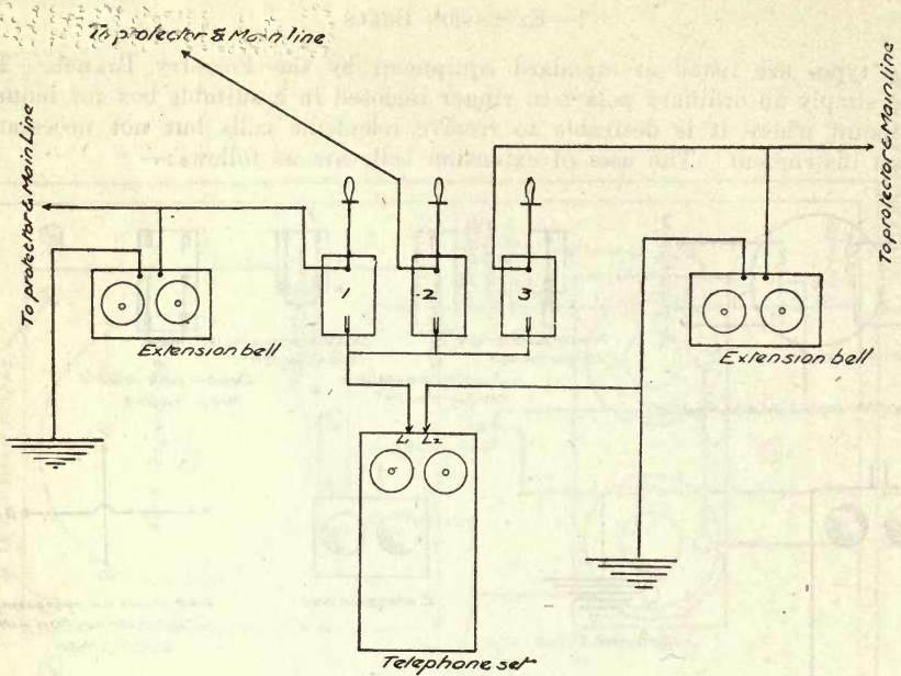
Fig. 54 Switching station, first method
