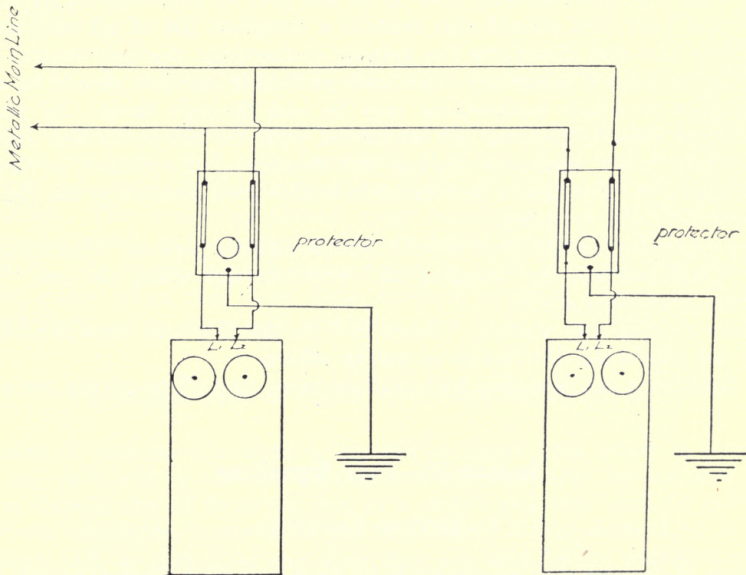
Fig. 91 Connecting bridging telephone on a metallic line
