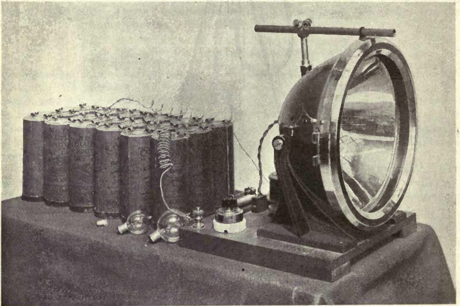
Fig. 107 Fischer high-power electric signalling lamp
