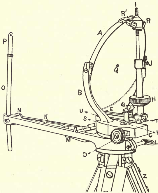
HELIOGRAPH WITH SIGHTING VANE.
