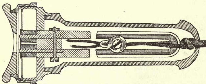
Fig. 71 Longitudinal section of bipolar receiver
