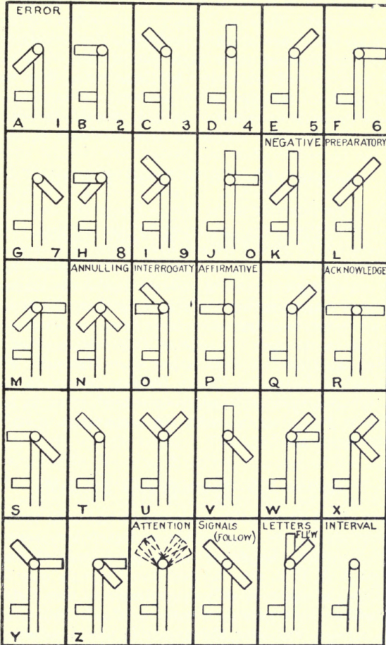
Fig. 112 Two-arm, fixed semaphore code
