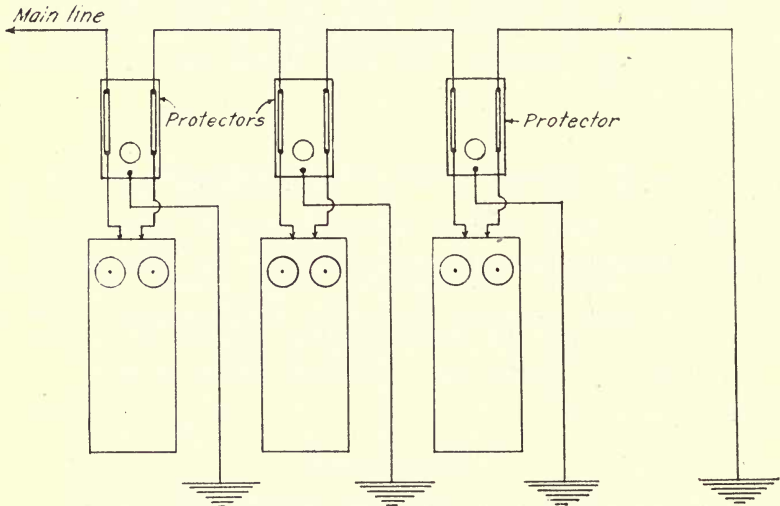
Fig. 89 Telephones connected in series on a grounded line
