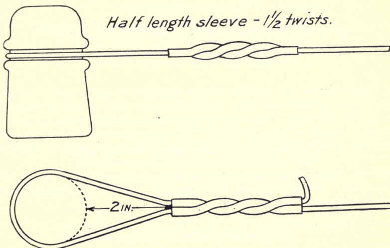
Fig. 25 Method of dead-ending hard-drawn copper wire
