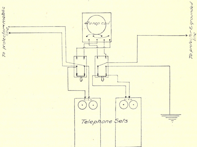
Fig. 59 Connecting grounded line to metallic line by use of switches and two telephones
