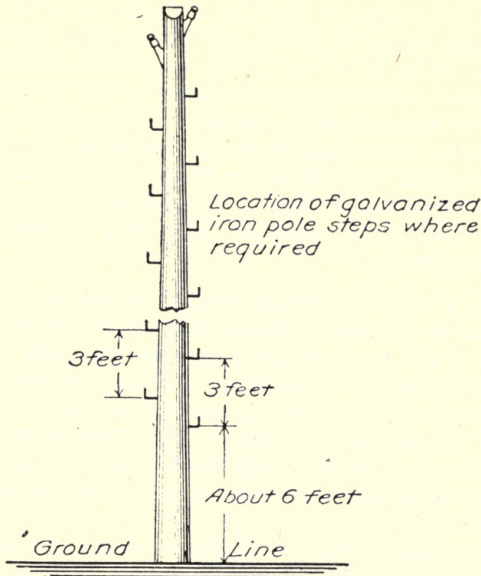
Fig. 9 Pole-steps
