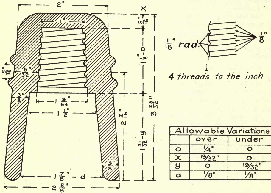
Specifications 6 Design of Forestry Branch standard pony glass insulator
