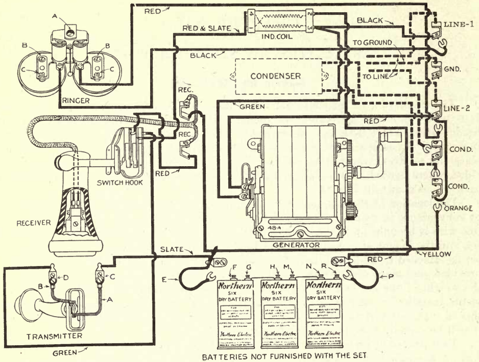
Fig. 41 Wiring diagram and directions for assembling standard wall telephone set
