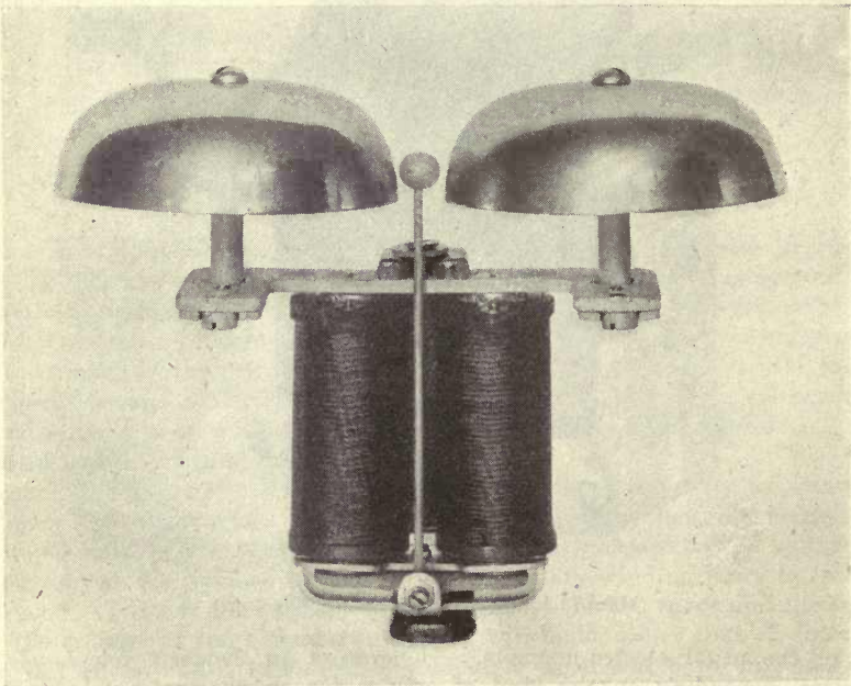
Fig. 79 Polarized ringer, unbiased type
