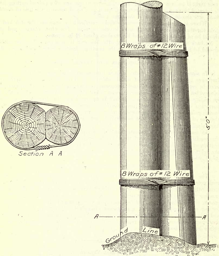
Fig. 94 Stub reinforcement of poles
