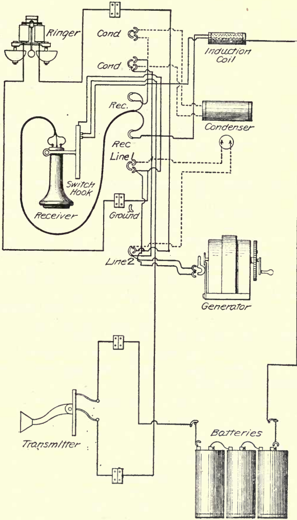
Fig. 97 Wiring of No. 1317 telephone set
