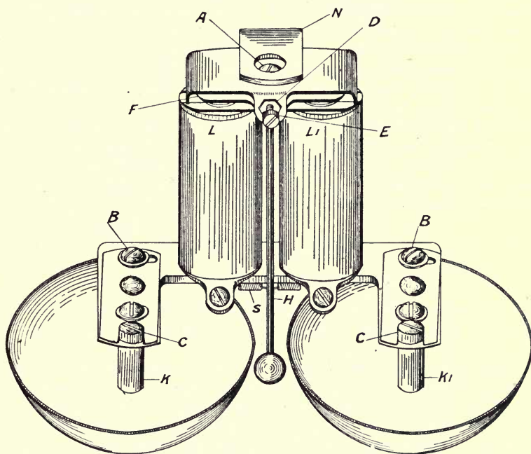
Fig. 96 Ringer of No. 127-F, extension bell, and Nos. 1317-P, 1317-S, 300-N and 1336-J telephones
