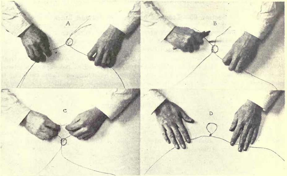
Fig. 35 Method of making temporary splice in emergency wire
