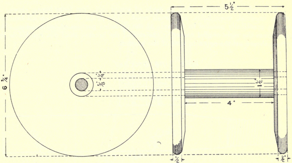
Sketch of Emergency Wire Spool
