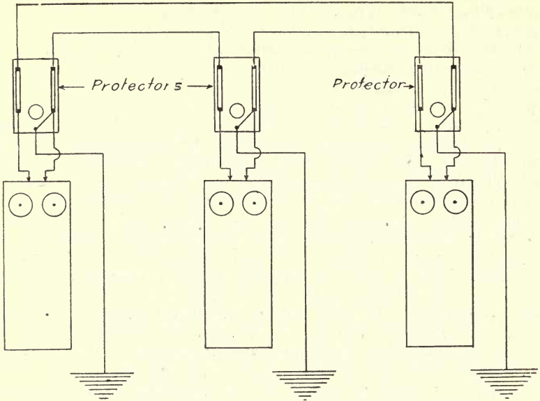
Fig. 88 Telephones connected in series on a metallic line
