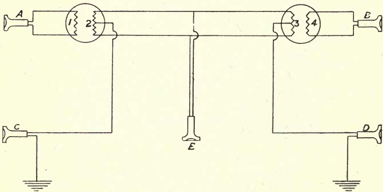
Fig. 87 Diagram of a phantom circuit
