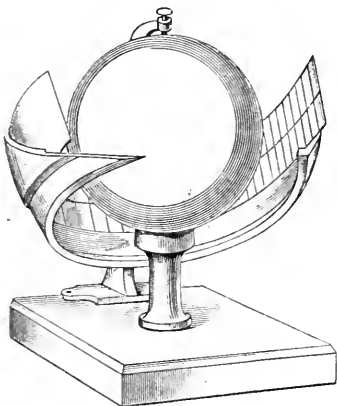
Fig. 10. Sonnenscheinautograph.
