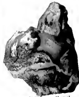
9 Plattiges Mineral
