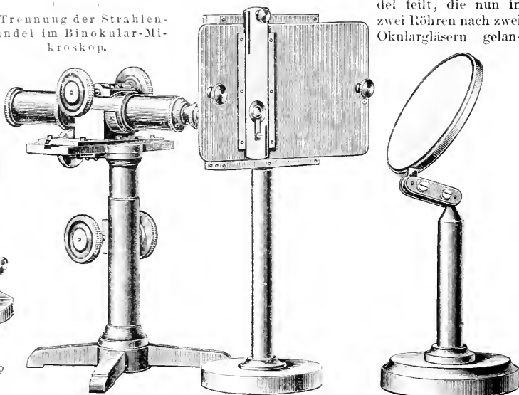
12. Aquarium-Mikroskop.
